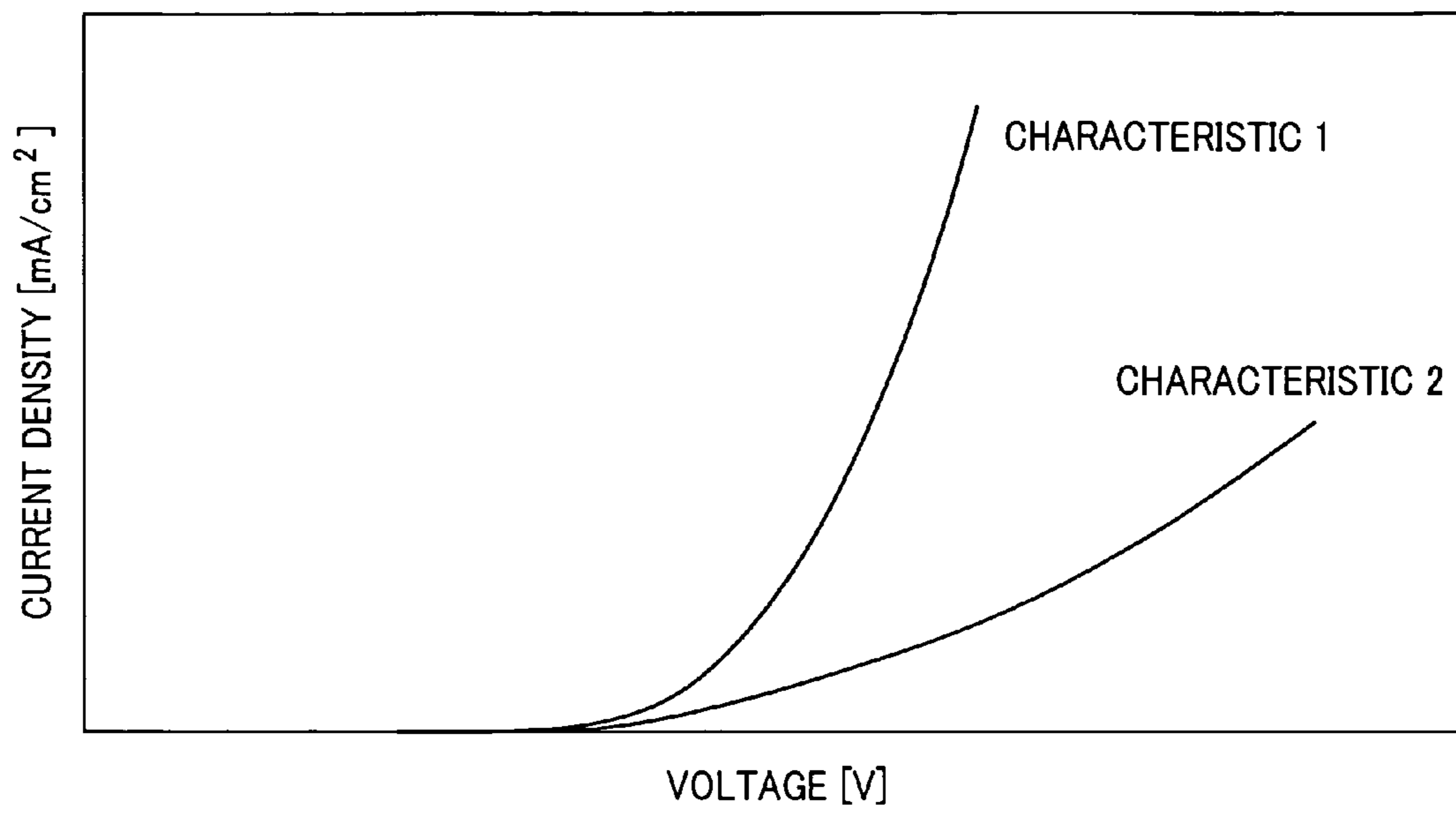
VOLTAGE VS CURRENT DENSITY
