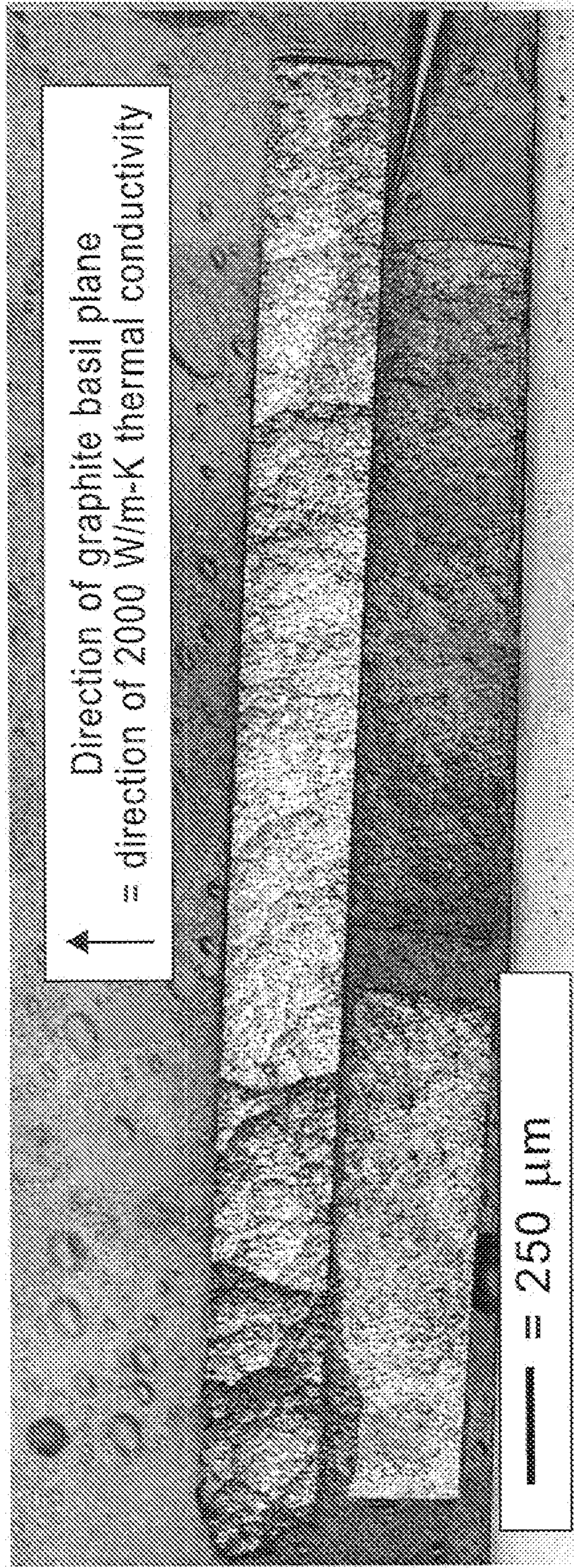
Cross section of graphite blocks
