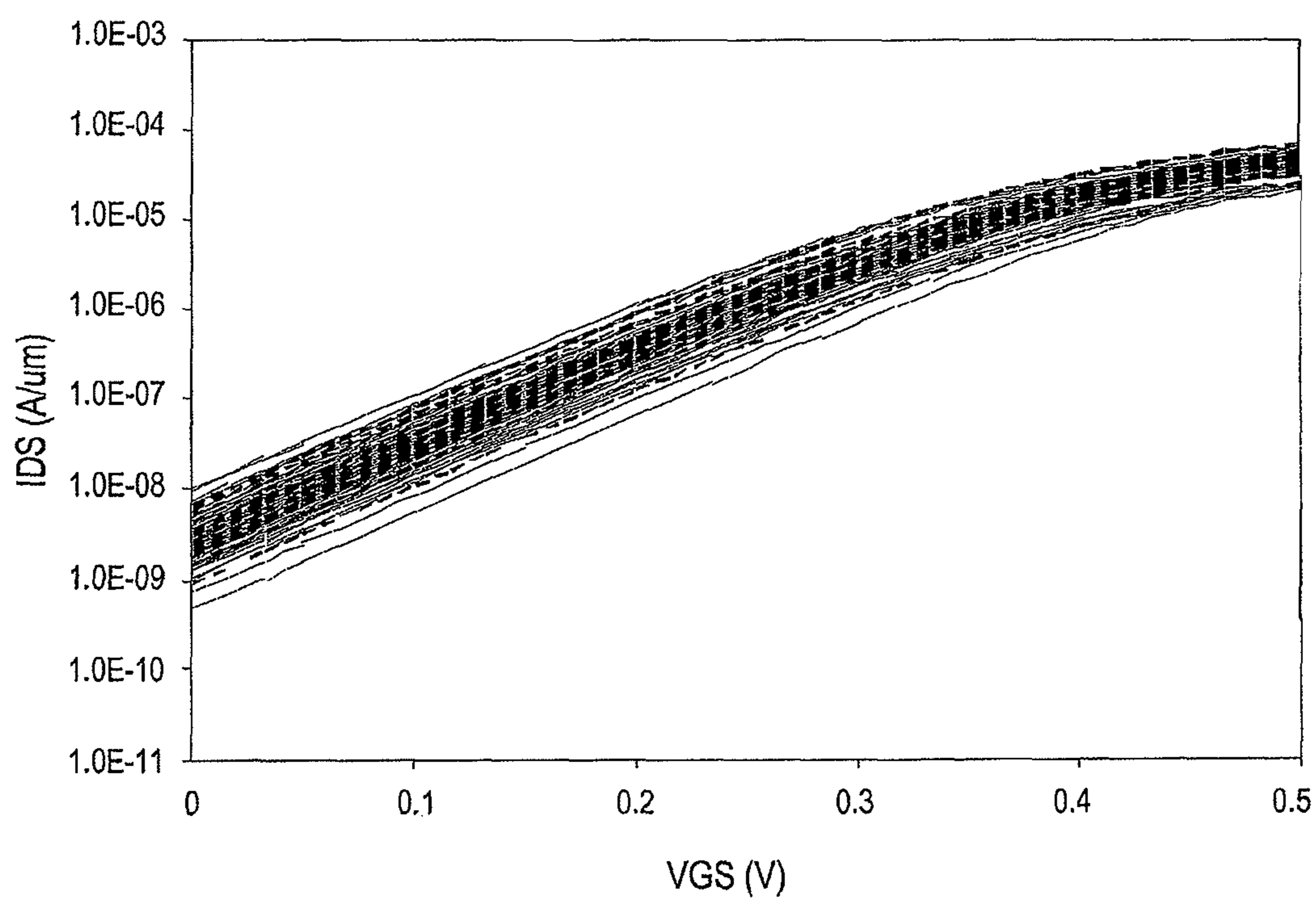
IDS-VGS Characteristics as a Result of RDF in Deeply-Depleted-Channel nMOS with V_{BS}=0V
