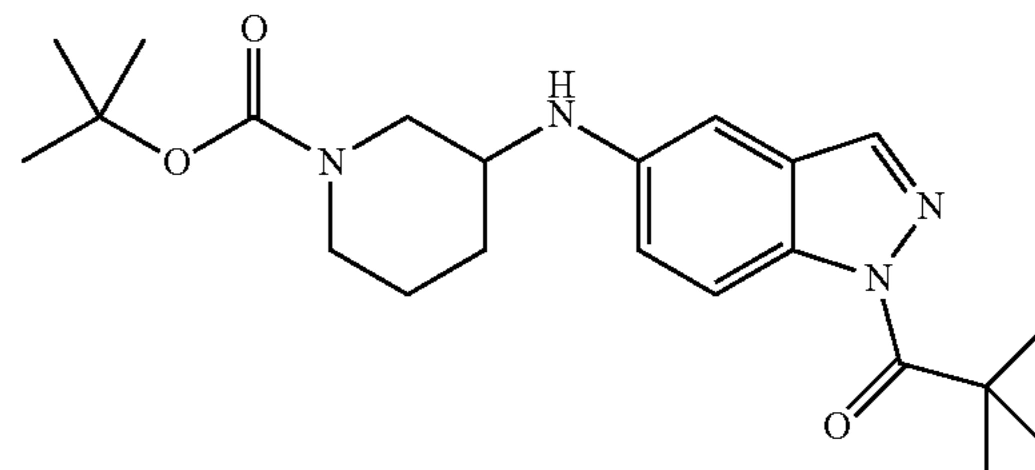
tert-Butyl 3-(1-Pivaloyl-1H-indazol-5-ylamino)piperidine-1-carboxylate
