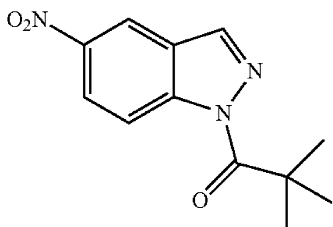
2,2-Dimethyl-1-(5-nitro-1H-indazol-1-yl)propan-1-one
