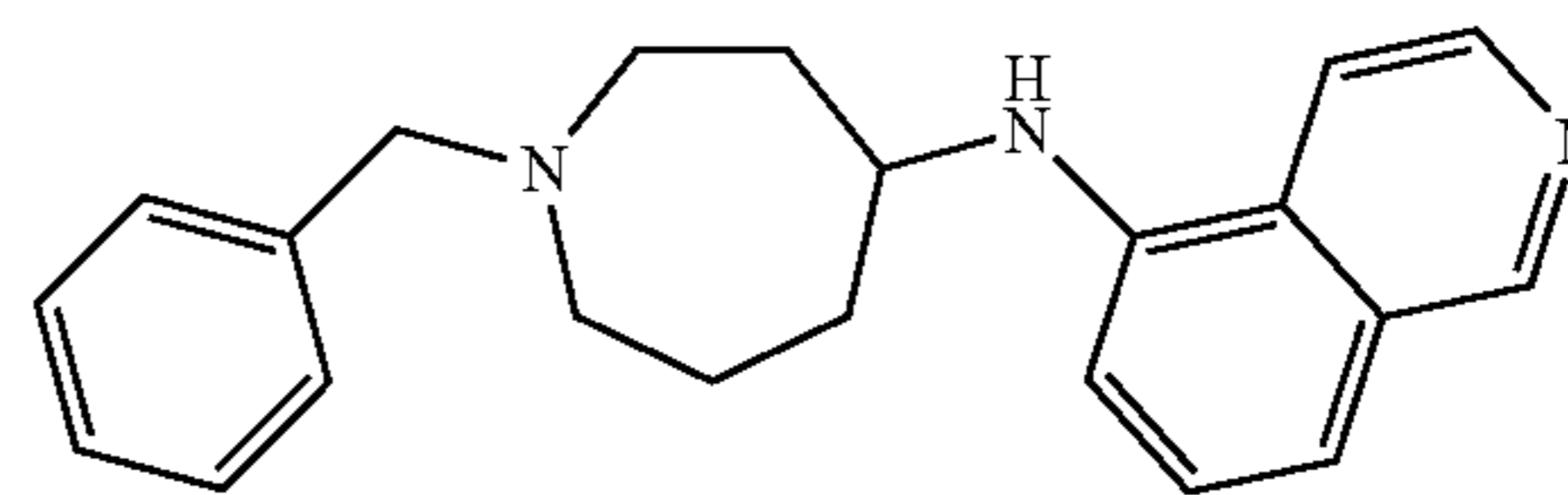
N-(1-Benzylazepan-4-yl)isoquinolin-5-amine, Compound 2.013
