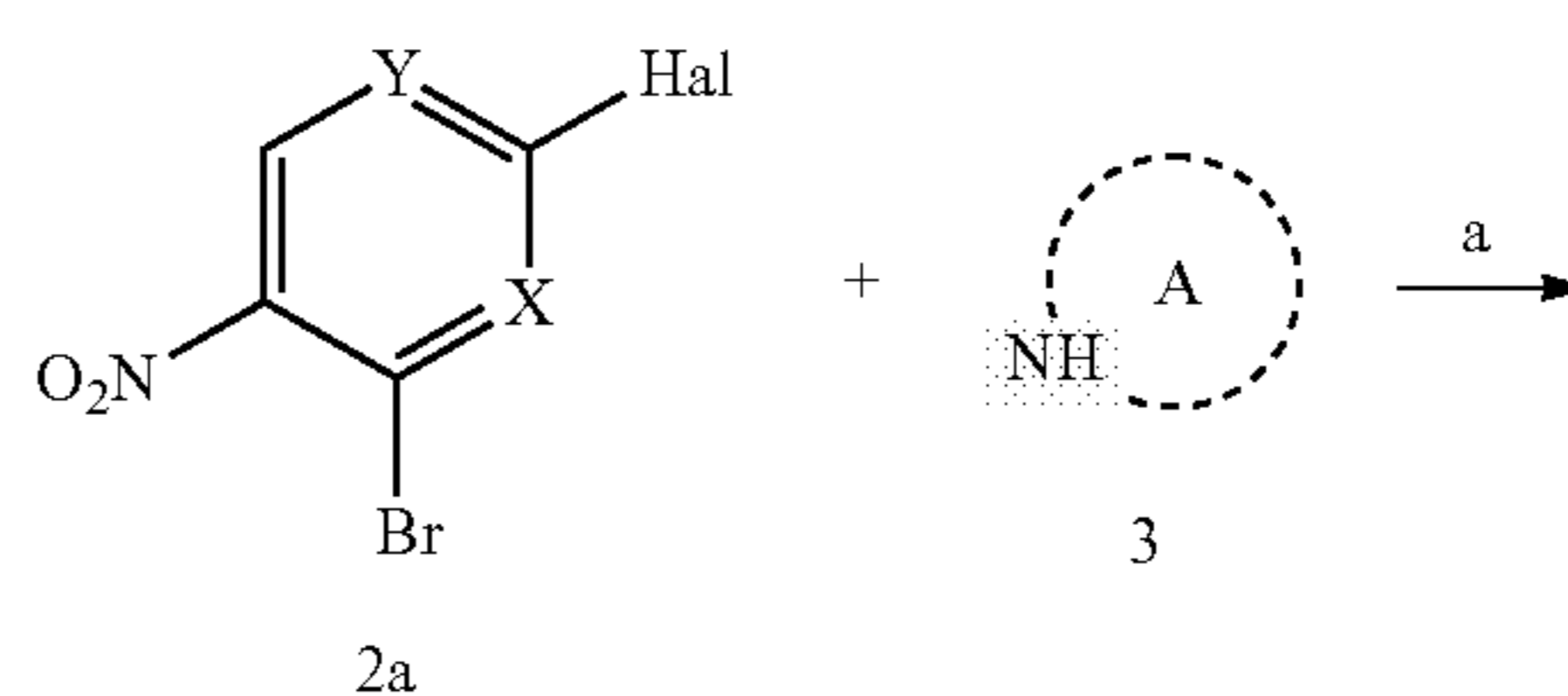
Scheme 2. Preparation of Compounds of Formula I
