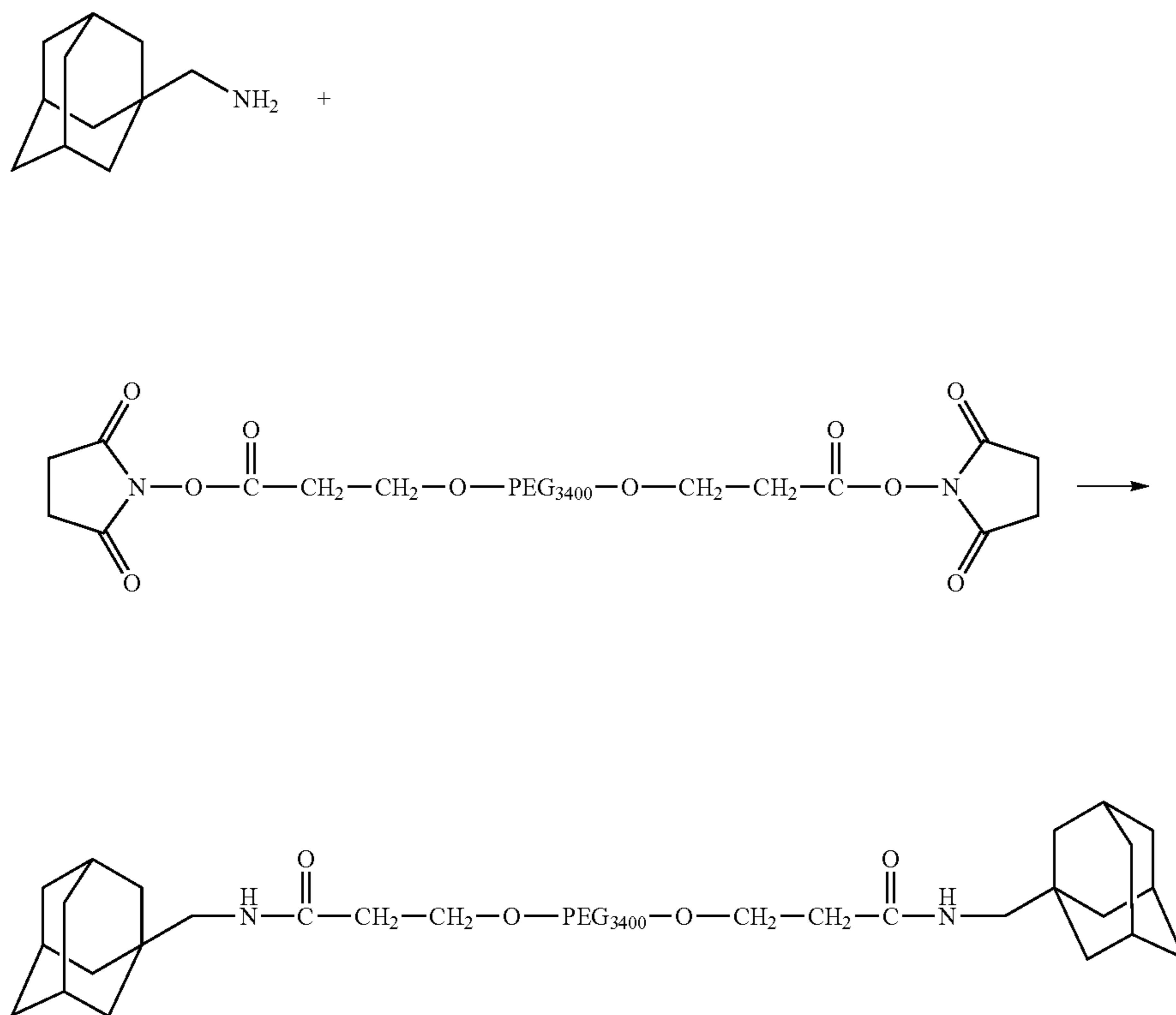
Scheme XXXXVI
