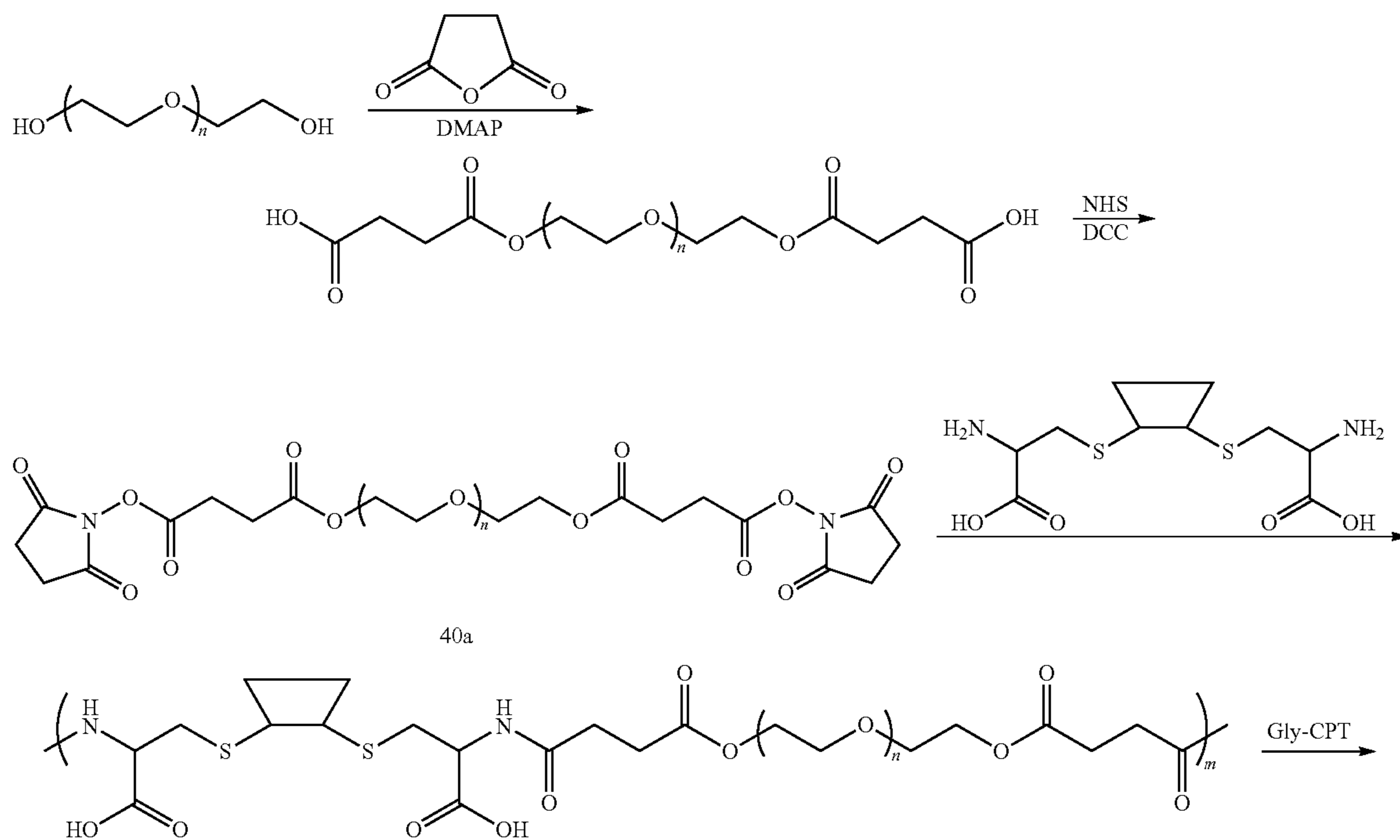
Scheme XXXXI
