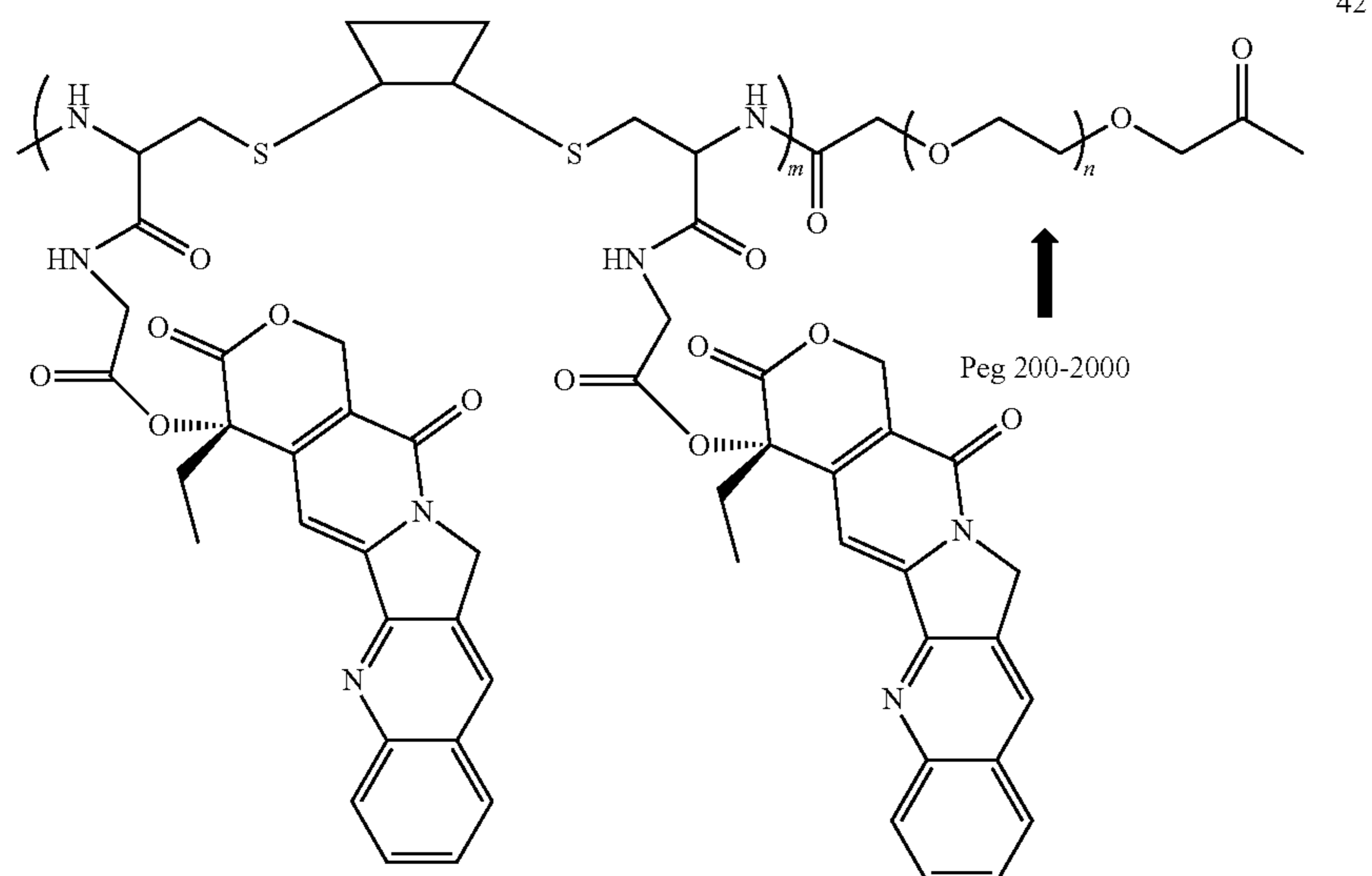
Scheme XXXXII
