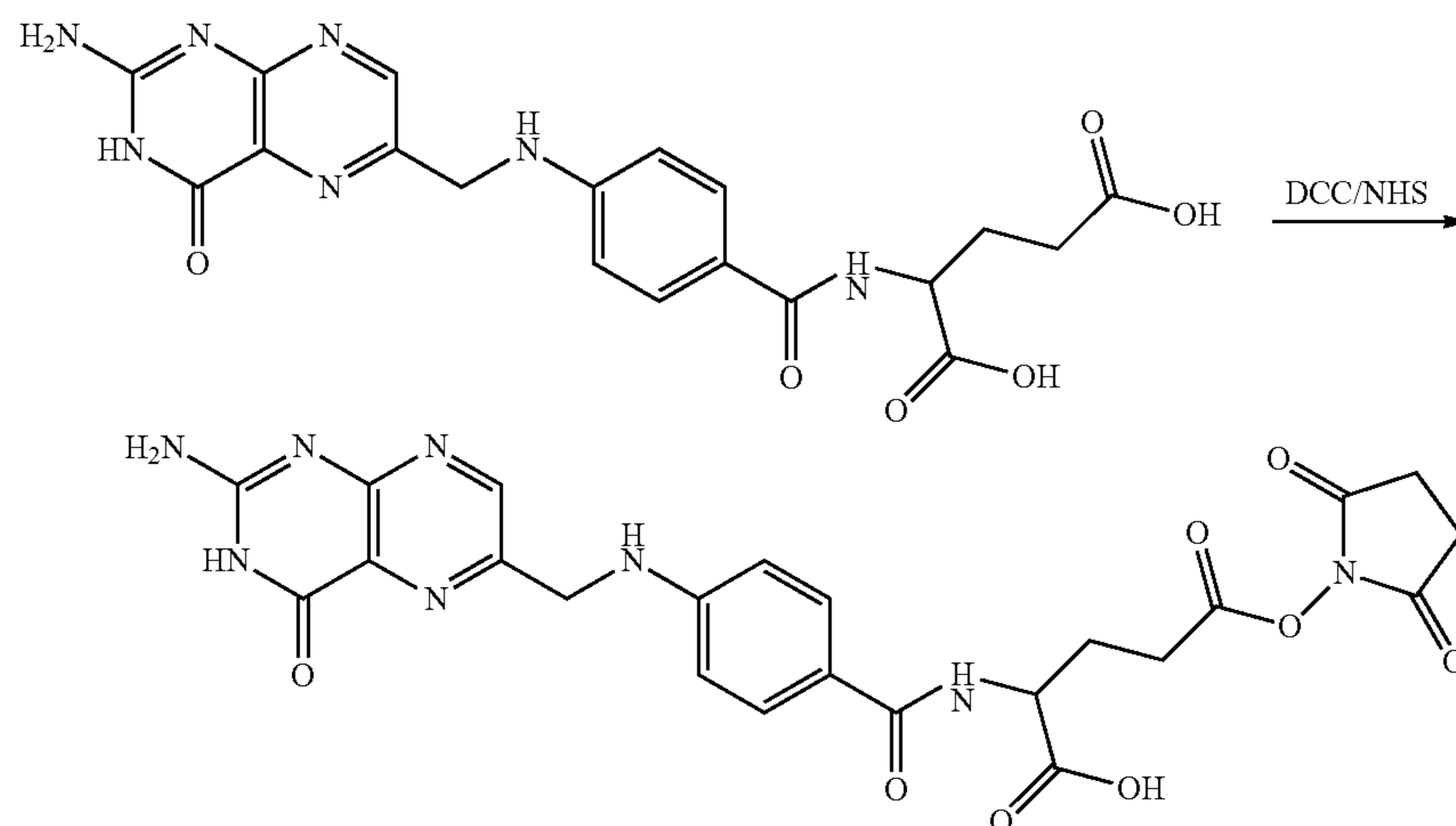
Scheme XXXXIX
