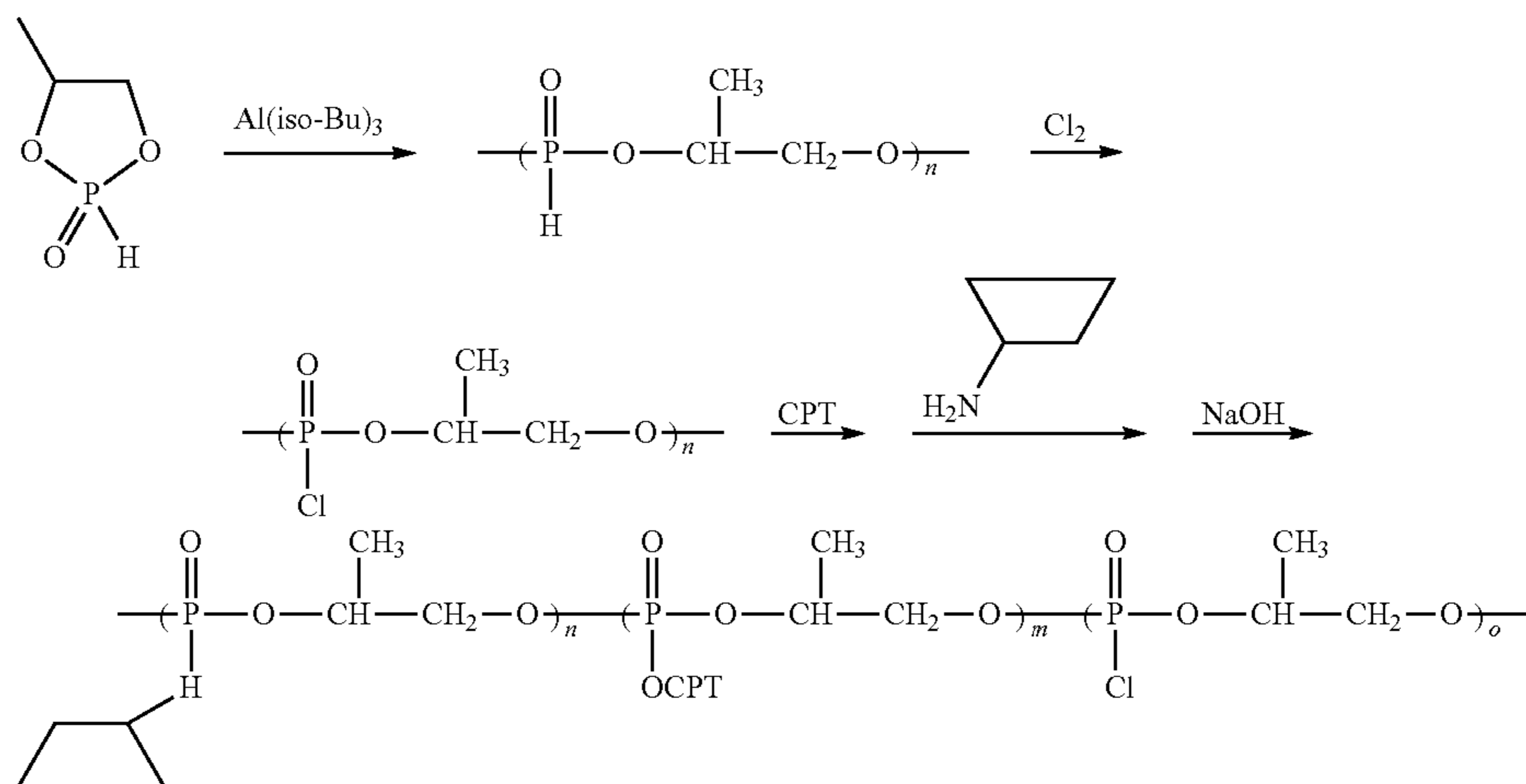
Scheme IX
