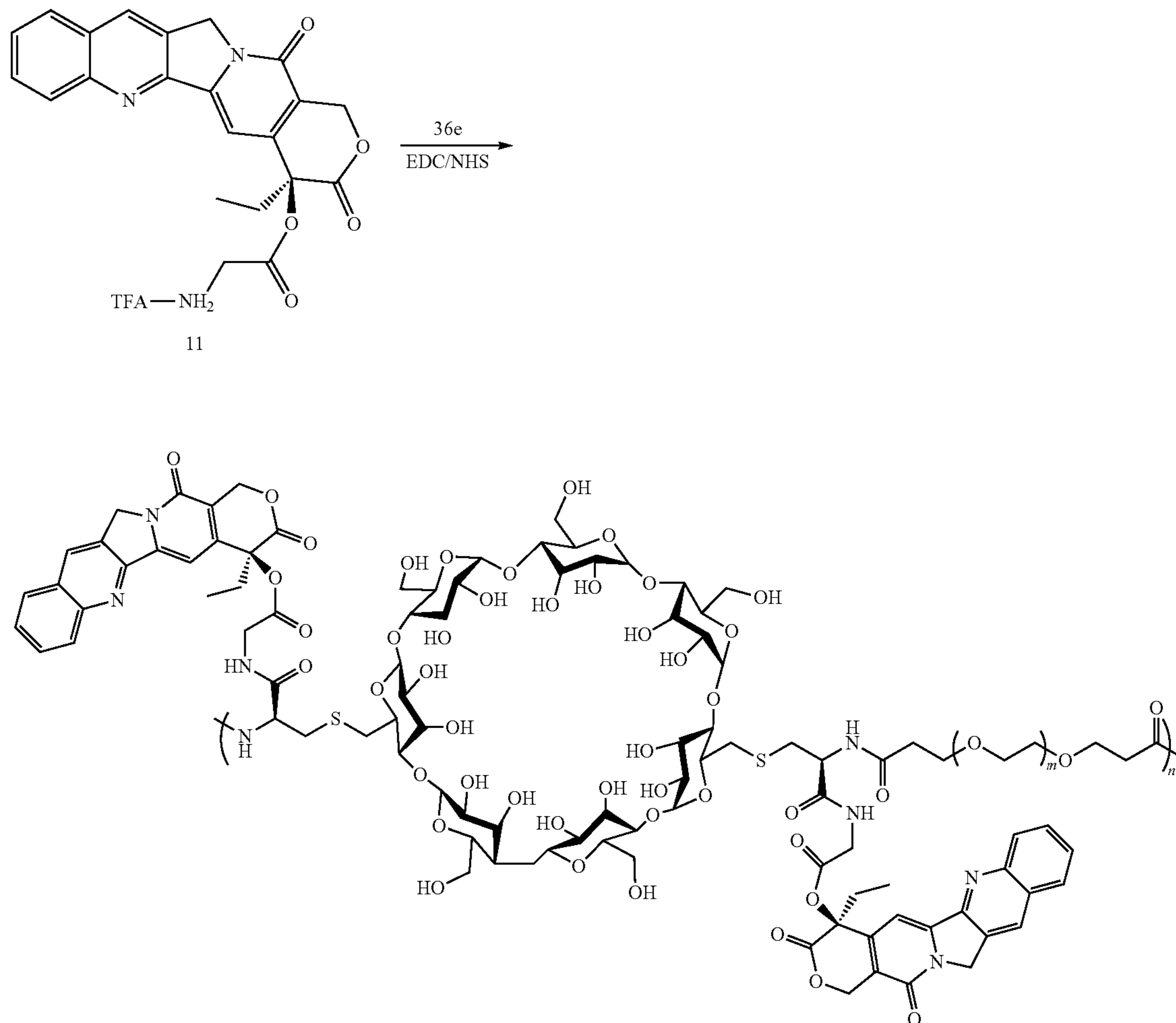
Scheme XXXIX
