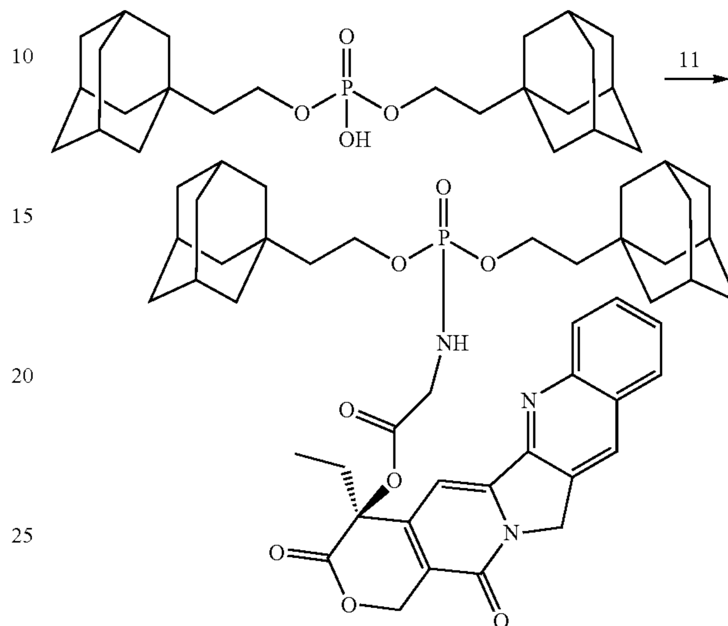
Scheme XXXXVIII
