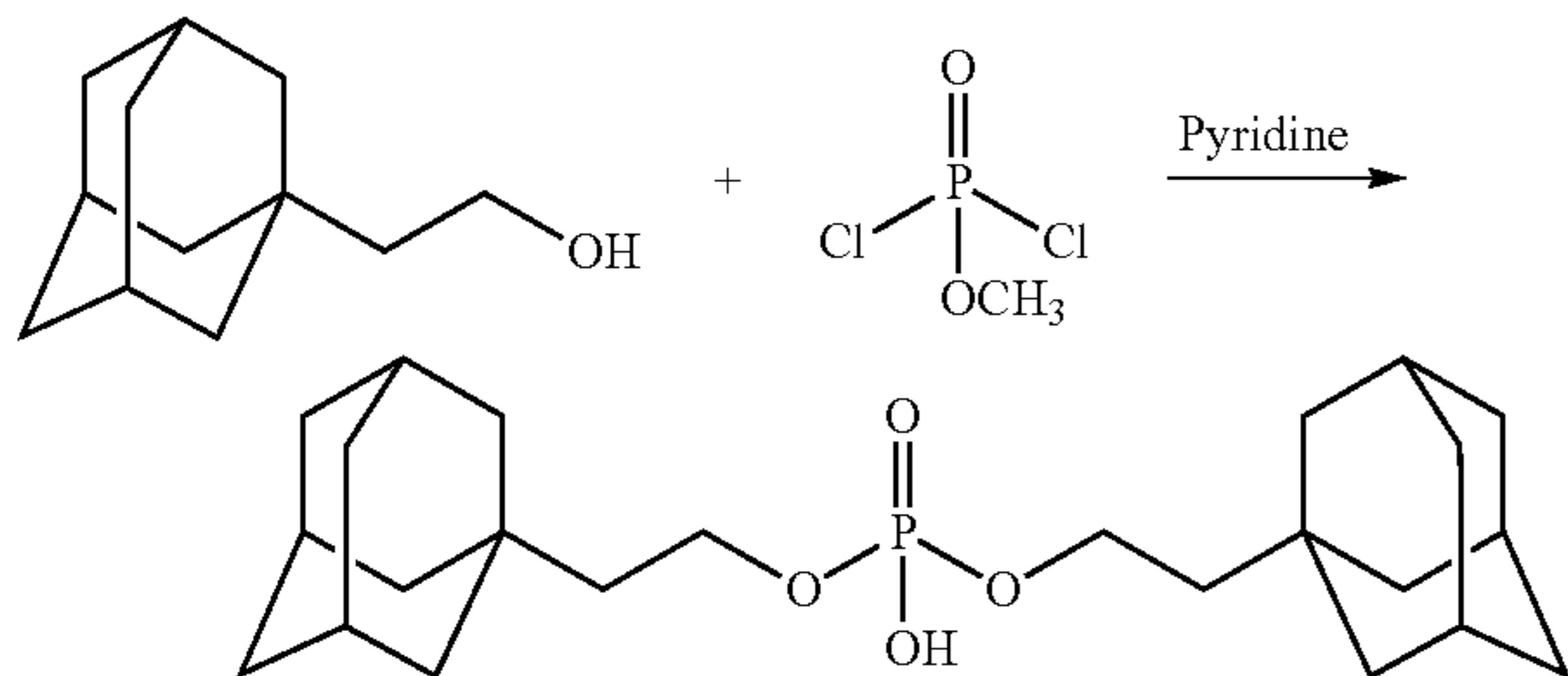
Scheme XXXXVII
