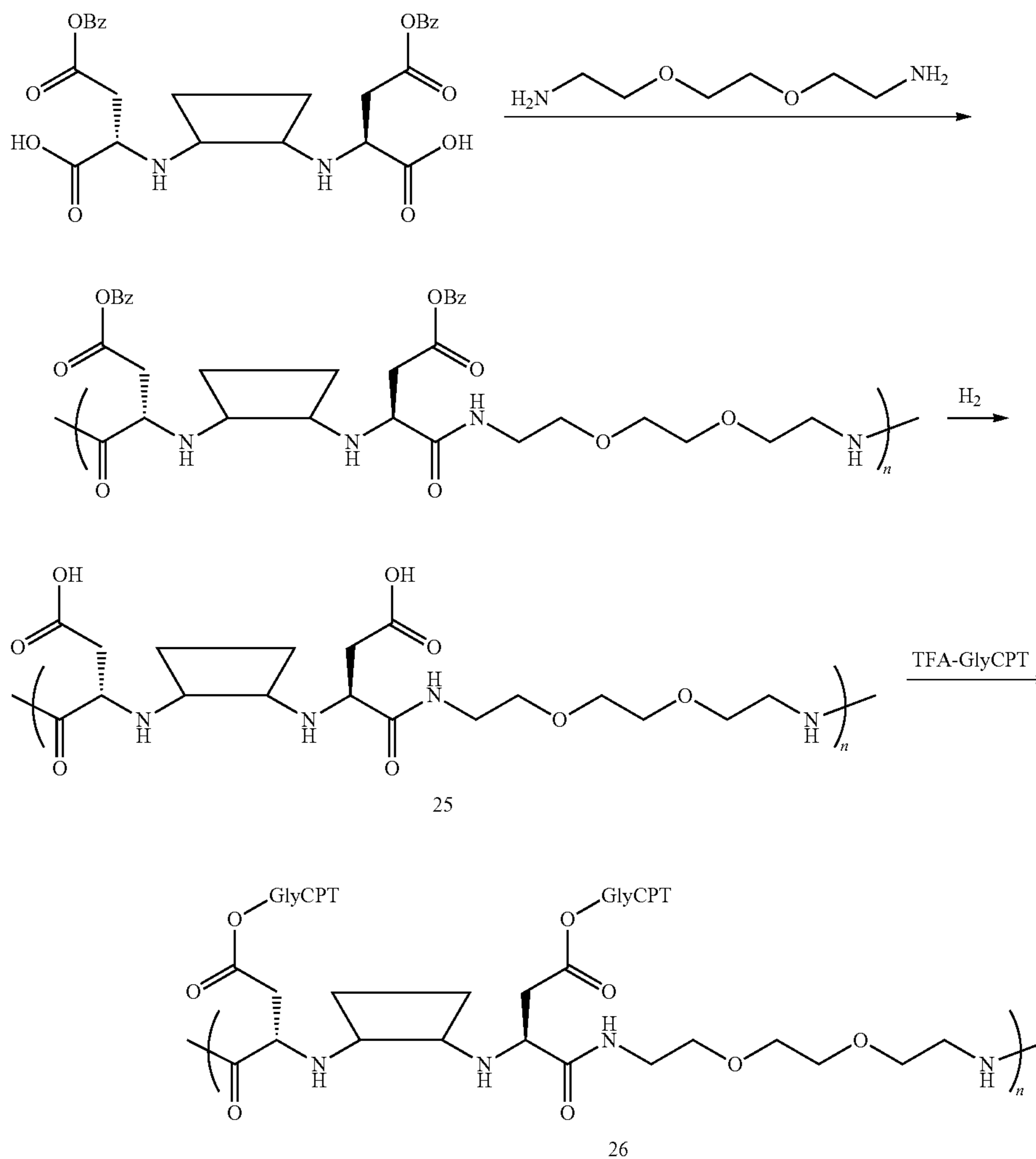
Scheme XXXI
