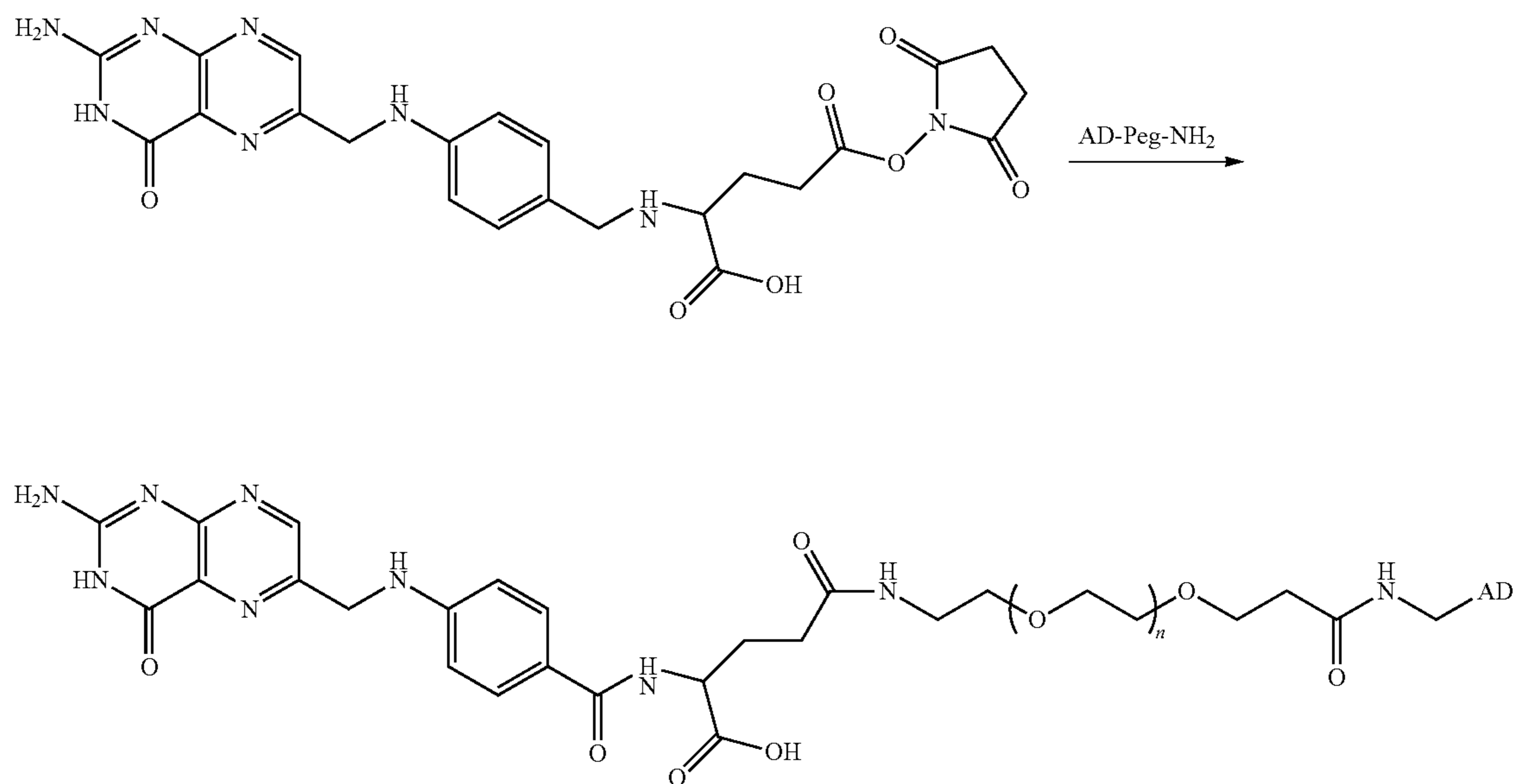
Scheme L
