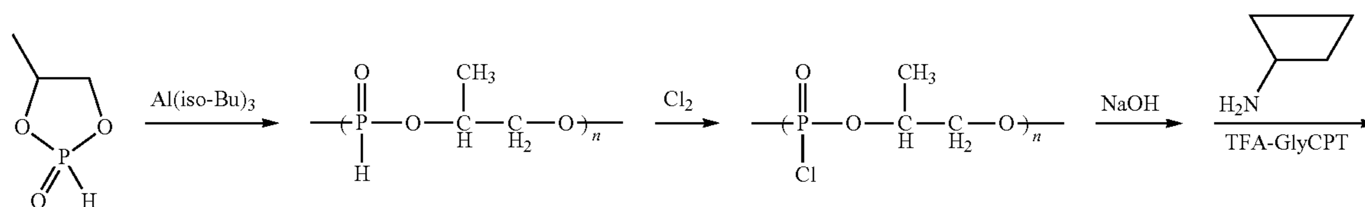
Scheme XXXIV
