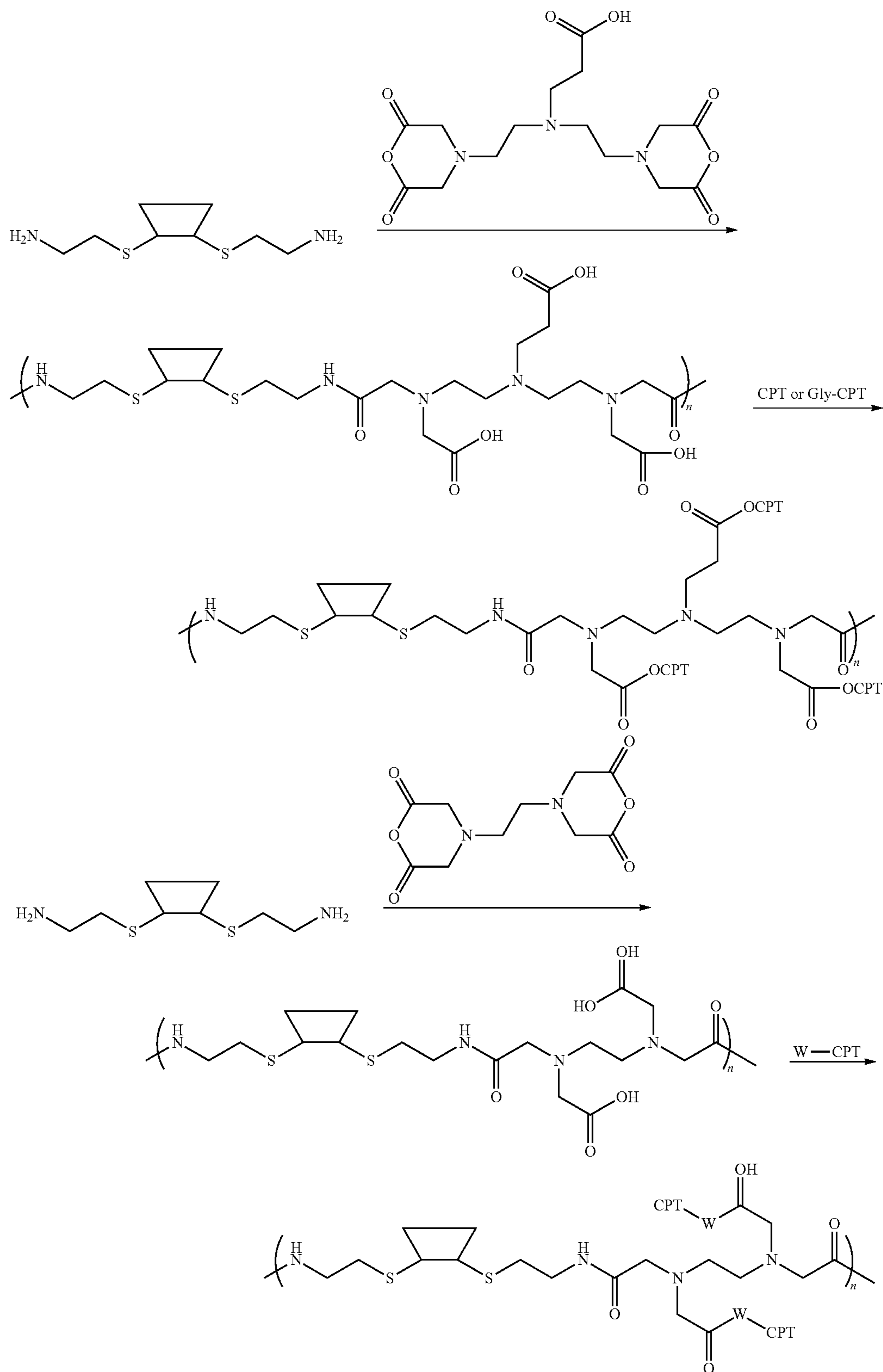
Scheme V
