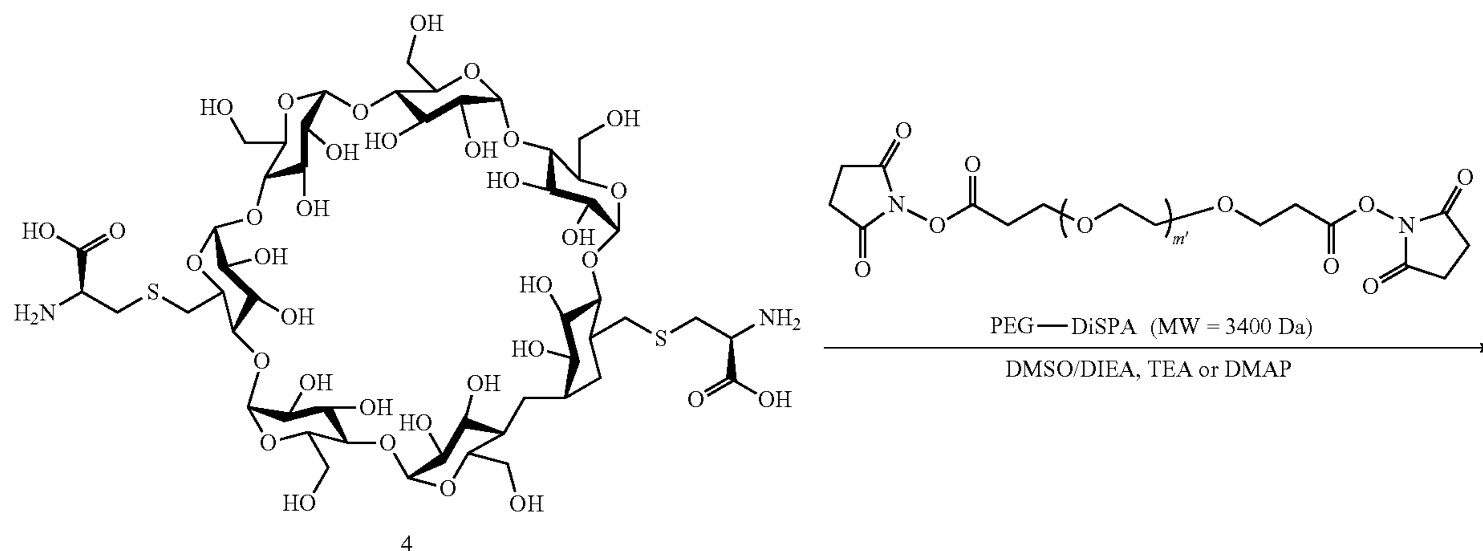
Scheme XXXVIIIa
