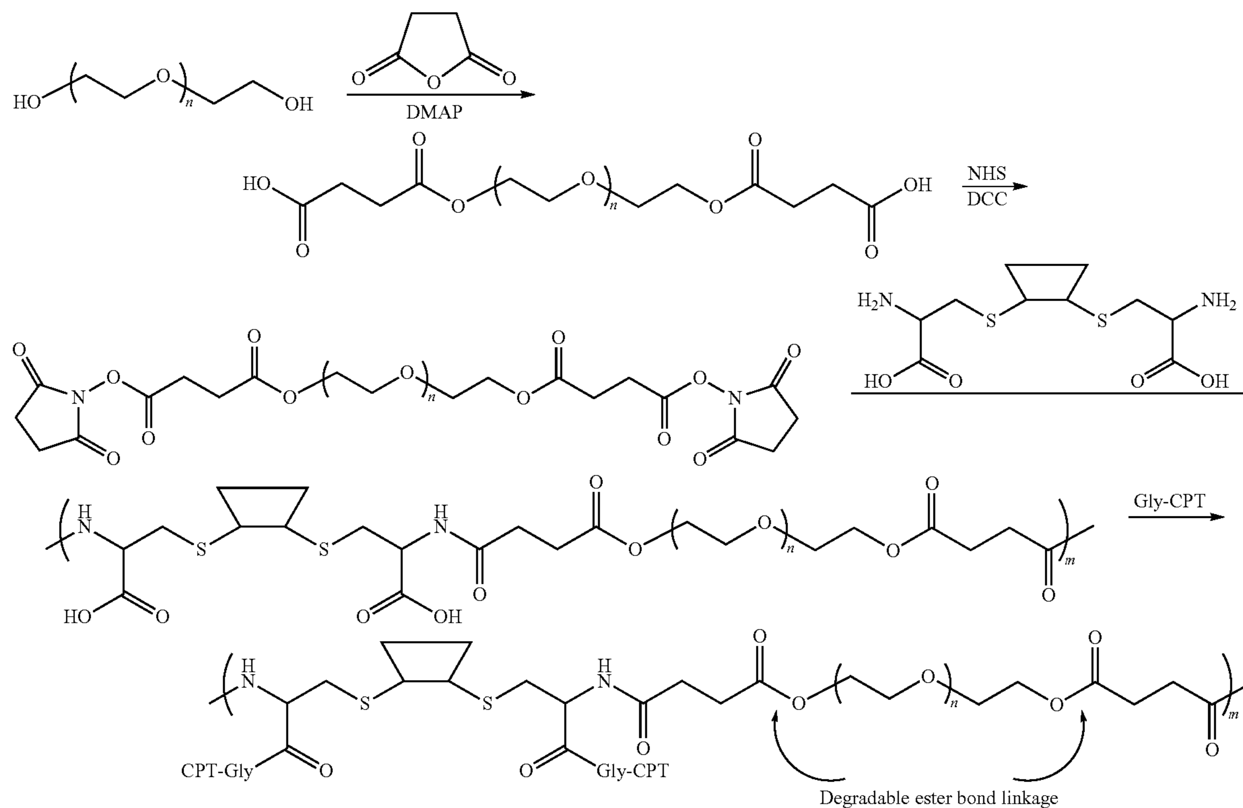
Scheme XIV
