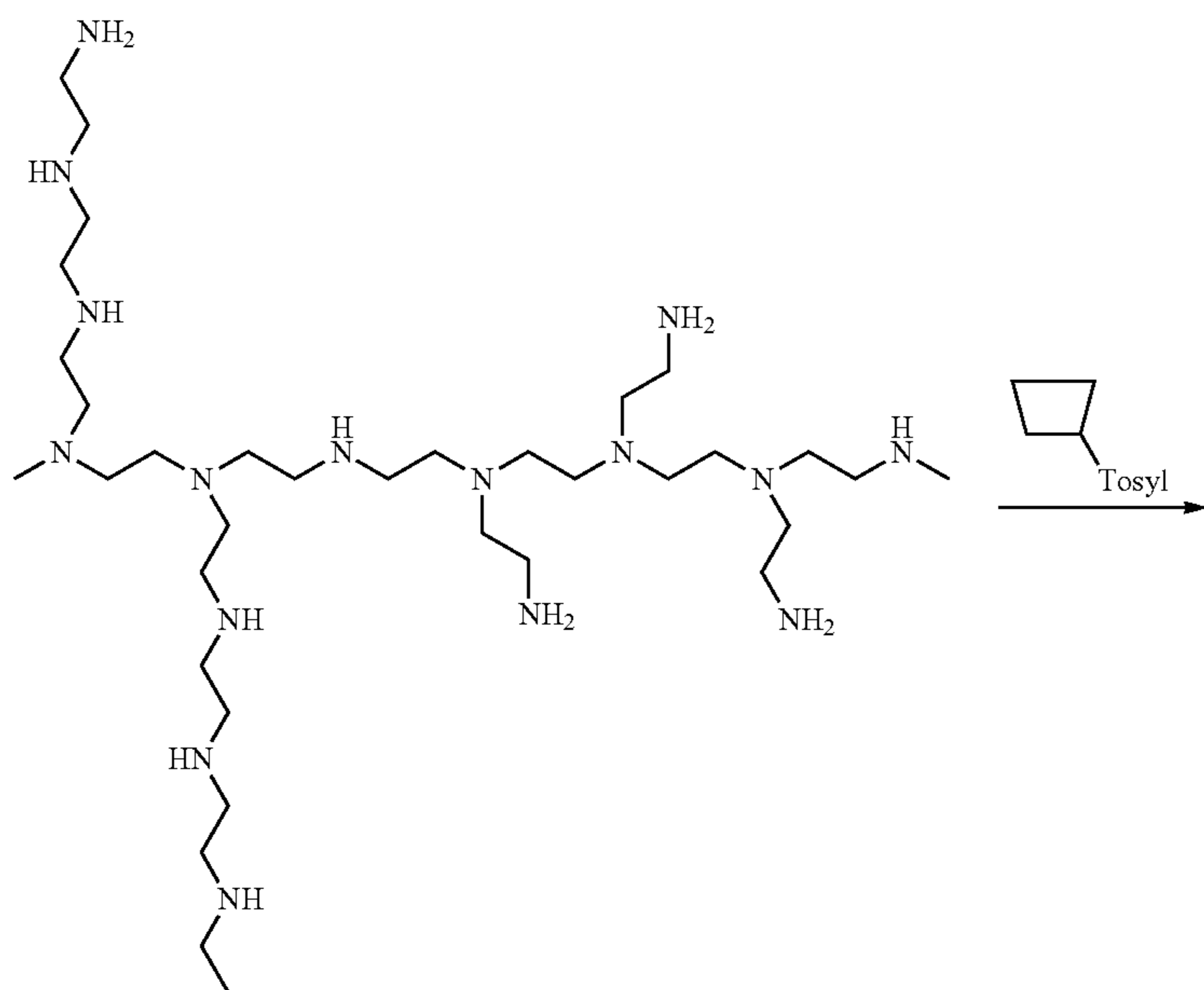
Scheme XXXXIV
