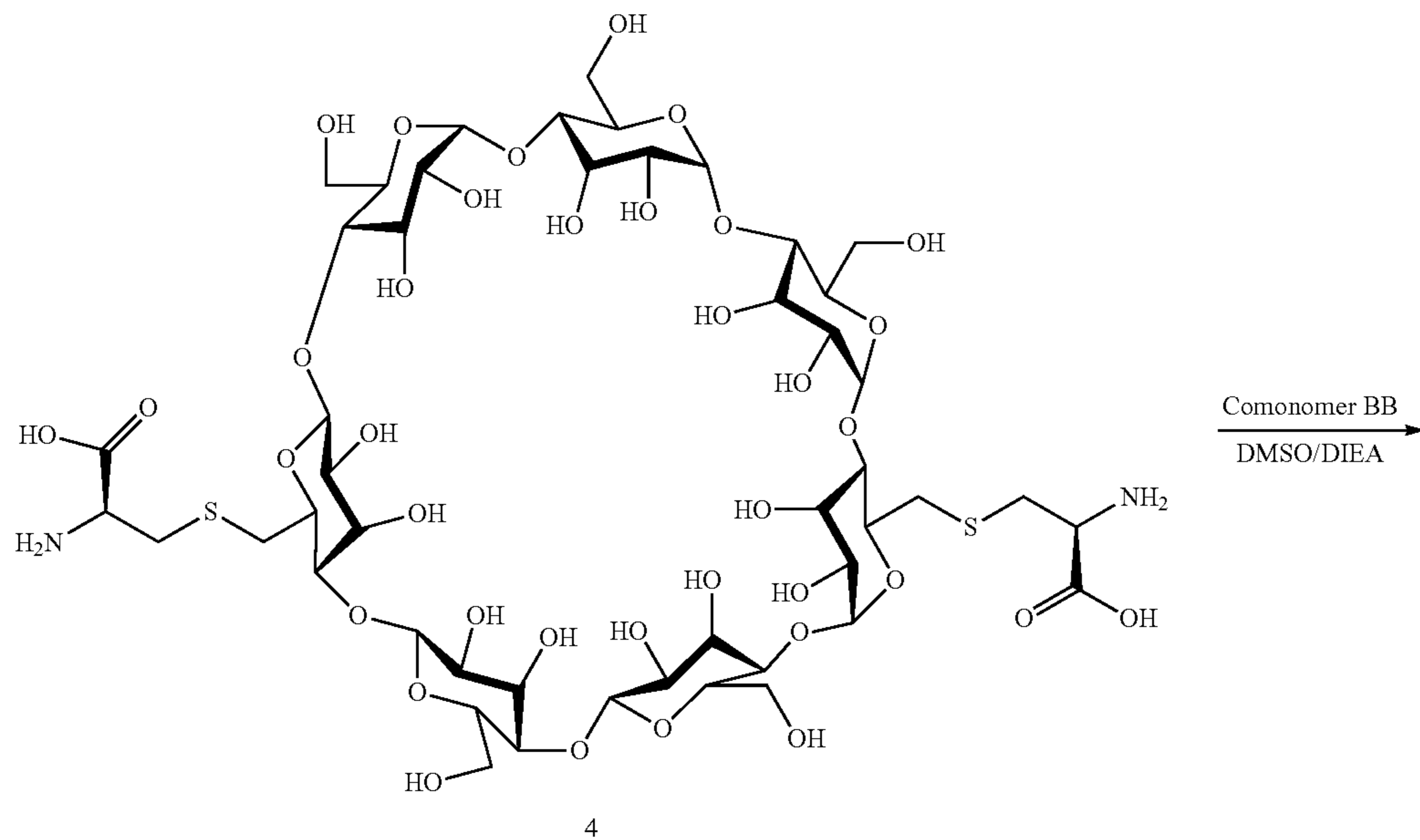
Scheme XXXVIIIb
