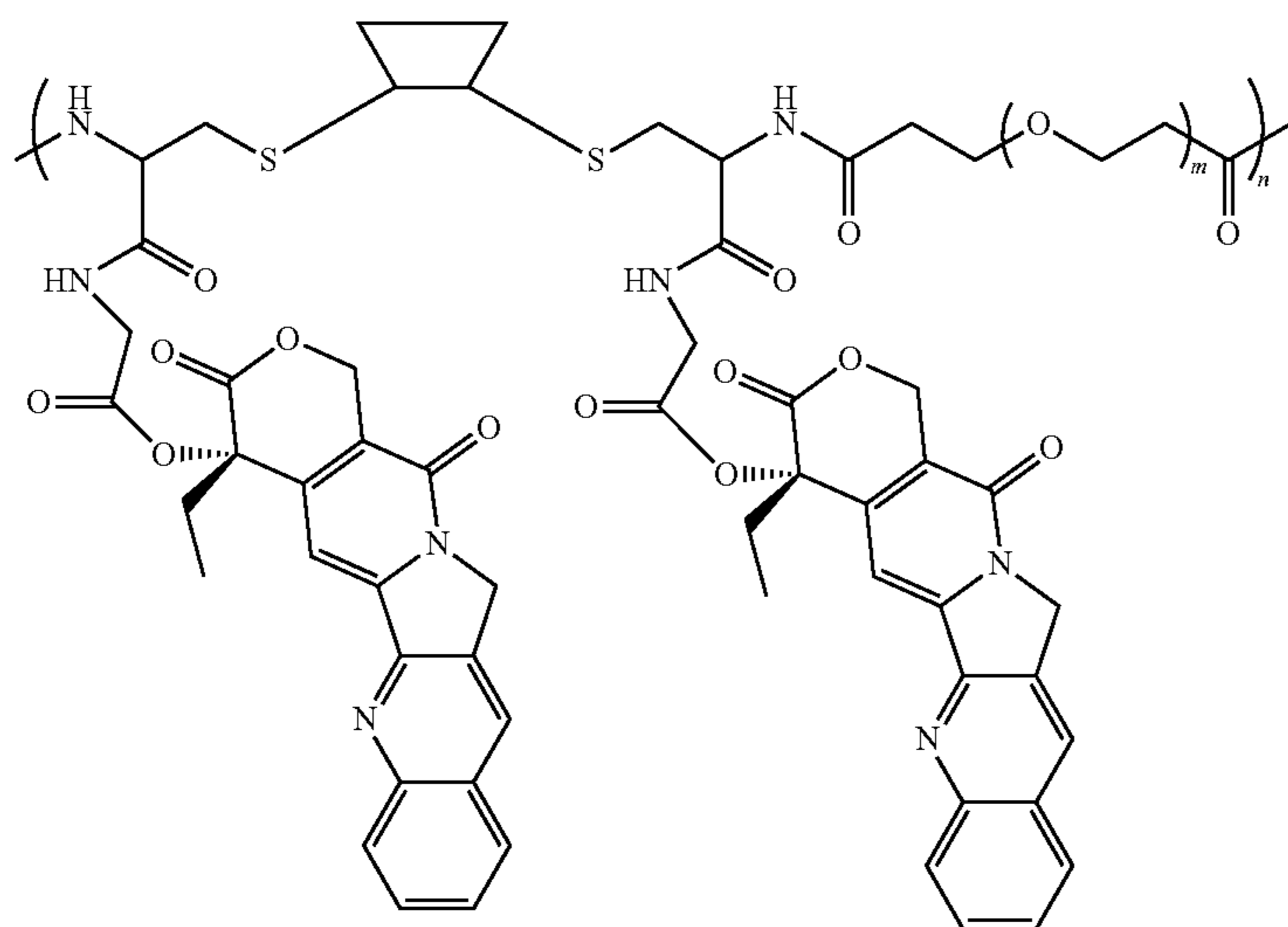
Scheme XXXXIII
