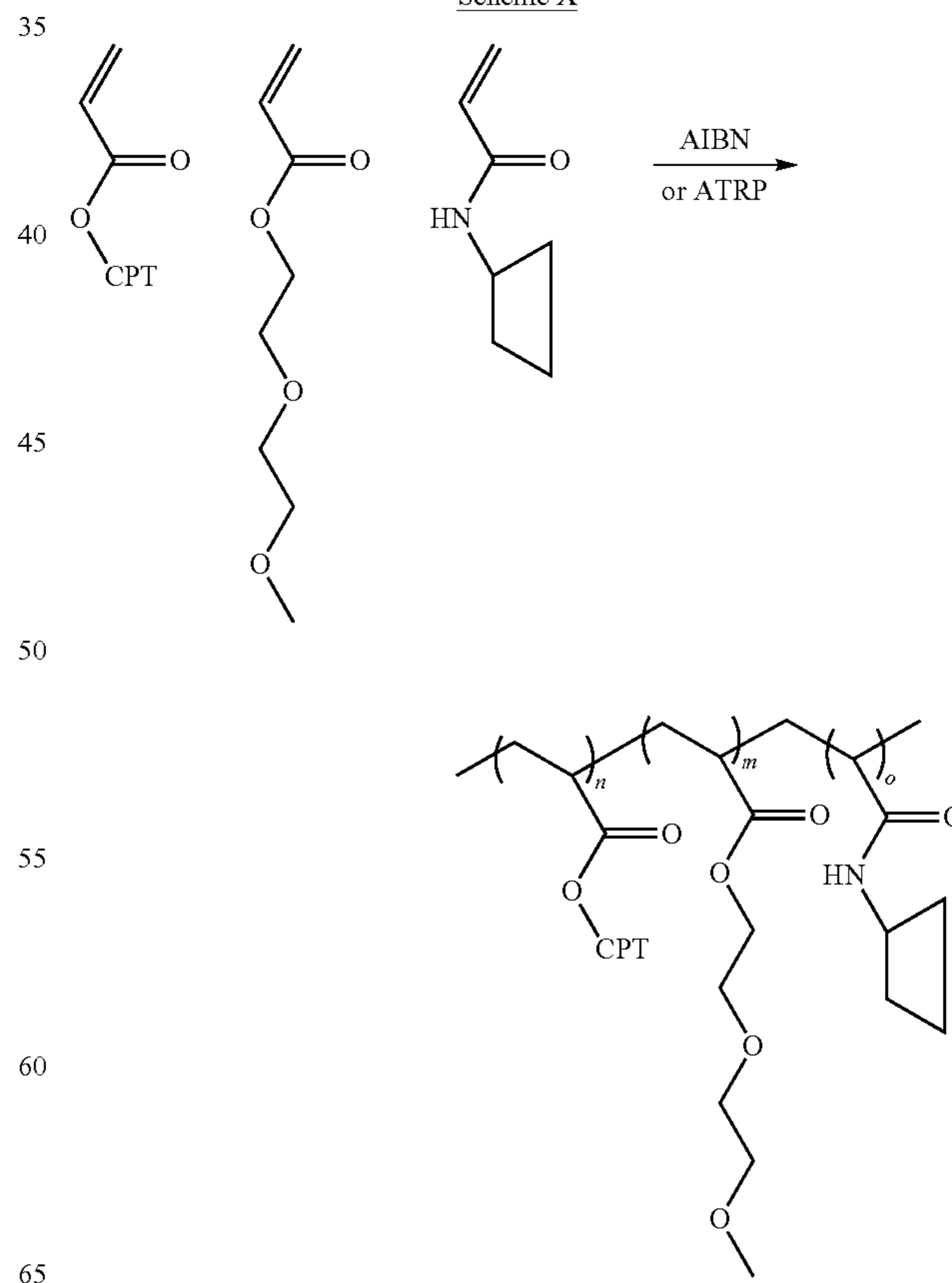
Scheme X
