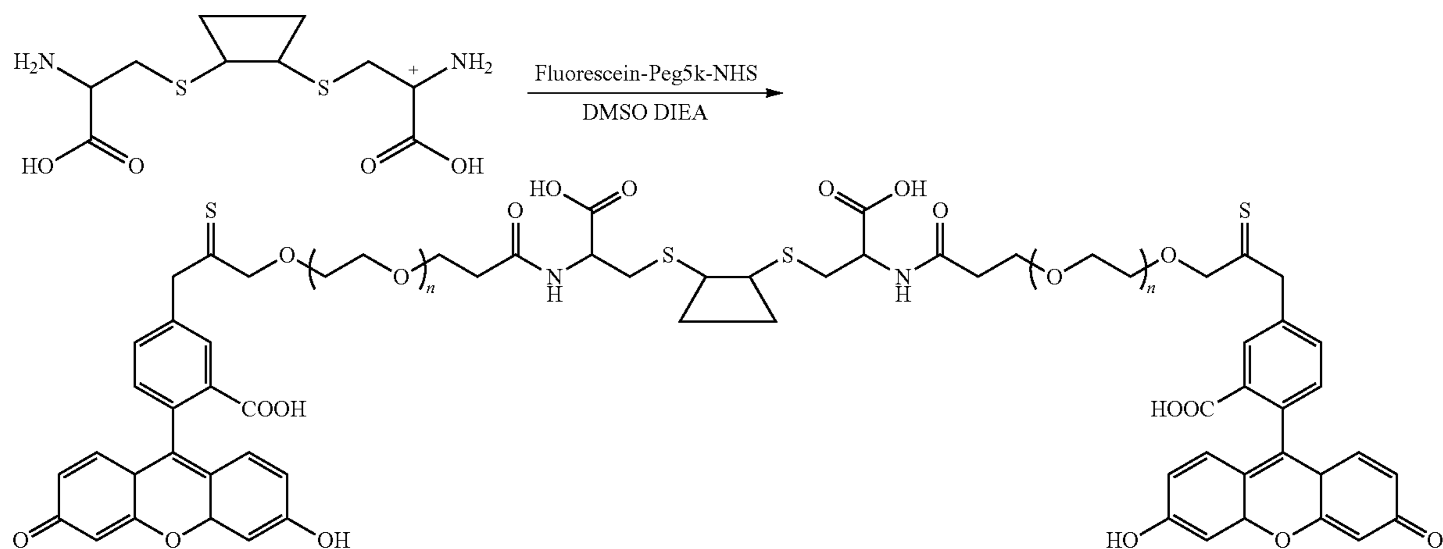
Scheme XXXX
