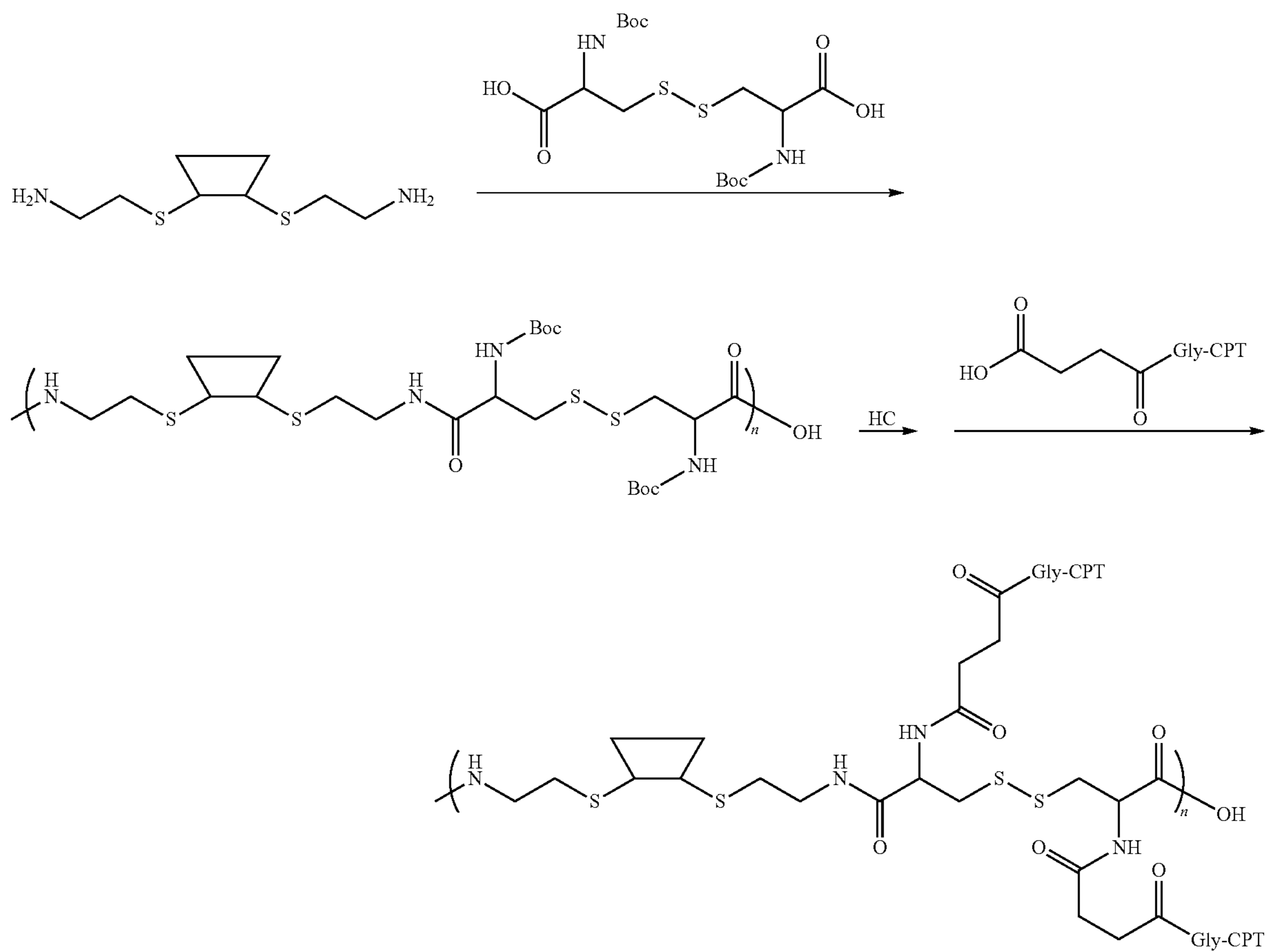
Scheme VII
