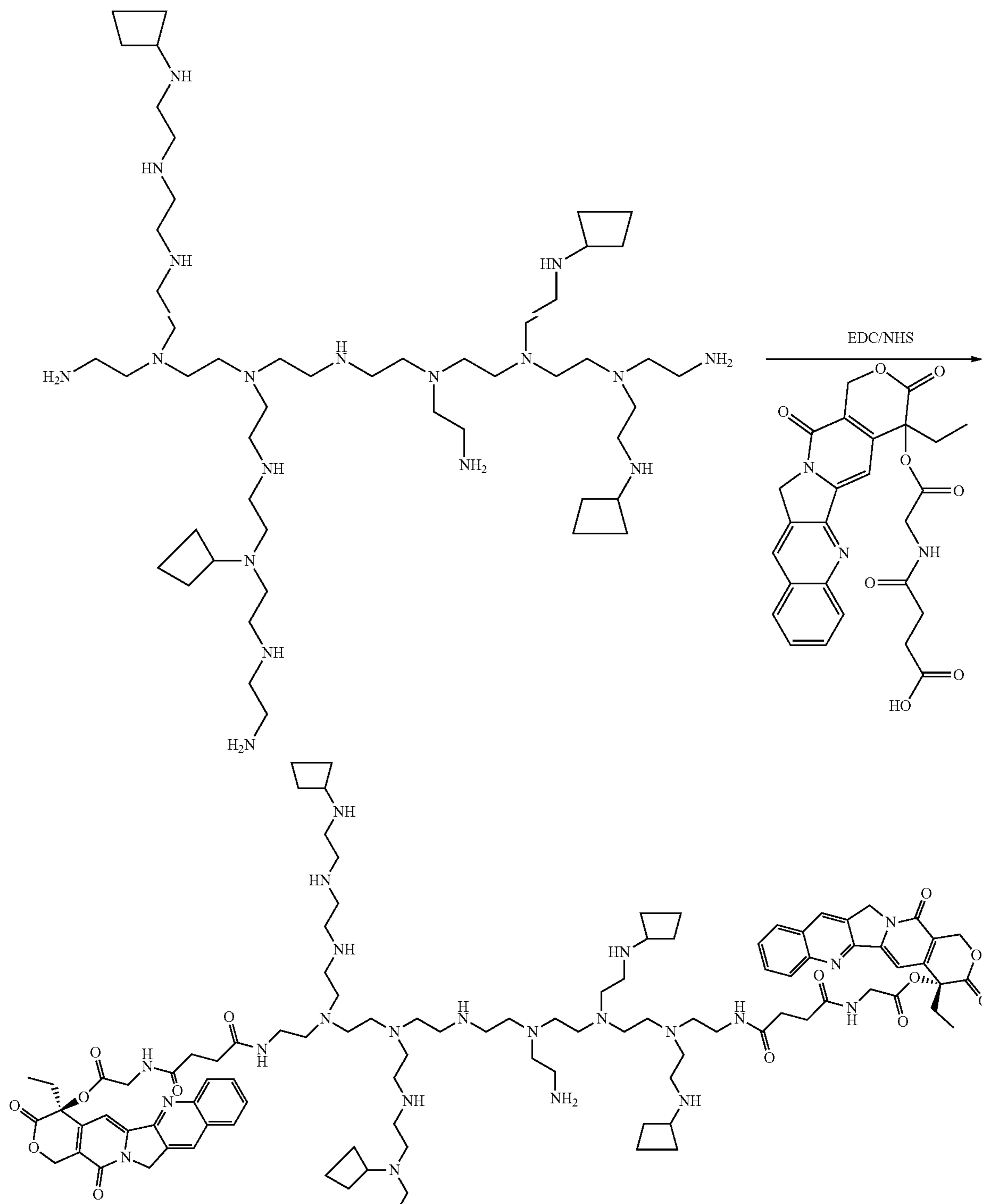
Scheme XXXXV
