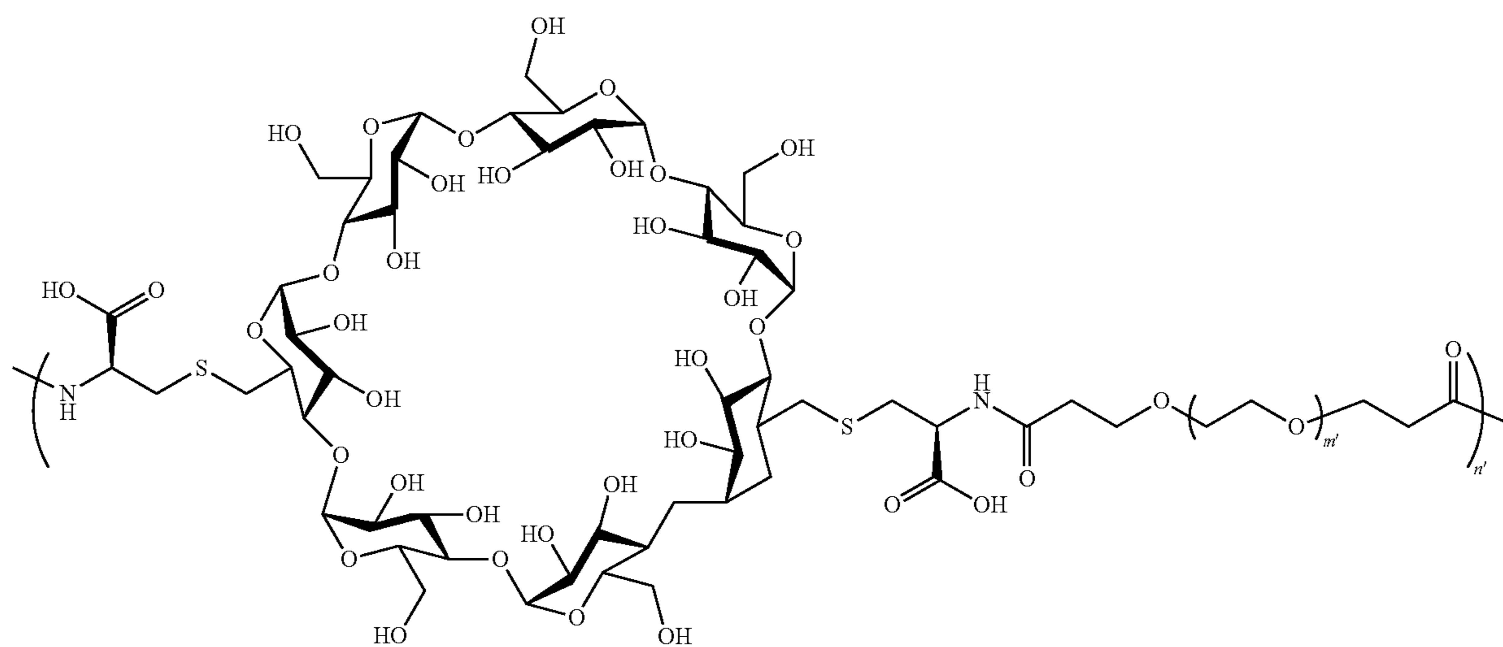
36a-f Poly(CDDCys-PA-PEG) Abbr: PA = propanoicamide bond between PEG and CD
