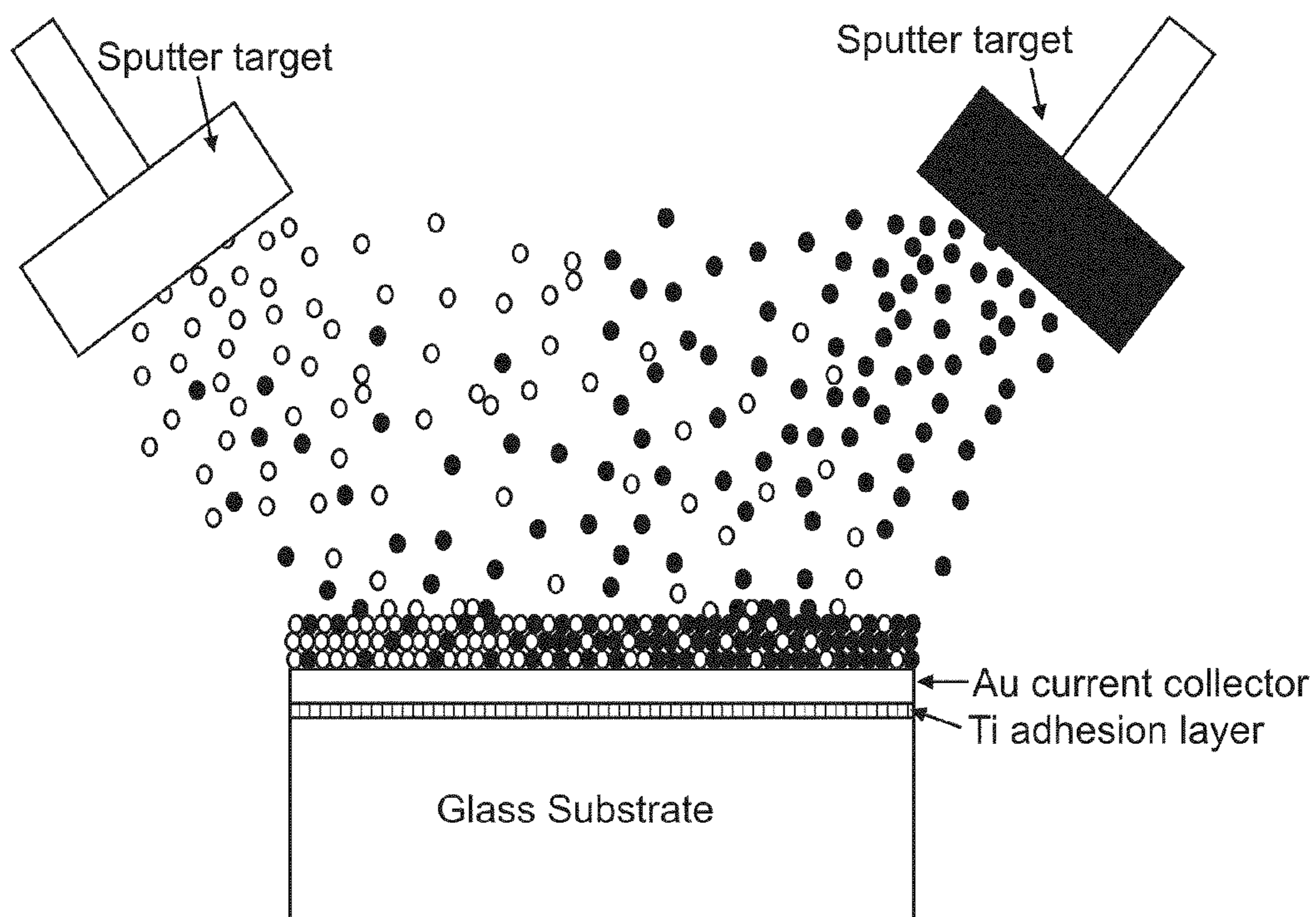
Figure 2a: Co-sputtering
