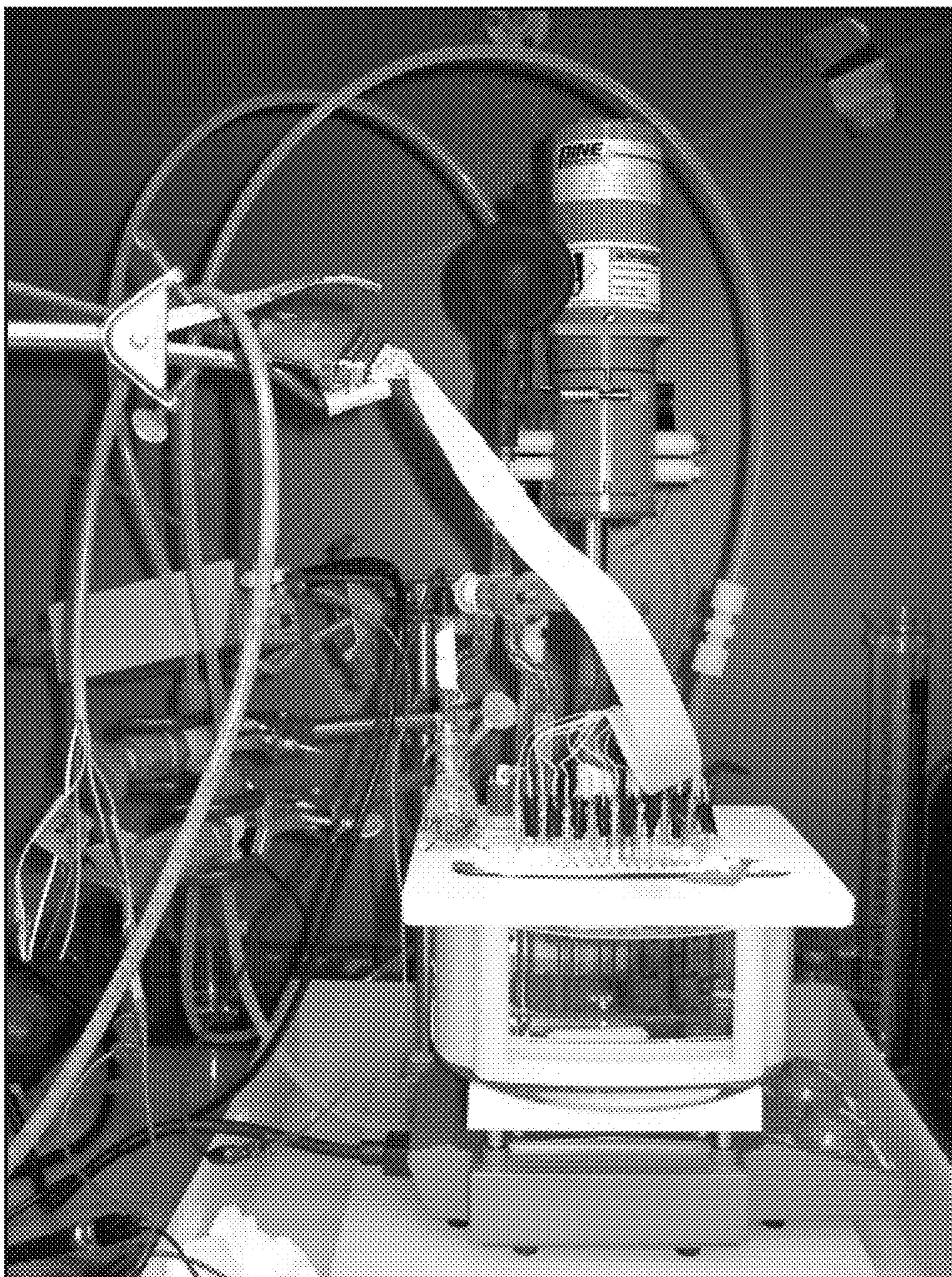
Figure 5a: Custom-built multi-electrode half cell
