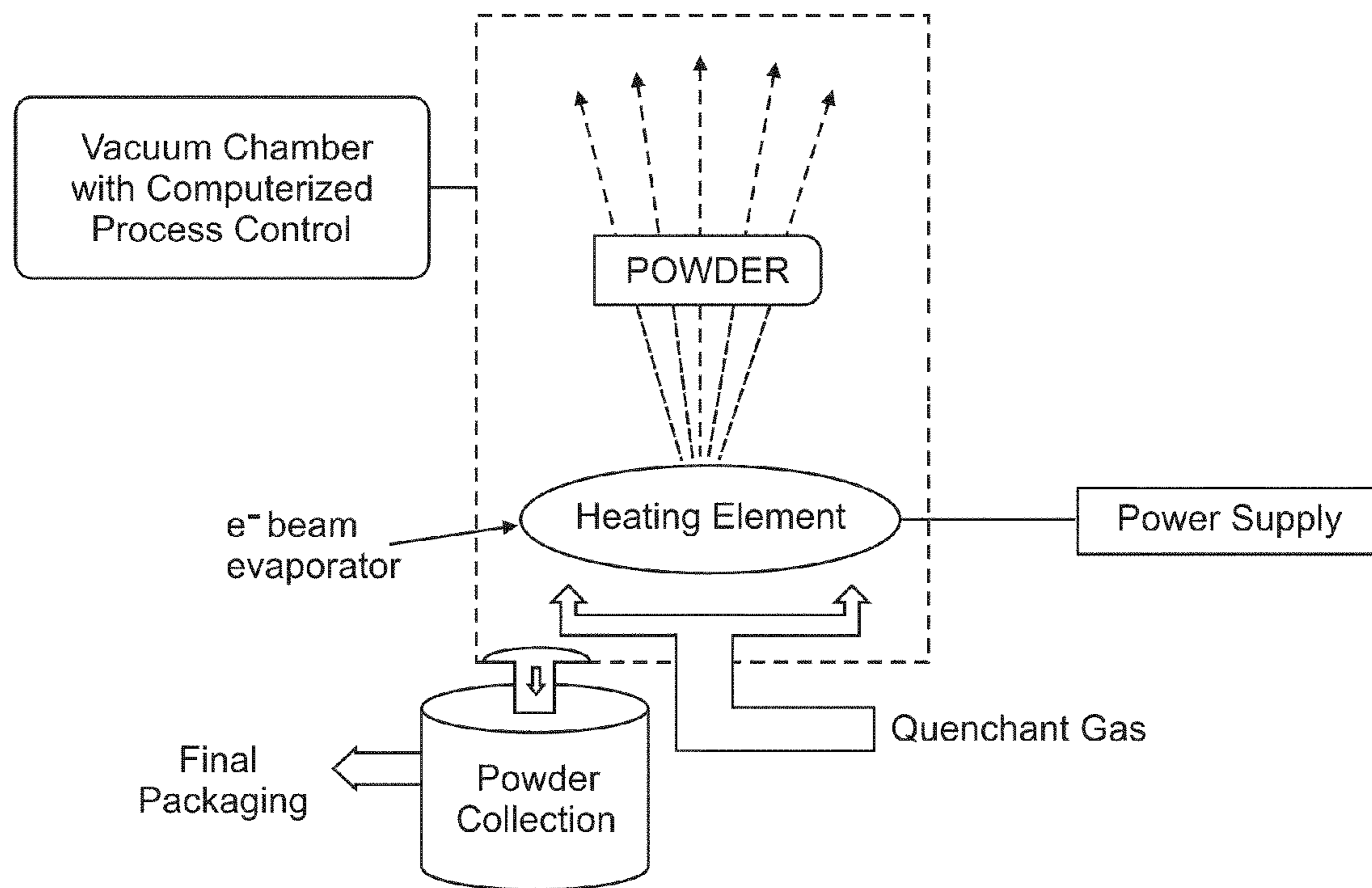
Figure 2c: Vapor-phase condensation
