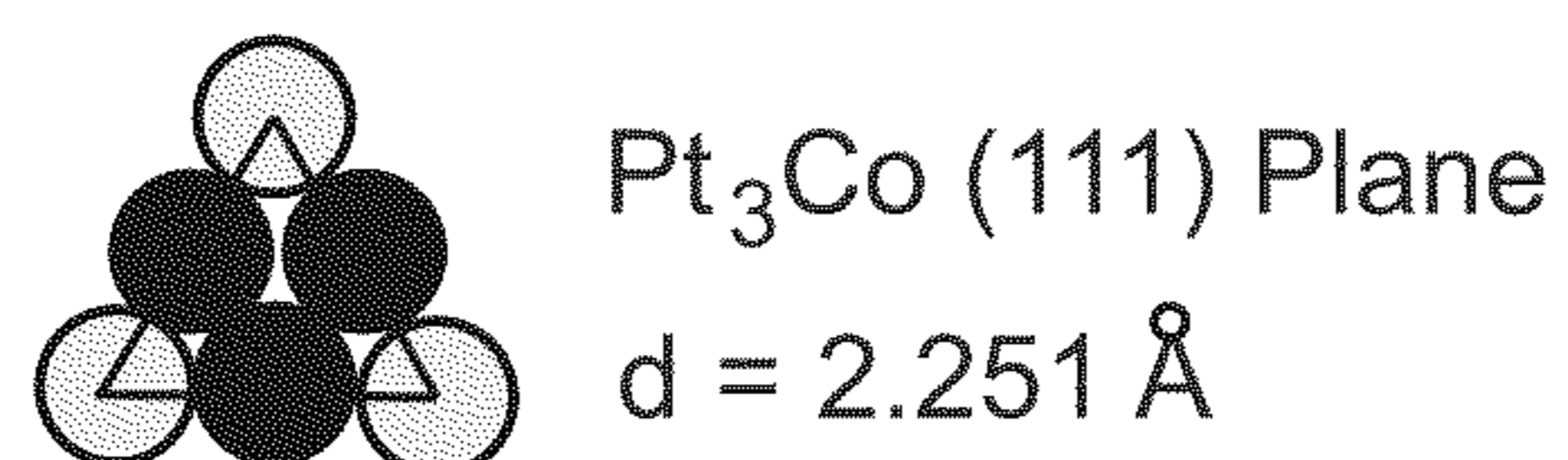
Ordered Pt 3 Co (Cu 3 Au-type)
