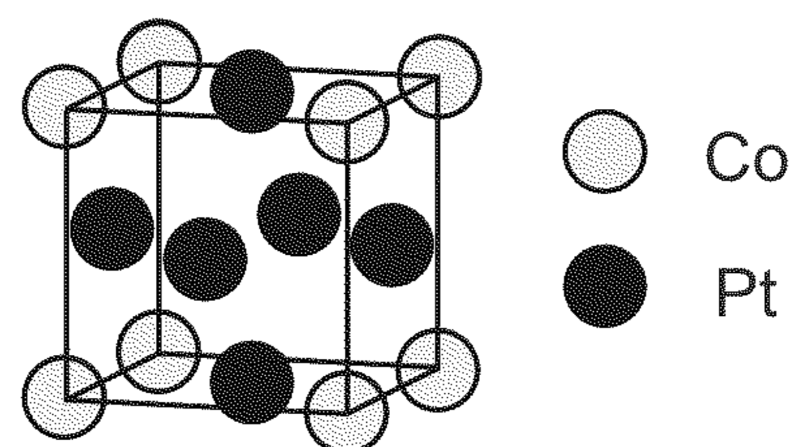
Ordered Pt 3 Co (Cu 3 Au-type)
