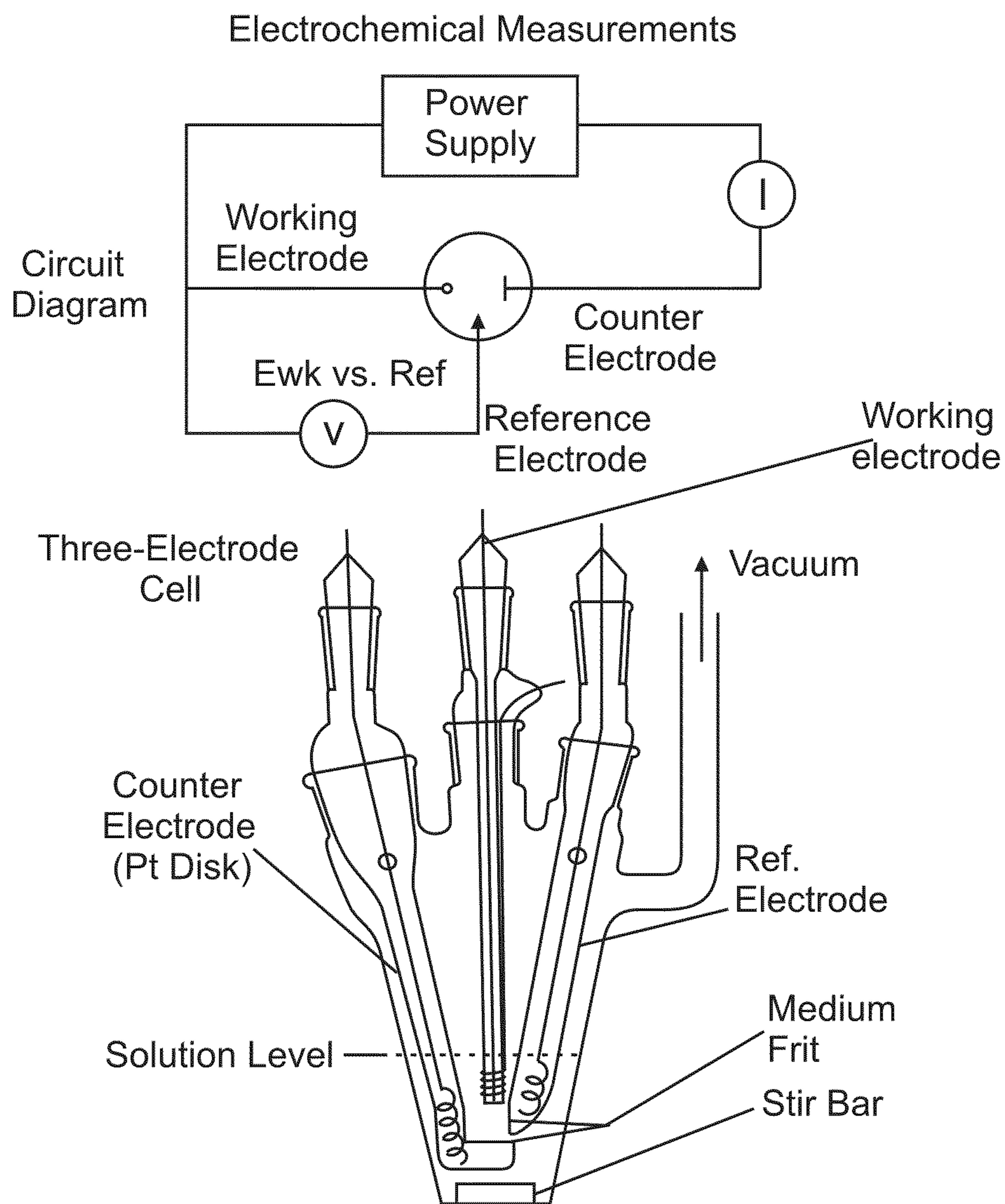
Figure 5b: Schematic of typical half cell
