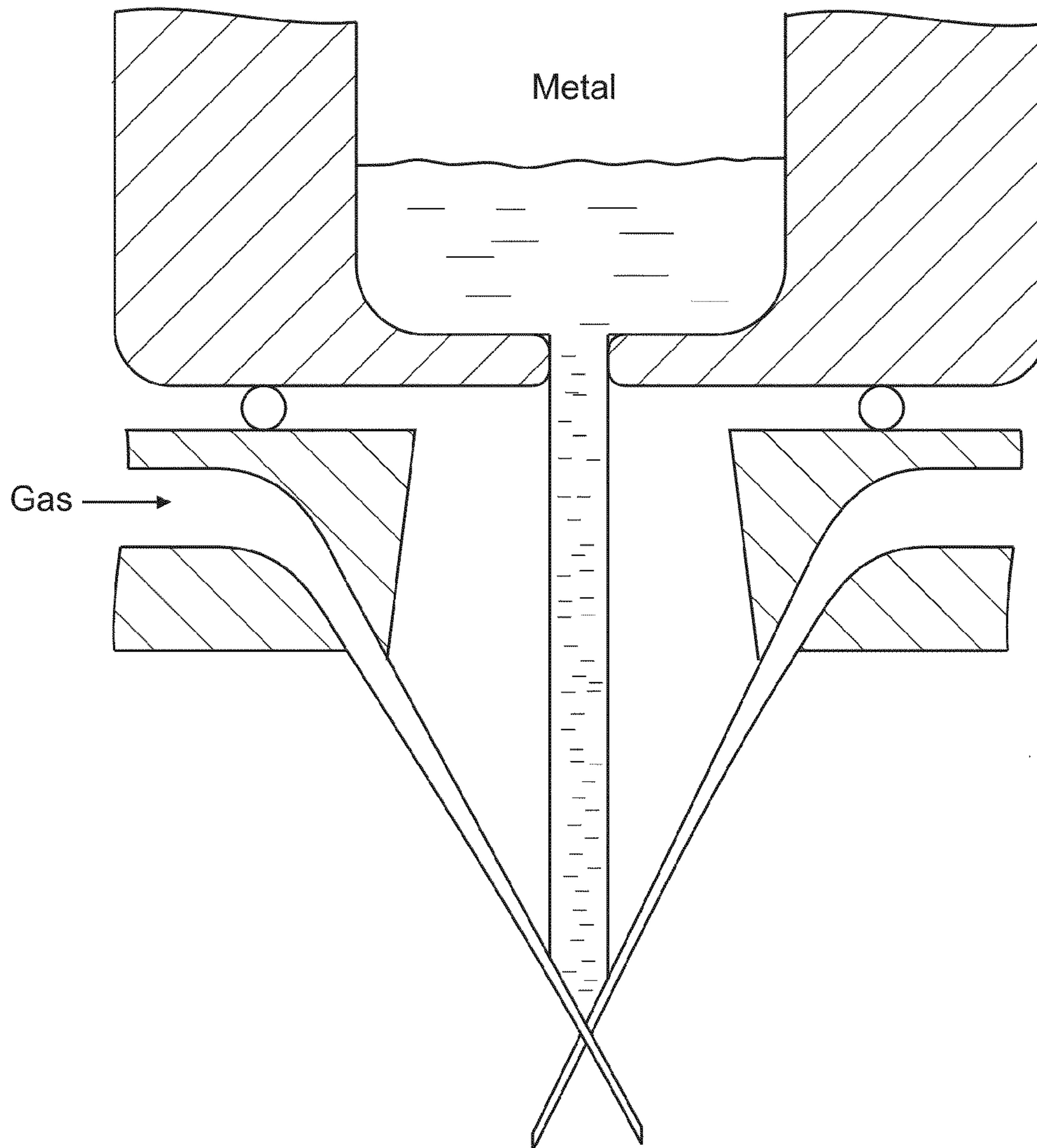
Figure 2f: Gas Atomization
