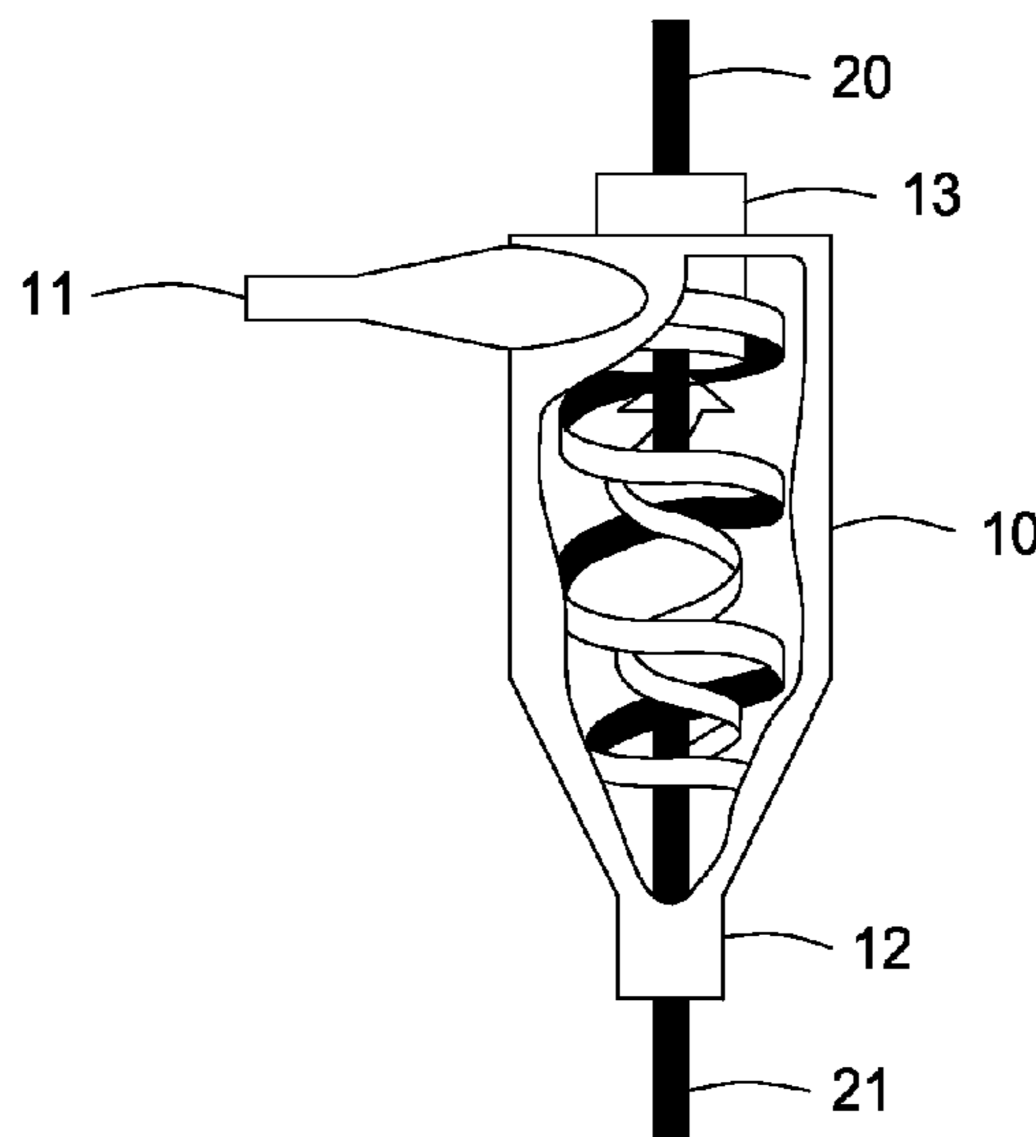
Carbon Arc in Cyclone separator
