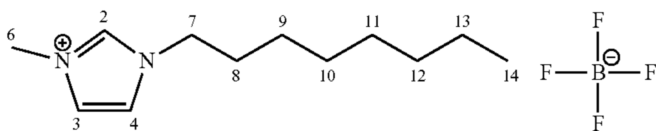
1-Octyl-3-methylimidazolium tetrafluoroborate
