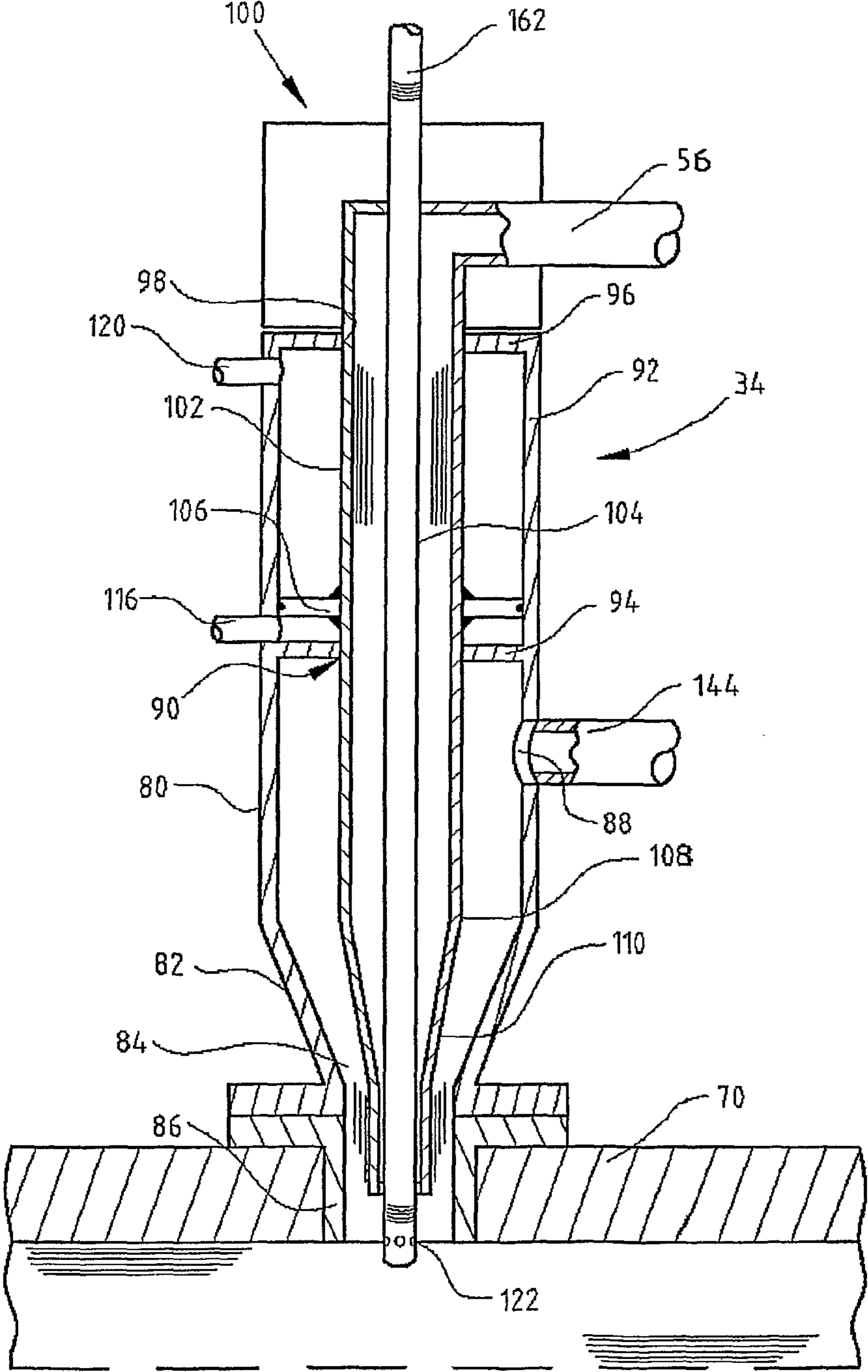
Fig. 2 (PRIOR ART)
