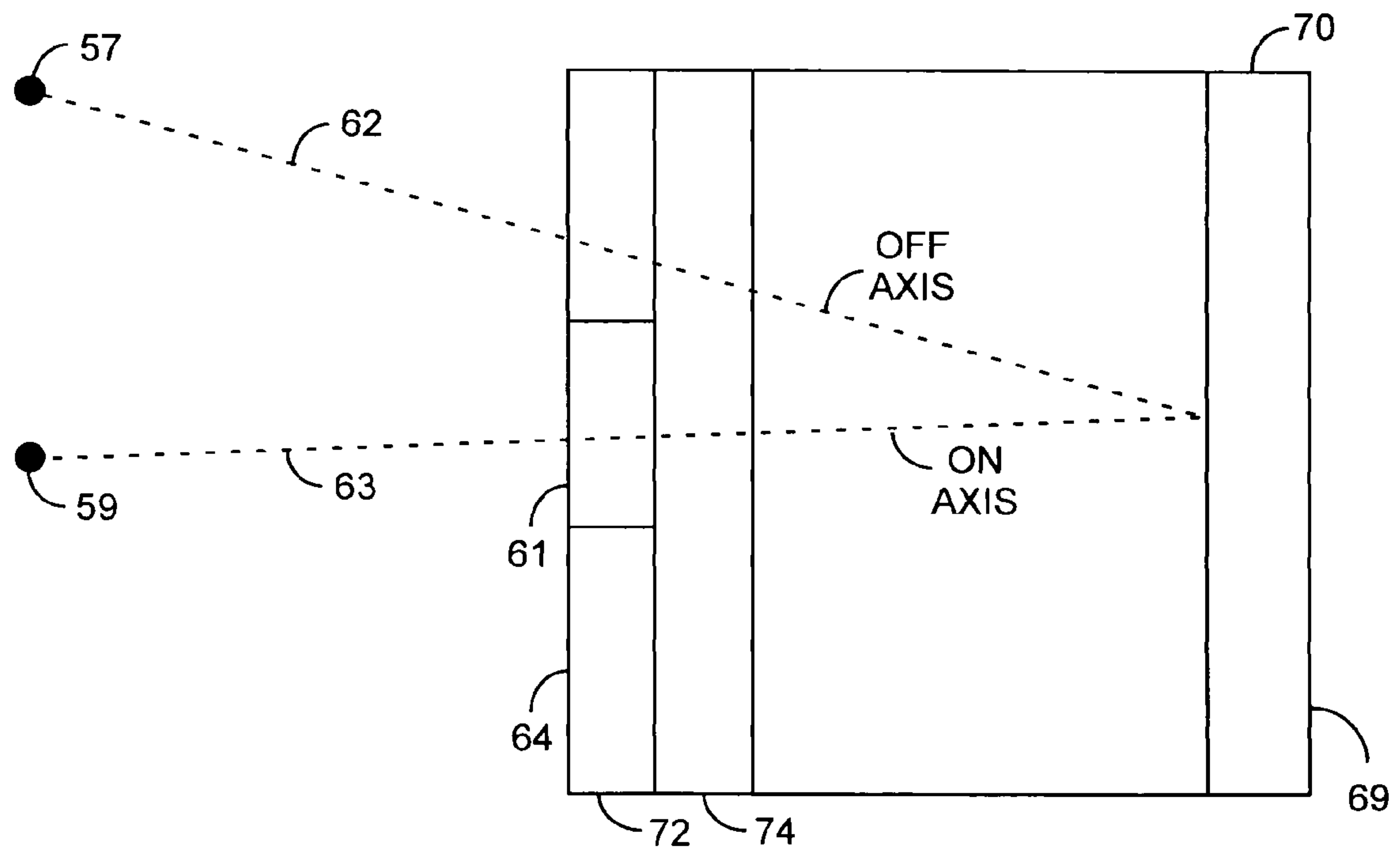
REDUCED GLARE CAMERA FIG. 8
