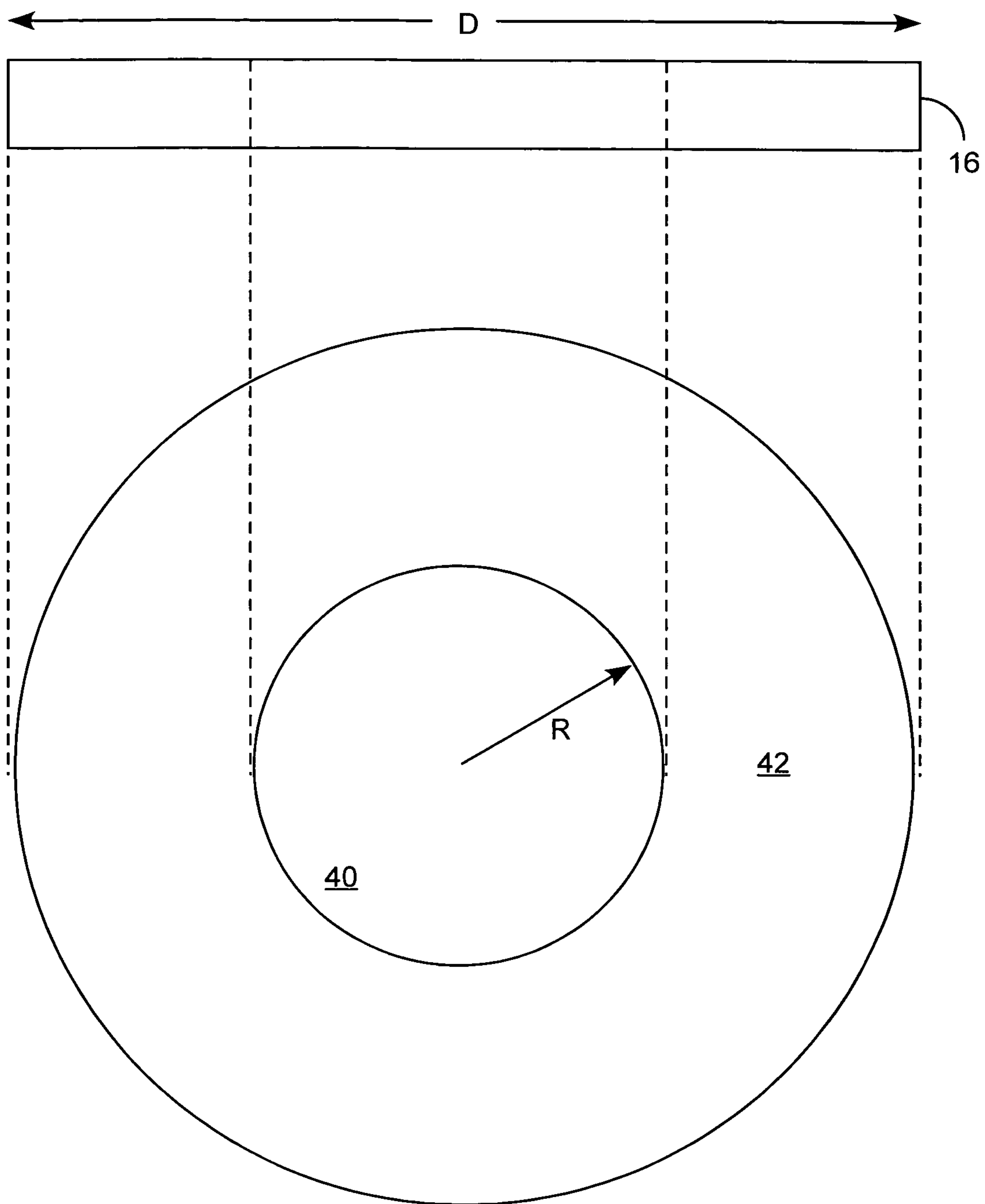
ANNULAR ABSORPTION FILTER
