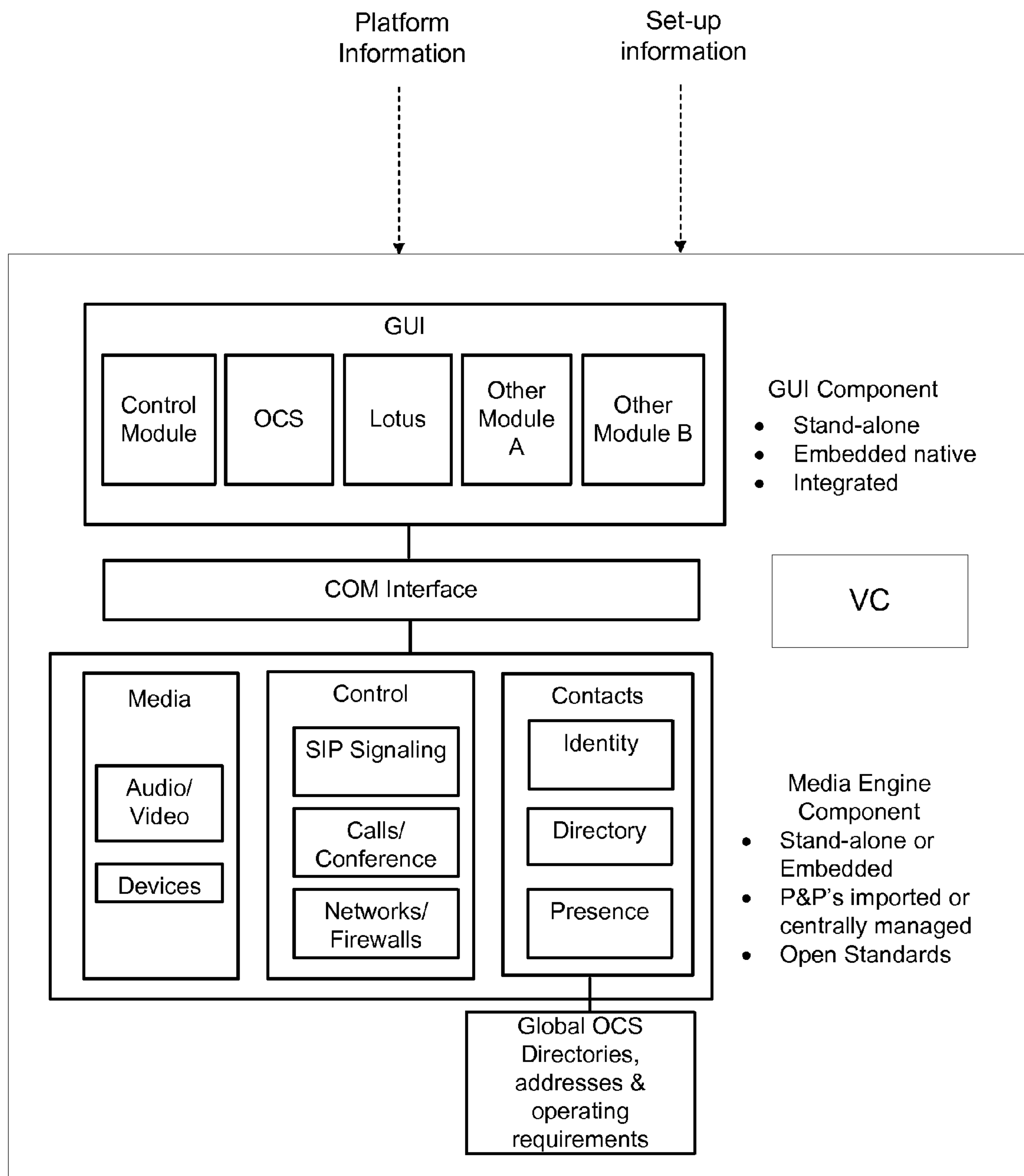
Figure 41c (configured by both platform and set-up information)
