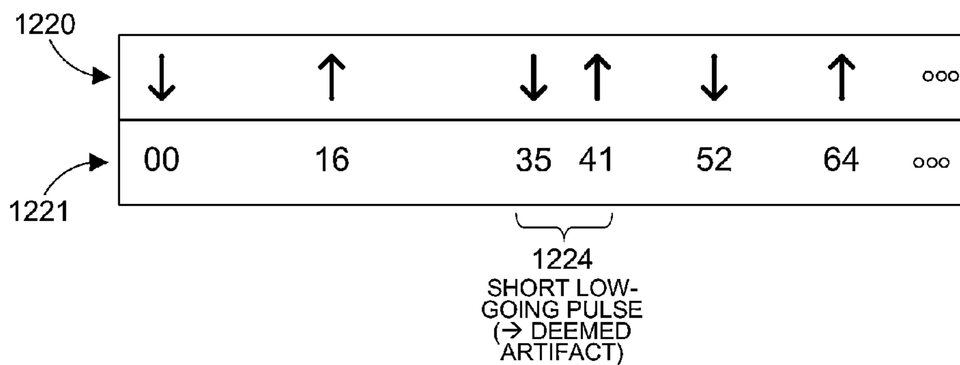
DIGITIZED DETECTED ENVELOPE SIGNAL - TRANSITIONS CONVERTED TO TIMES
