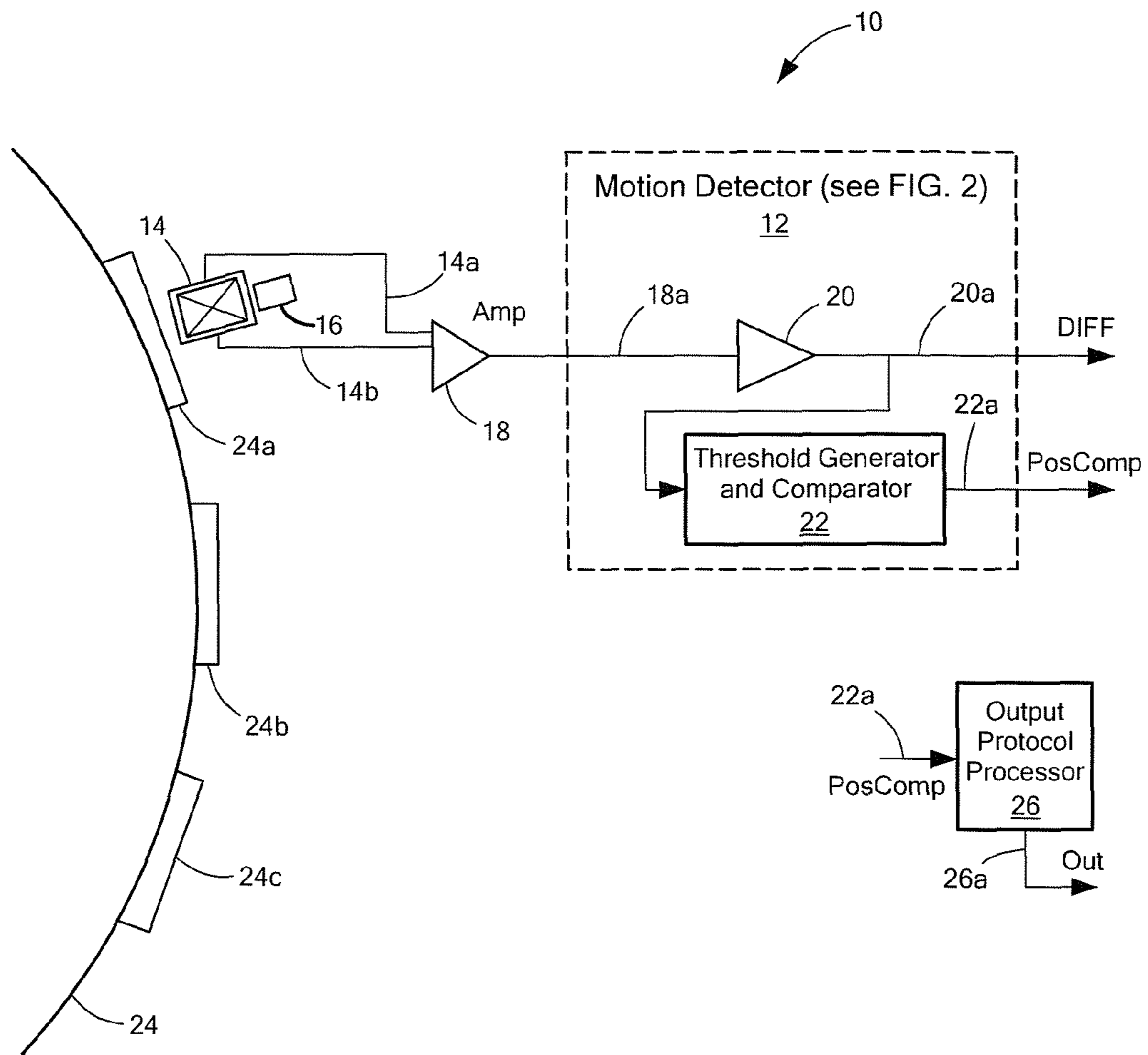
FIG. 1 (prior art)
