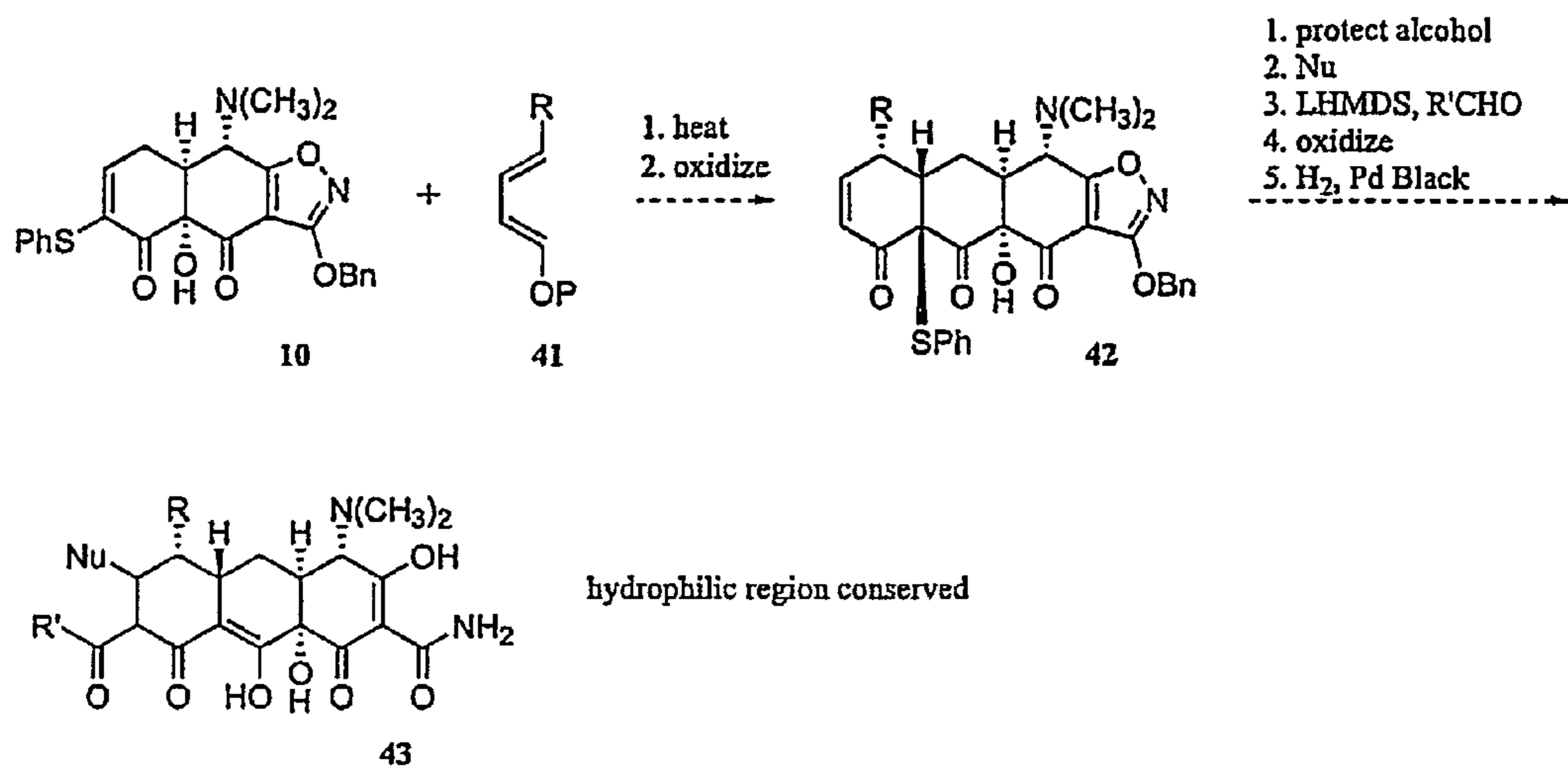
Figure 7 Summary of Targeted "Tricyclines"
