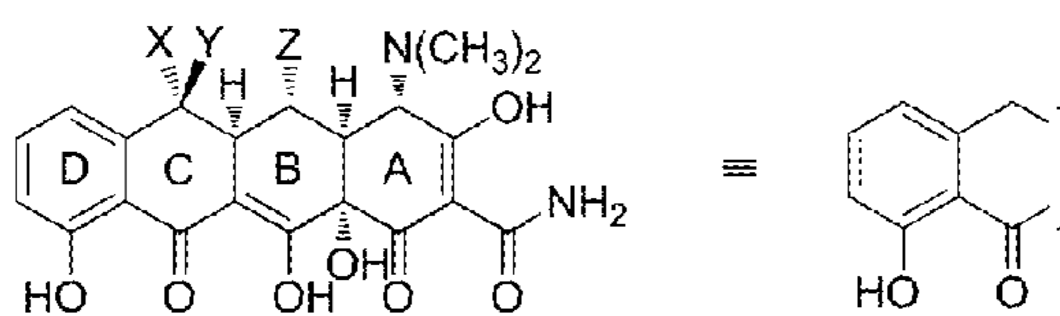
Figure 14B Representative Structures
