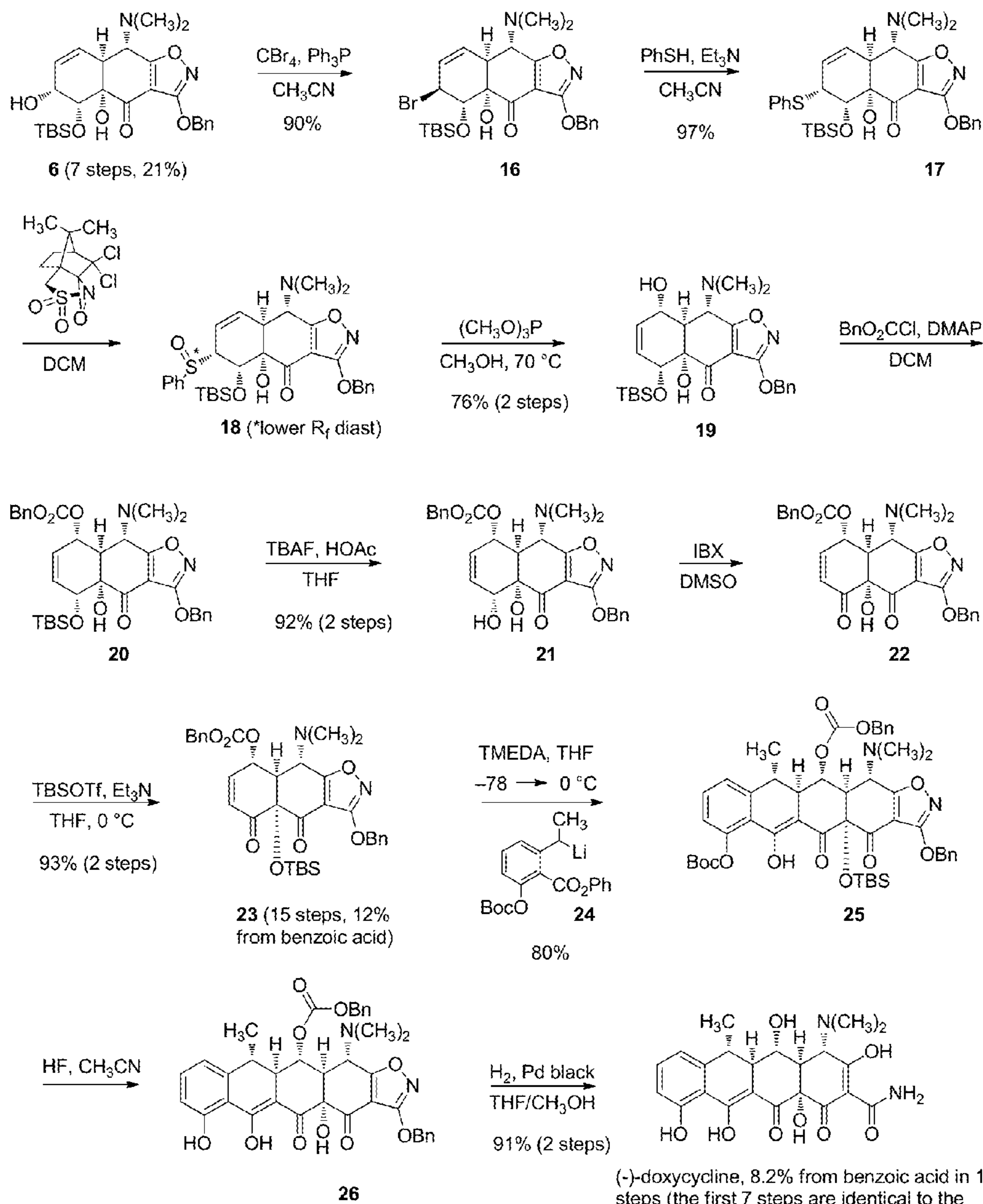
Figure 3 Total Synthesis of Doxycycline
