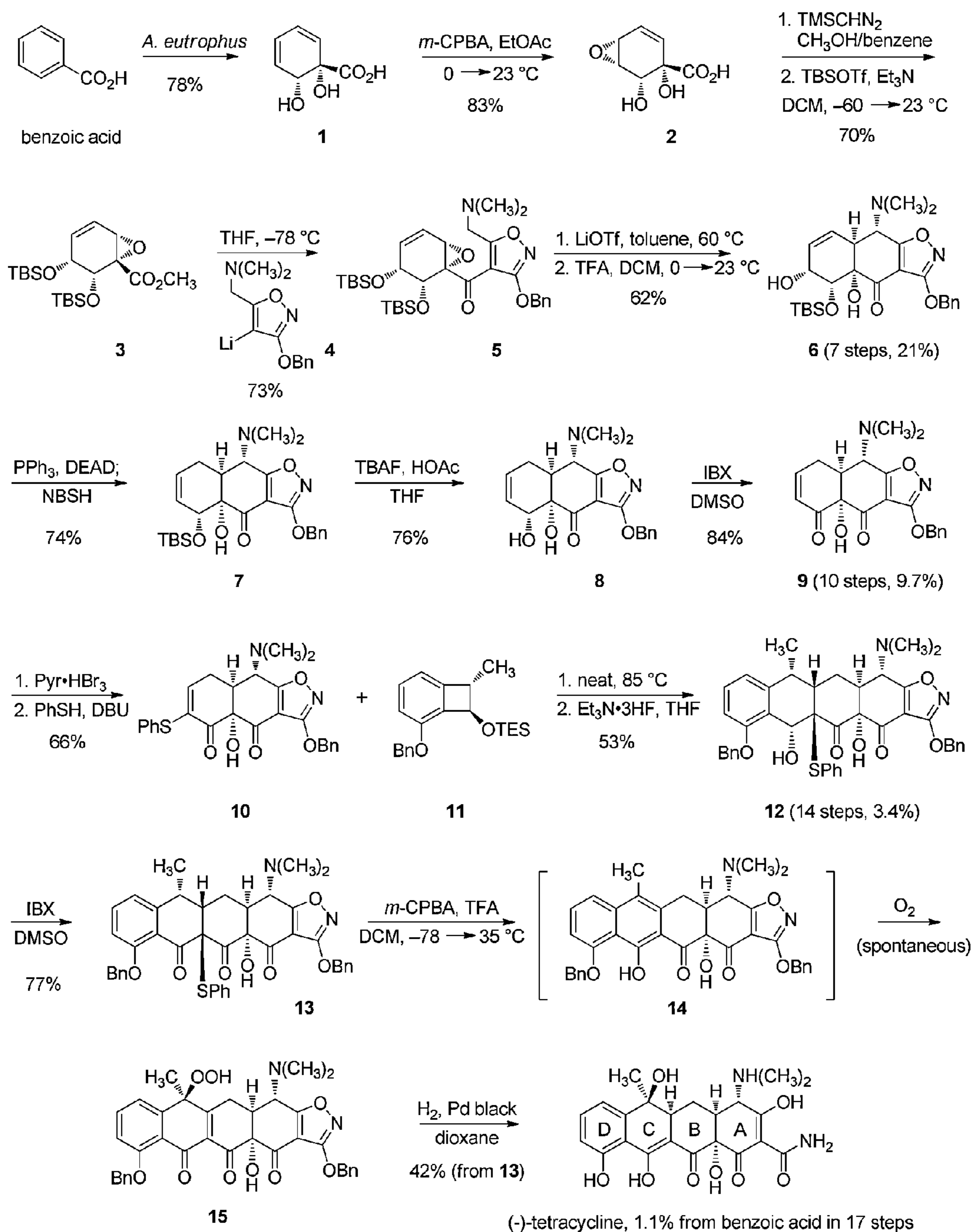
Figure 2 Total Synthesis of Tetracycline
