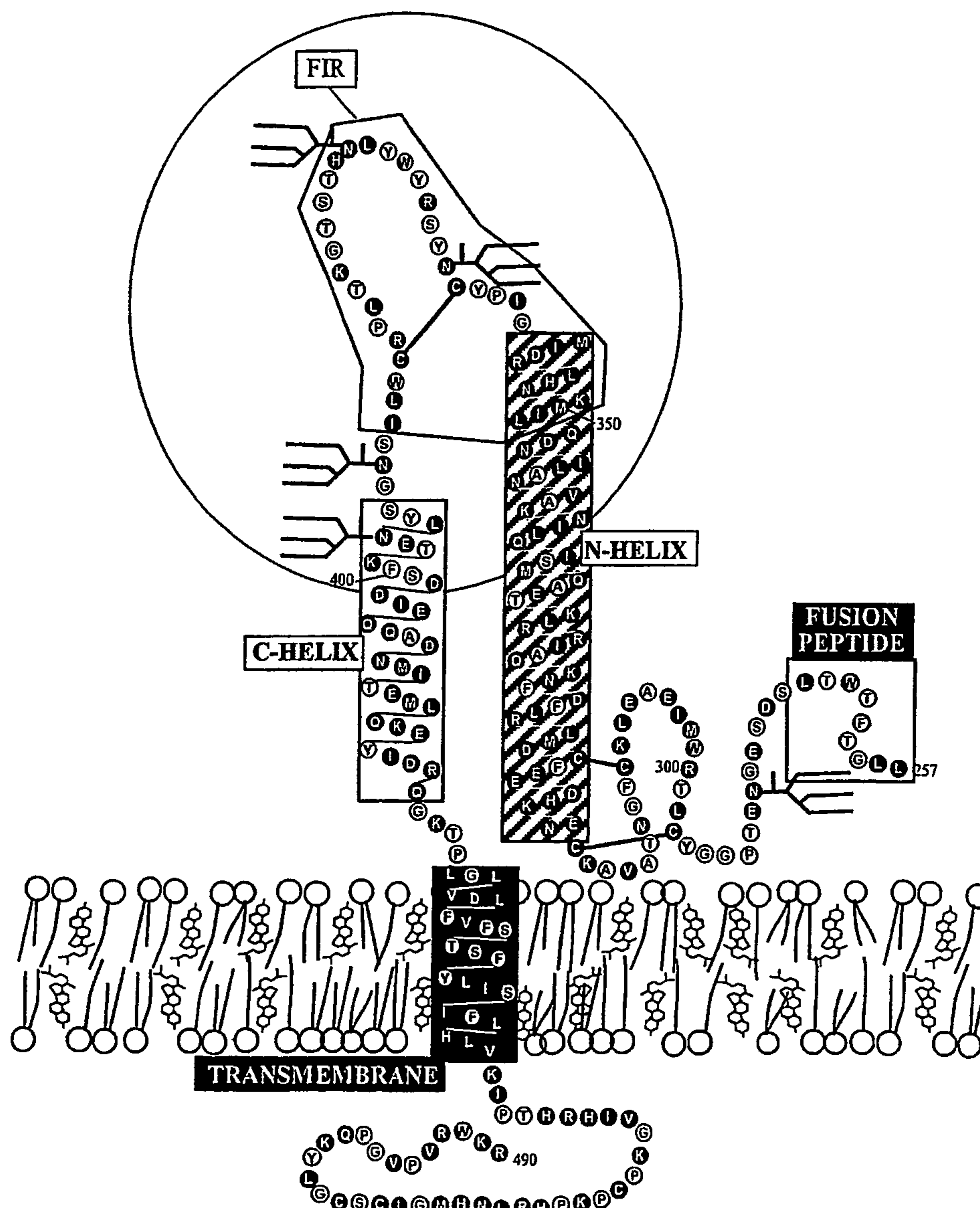
Lassa virus GP2 Figure 2
