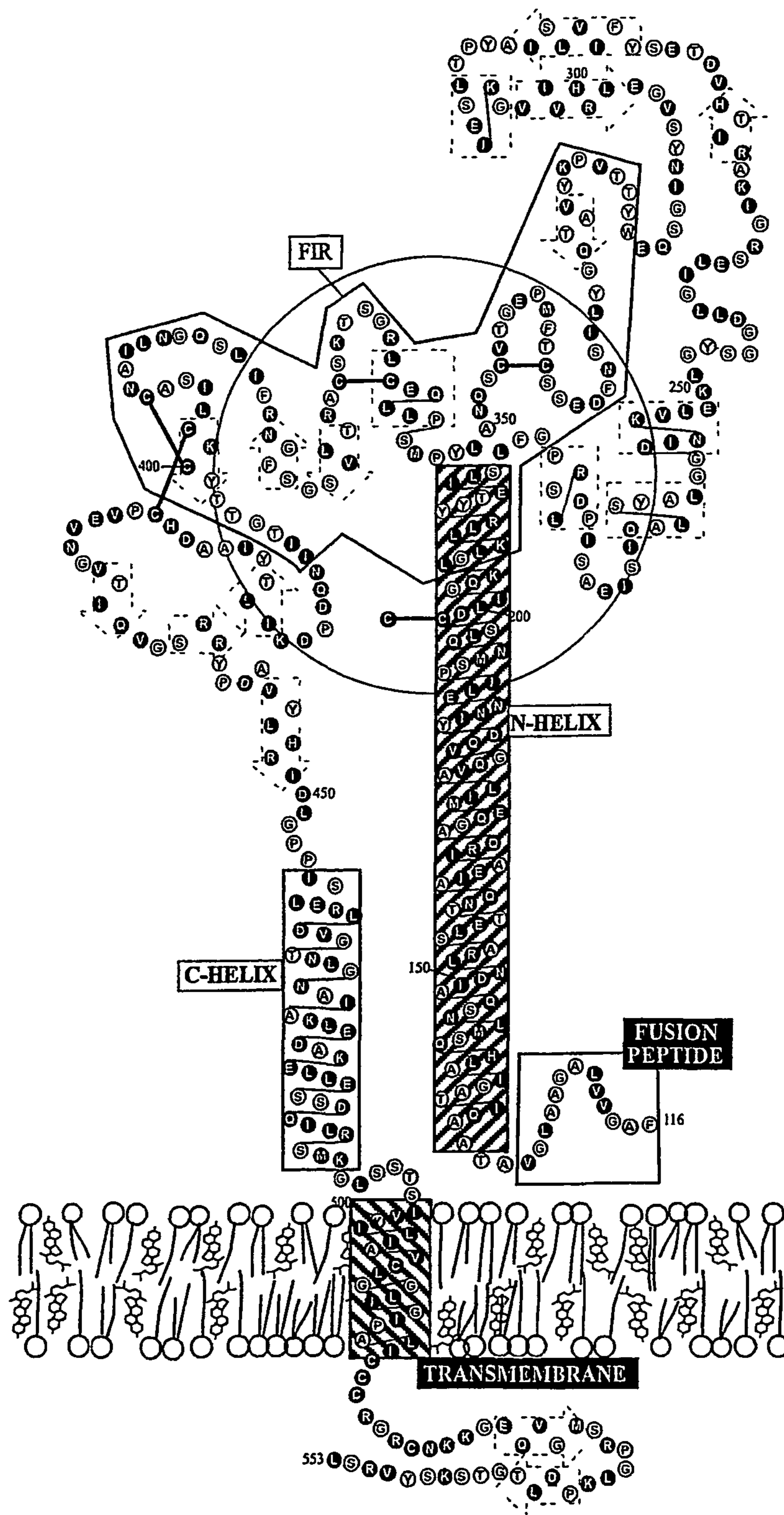
measles virus F1 Figure 6
