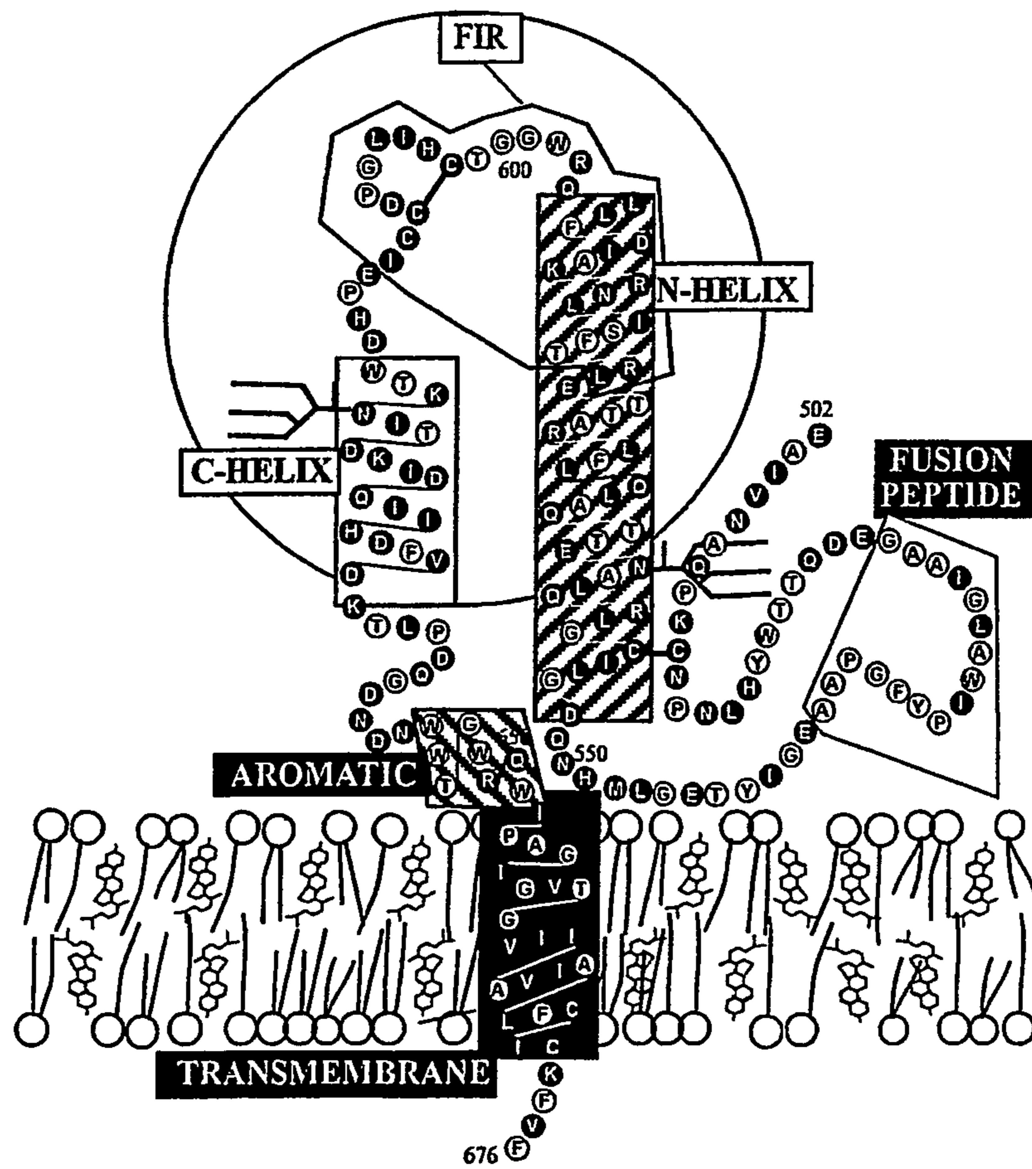
Ebola virus GP2 Figure 4
