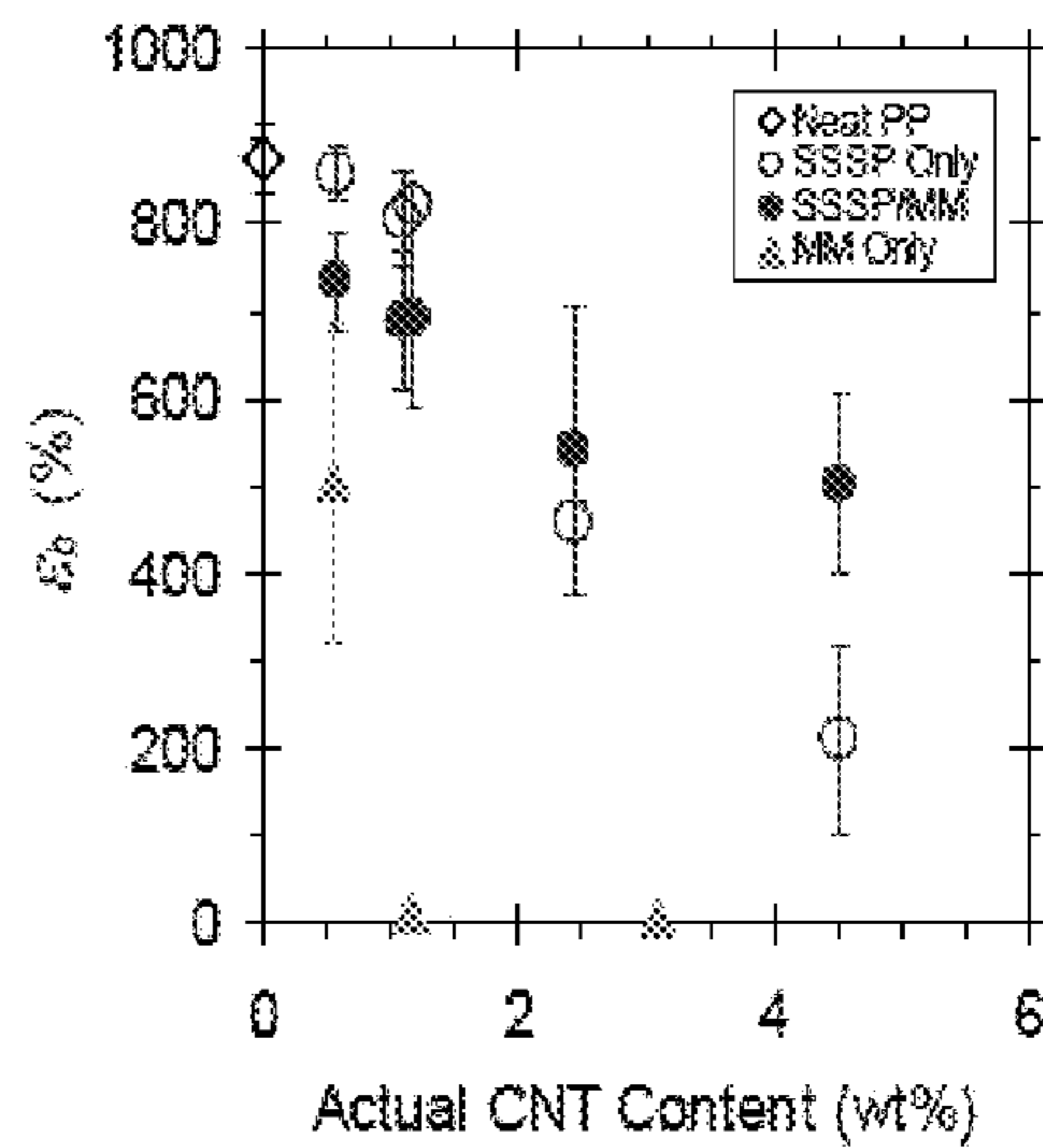
❖ CNT-2 (<8 nm \phi MWCNT)
