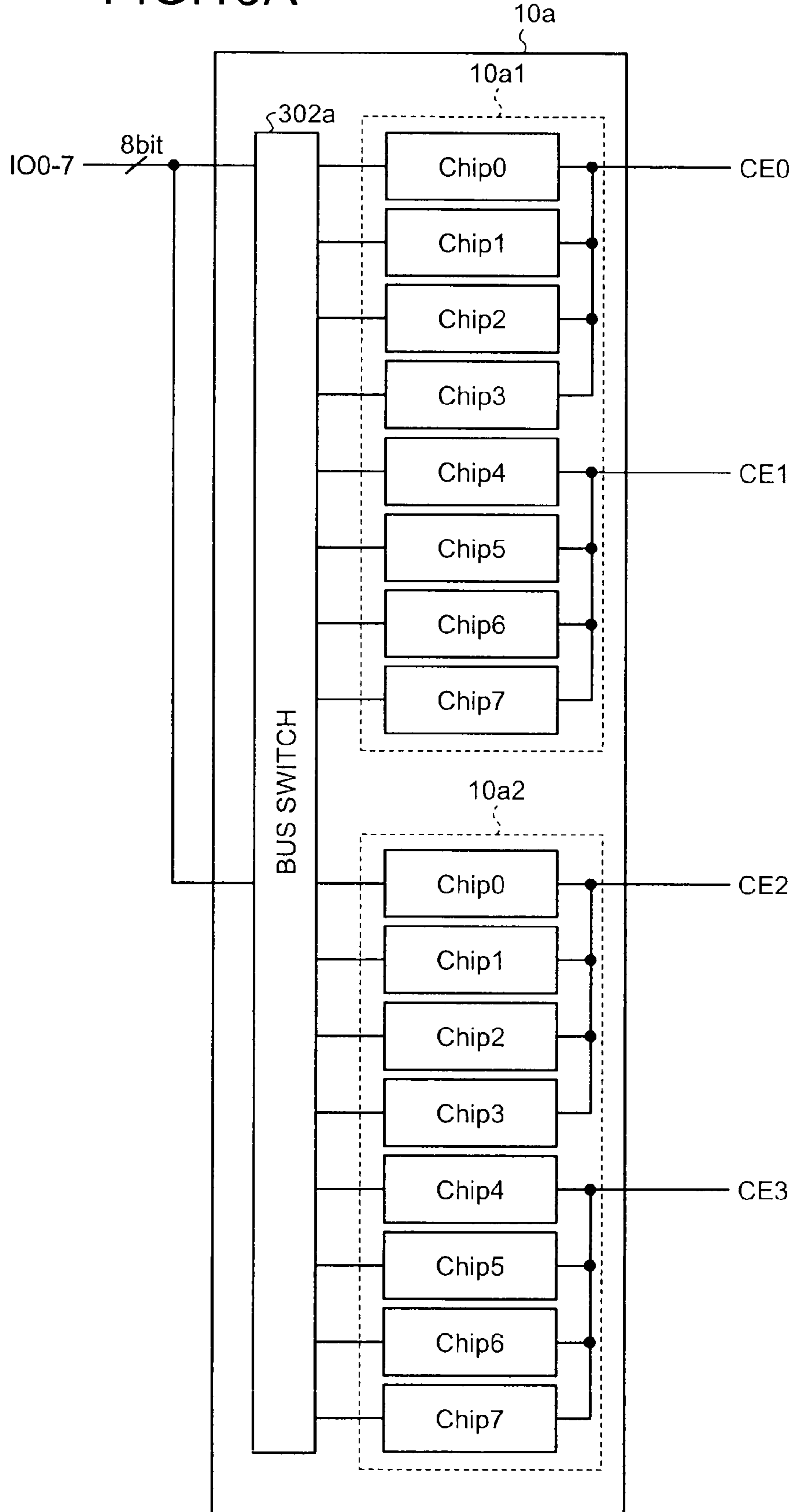
NAND MEMORY PACKAGE
