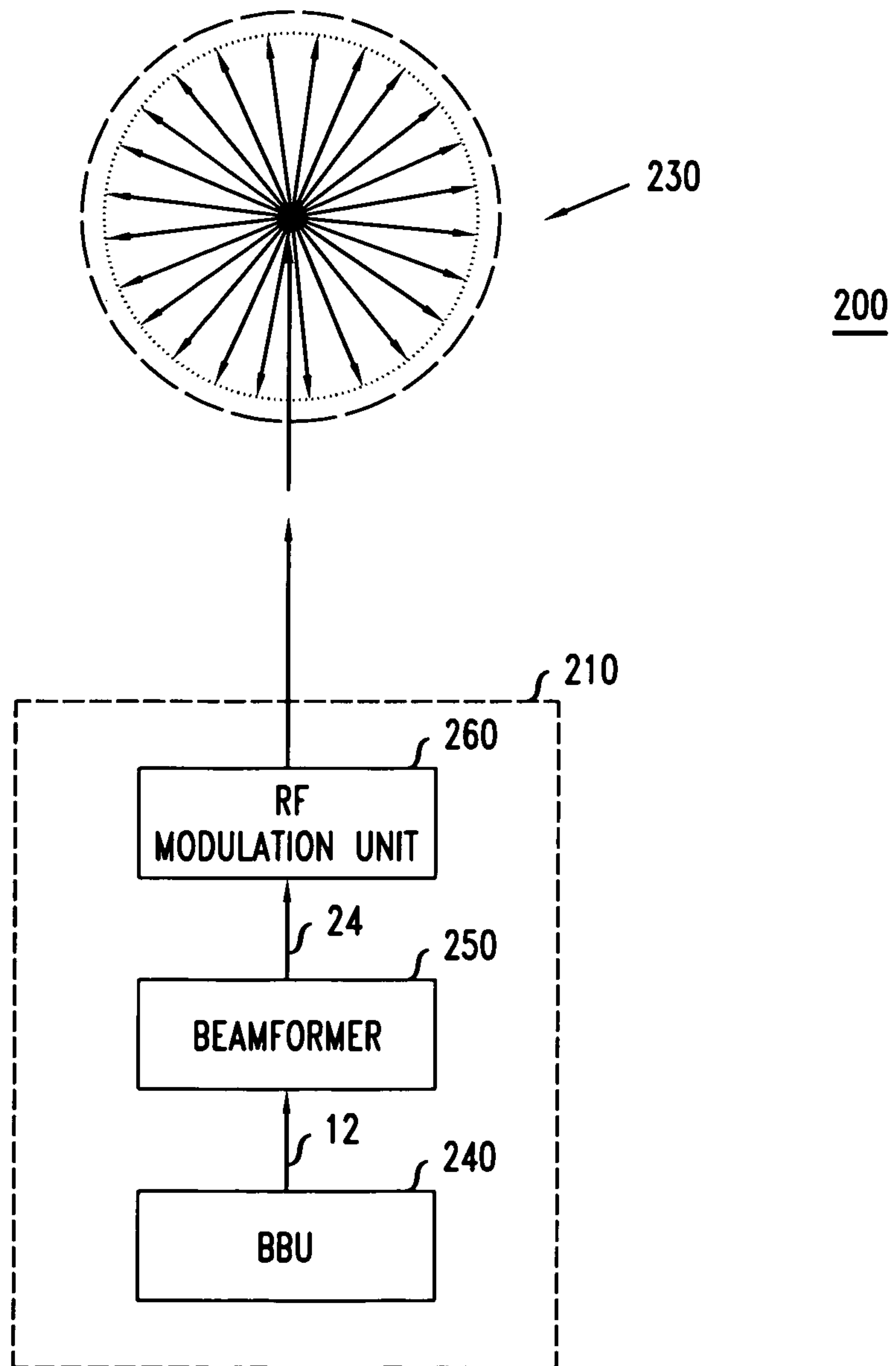
24-ANTENNA CIRCULAR ANTENNA ARRAY (TOP-DOWN VIEW)
