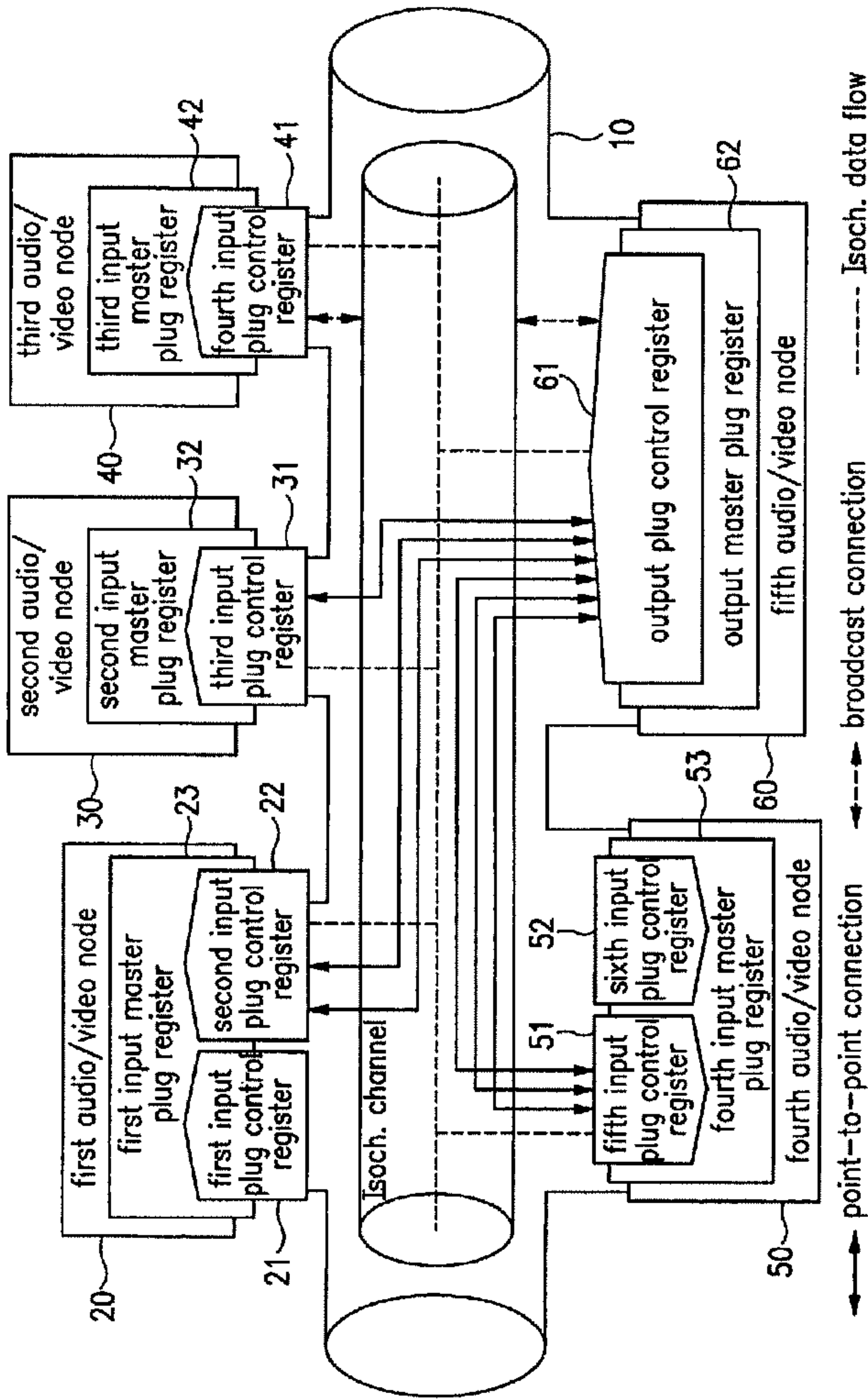
FIG. 1 Related Art
