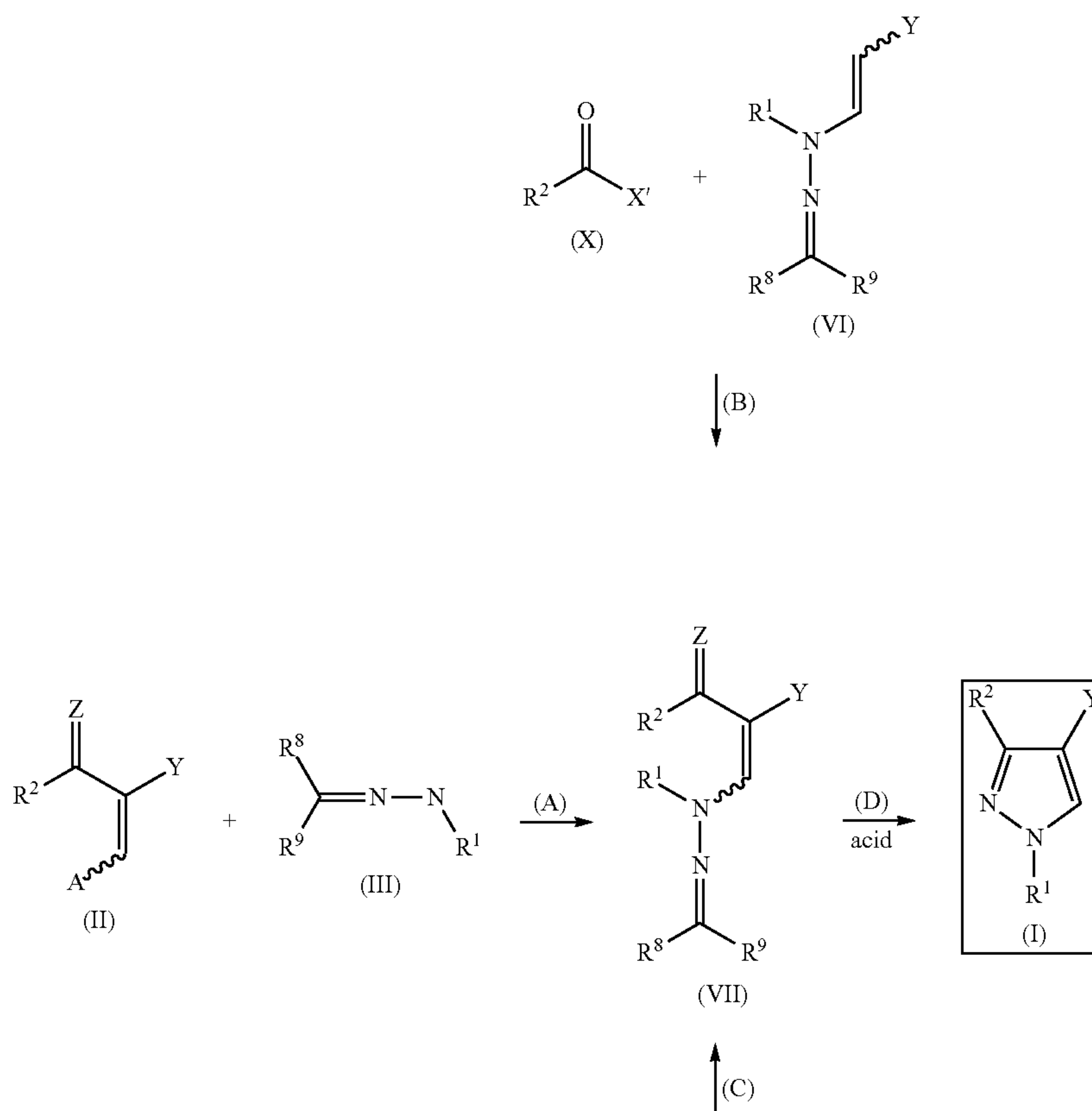
Scheme 3
