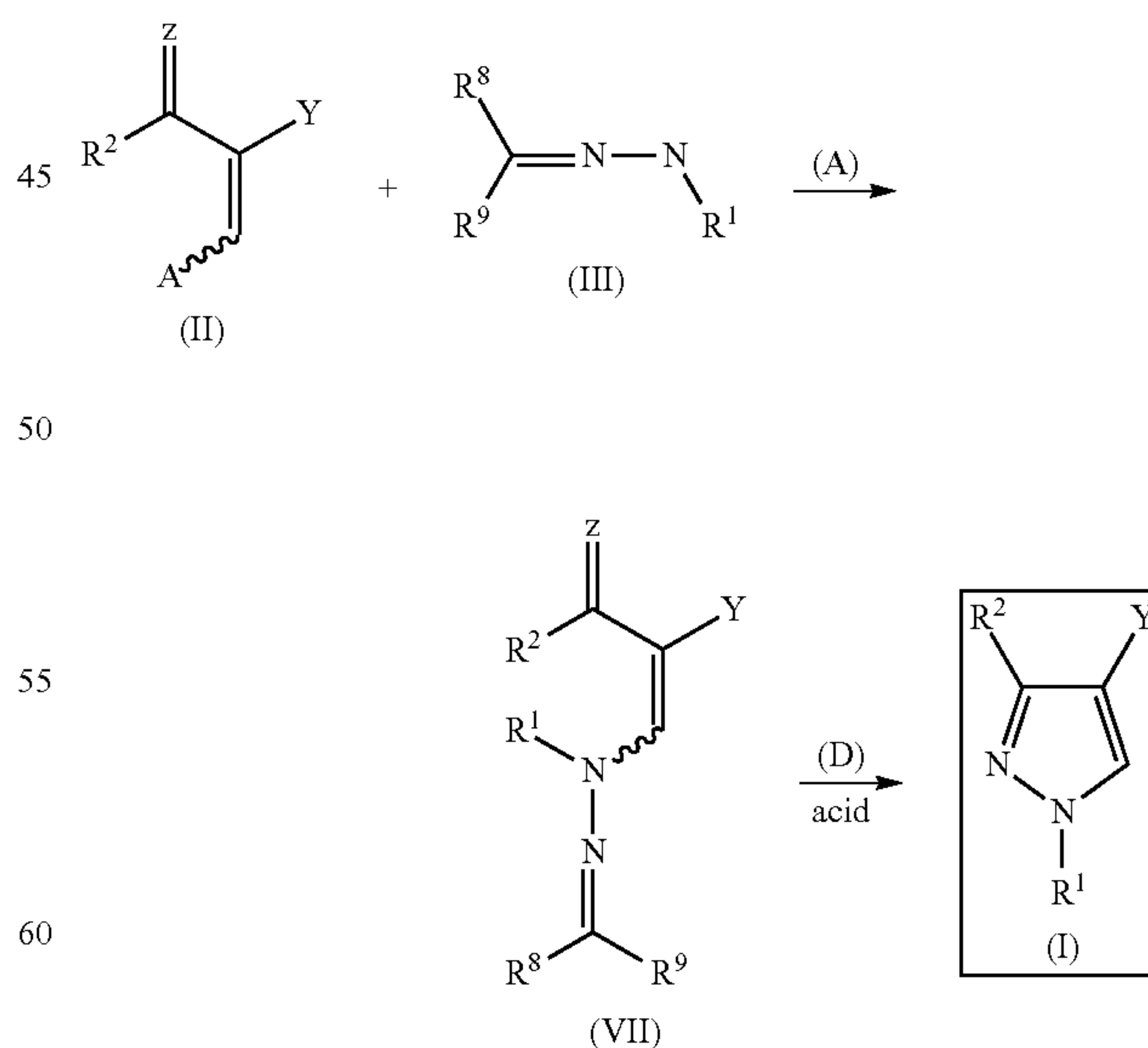
Scheme 4
