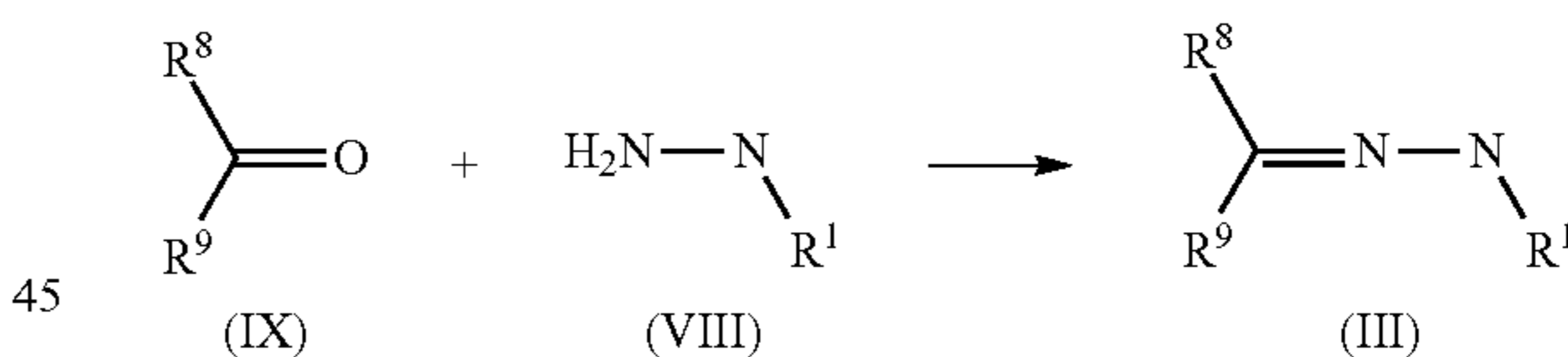
Scheme 5
