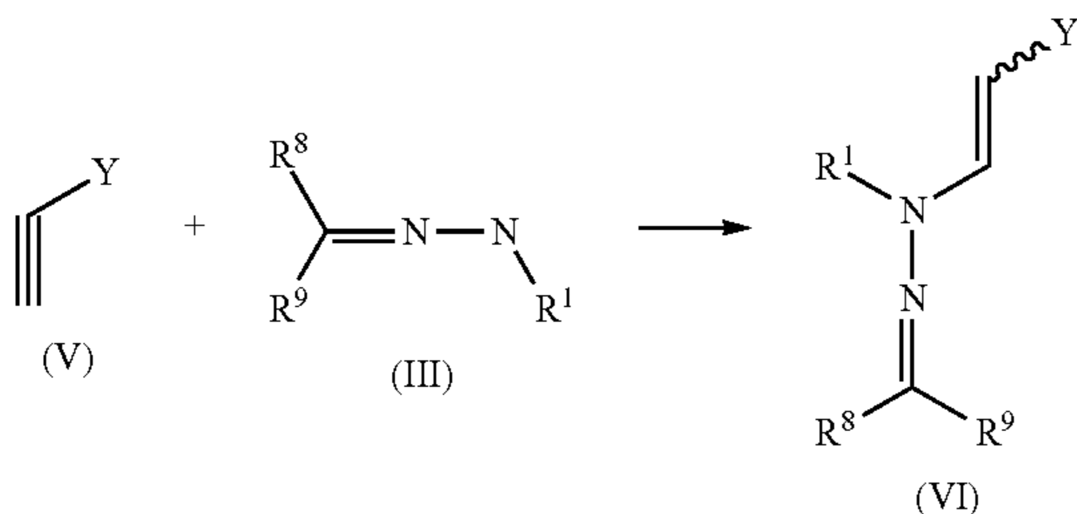
Scheme 7
