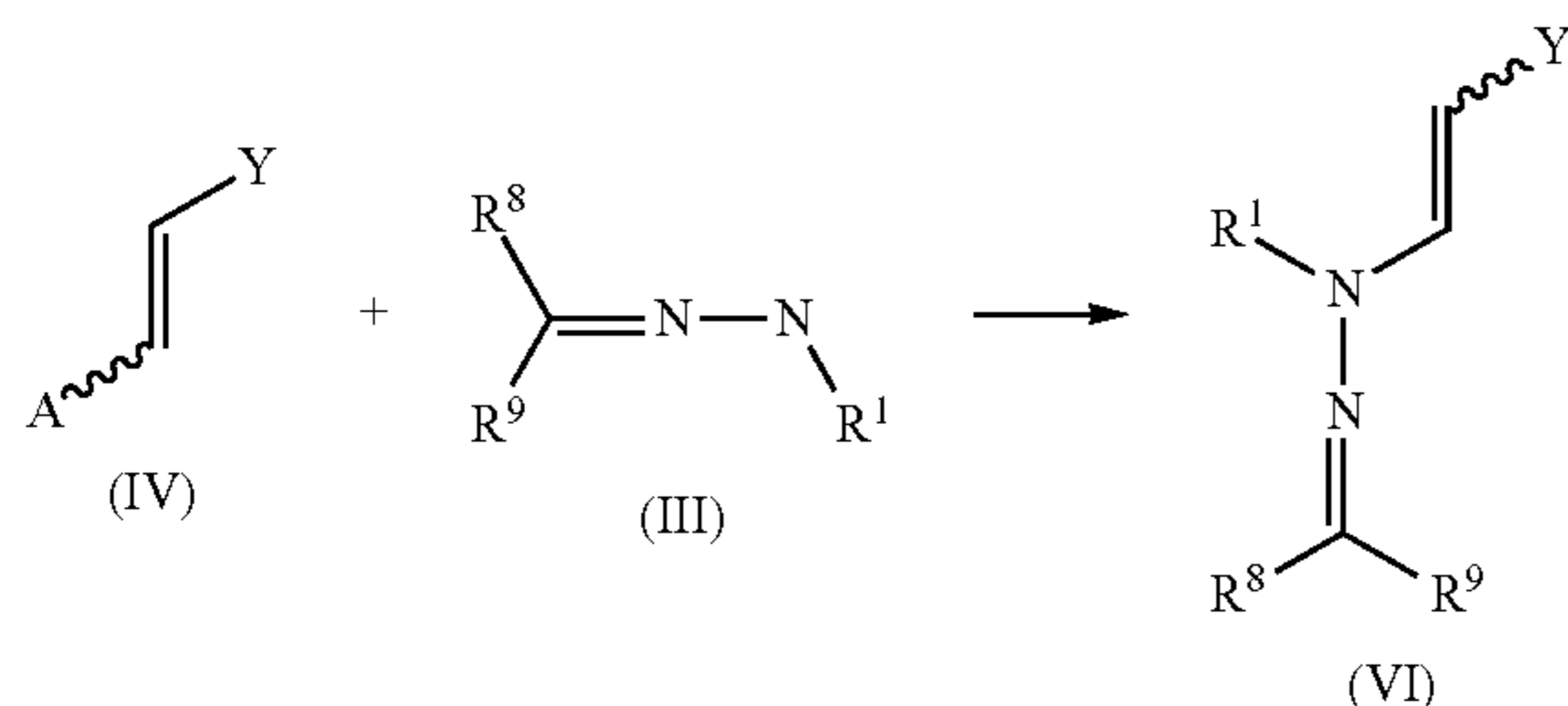
Scheme 8
