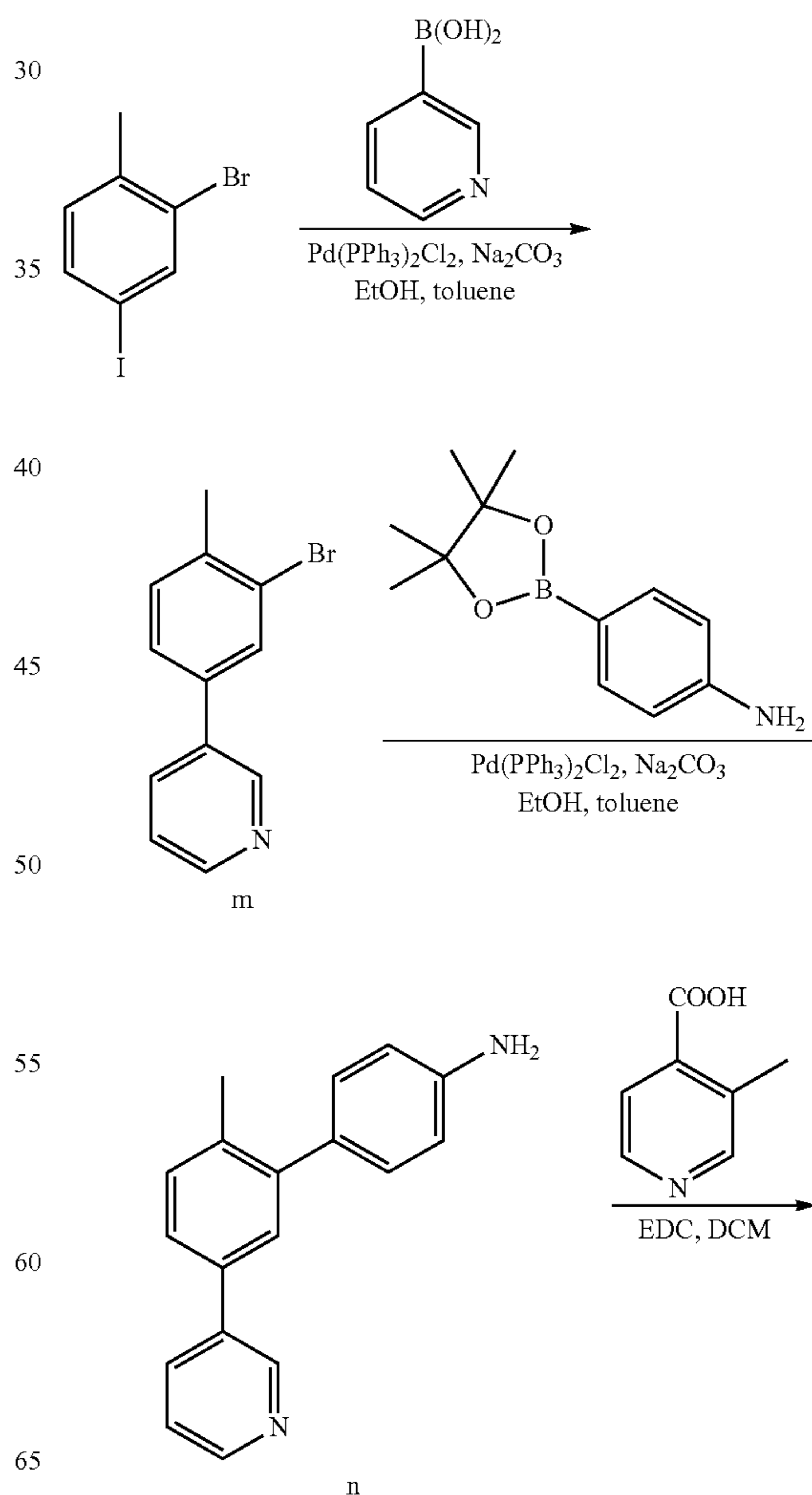
Scheme IX
