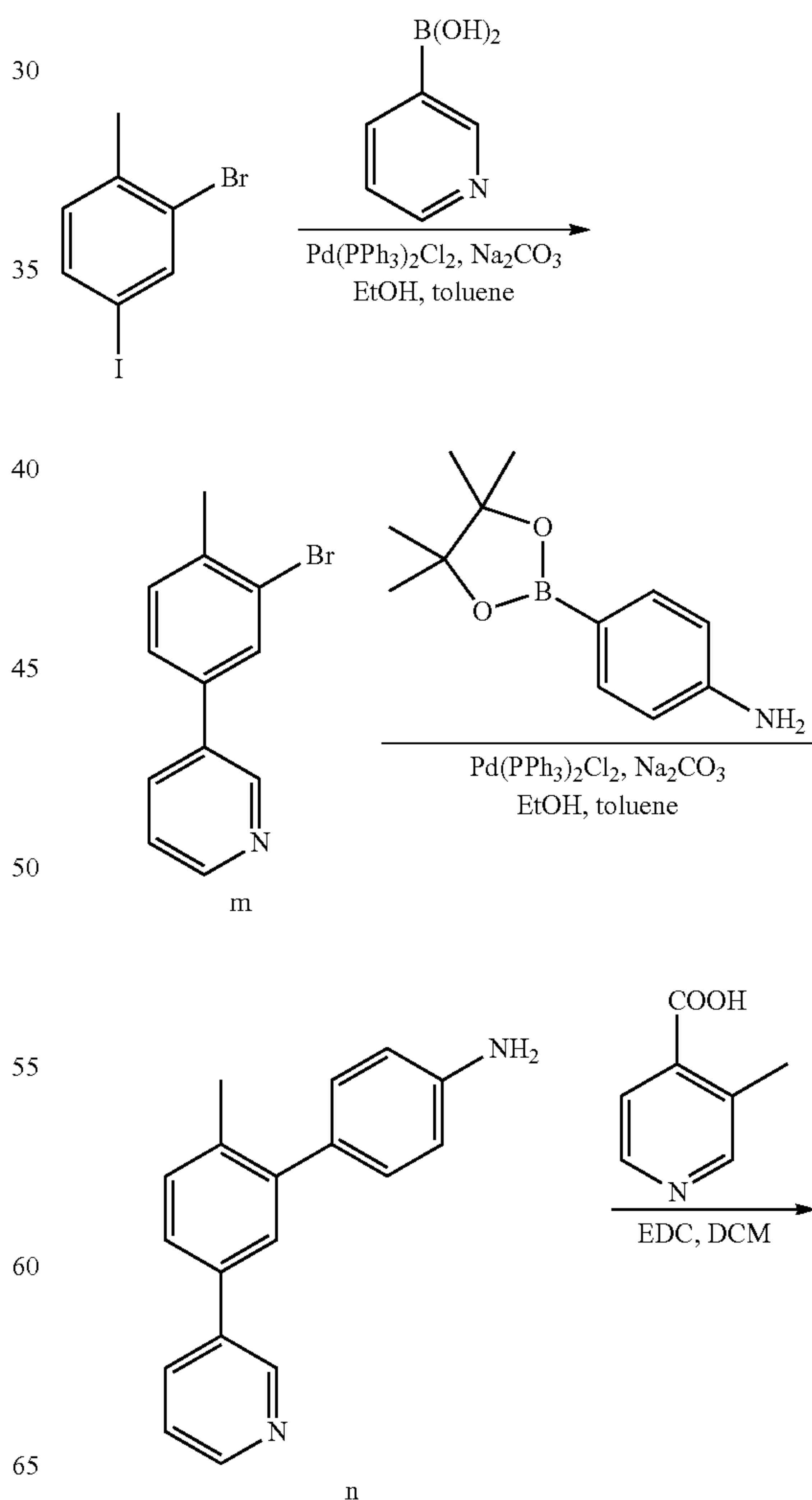
Scheme IX
