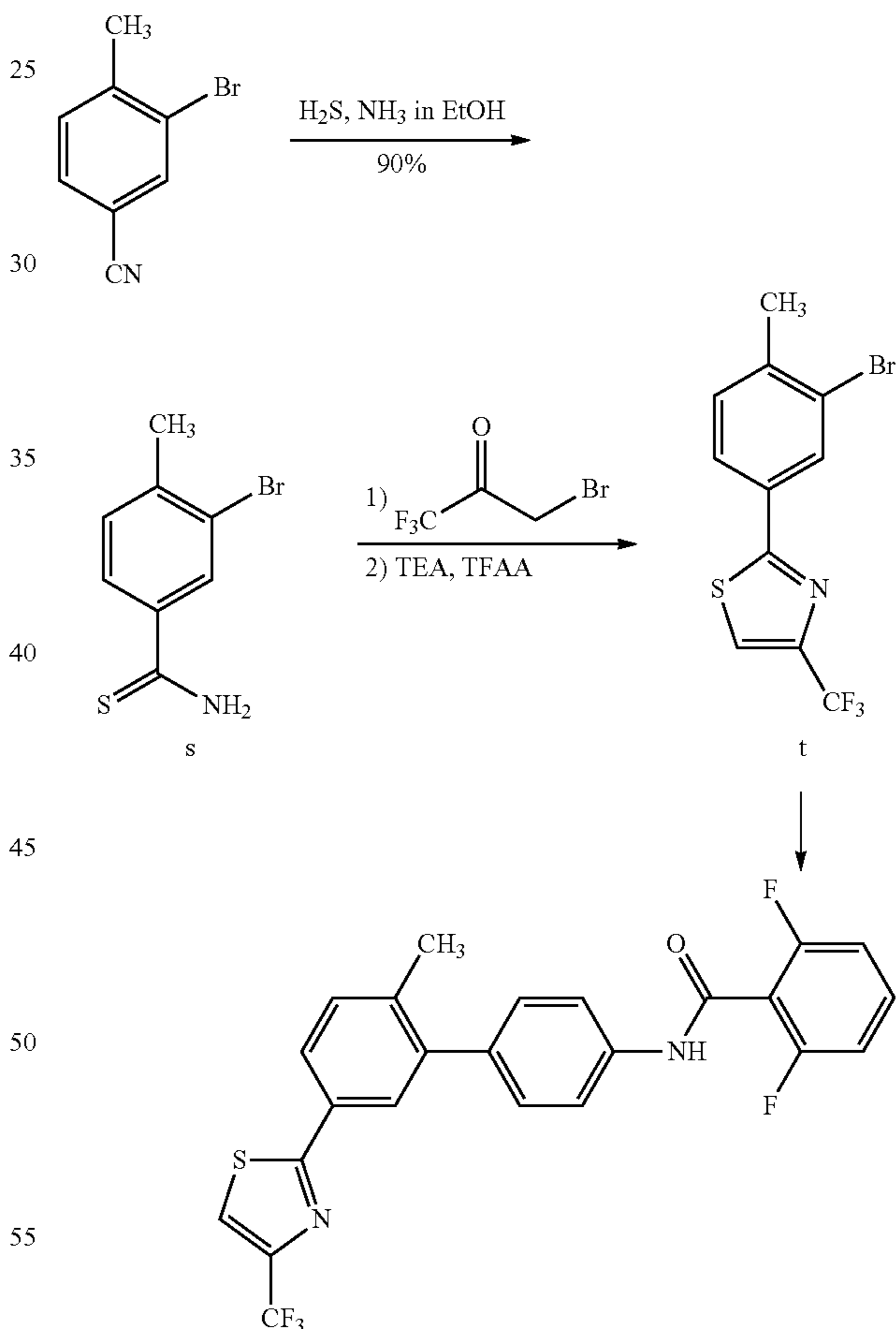
Compound 39
