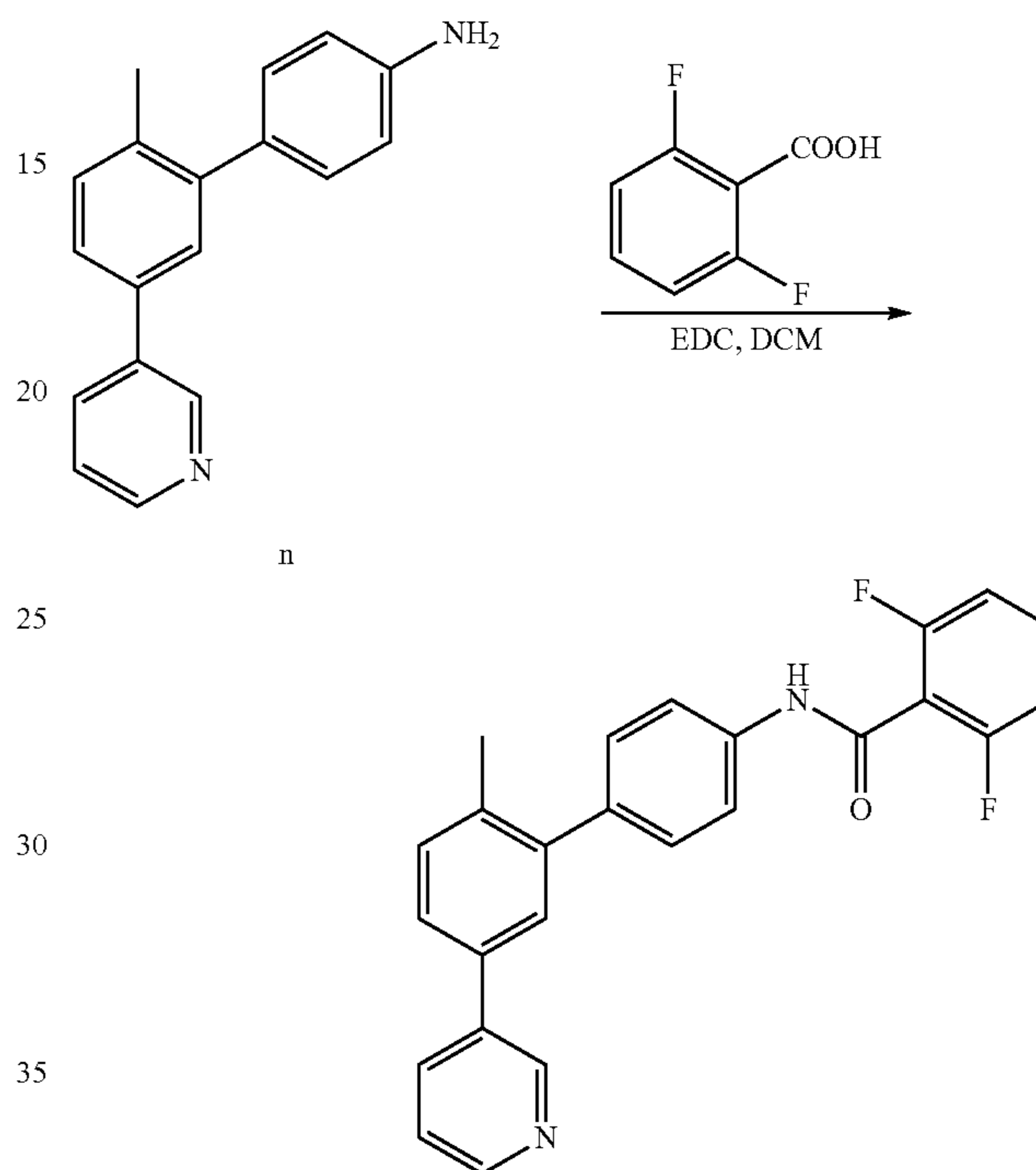
Compound 22
