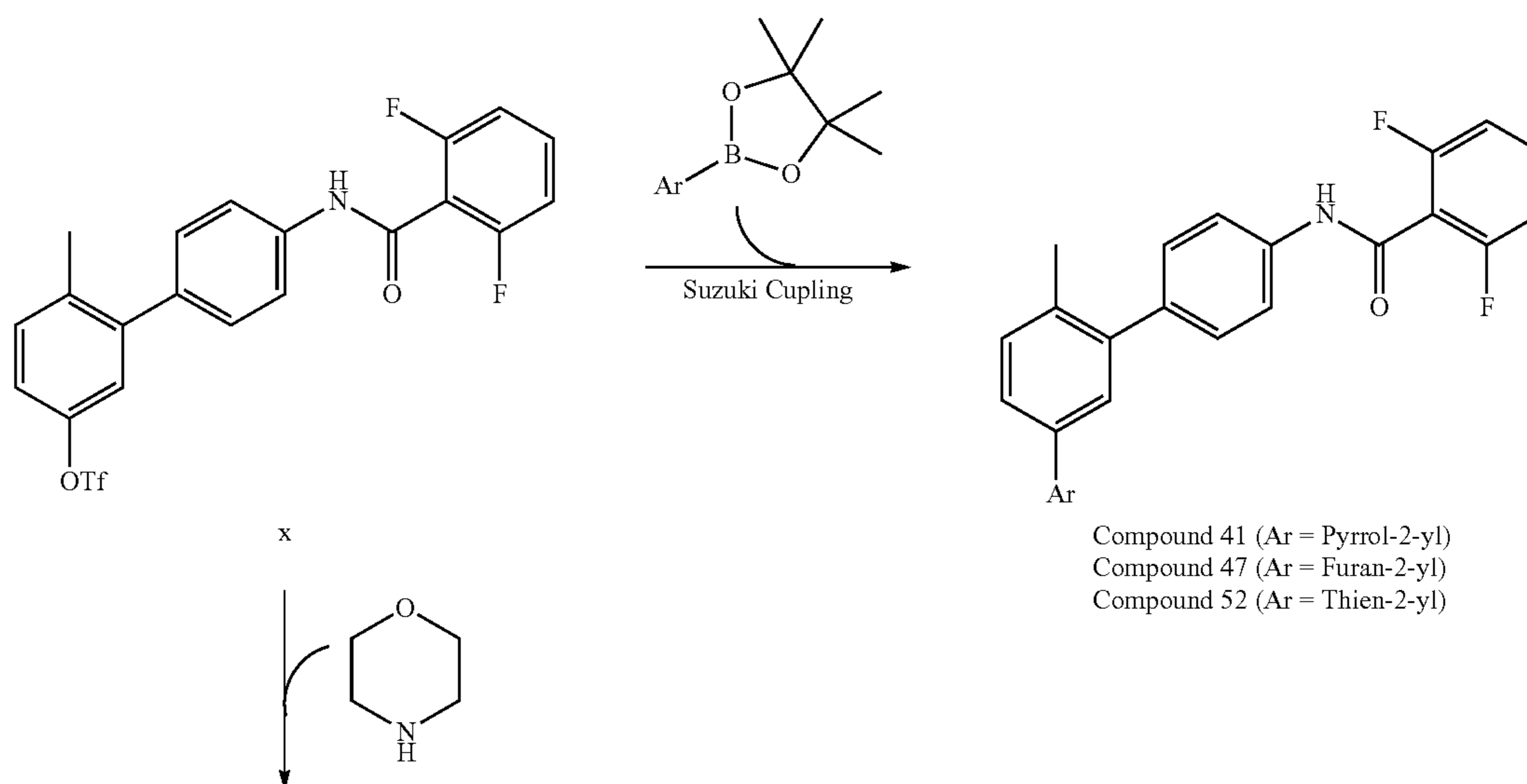
Scheme XVIII
