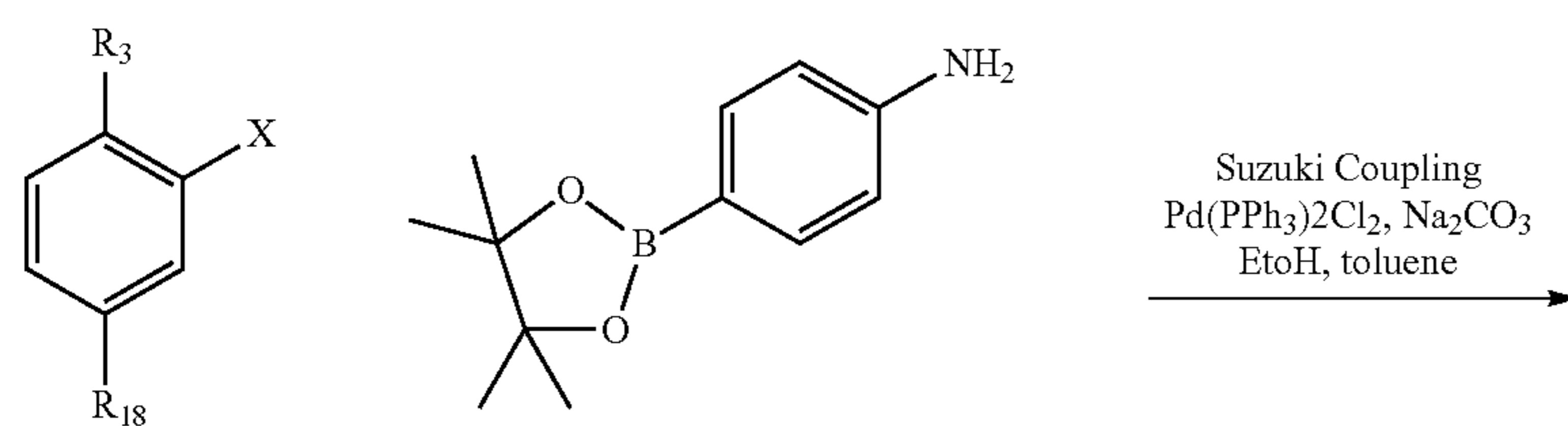
Scheme B
