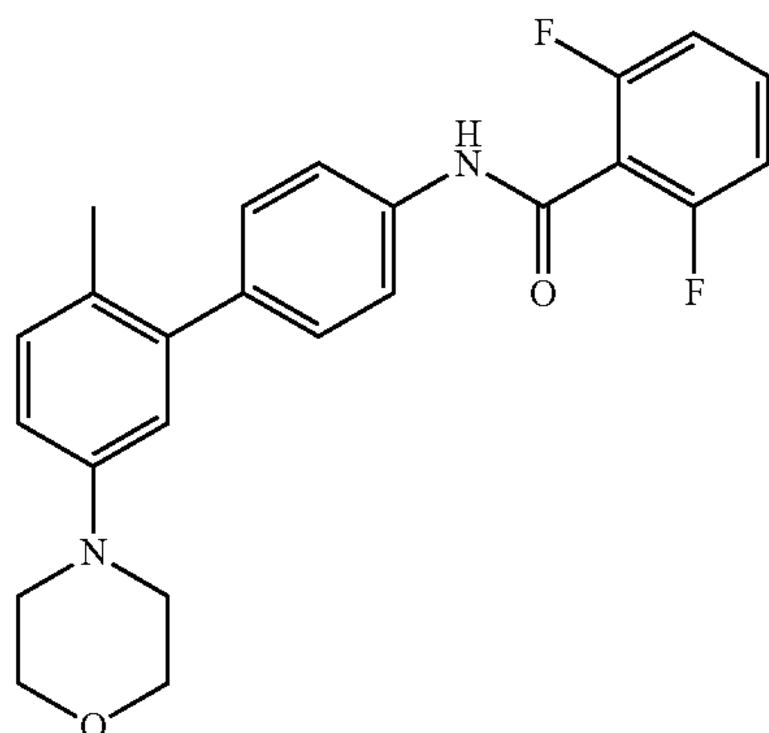
Compound 43
