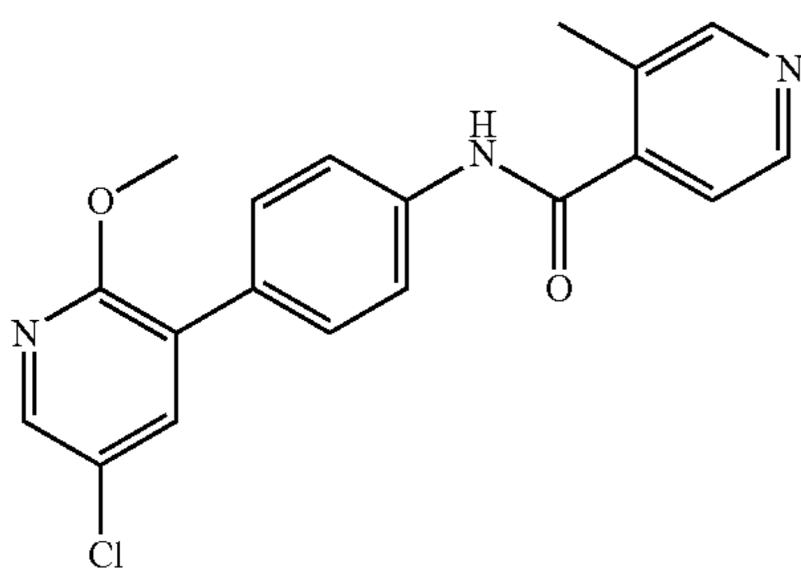
Compound 18: 3-Methyl-N-[4-(5-chloro-2-methoxy-pyridin-3-yl)-phenyl]-isonicotinamide
