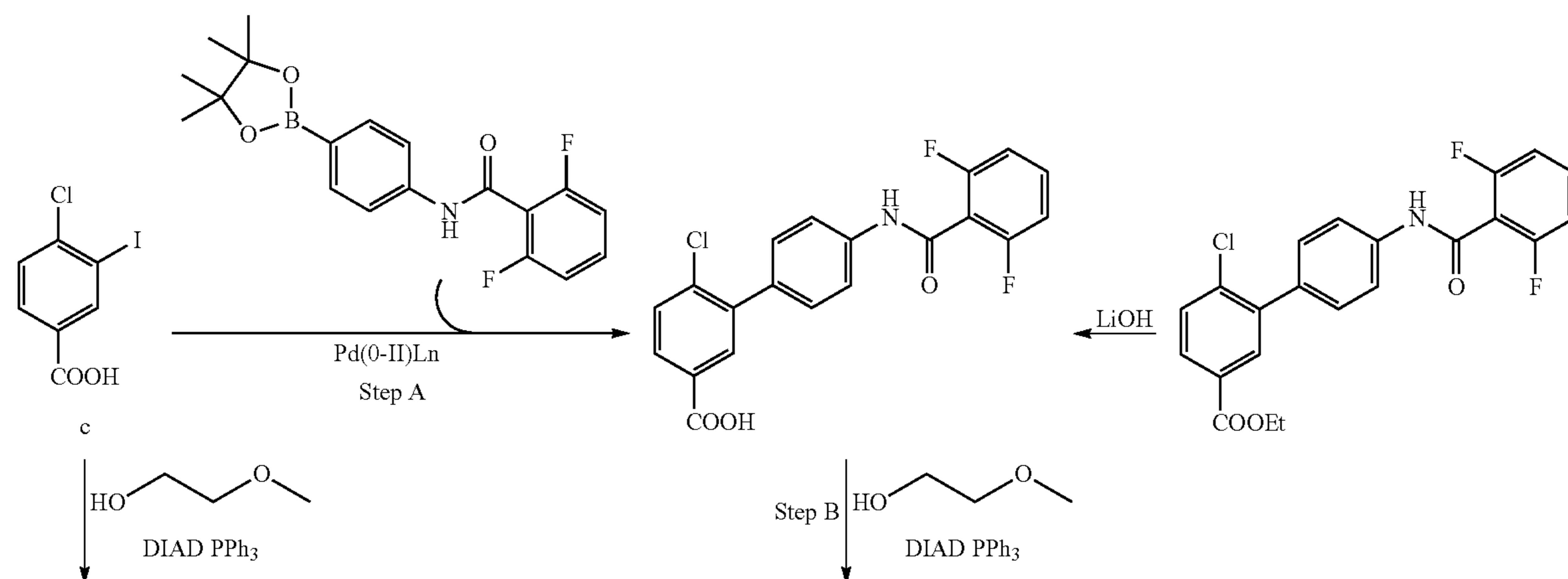
Scheme II
