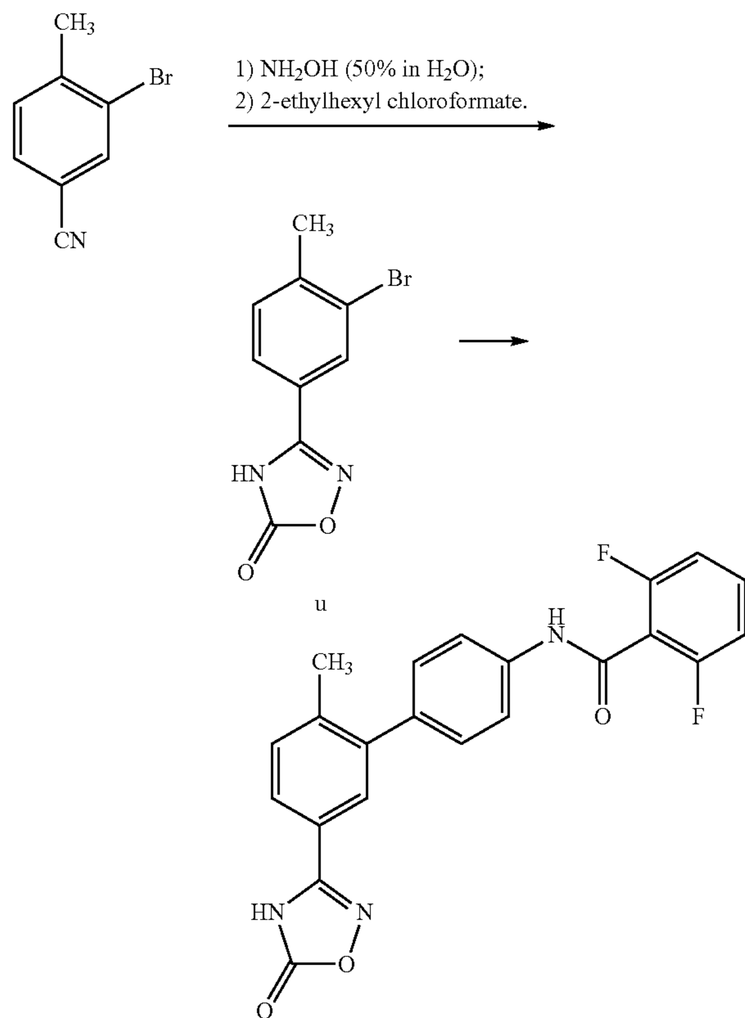
Compound 42
