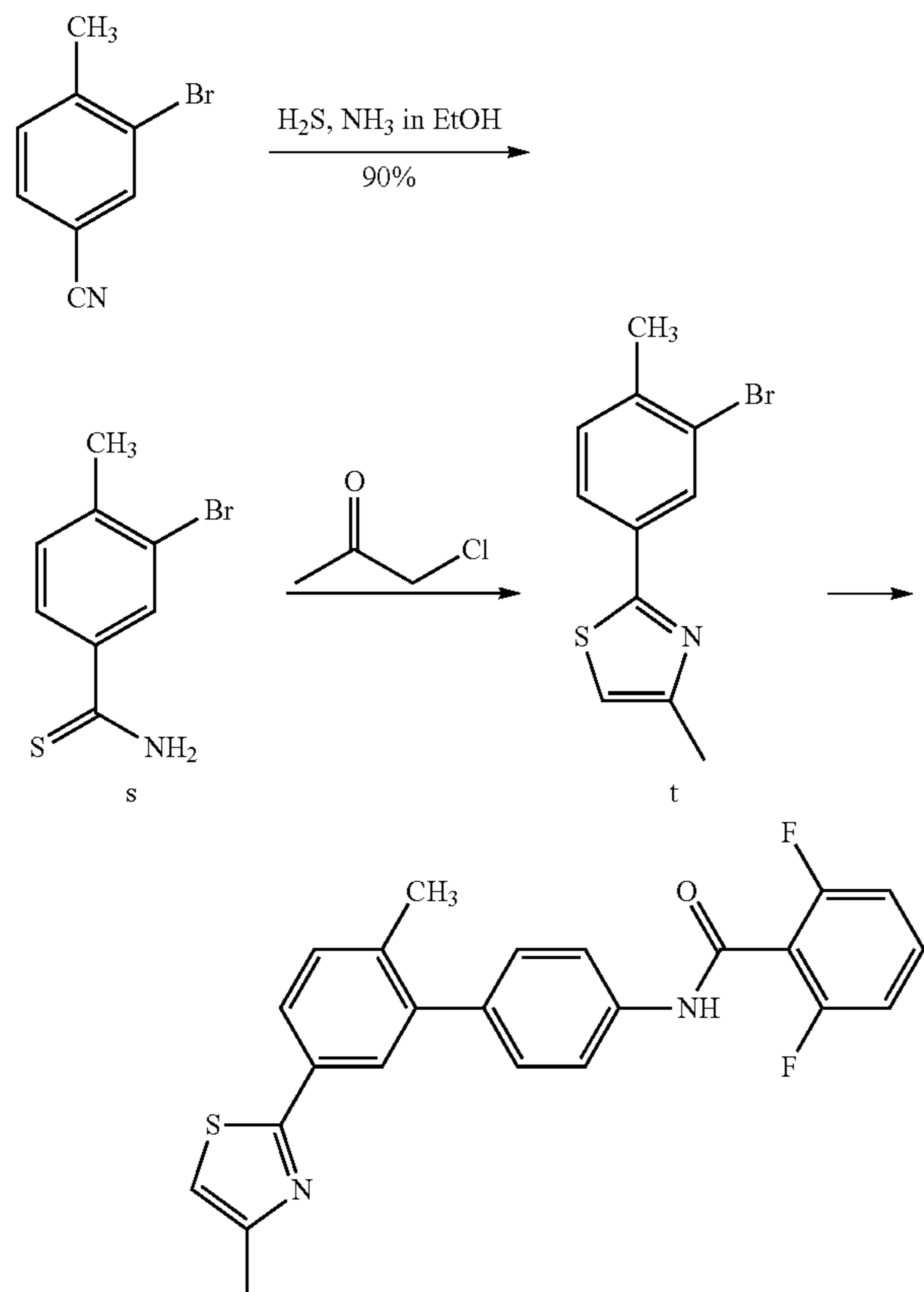
Compound 38
