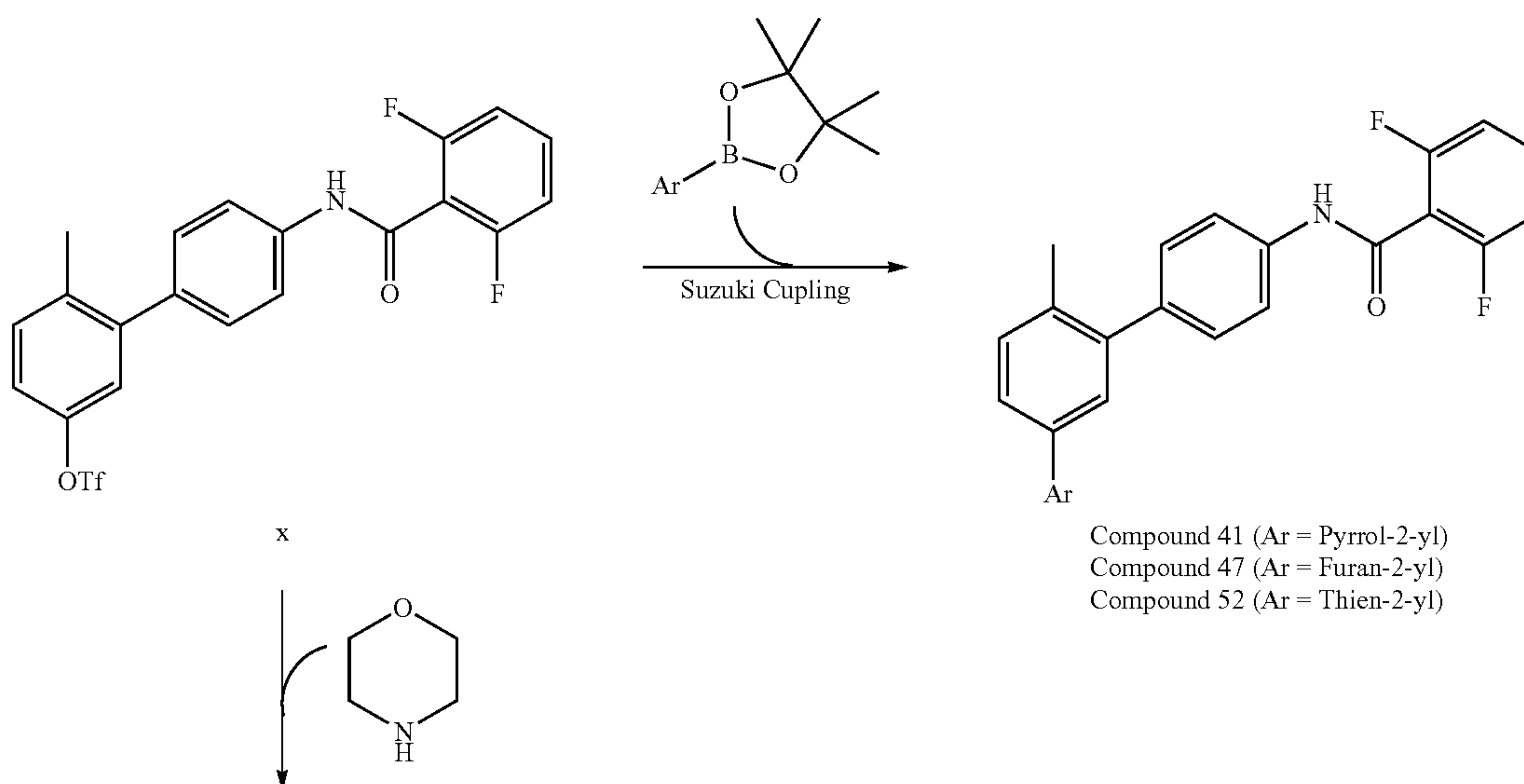
Scheme XVIII
