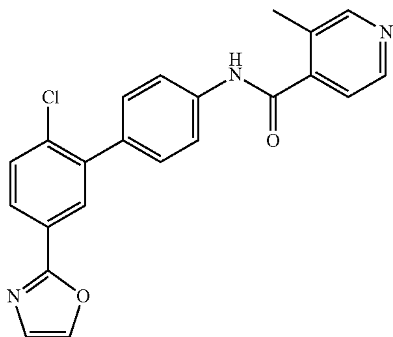
Compound 16: 3-Methyl-N-(2'-chloro-5'-oxazol-2-yl-biphenyl-4-yl)-isonicotinamide
