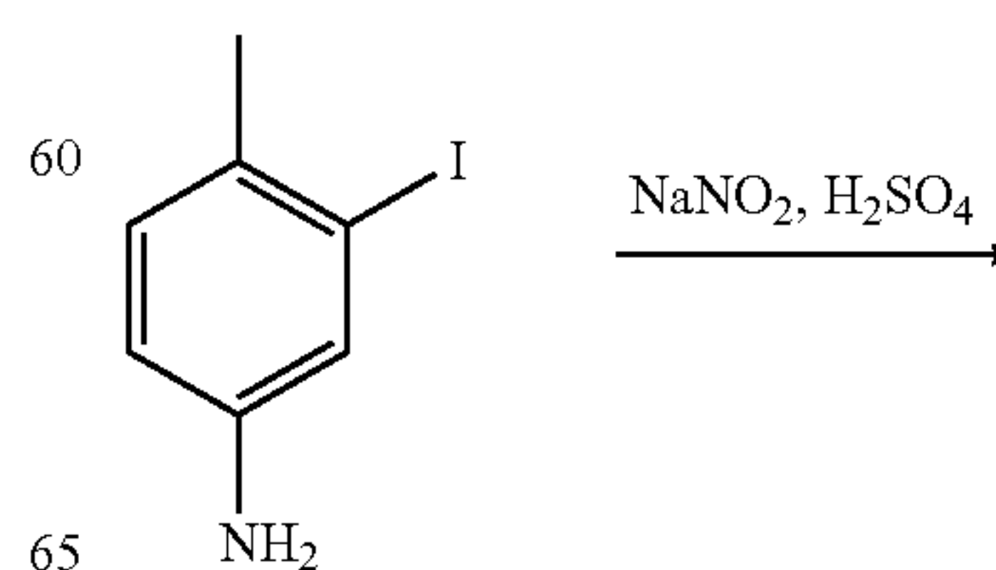
Scheme XVII
