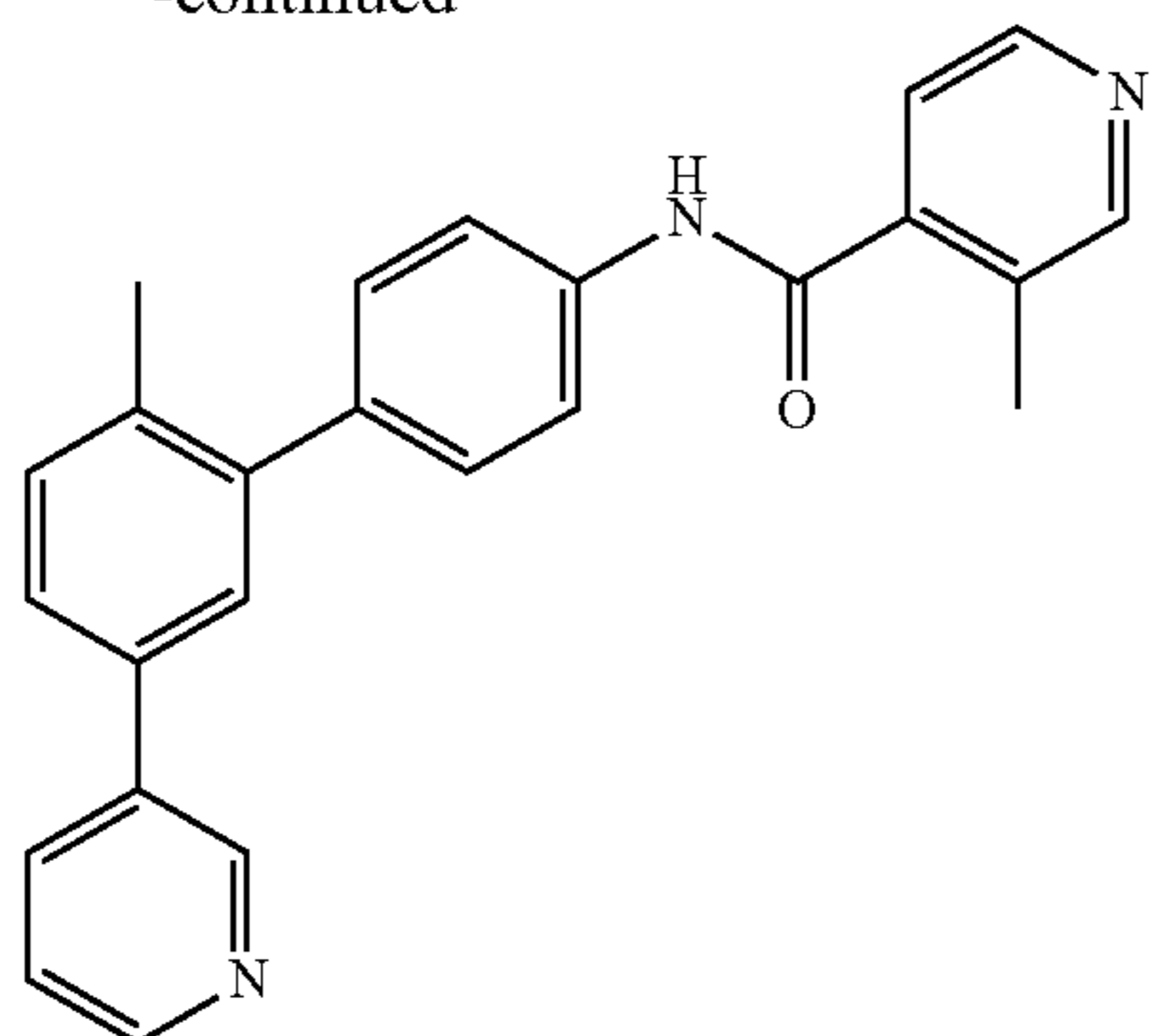
Compound 20
