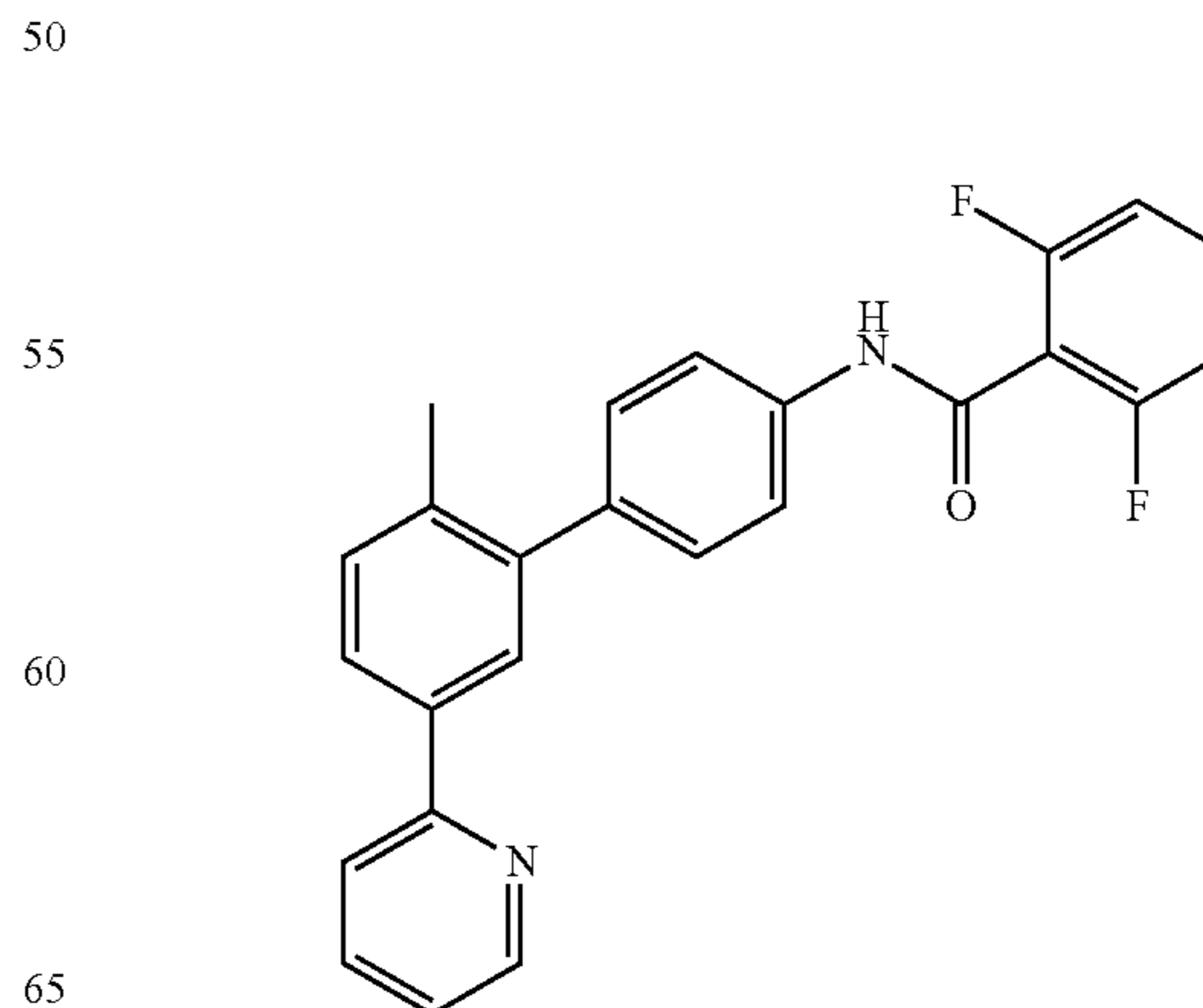
Compound 23: 2,6-Difluoro-N-[2'-methyl-5'-(pyridin-2-yl)-biphenyl-4-yl]-benzamide
