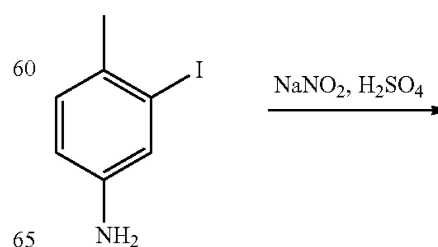
Scheme XVII
