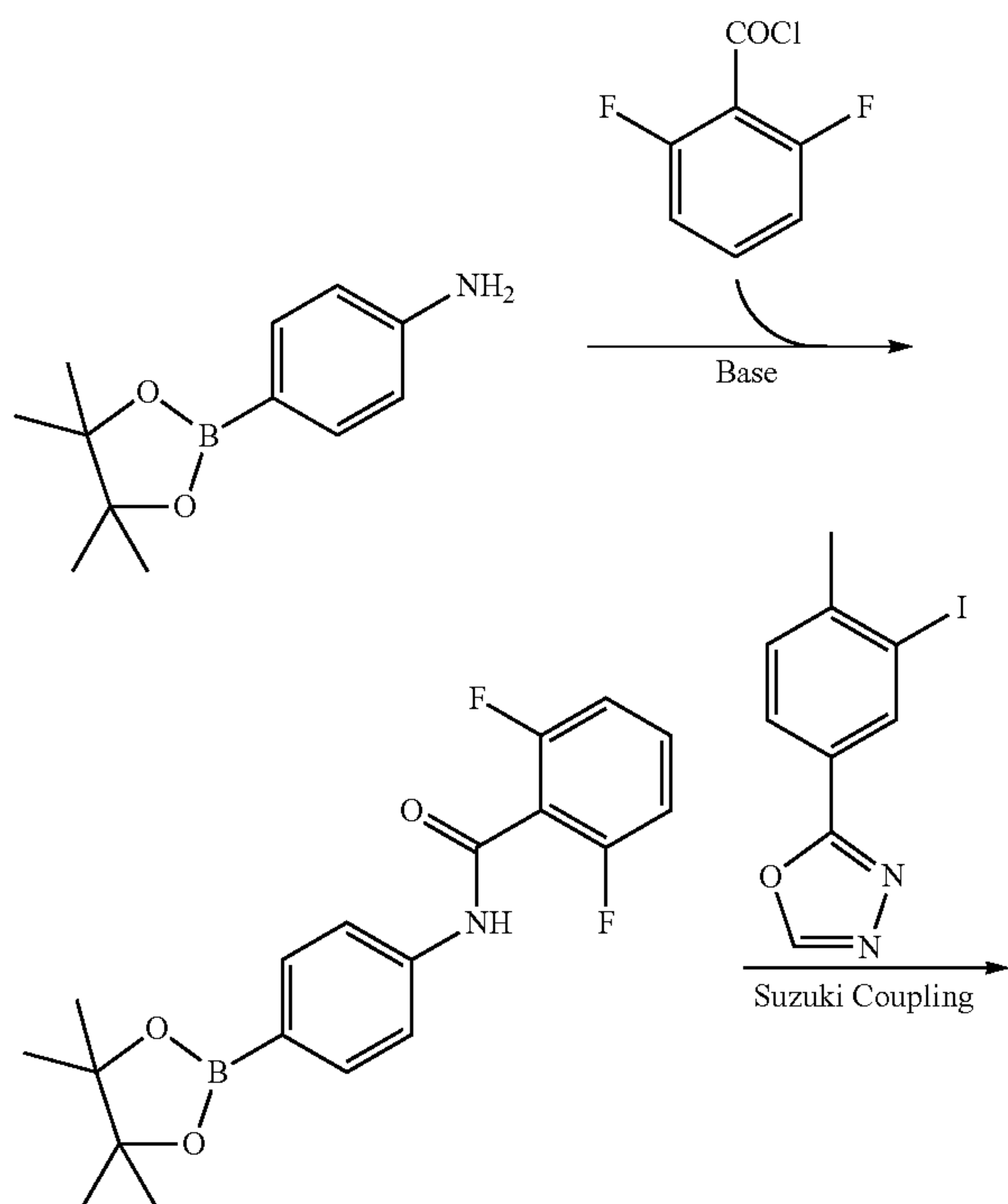
Scheme XX
