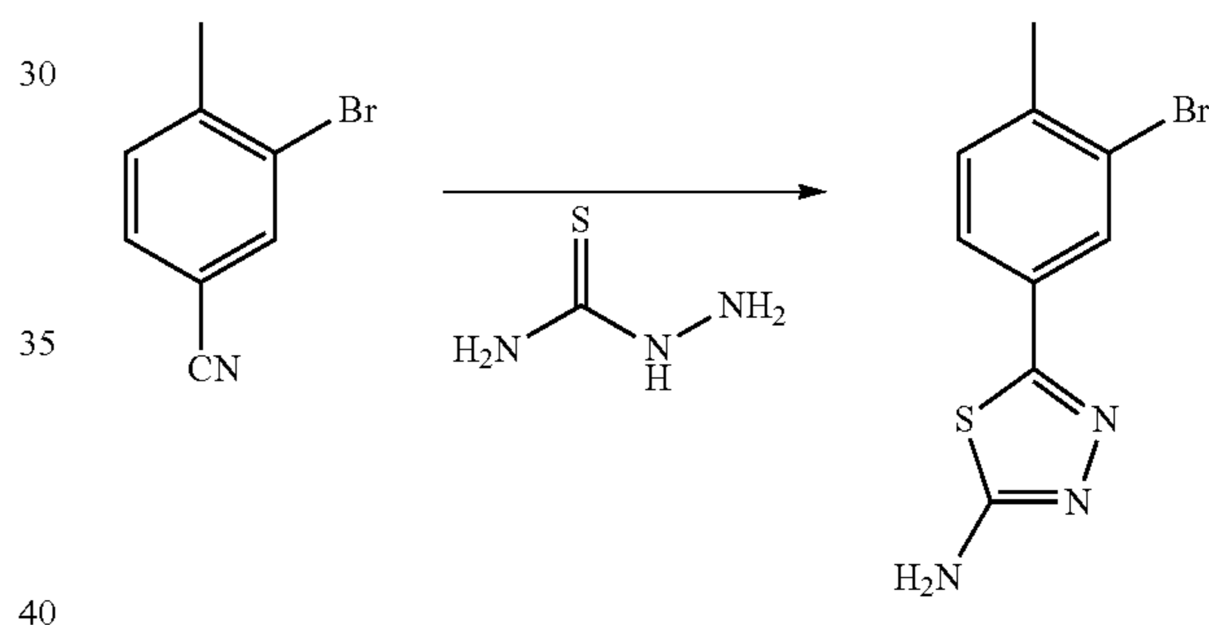
Scheme XXII
