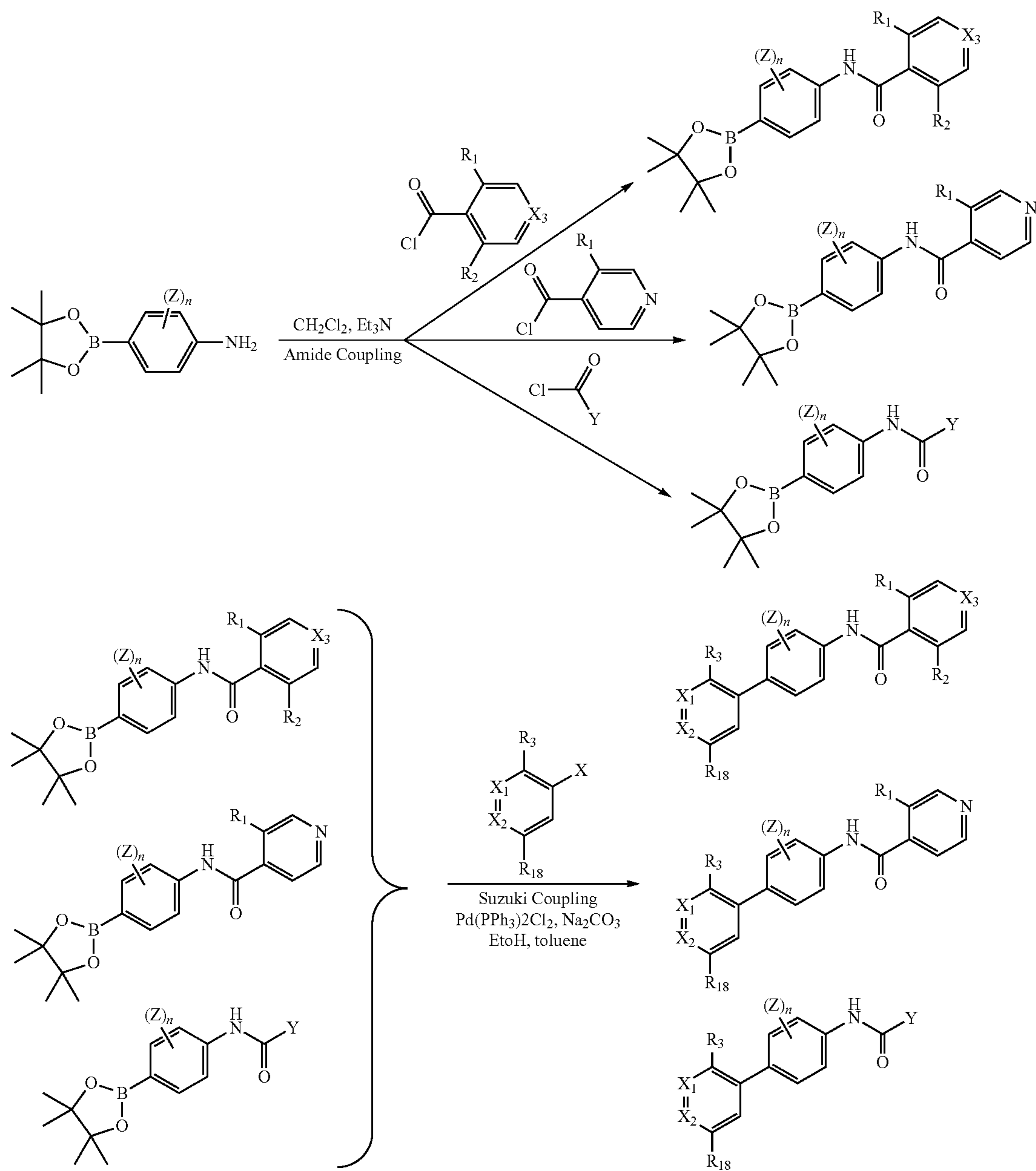
Scheme A
