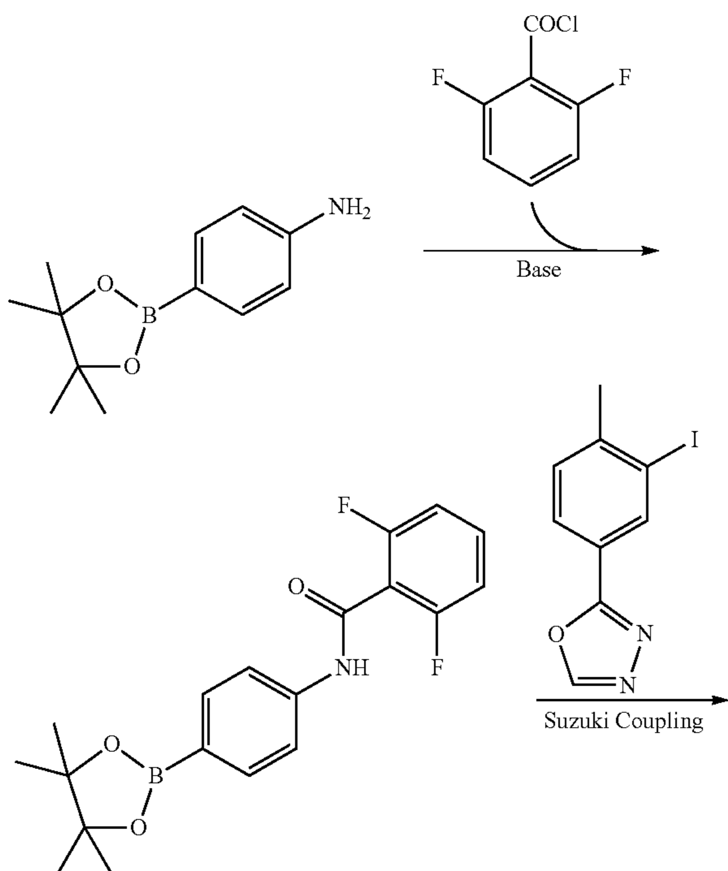
Scheme XX
