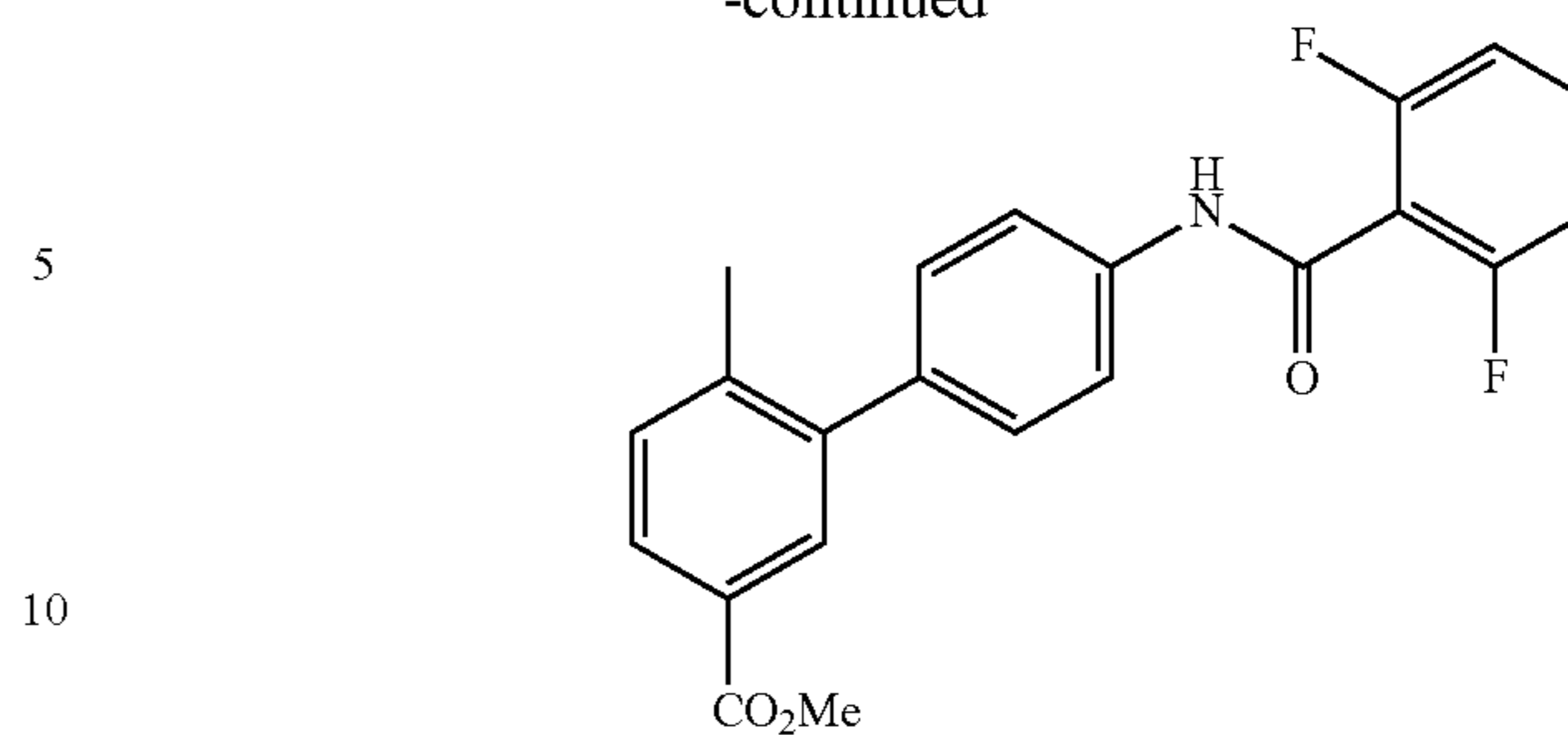
Compound 1
