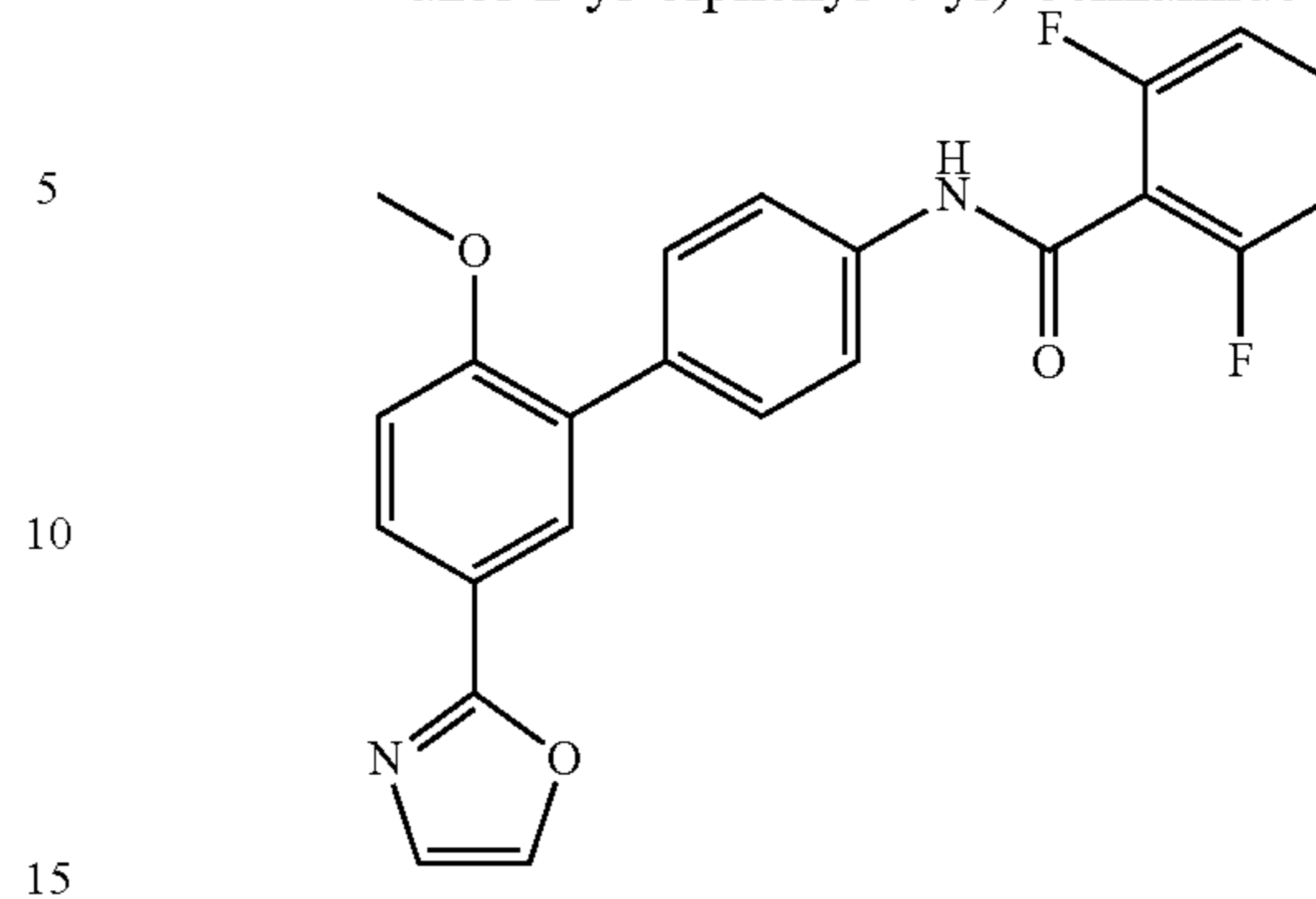
Compound 13: 2,6-Difluoro-N-(2'-methoxy-5'-oxazol-2-yl-biphenyl-4-yl)-benzamide
