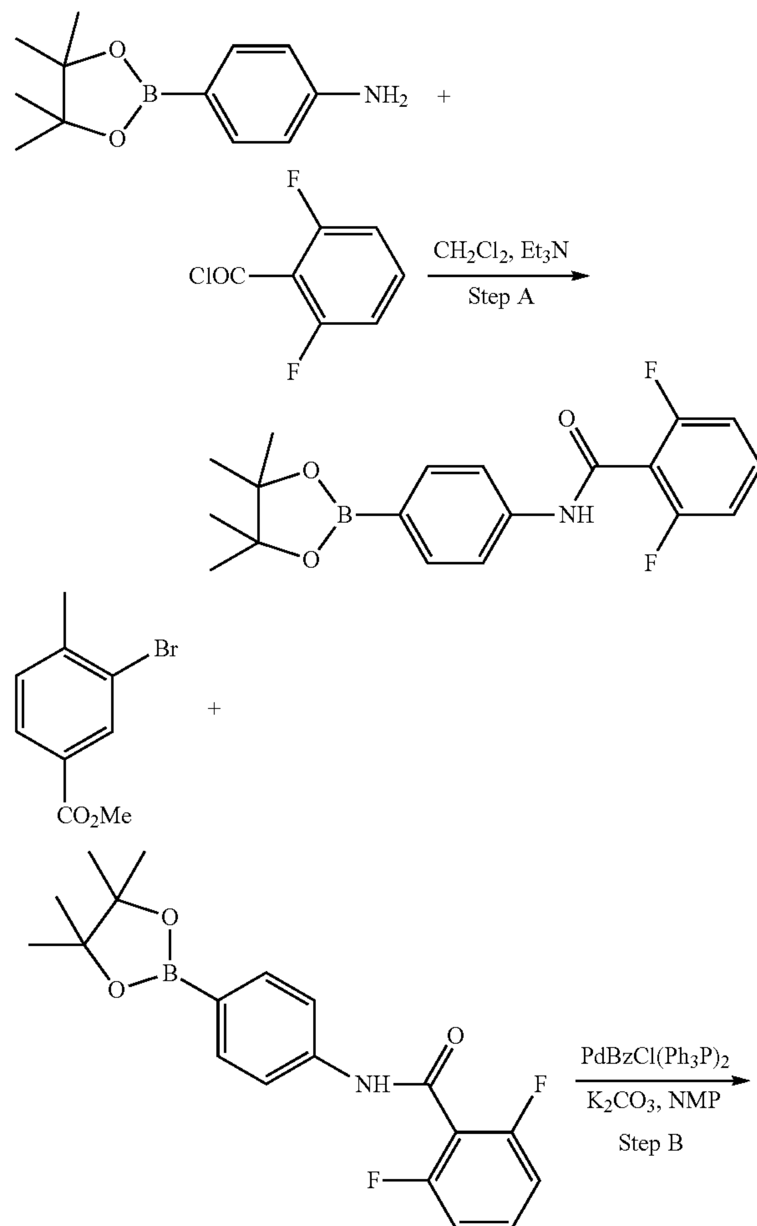
Scheme I
