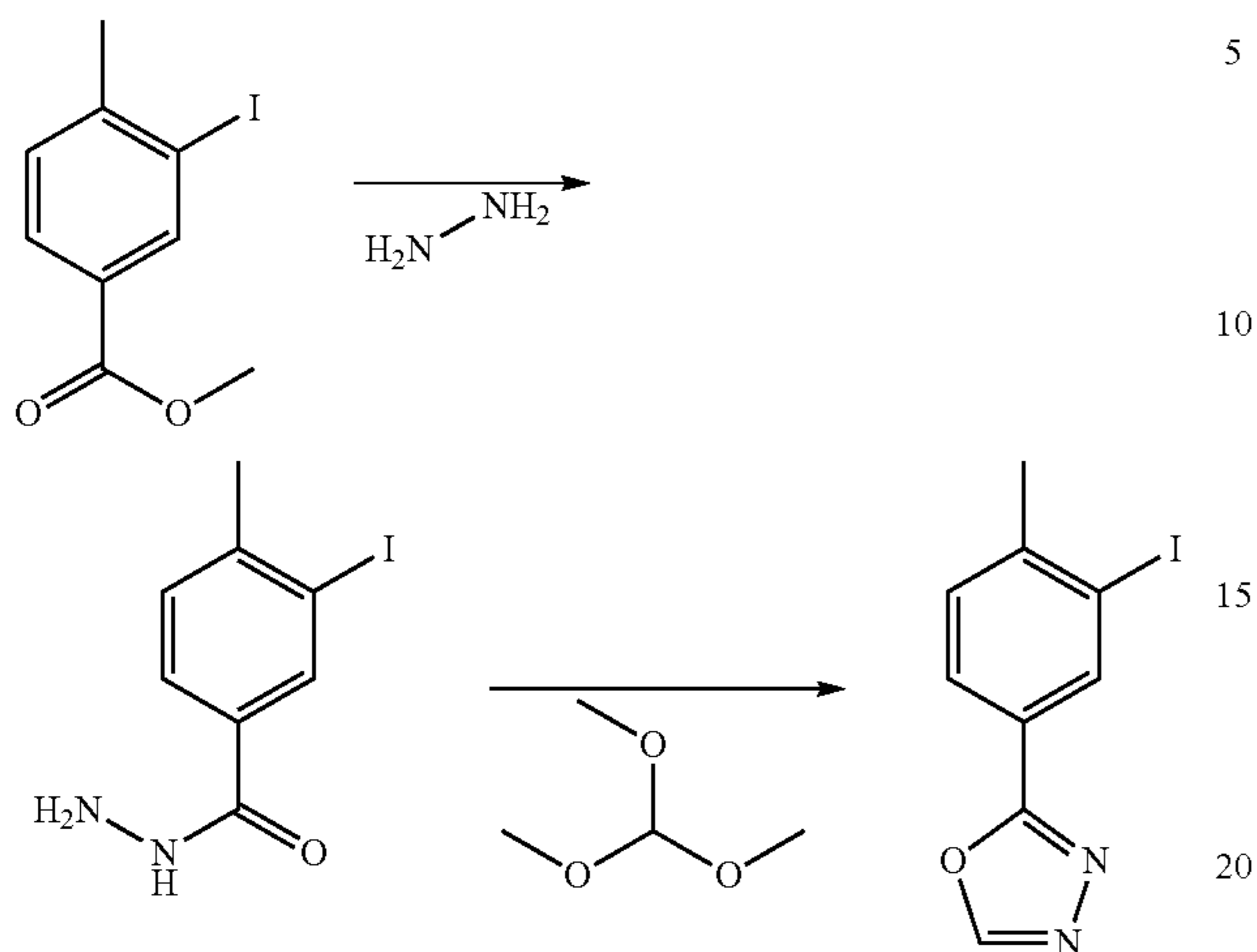
Scheme XIX
