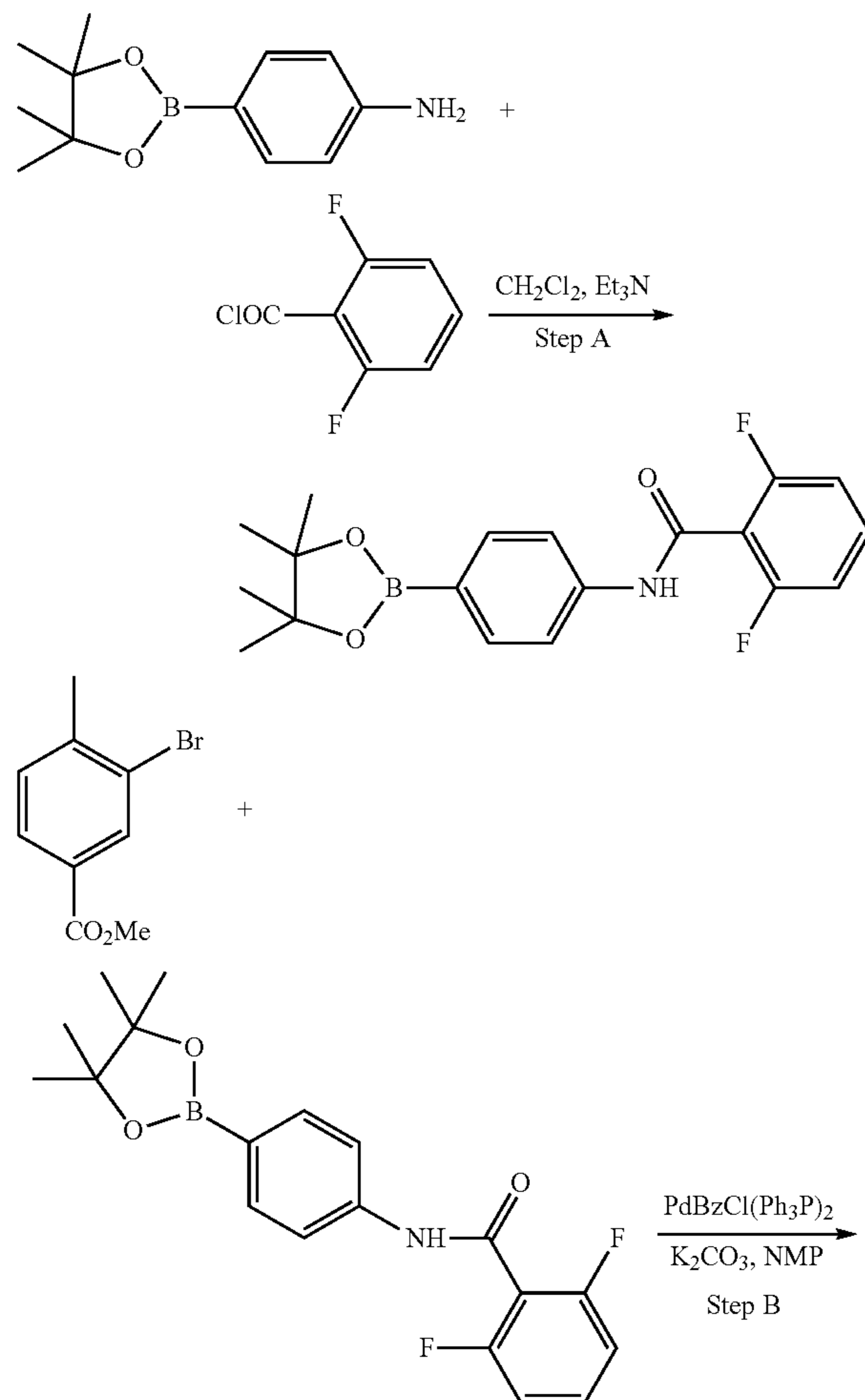
Scheme I
