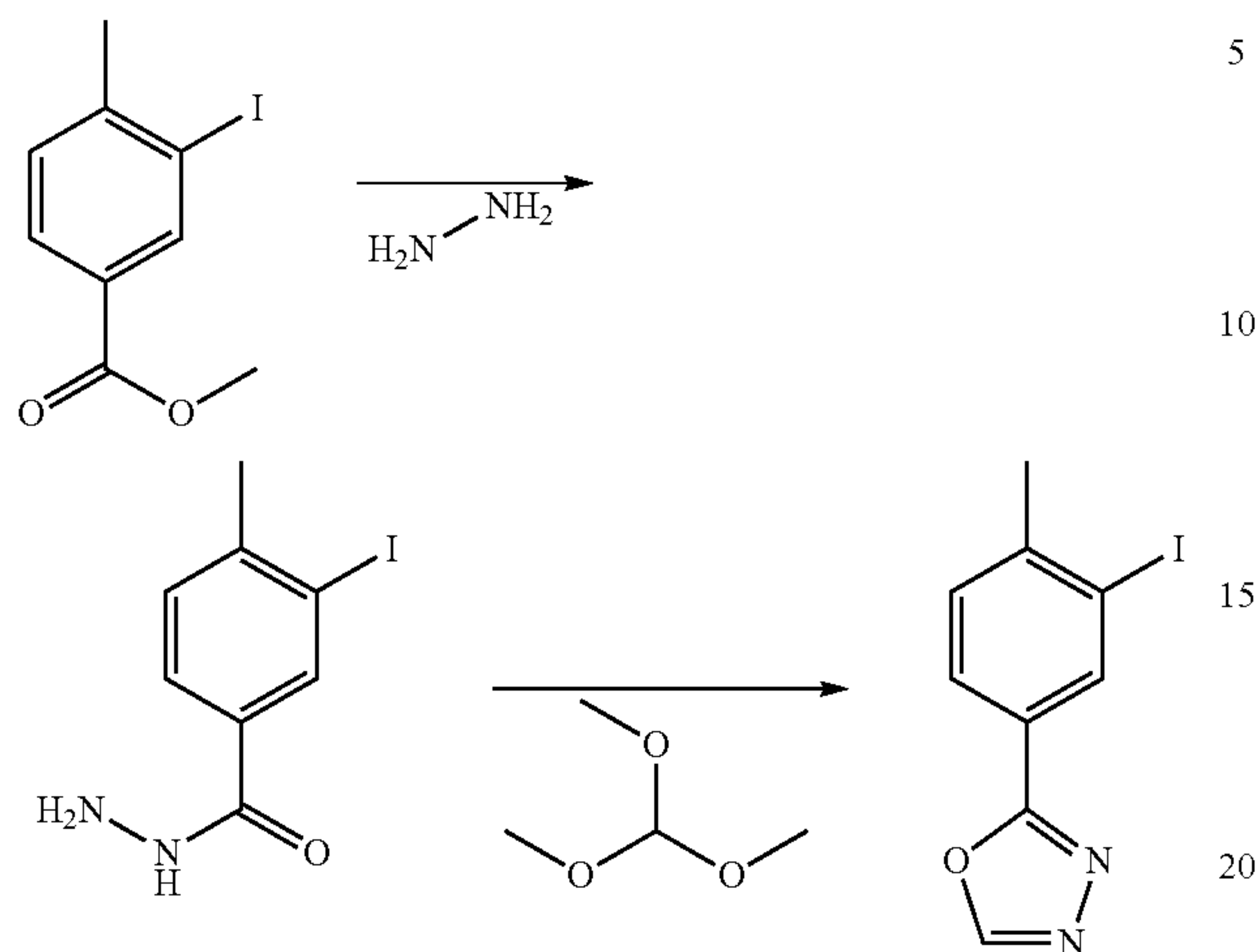
Scheme XIX
