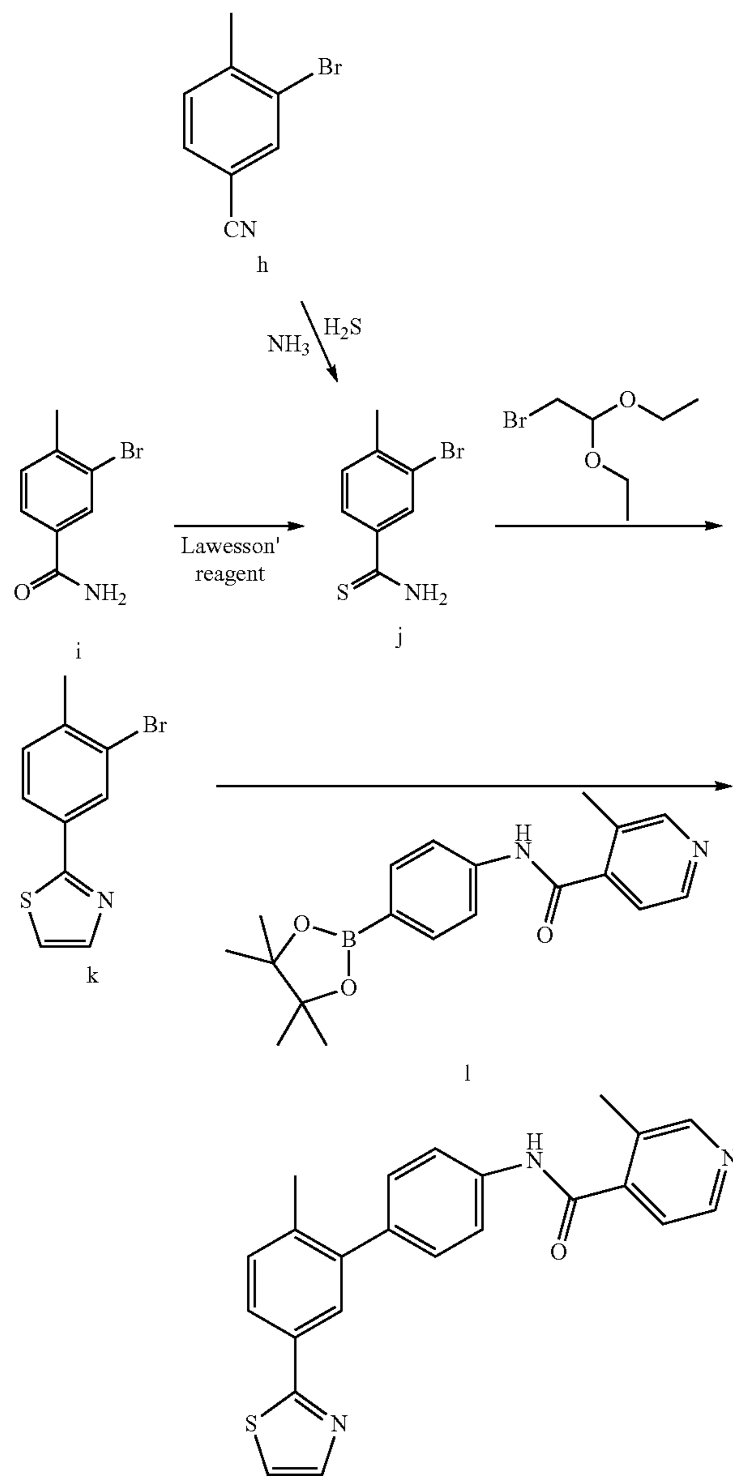
Compound 14
