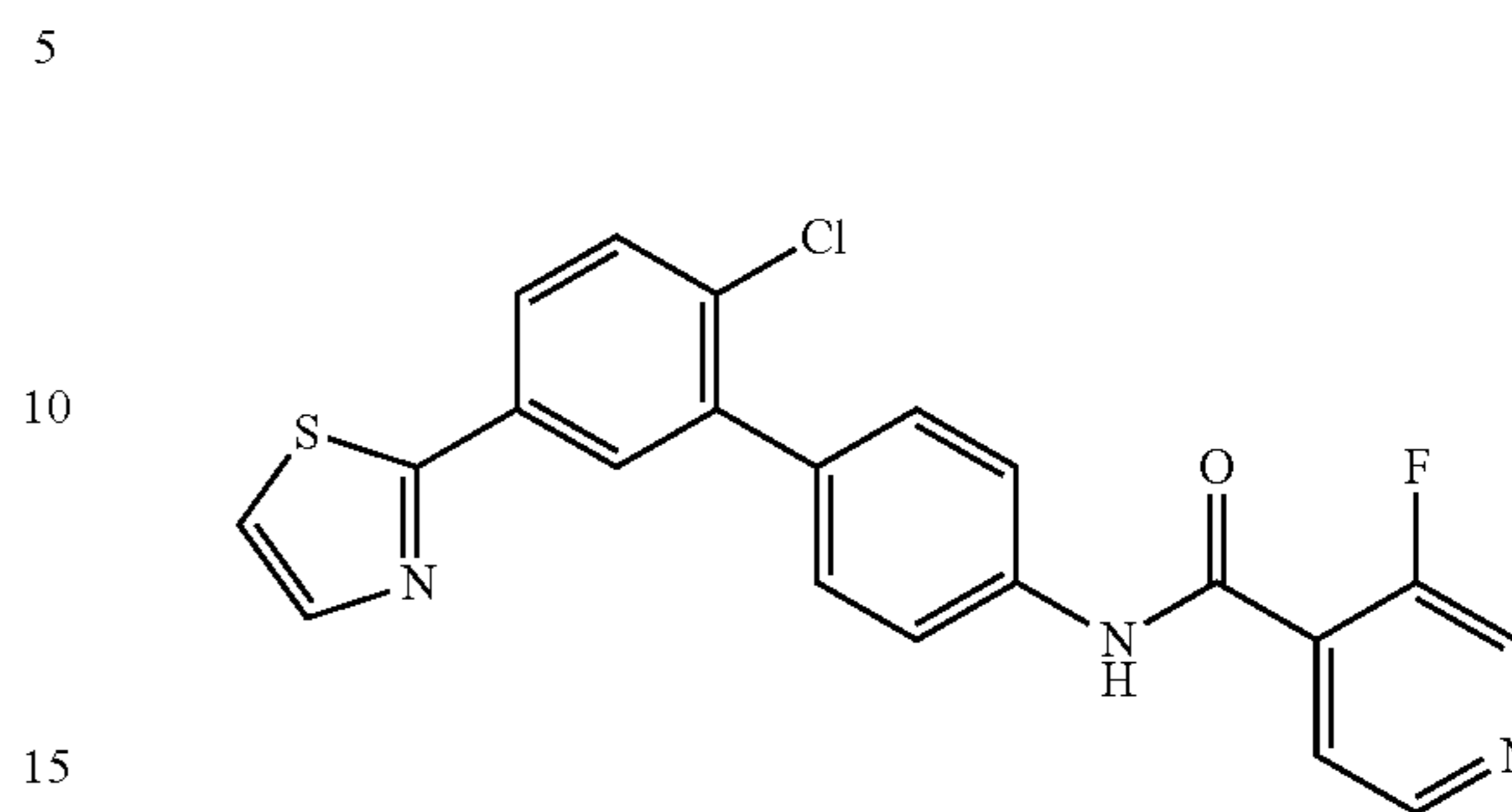
Compound 58: 3-Fluoro-N-[5'-(thiazol-2-yl)-2'-chloro-biphenyl-4-yl]-isonicotinamide
