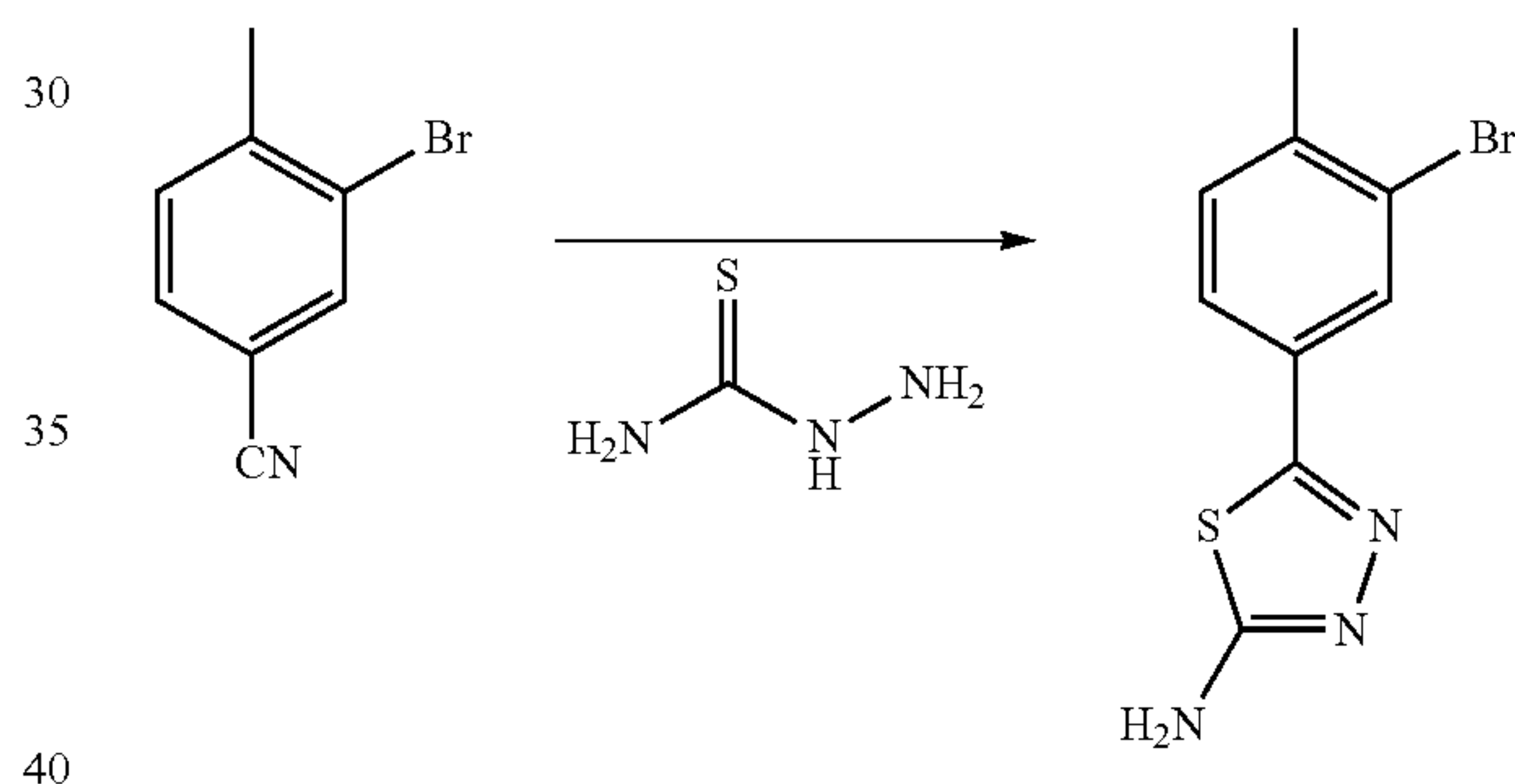
Scheme XXII
