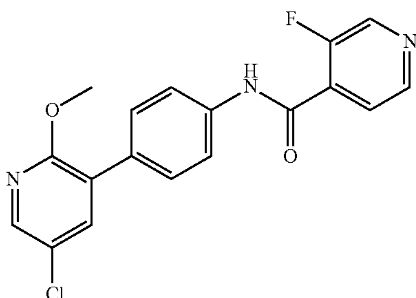
Compound 19: 3-Fluoro-N-[4-(5-chloro-2-methoxy-pyridin-3-yl)-phenyl]-isonicotinamide
