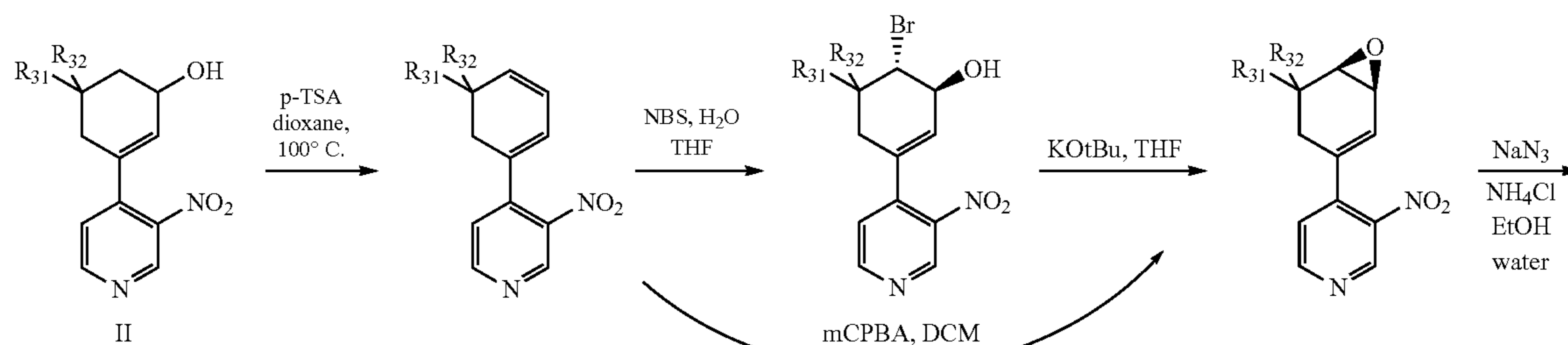
Scheme 2.
