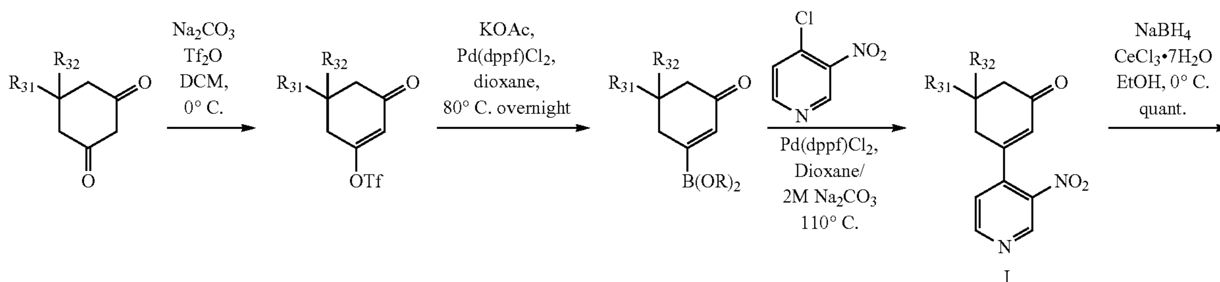
Scheme 1.
