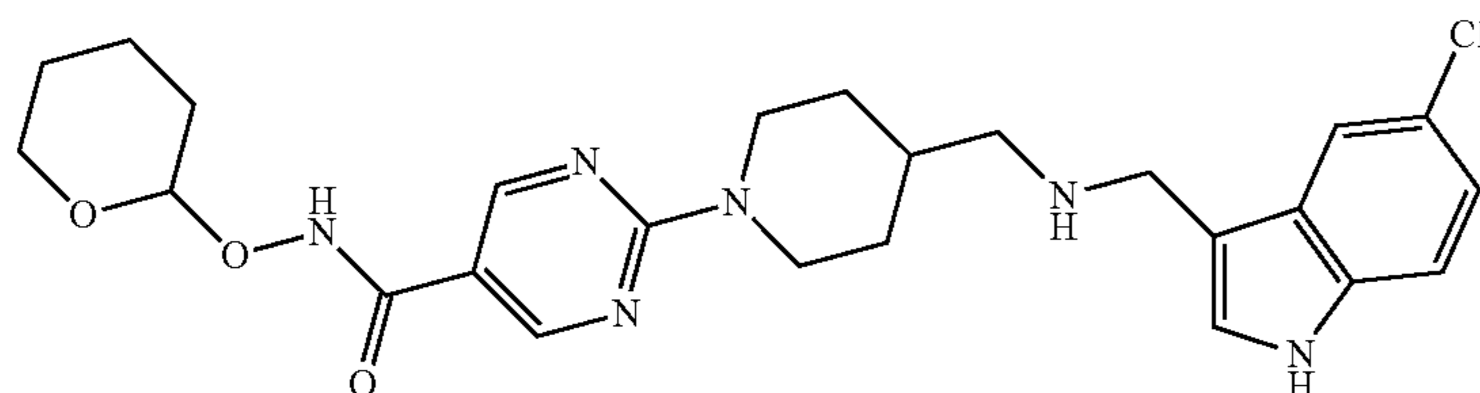
Interm. 7; Ex. [A2]
