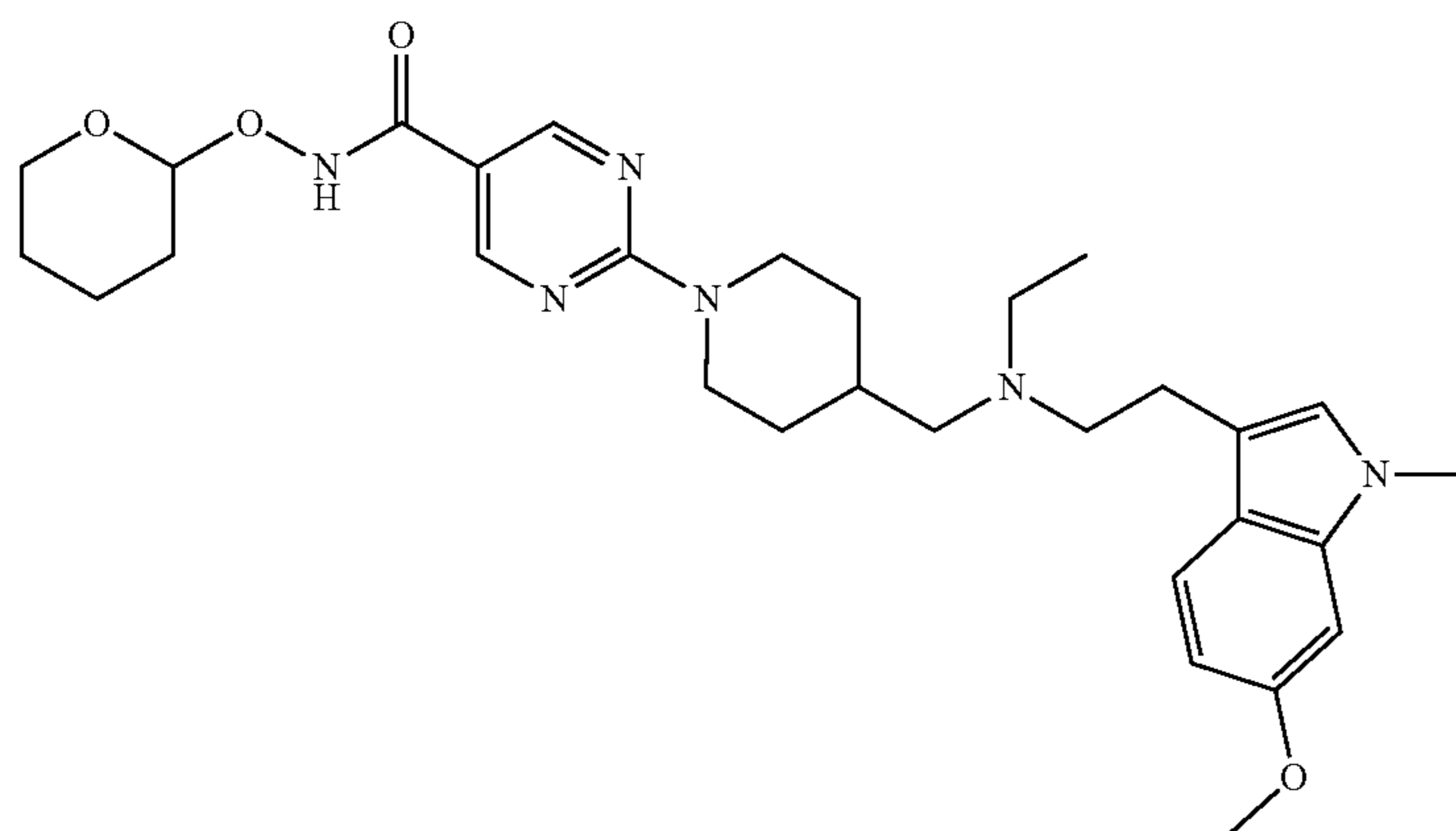
Interm. 169; Ex. [A12]; mp. 80° C.
