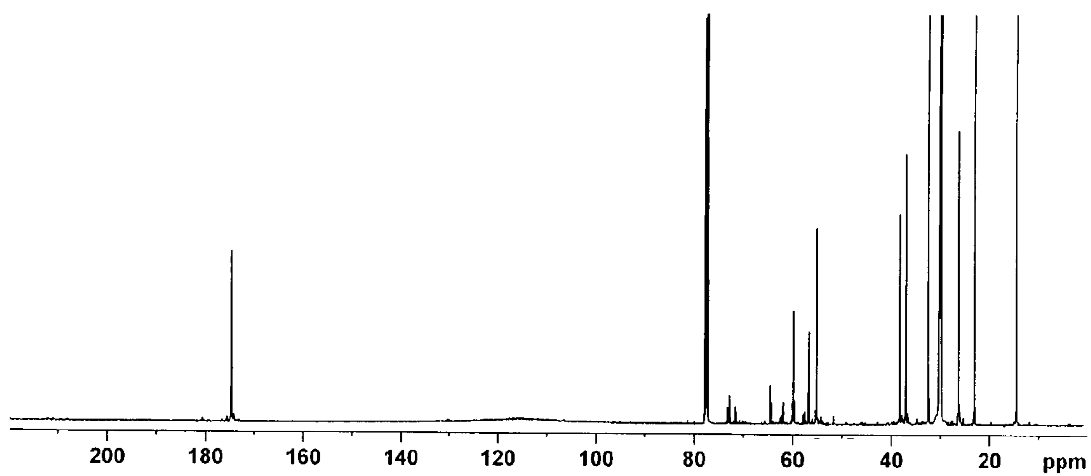
Figure 4b. ^{13}\text{C} NMR spectrum of Varisoft 510
