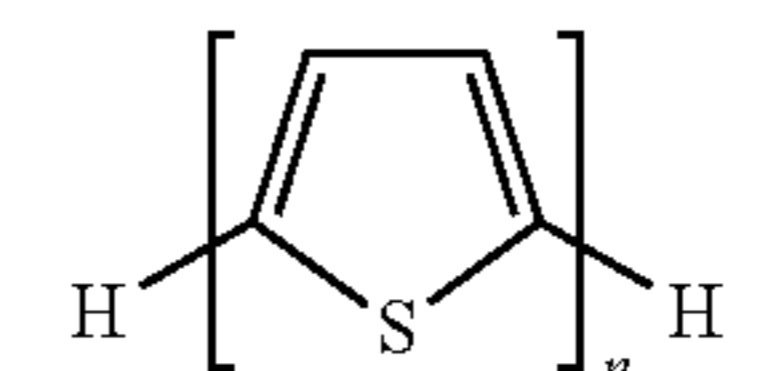
oligothiophenes
