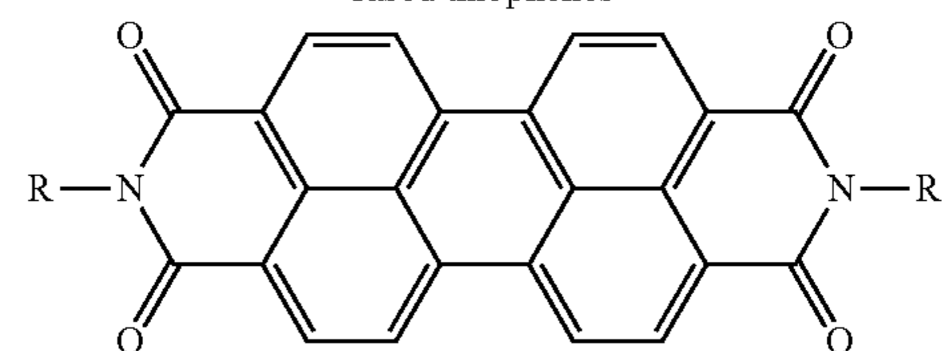
perylene bisimides
