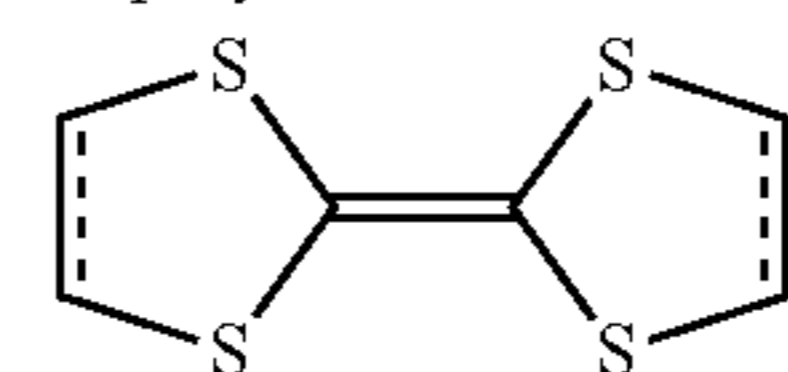
tetrathiofulvalenes
