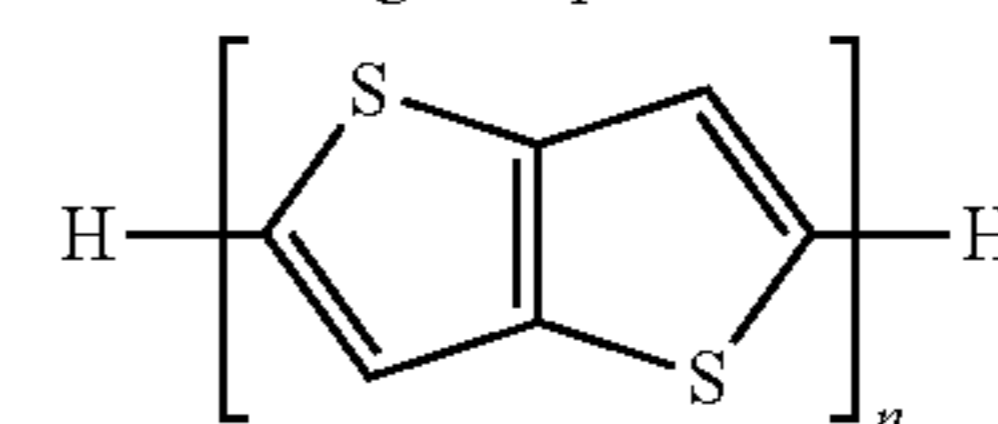
oligothiophenes
