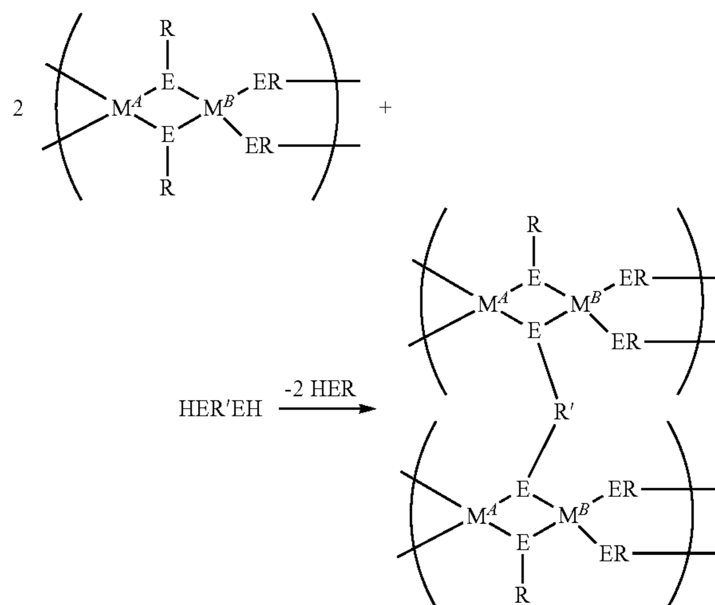
REACTION SCHEME 14
