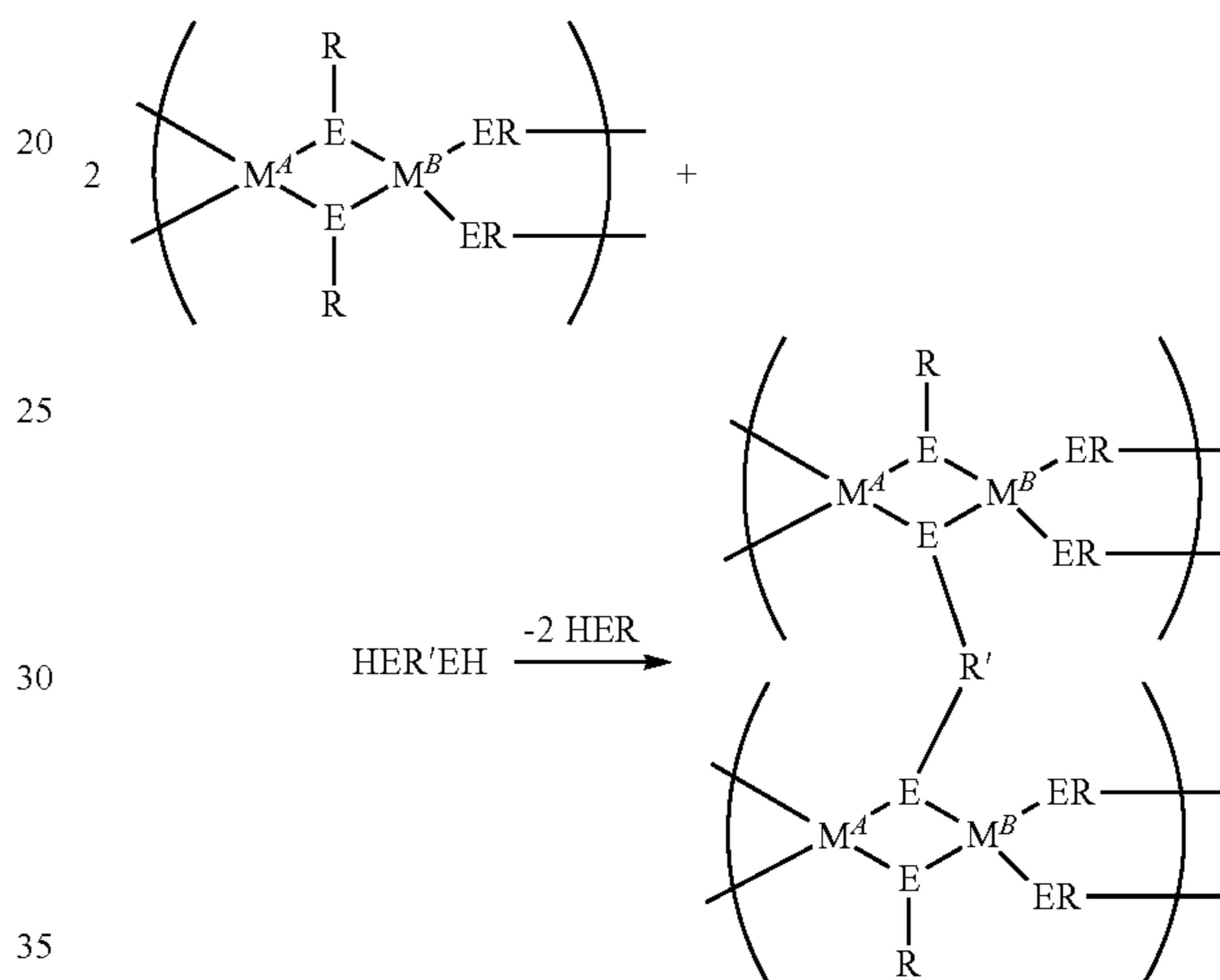
REACTION SCHEME 14
