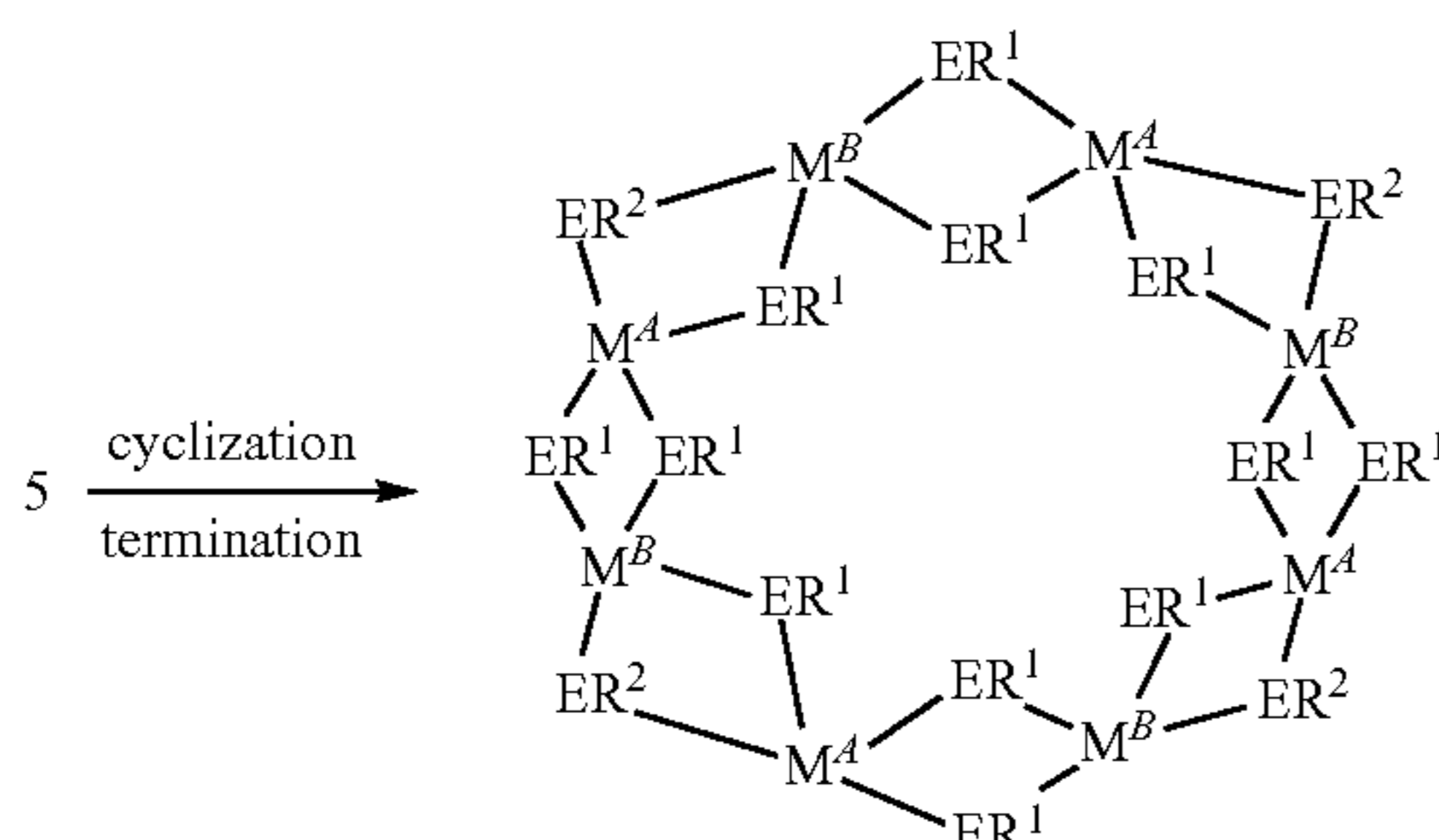
REACTION SCHEME 7:
