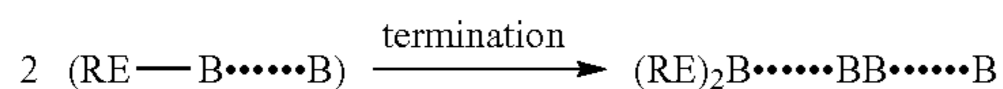
REACTION SCHEME 6:
