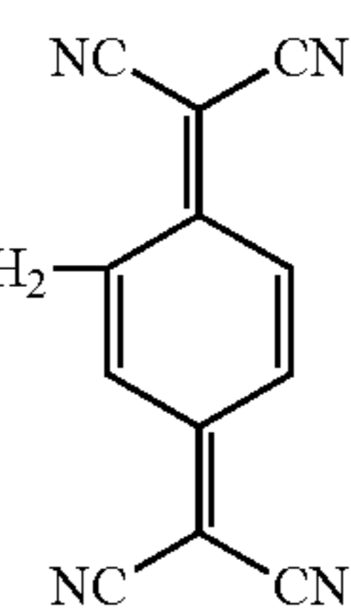
Dye 14
