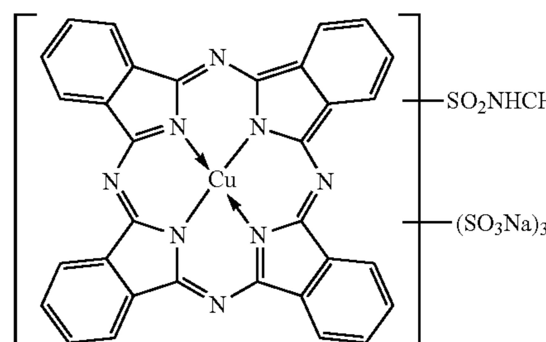
Dye 13
