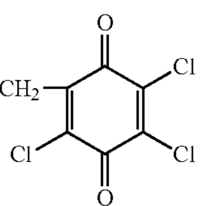
Dye 13
