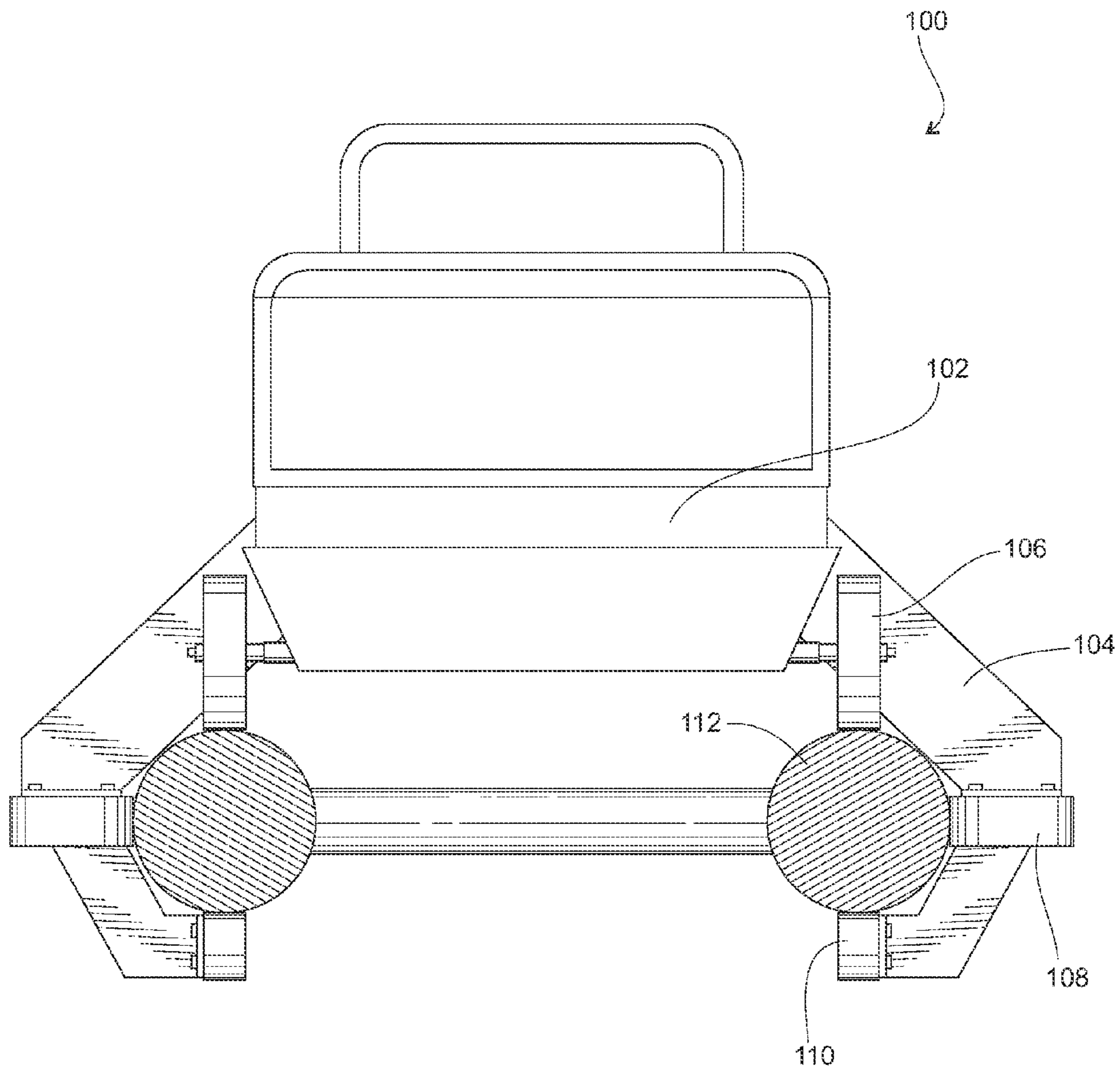
Fig. 1 PRIOR ART
