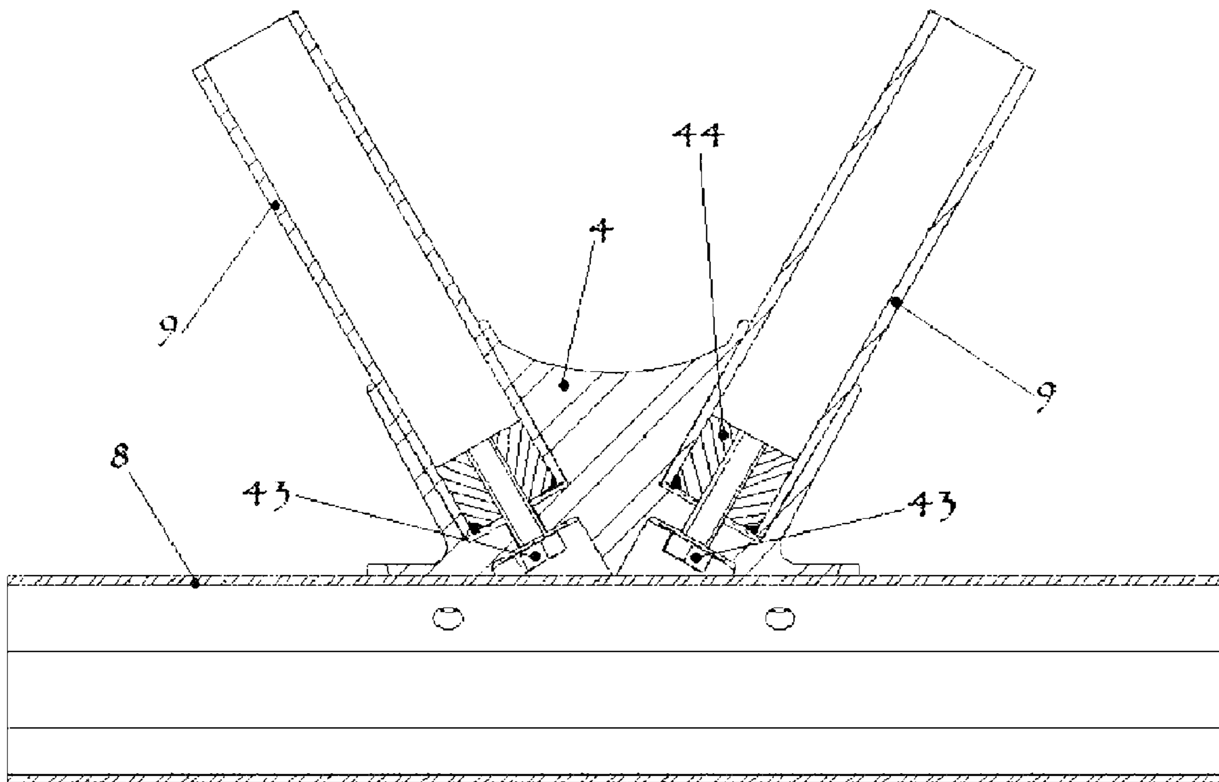
SECTION F-F
