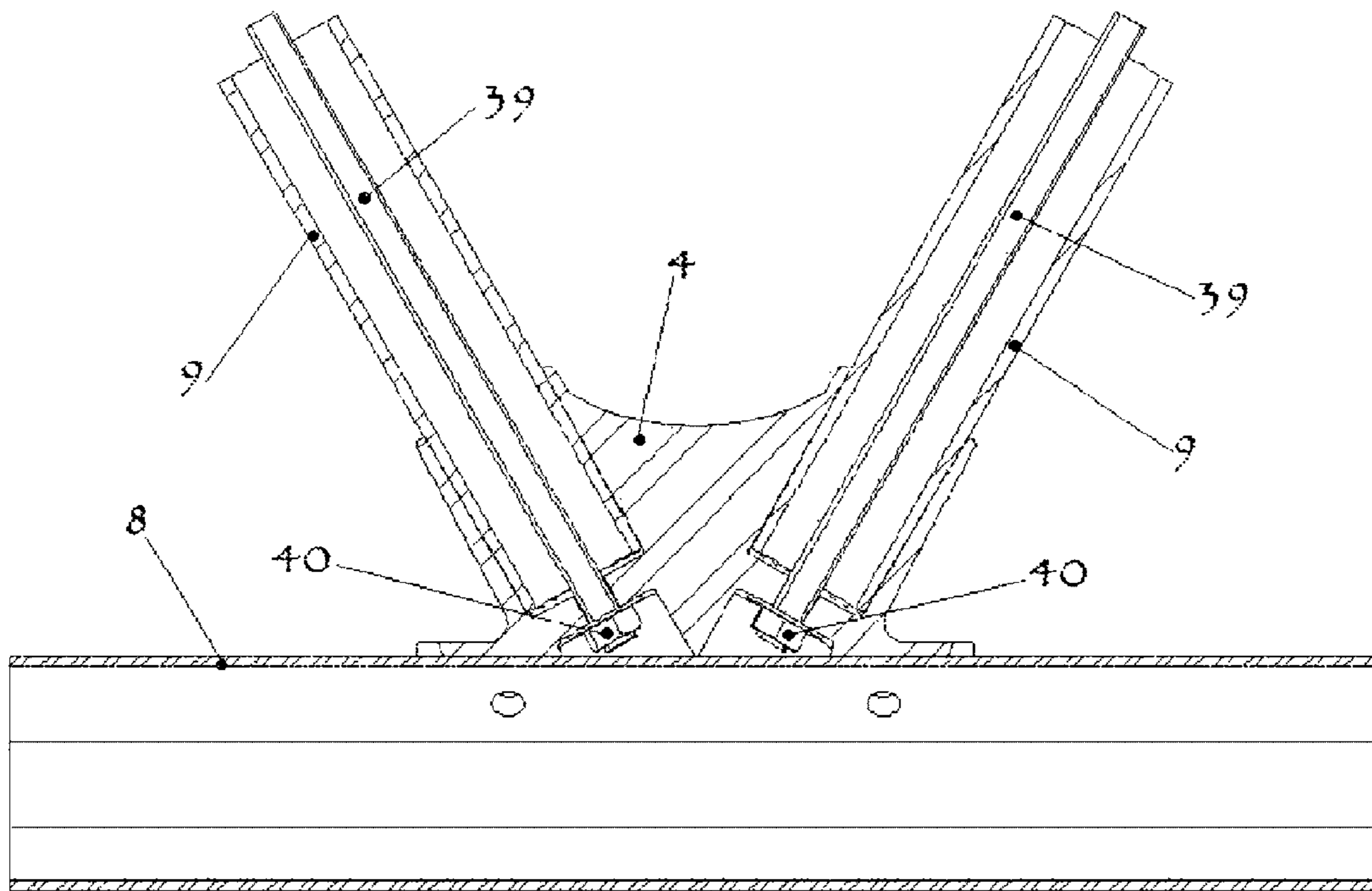
SECTION E-E
