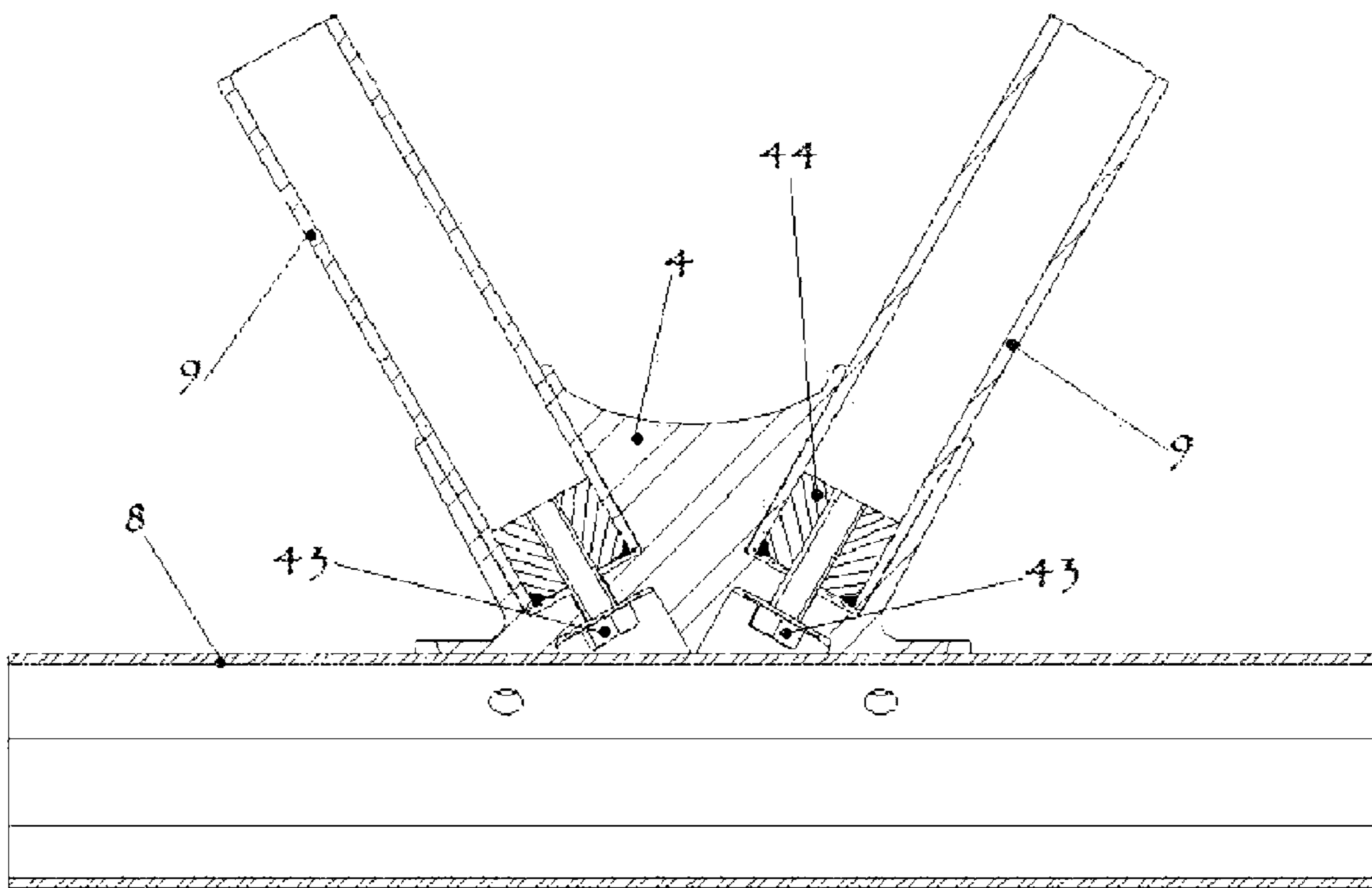
SECTION F-F
