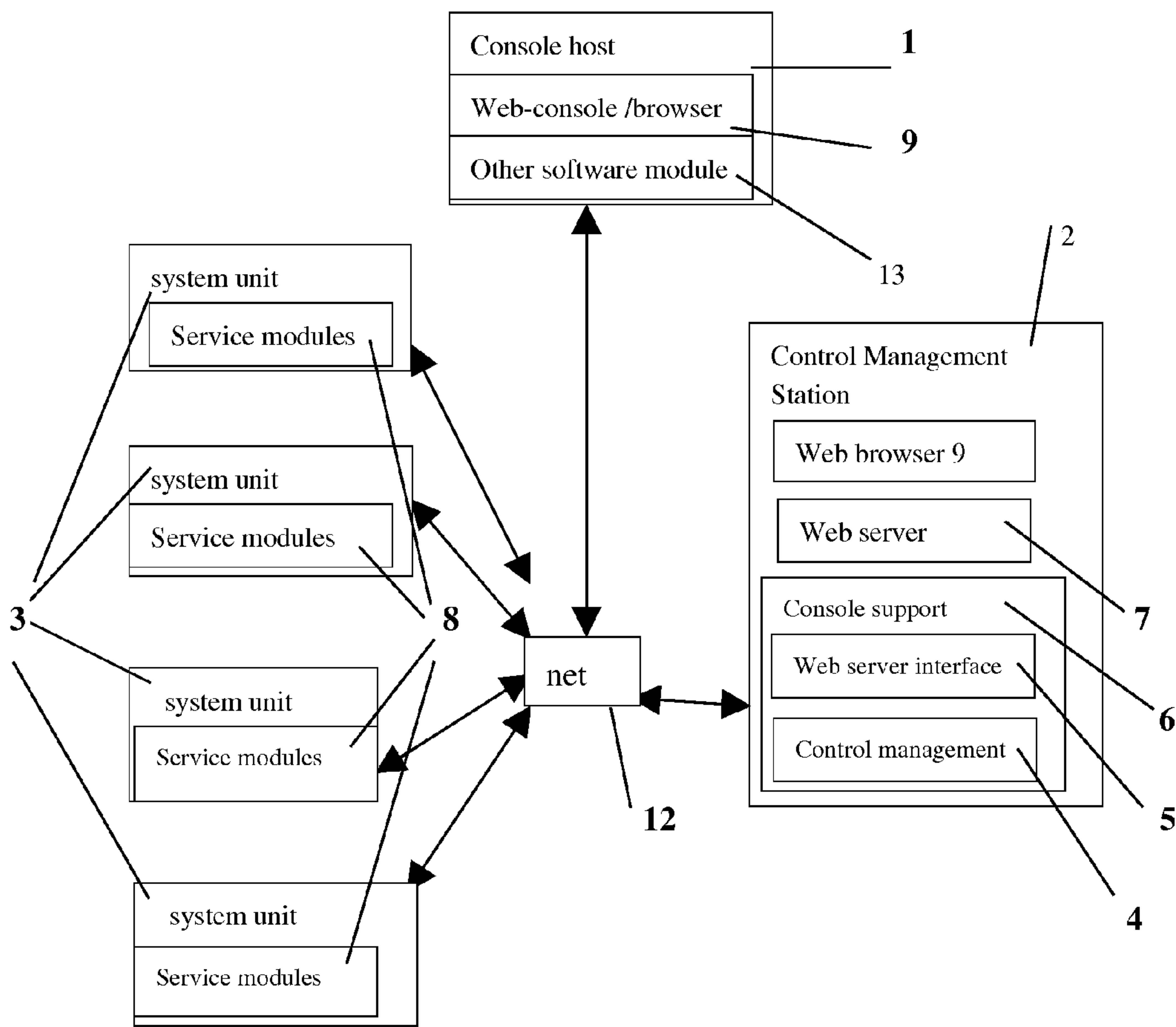
Fig. 3) The Software of WCUWE for typical CCDSVM:
