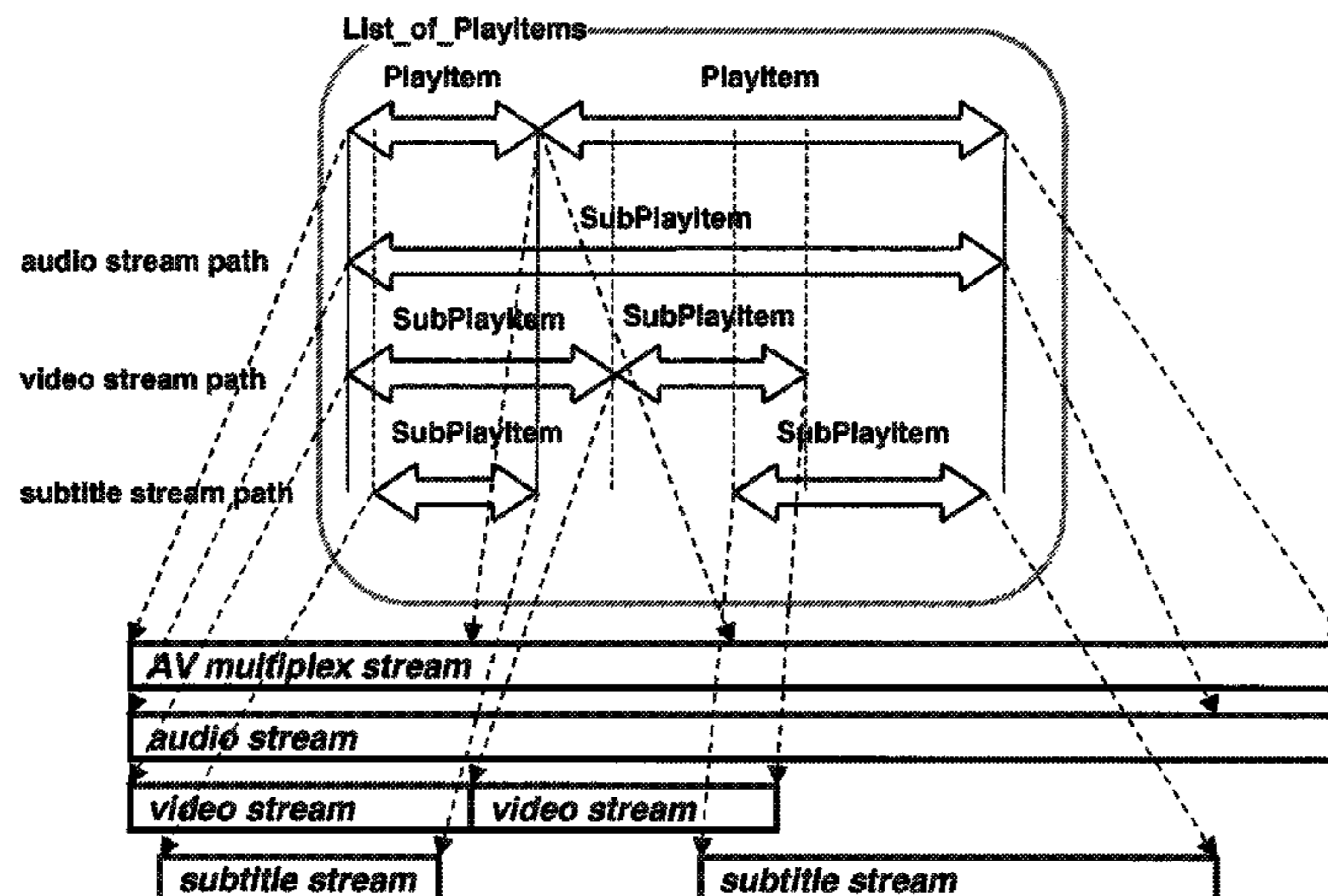
List_of_PlayItems Example
