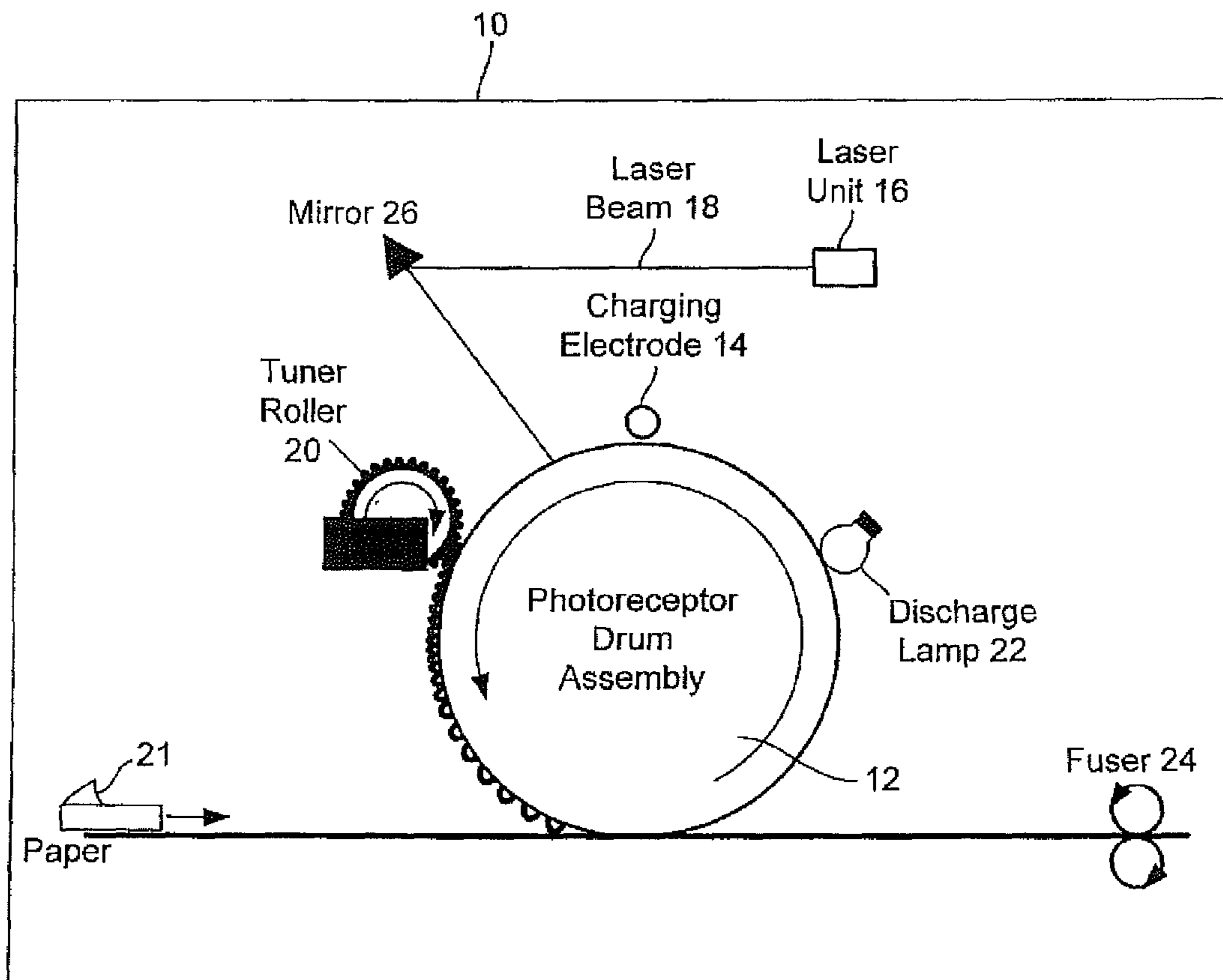
FIG. 1 (Background Art)
