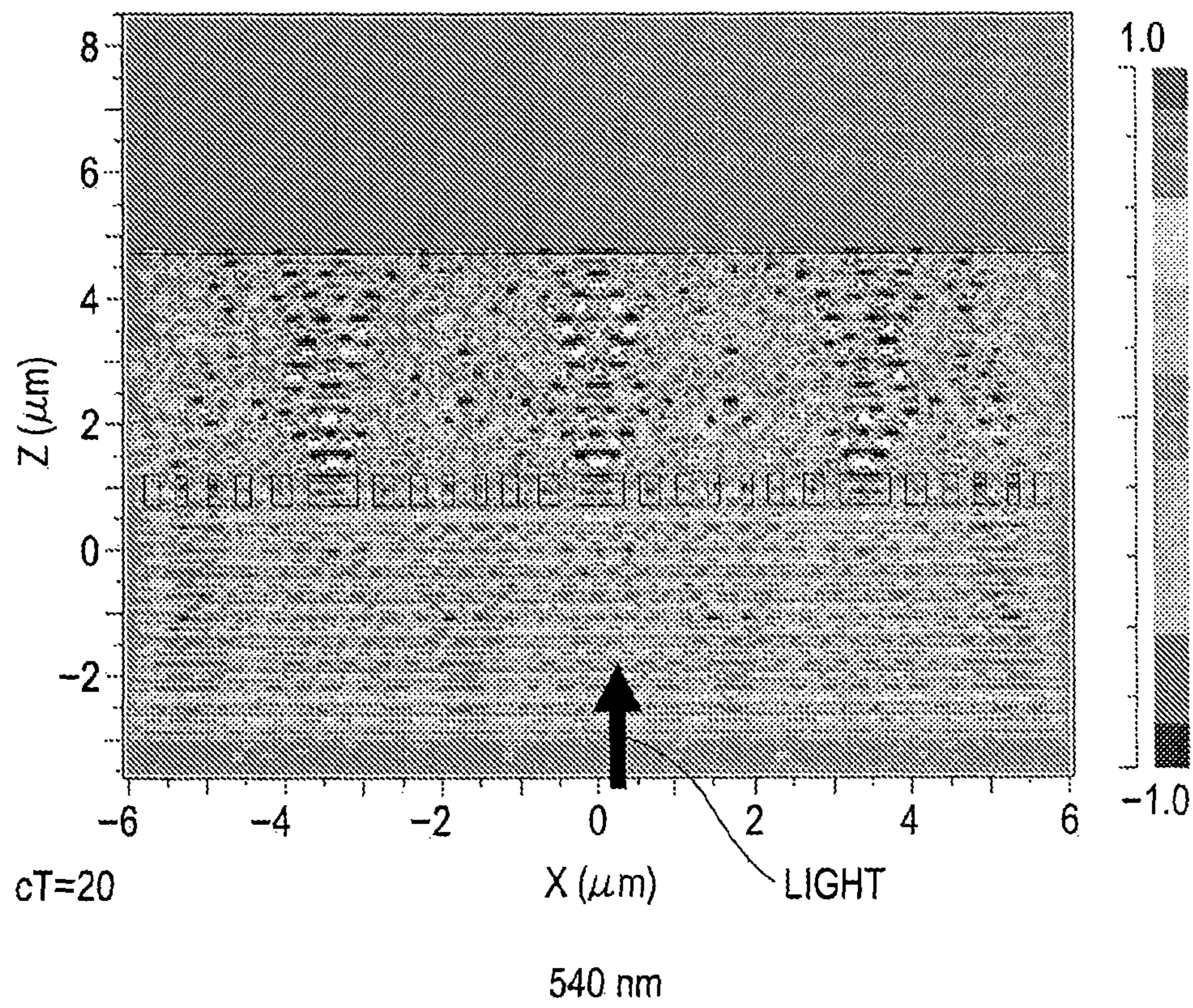
CONTOUR MAP OF E_y
