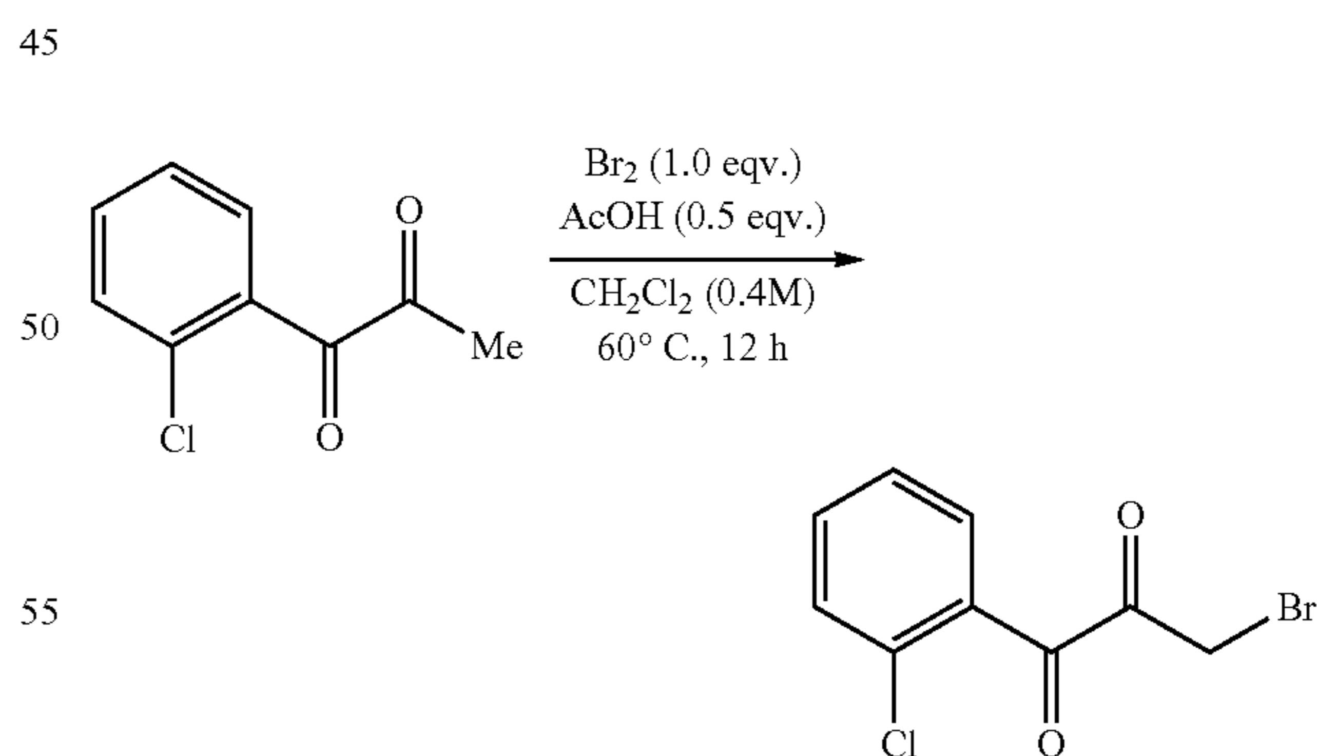
3-Bromo-1-(2-chlorophenyl)propane-1,2-dione
