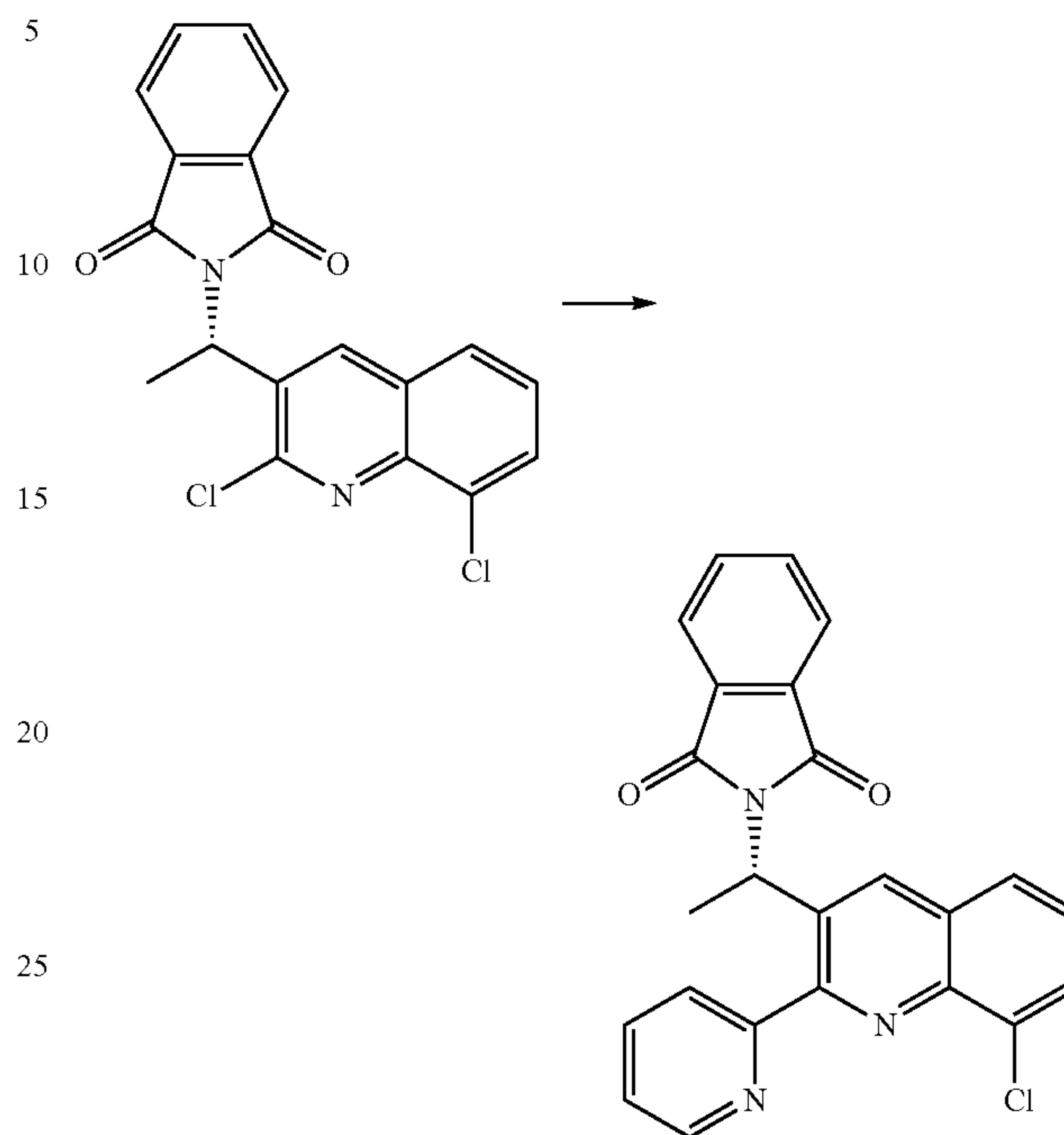
2((S)-1-(8-Chloro-2-(pyridin-2-yl)quinolin-3-yl)ethyl)isoindoline-1,3-dione
