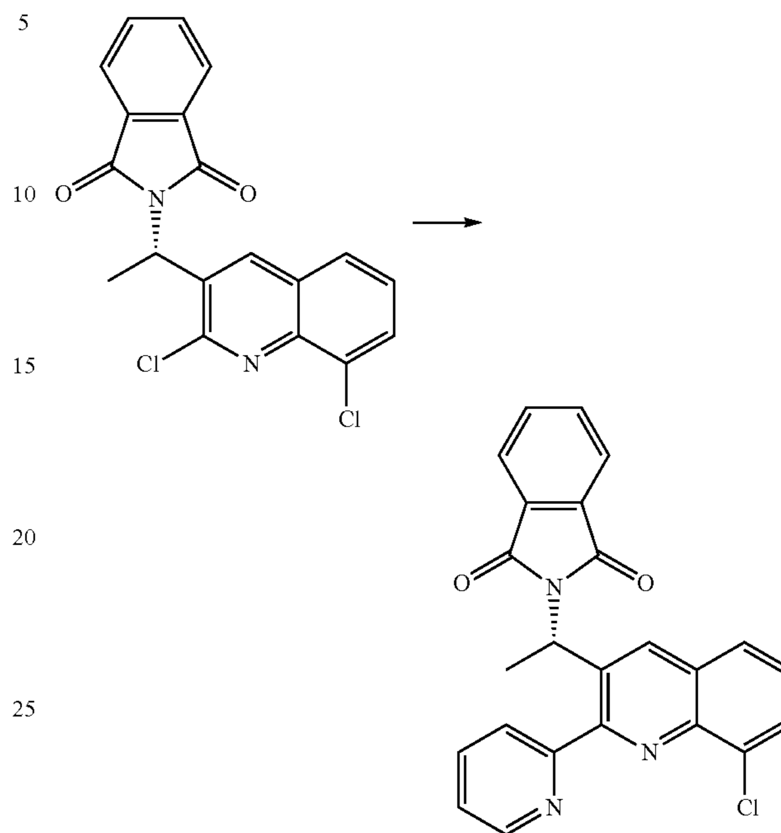
2((S)-1-(8-Chloro-2-(pyridin-2-yl)quinolin-3-yl)ethyl)isoindoline-1,3-dione
