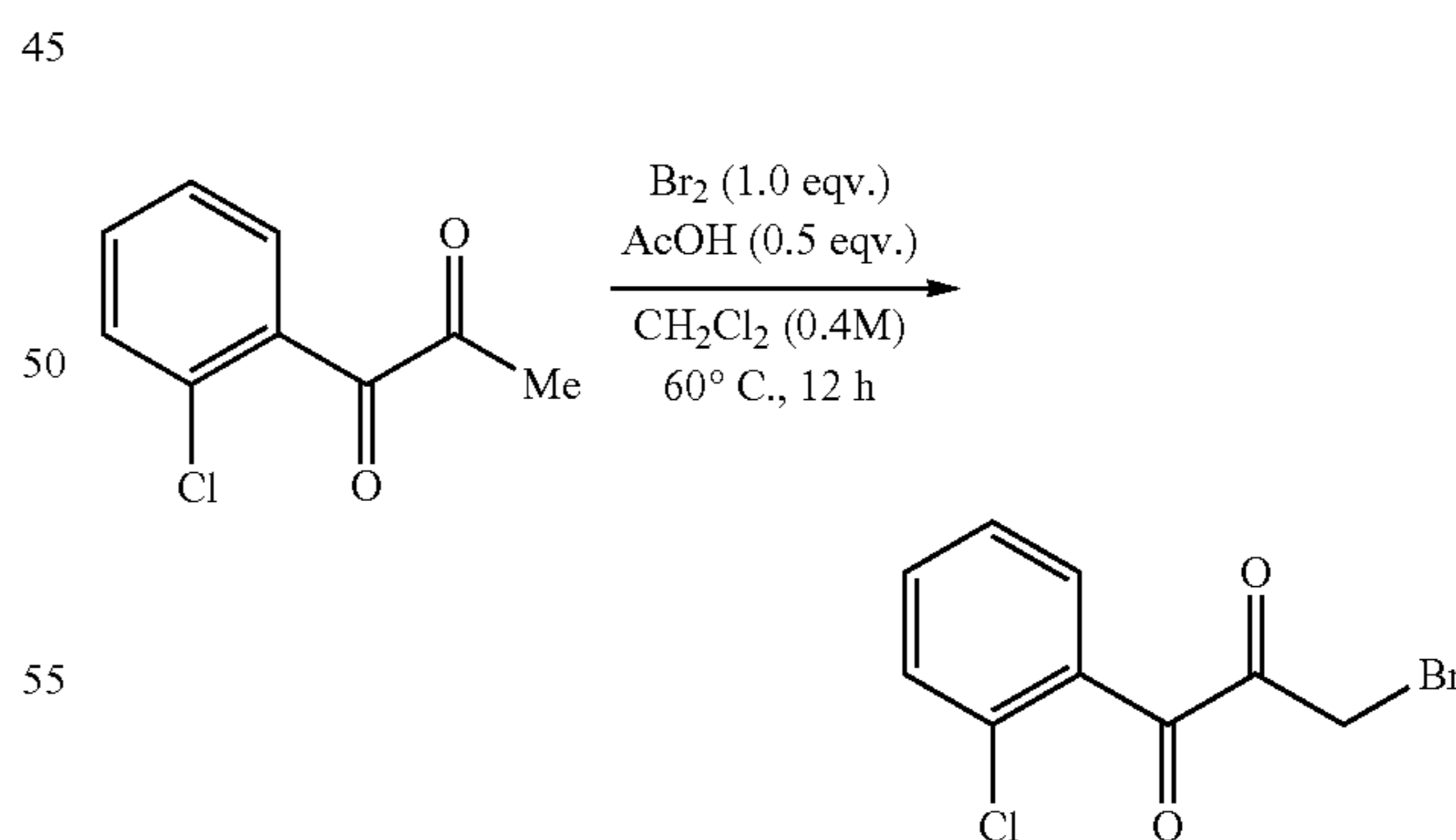
3-Bromo-1-(2-chlorophenyl)propane-1,2-dione
