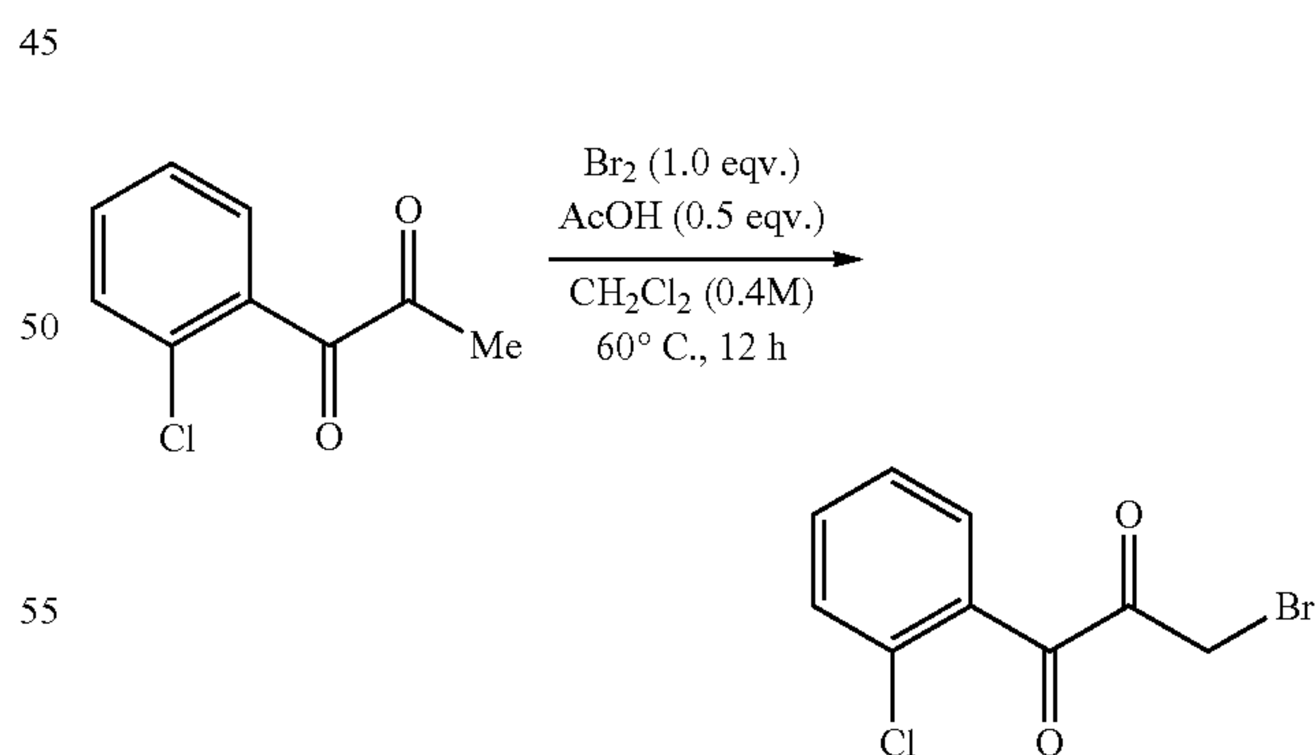
3-Bromo-1-(2-chlorophenyl)propane-1,2-dione
