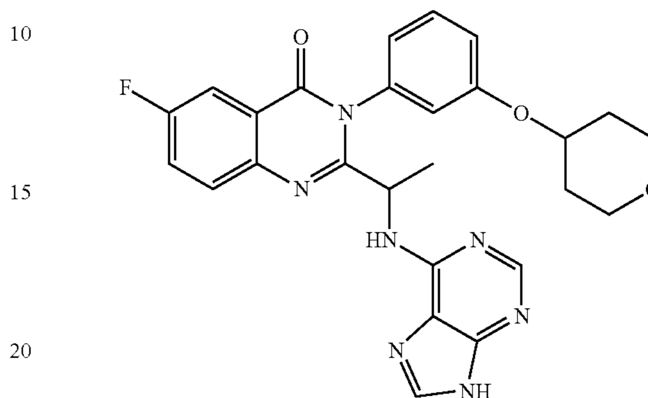
6-Fluoro-2-[1-(9H-purin-6-ylamino)-ethyl]-3-[3-(tetrahydro-pyran-4-yloxy)-phenyl]-3H-quinazolin-4-one (148)
