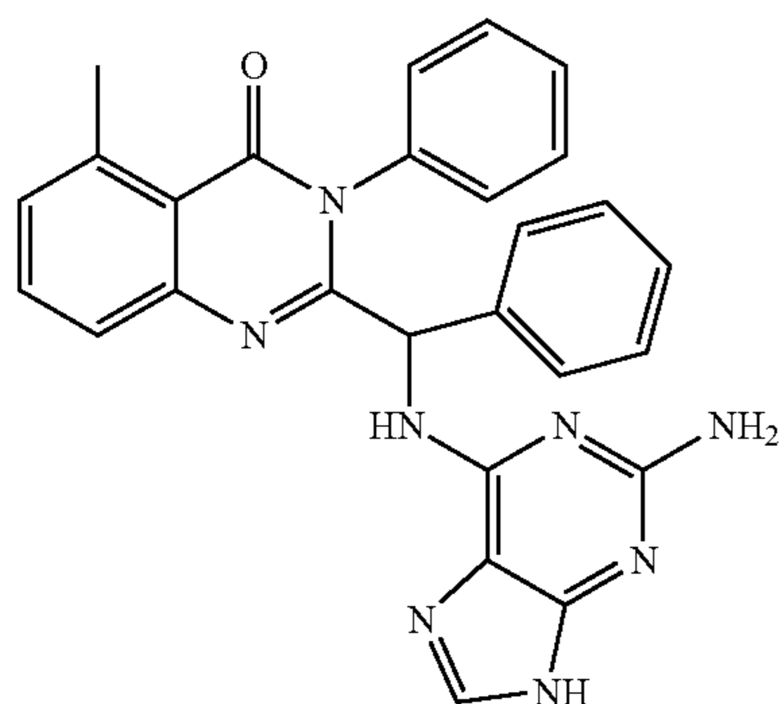
2-[(2-fluoro-9H-purin-6-ylamino)-phenyl-methyl]-5-methyl-3-phenyl-3H-quinazolin-4-one (44)
