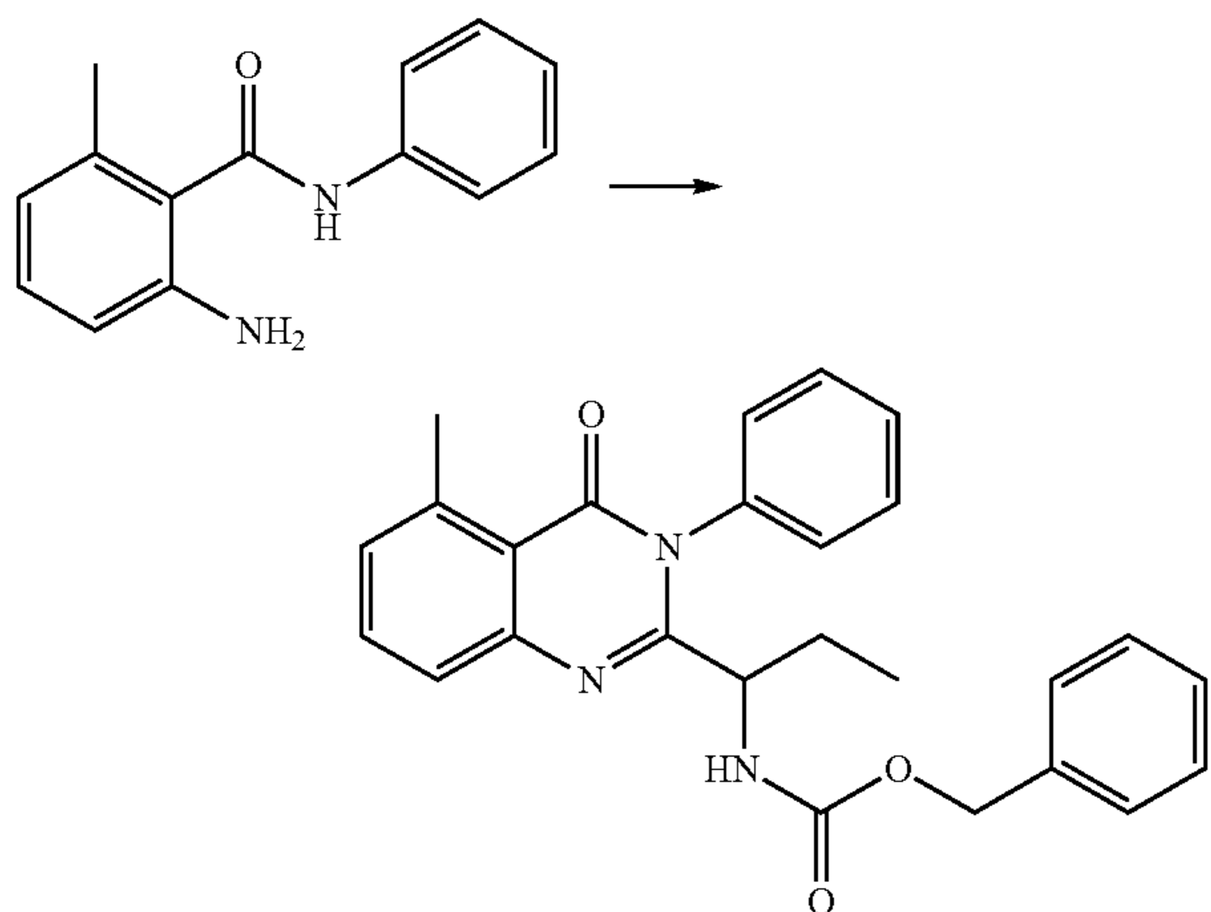
2-(1-amino-propyl)-5-methyl-3-phenyl-3H-quinazolin-4-one (17)
