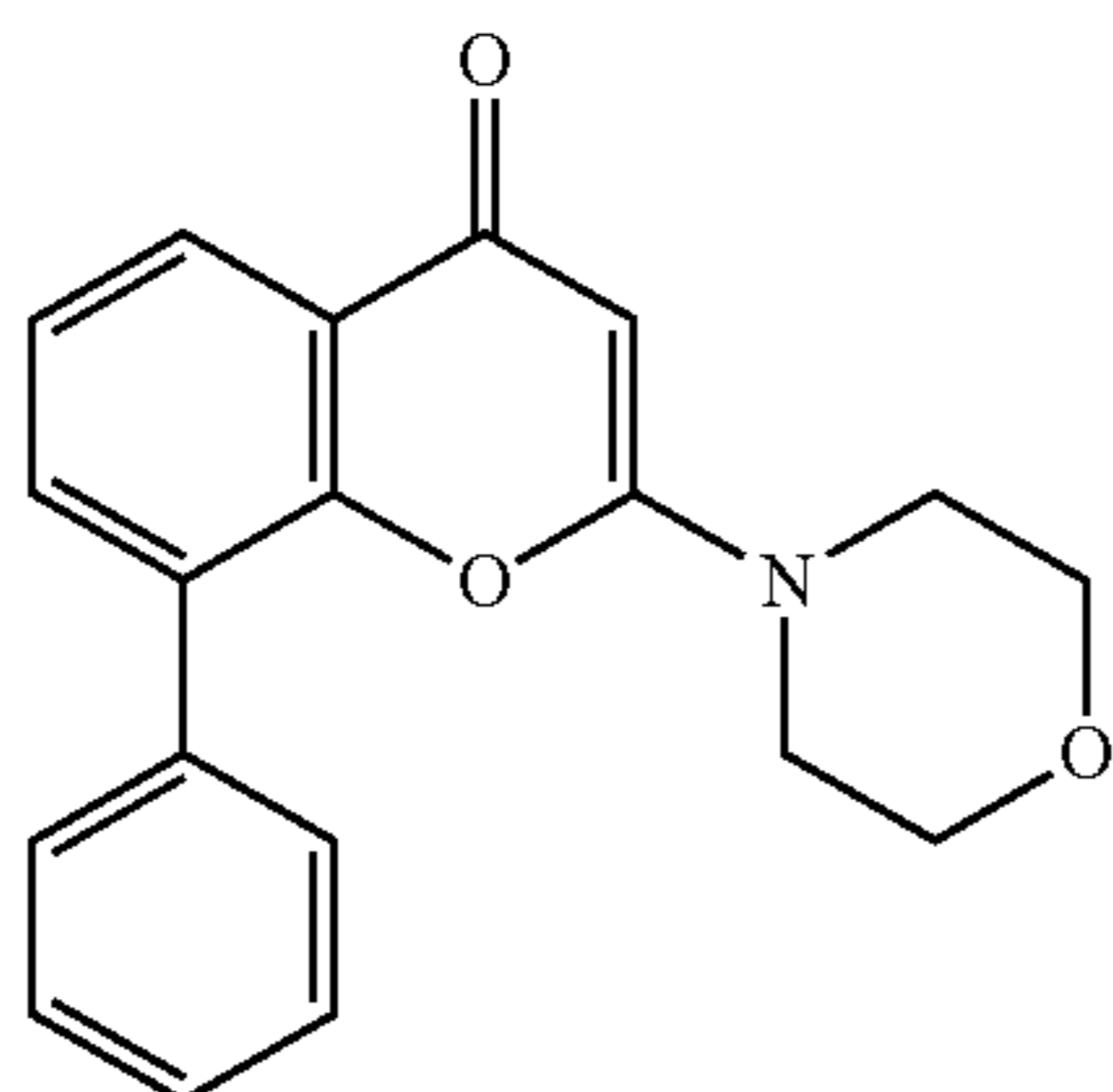
LY294002
