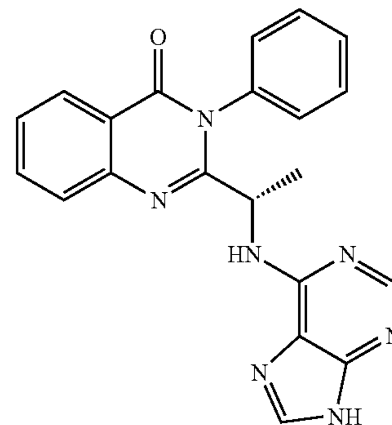
(S)-6-fluoro-3-phenyl-2-[(1-(9H-purin-6-ylamino)-ethyl)]-3H-quinazolin-4-one (113)
