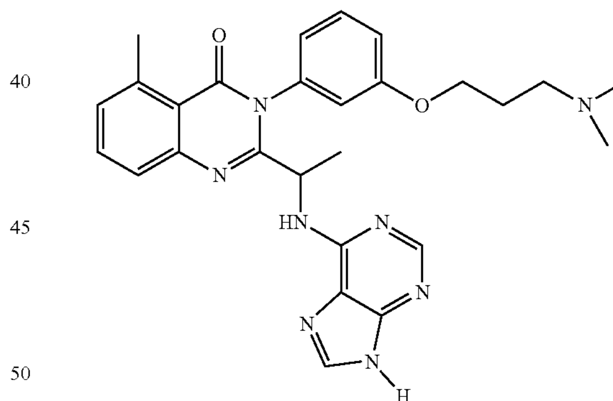
3-[3-(3-Dimethylamino-propoxy)-phenyl]-5-methyl-2-[1-(9H-purin-6-ylamino)-ethyl]-3H-quinazolin-4-one (150)
