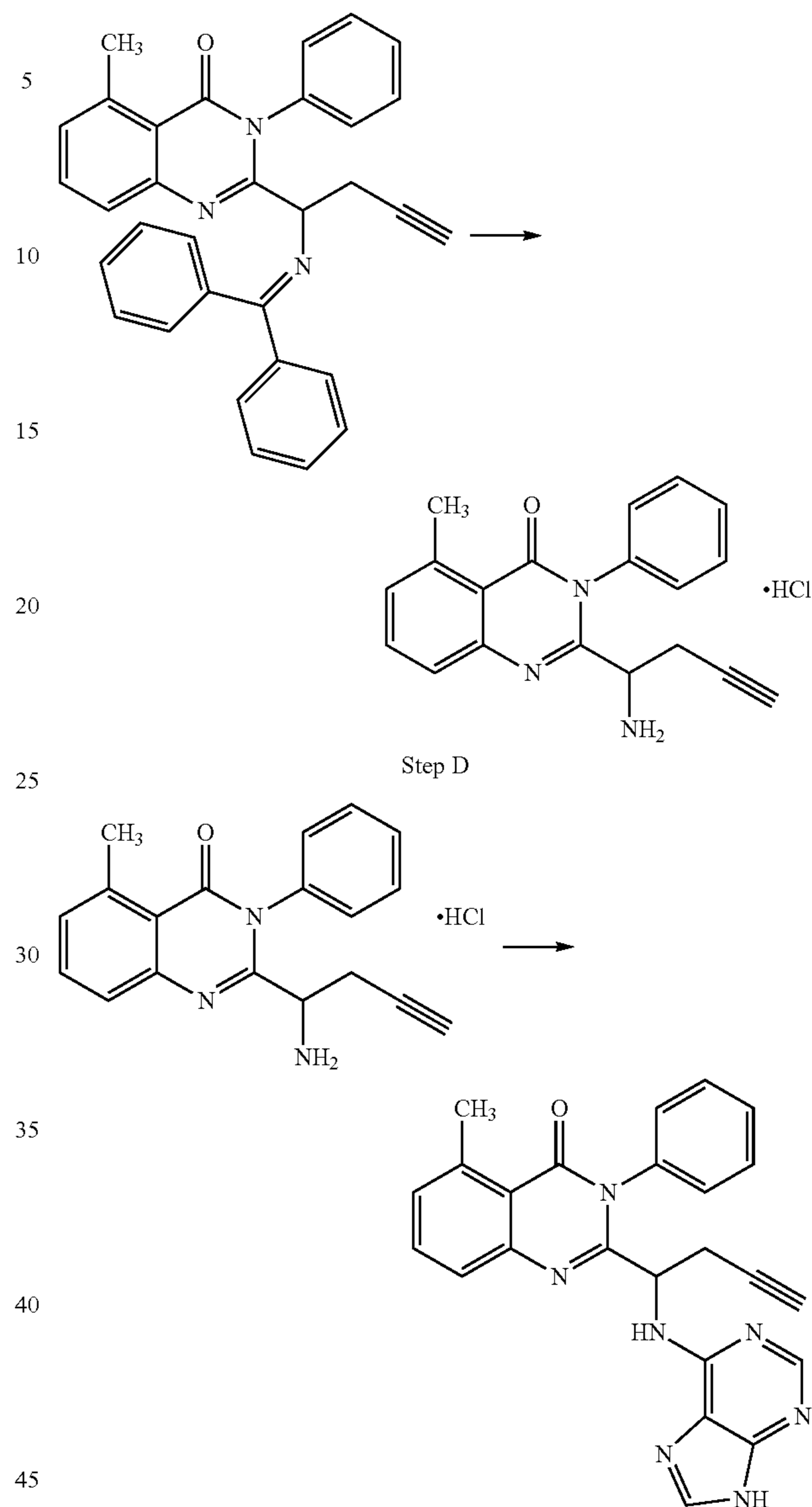
2-[1-(2-amino-9H-purin-6-ylamino)-but-3-ynyl]-5-methyl-3-phenyl-3H-quinazolin-4-one (161)
