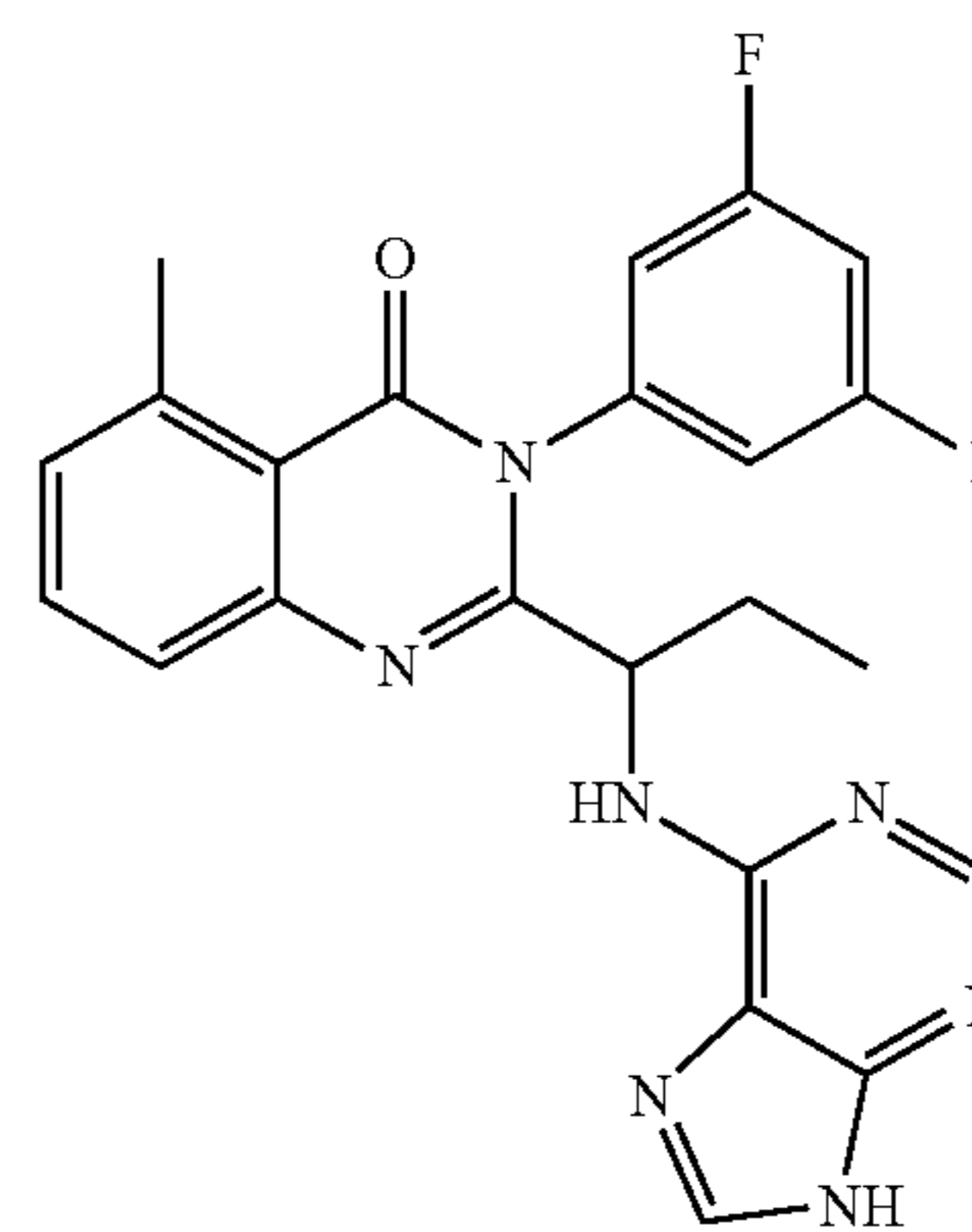
2-[1-(2-amino-9H-purin-6-ylamino)-propyl]-3-(3,5-difluoro-phenyl)-5-methyl-3H-quinazolin-4-one (94)
