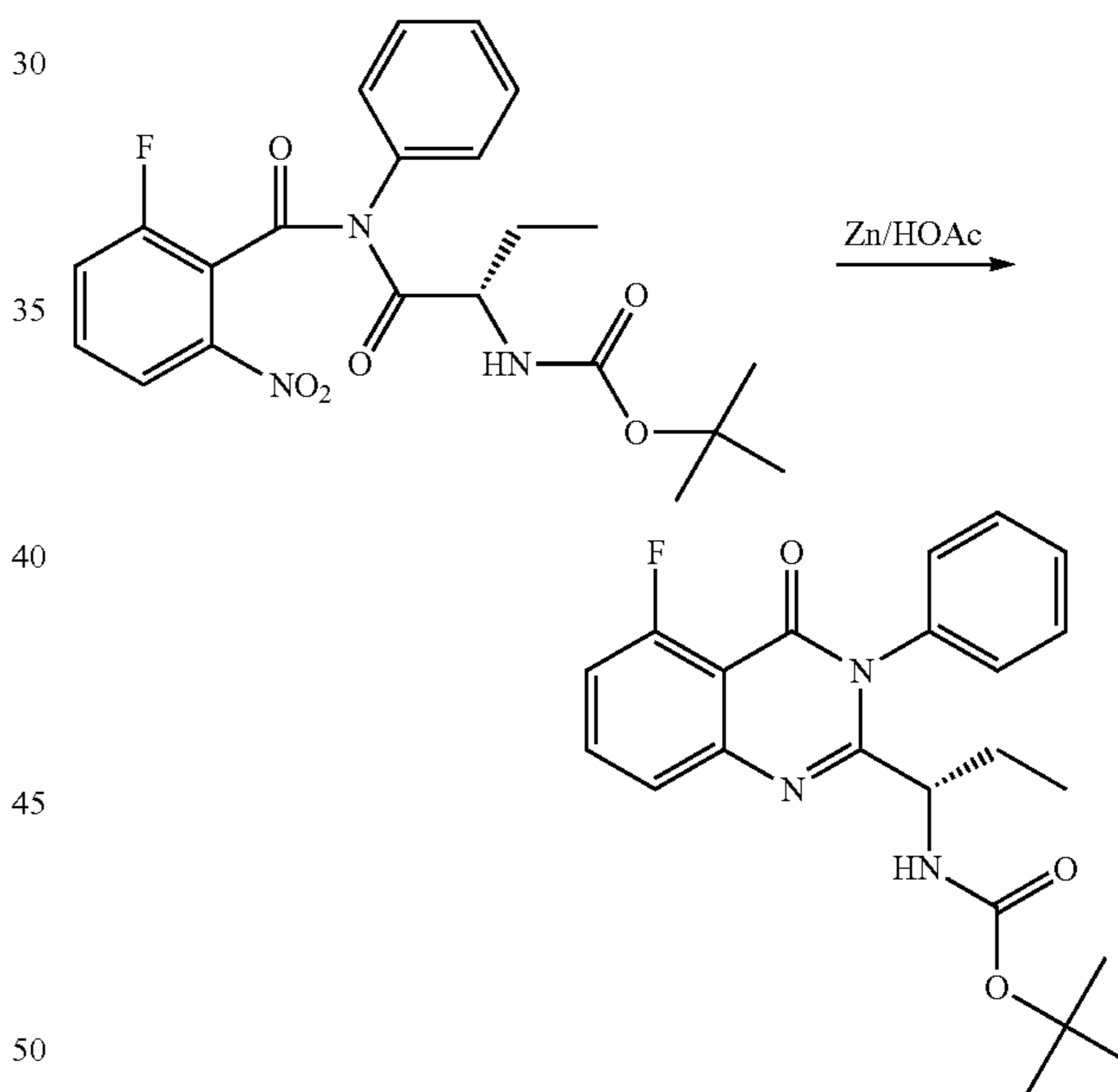
(S)-2-(1-amino-propyl)-5-fluoro-3-phenyl-3H-quinazolin-4-one (111)
