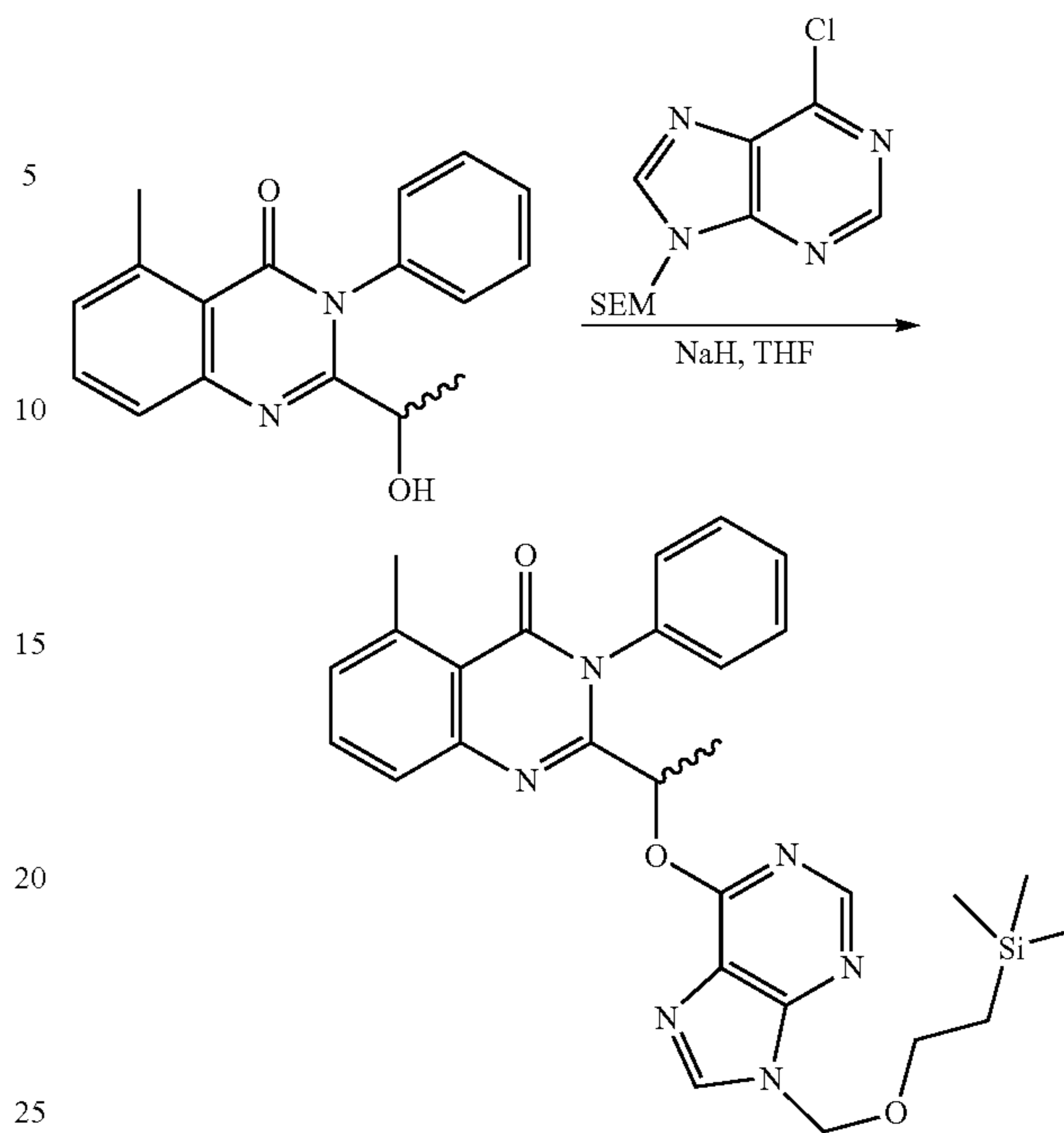
2-(1-hydroxy-ethyl)-5-methyl-3-phenyl-3H-quinazolin-4-one (181)
