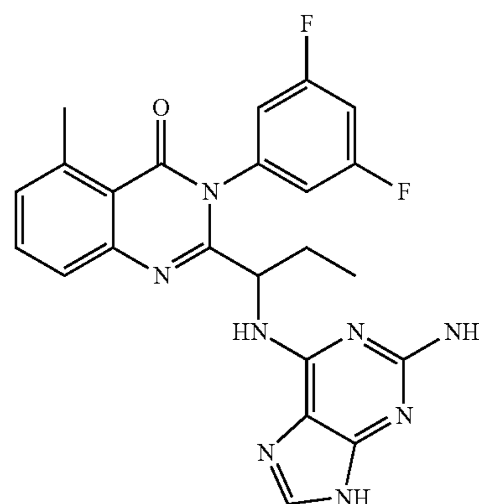
3-(3,5-difluoro-phenyl)-2-[1-(9H-purin-6-ylamino)-ethyl]-3H-quinazolin-4-one (95)
