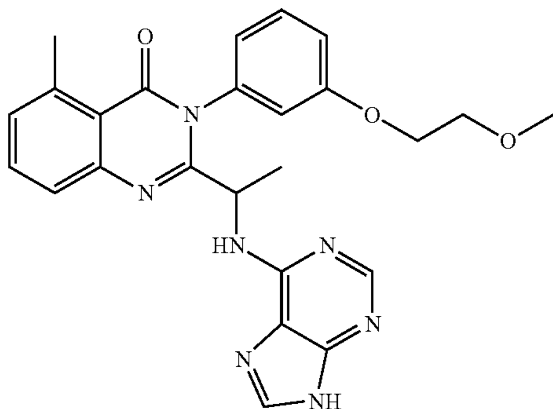
3-[3-(2-Methoxy-ethoxy)phenyl]-5-methyl-2-[1-(9H-purin-6-ylamino)-ethyl]-3H-quinazolin-4-one (147)
