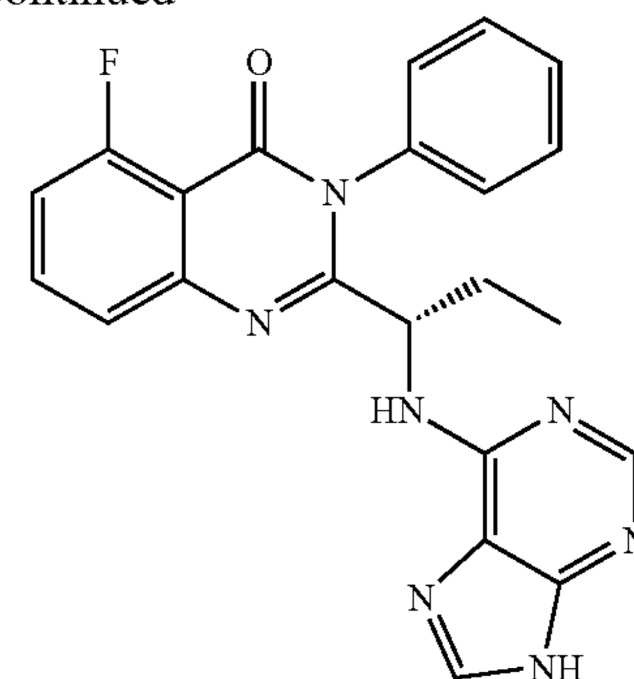
(S)-3-phenyl-2-[1-(9H-purin-6-ylamino)-ethyl]-3H-quinazolin-4-one (112)
