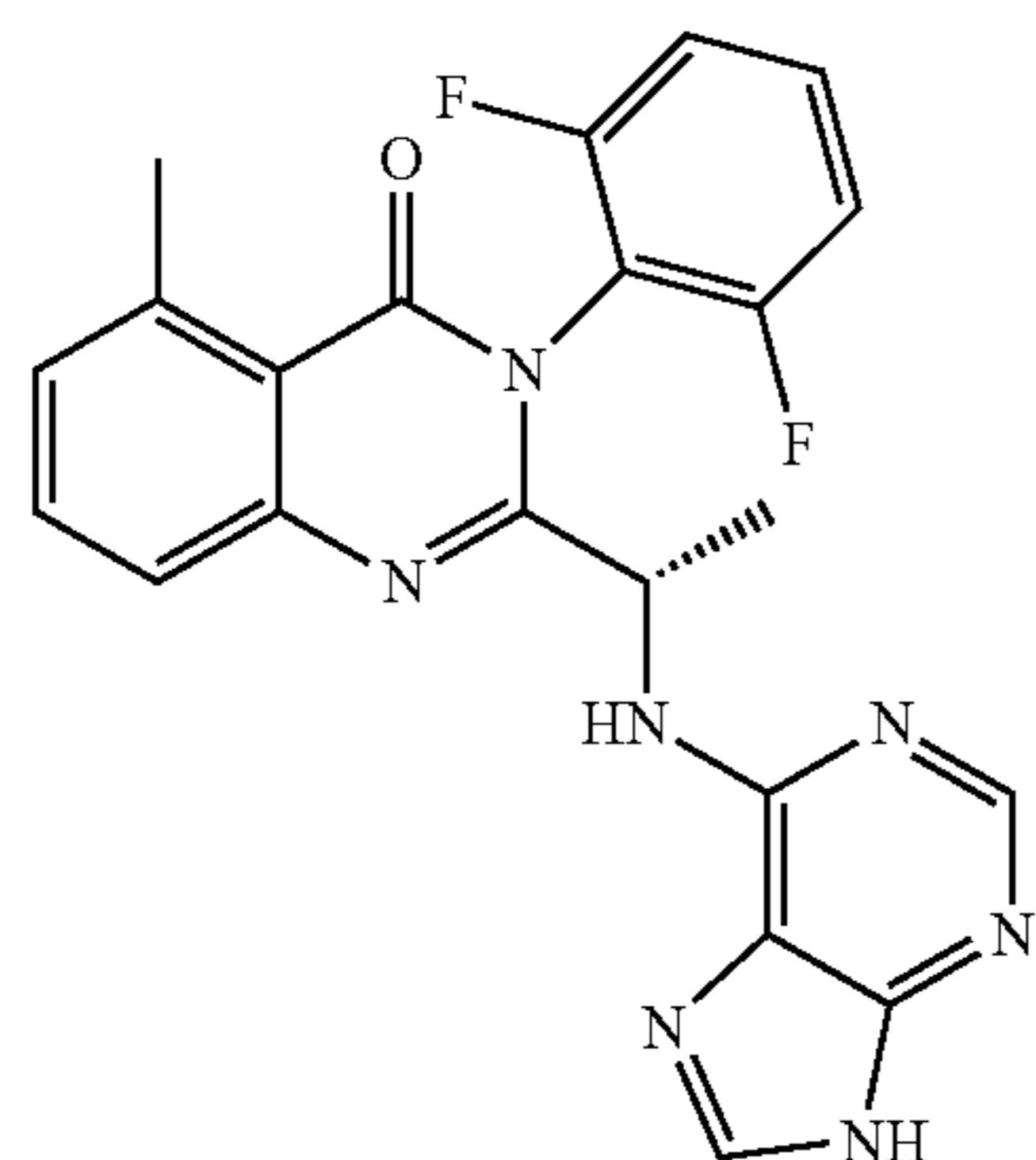
(S)-3-(2,6-difluoro-phenyl)-2-[1-(9H-purin-6-ylamino)-ethyl]-3H-quinazolin-4-one (119)
