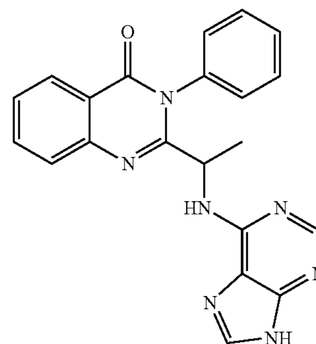
2-[5-amino-1-(9H-purin-6-ylamino)-pentyl]-5-methyl-3-phenyl-3H-quinazolin-4-one (54)
