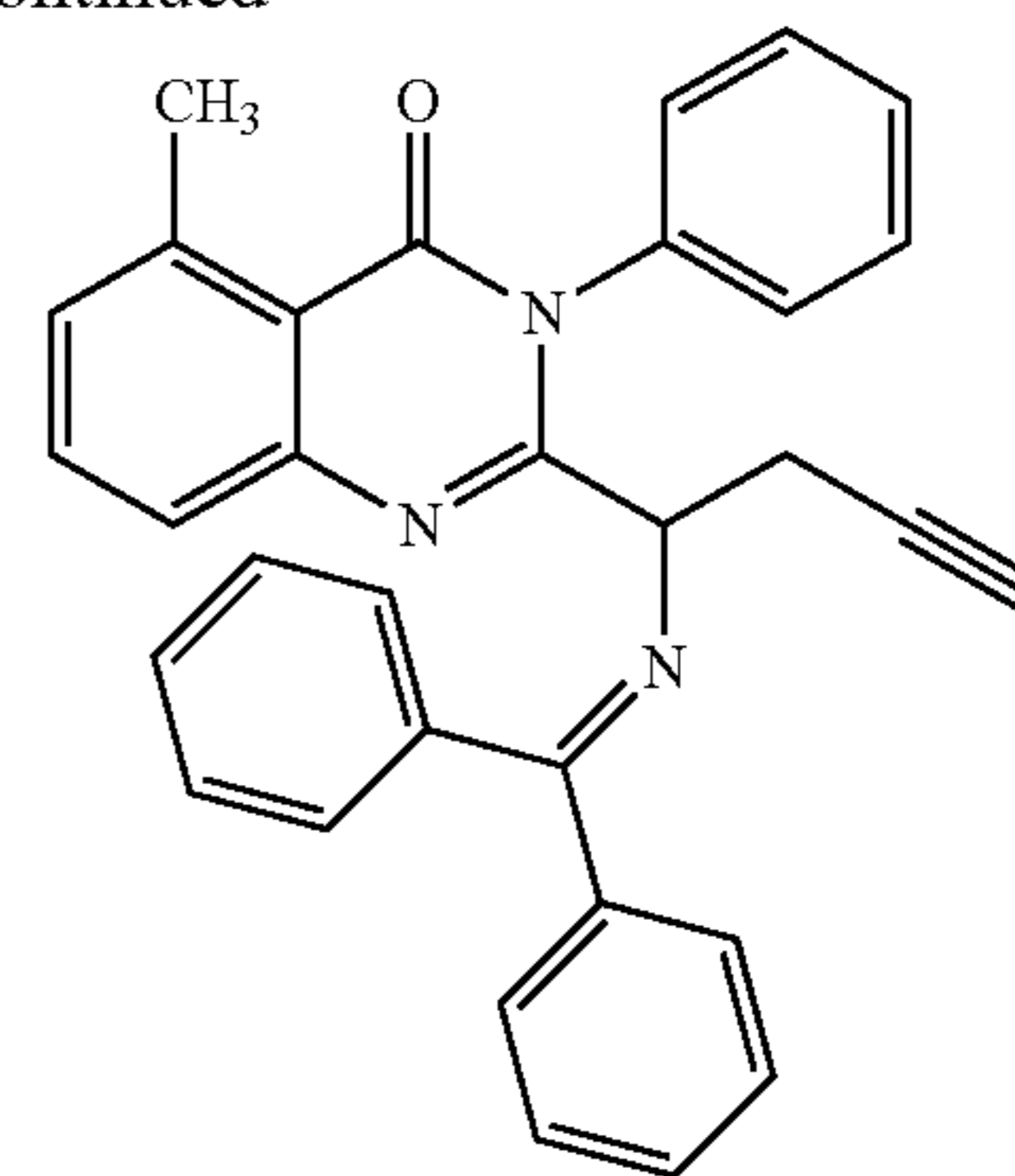
2-(1-(amino-but-3-ynyl)-5-methyl-3-phenyl-3H-quinazolin-4-one (164)
