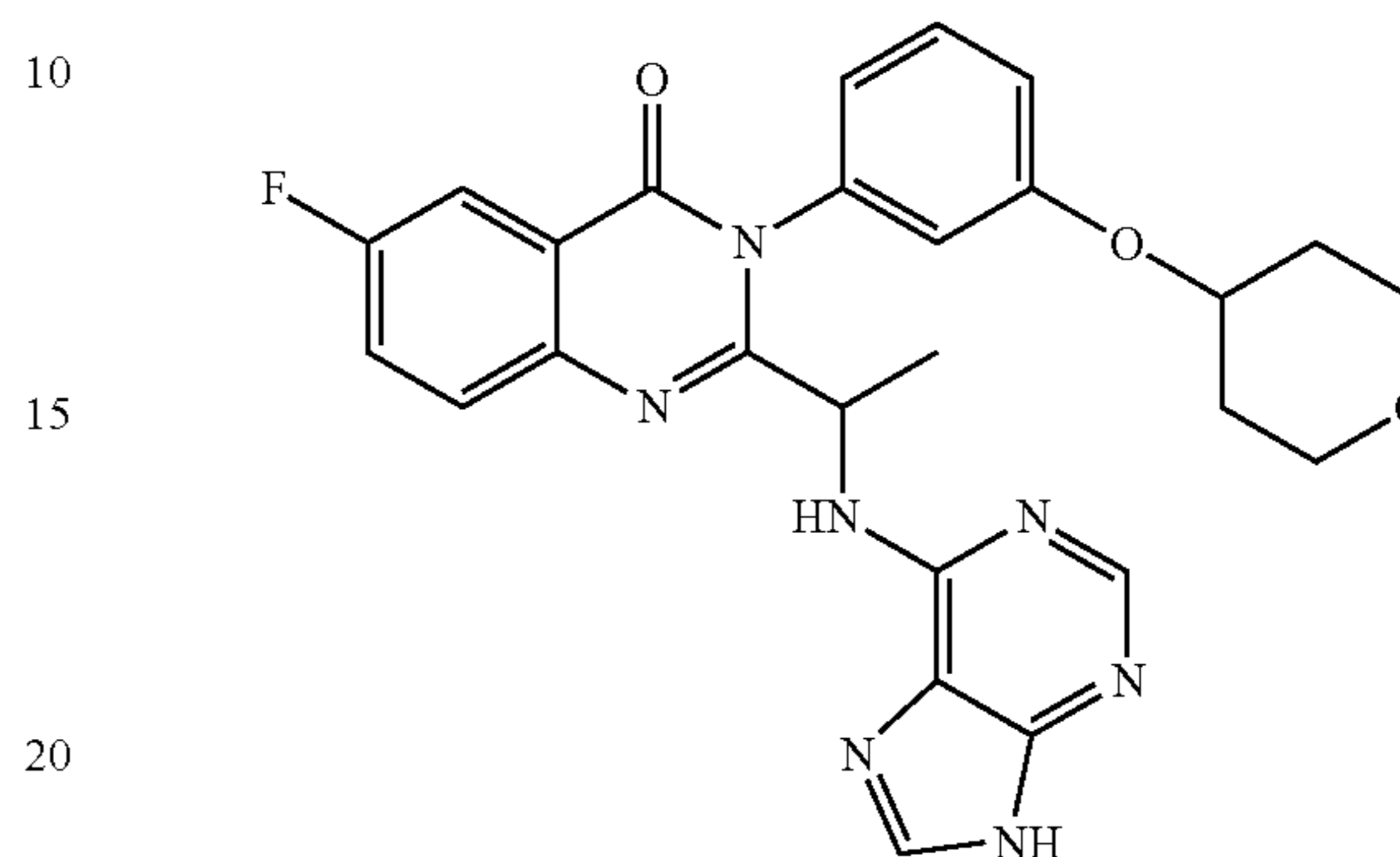
6-Fluoro-2-[1-(9H-purin-6-ylamino)-ethyl]-3-[3-(tetrahydro-pyran-4-yloxy)-phenyl]-3H-quinazolin-4-one (148)
