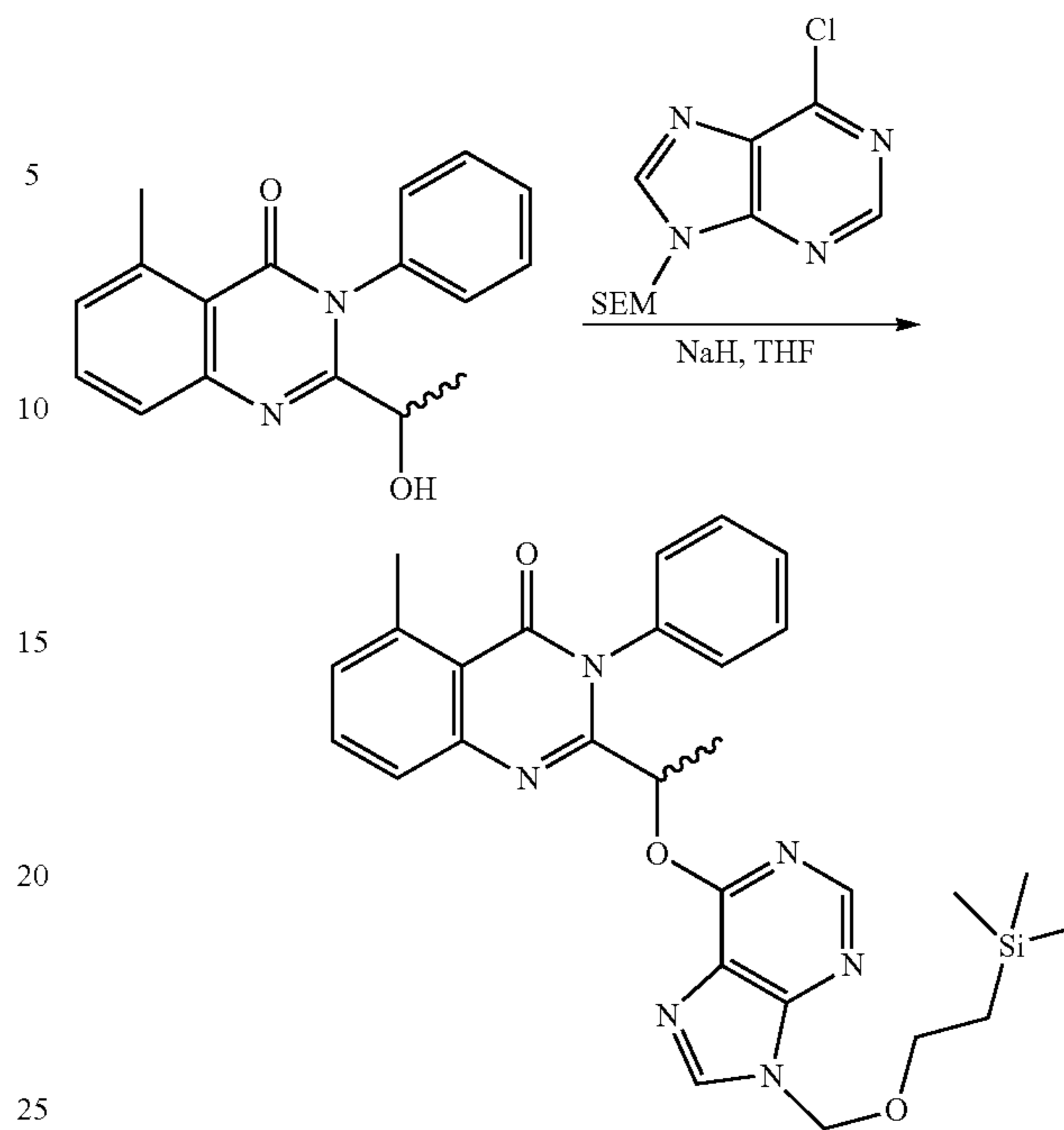
2-(1-hydroxy-ethyl)-5-methyl-3-phenyl-3H-quinazolin-4-one (181)
