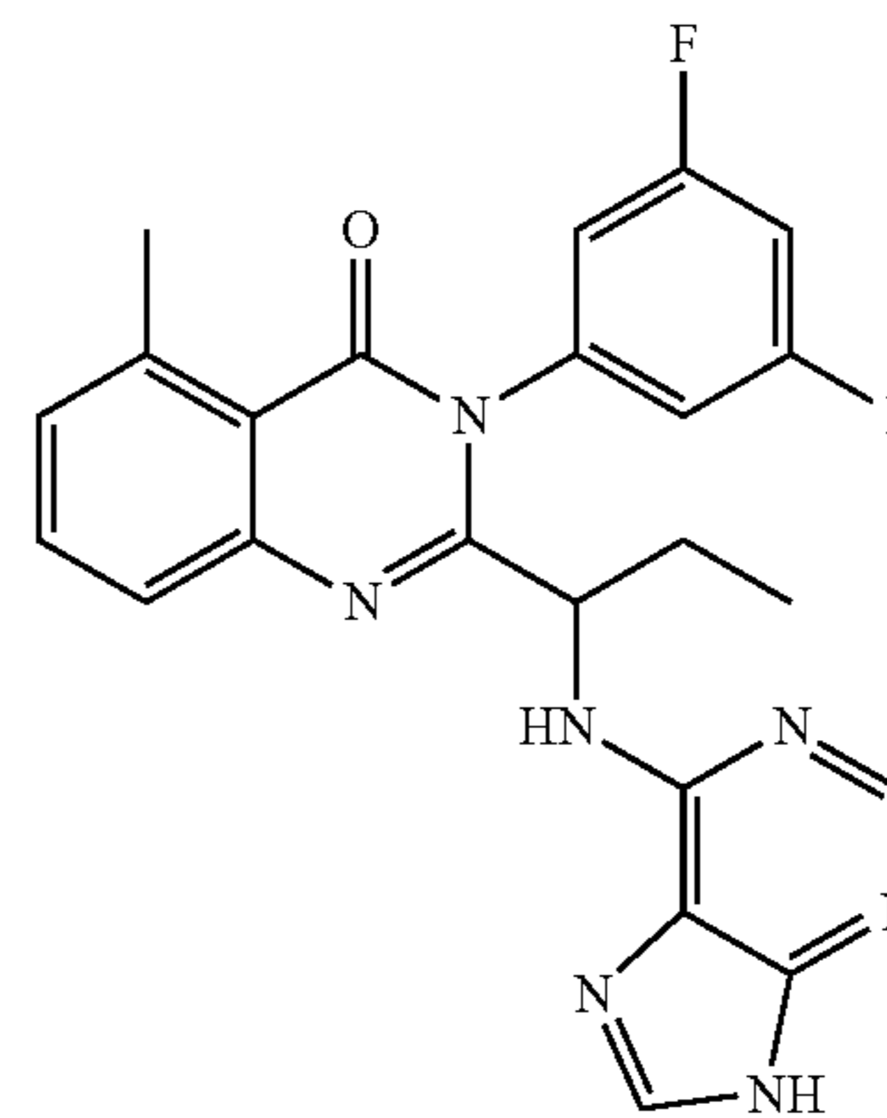
2-[1-(2-amino-9H-purin-6-ylamino)-propyl]-3-(3,5-difluoro-phenyl)-5-methyl-3H-quinazolin-4-one (94)
