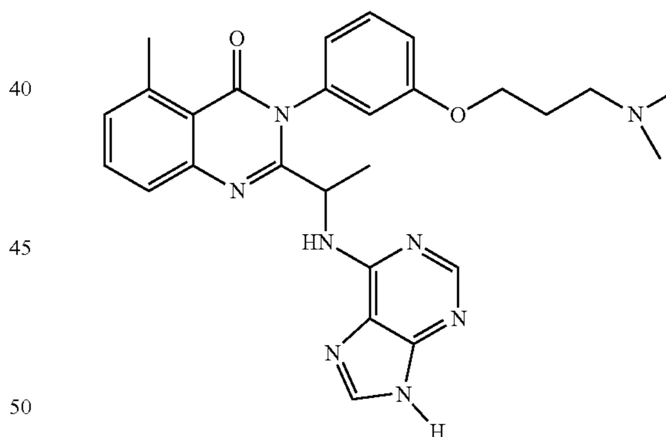
3-[3-(3-Dimethylamino-propoxy)-phenyl]-5-methyl-2-[1-(9H-purin-6-ylamino)-ethyl]-3H-quinazolin-4-one (150)
