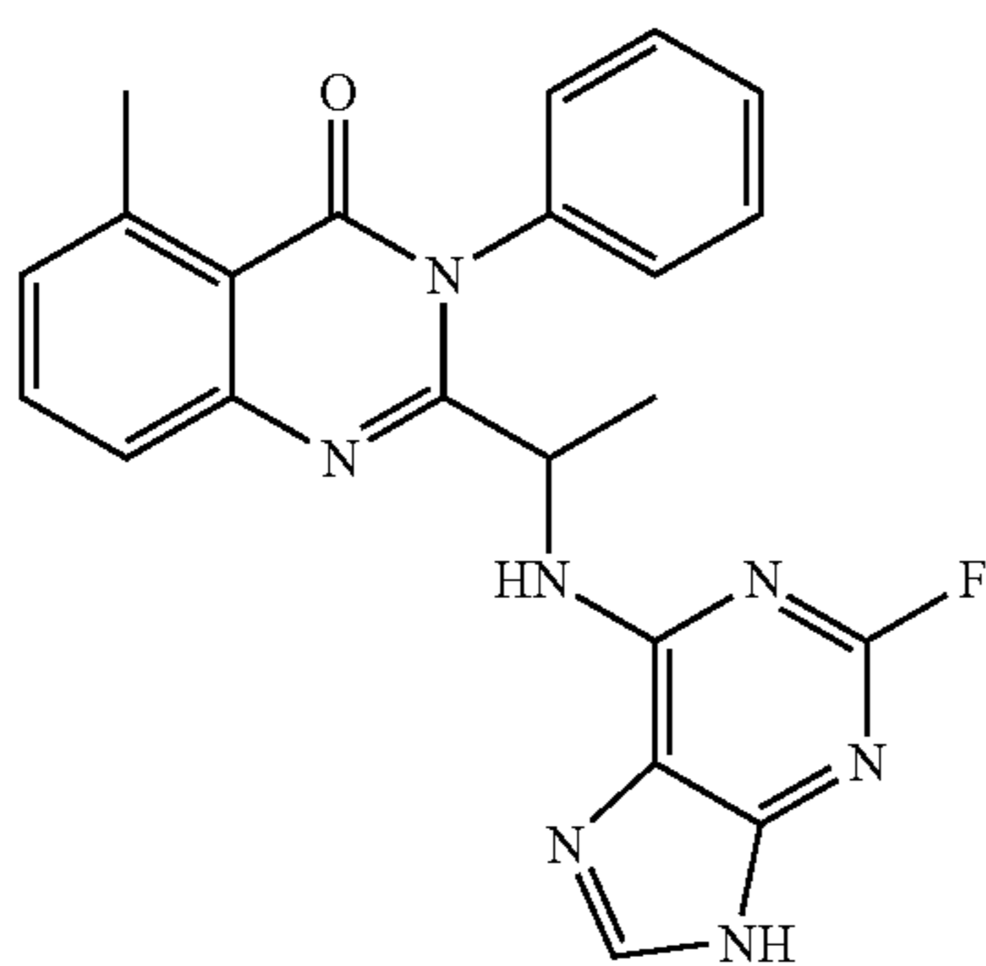
3-(2,6-difluoro-phenyl)-5-methyl-2-[1-(9H-purin-6-ylamino)-ethyl]-3H-quinazolin-4-one (19)
