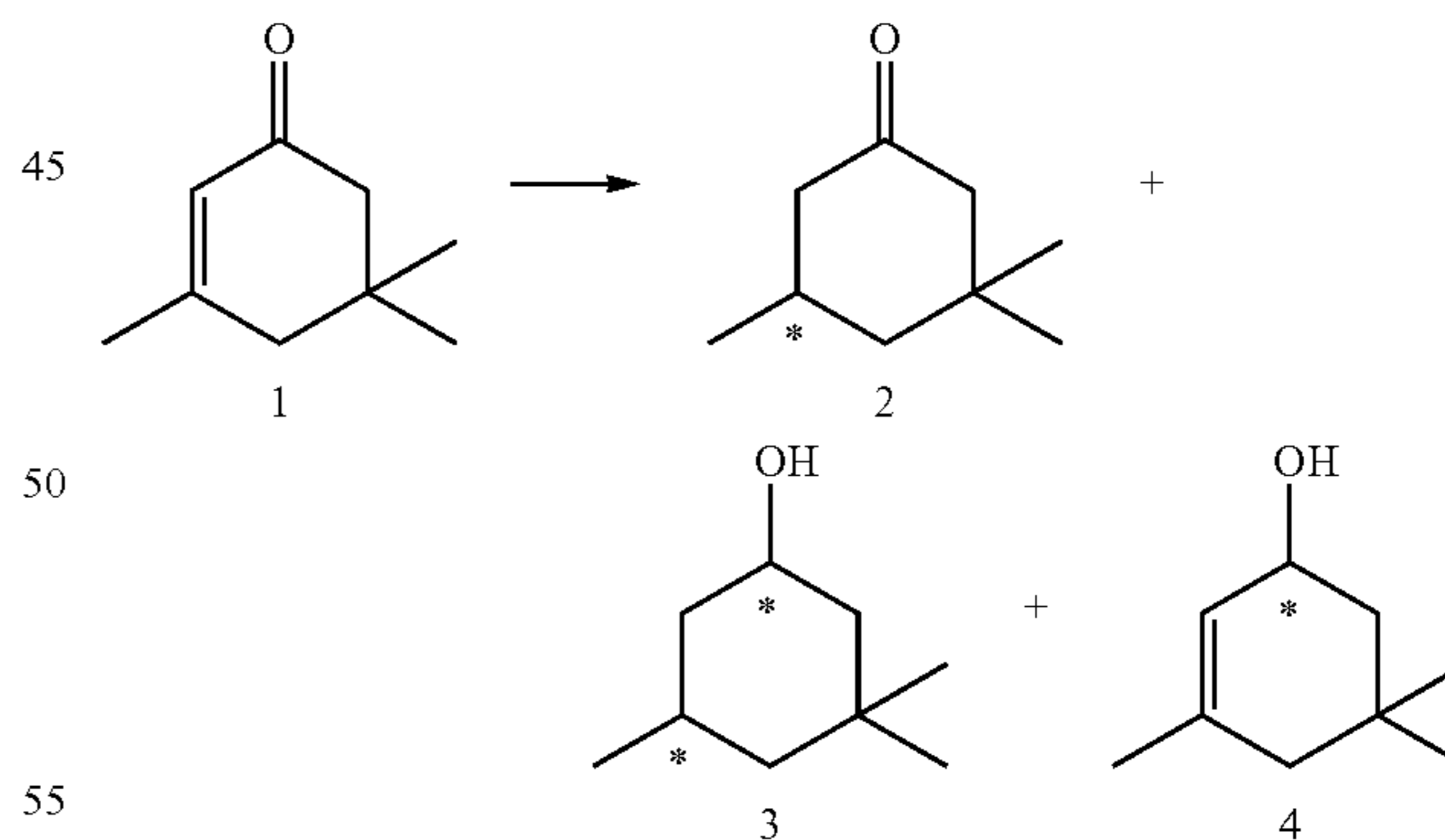
Scheme A: Asymmetric hydrogenation of isophorone 1
