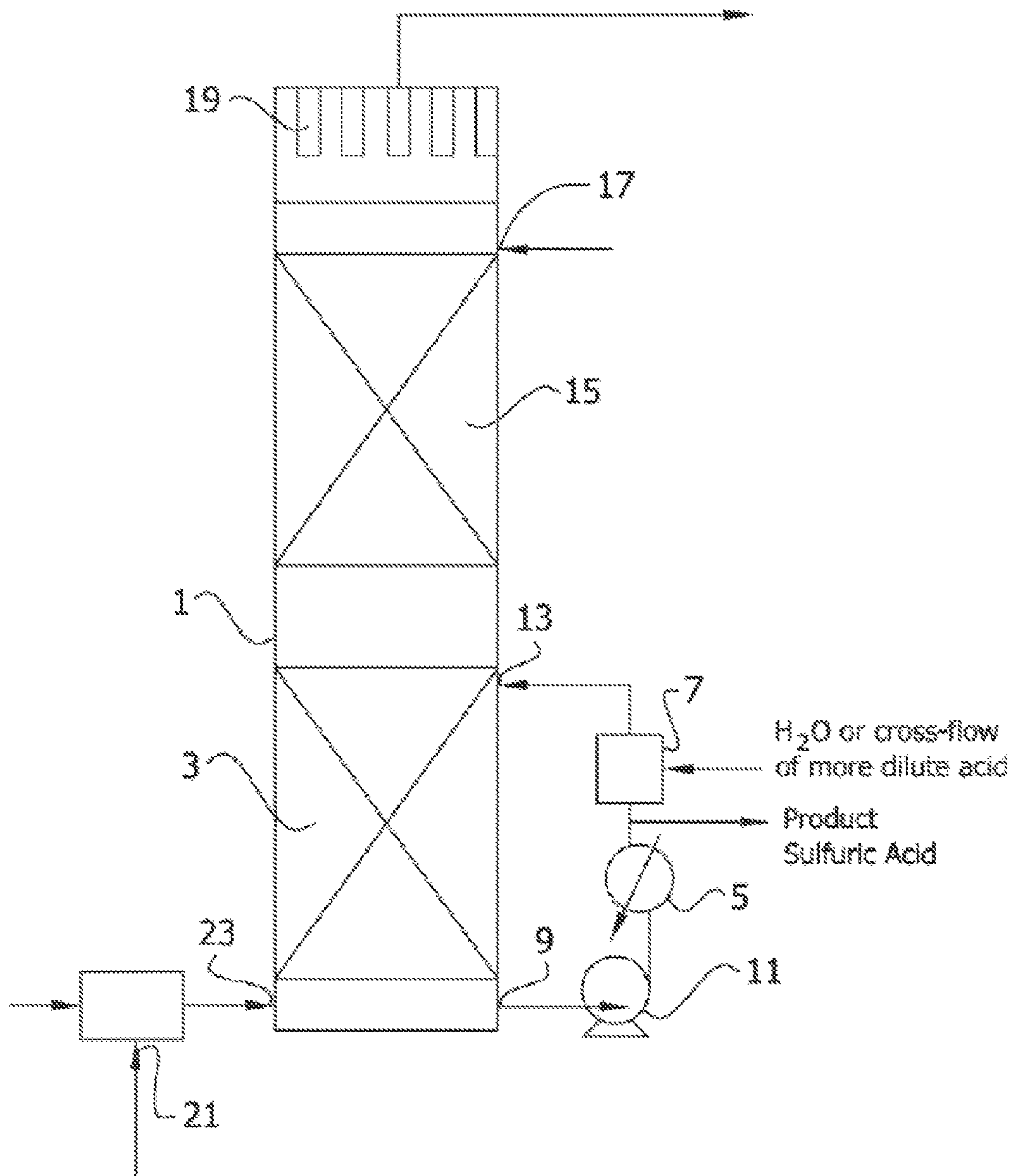
PRIOR ART
