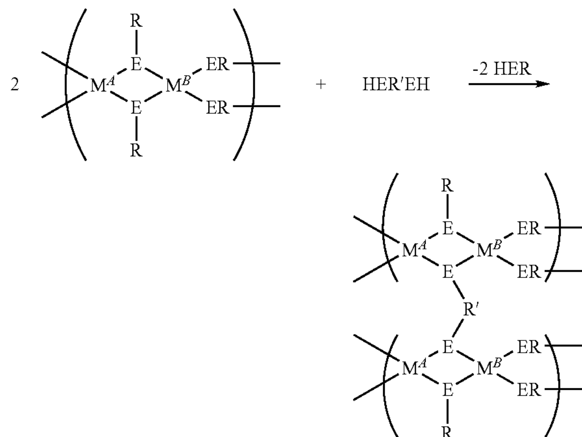
REACTION SCHEME 14
