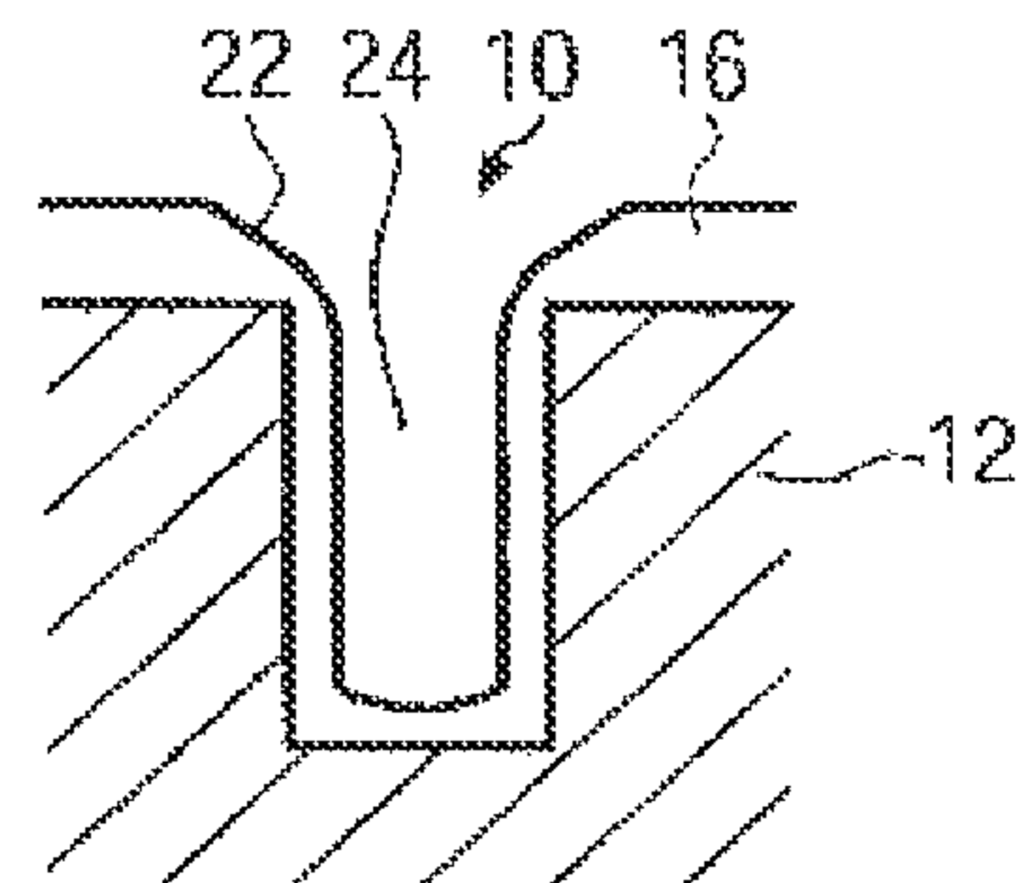
FIG. 1C (prior art)
