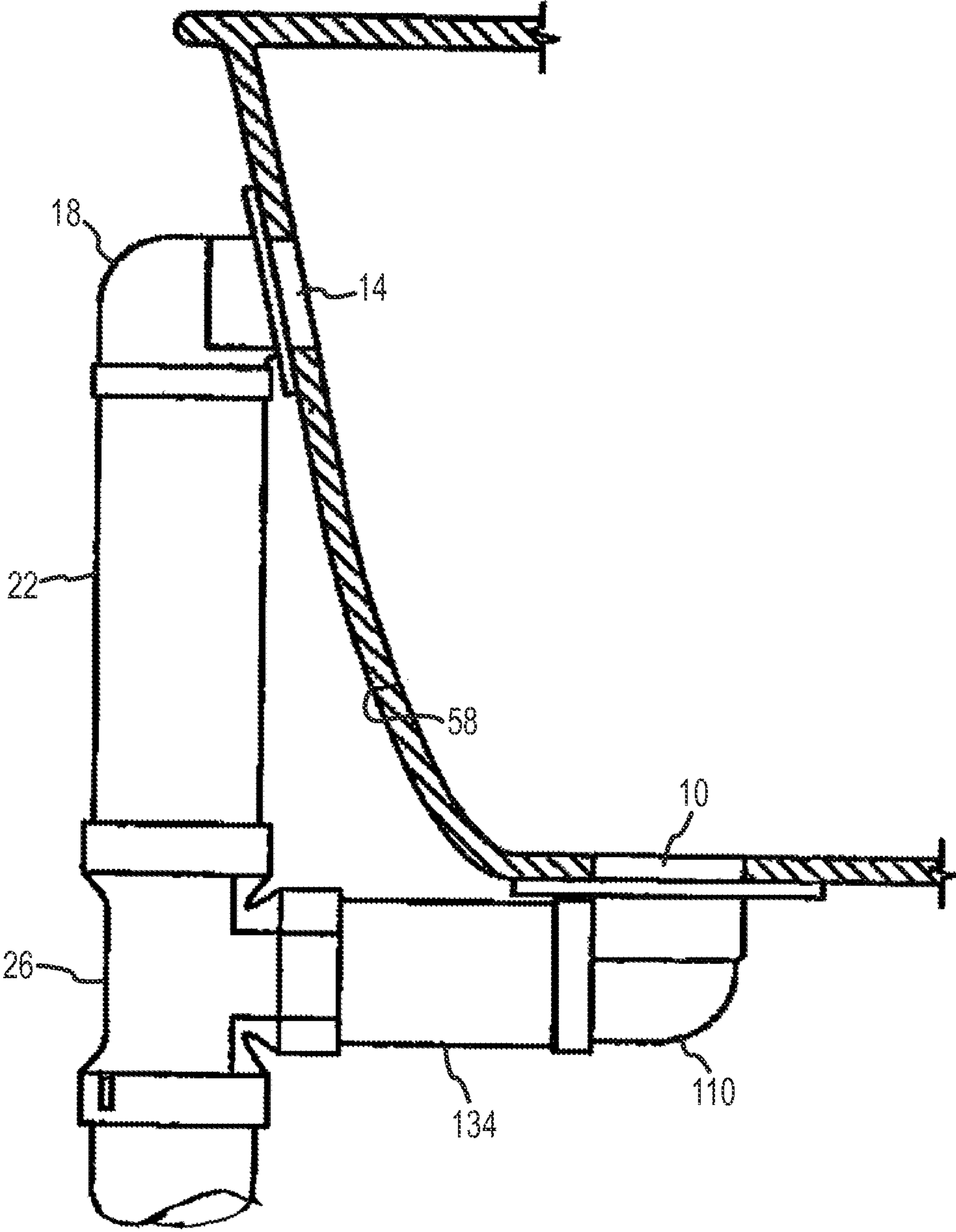
FIG. 12 (PRIOR ART)
