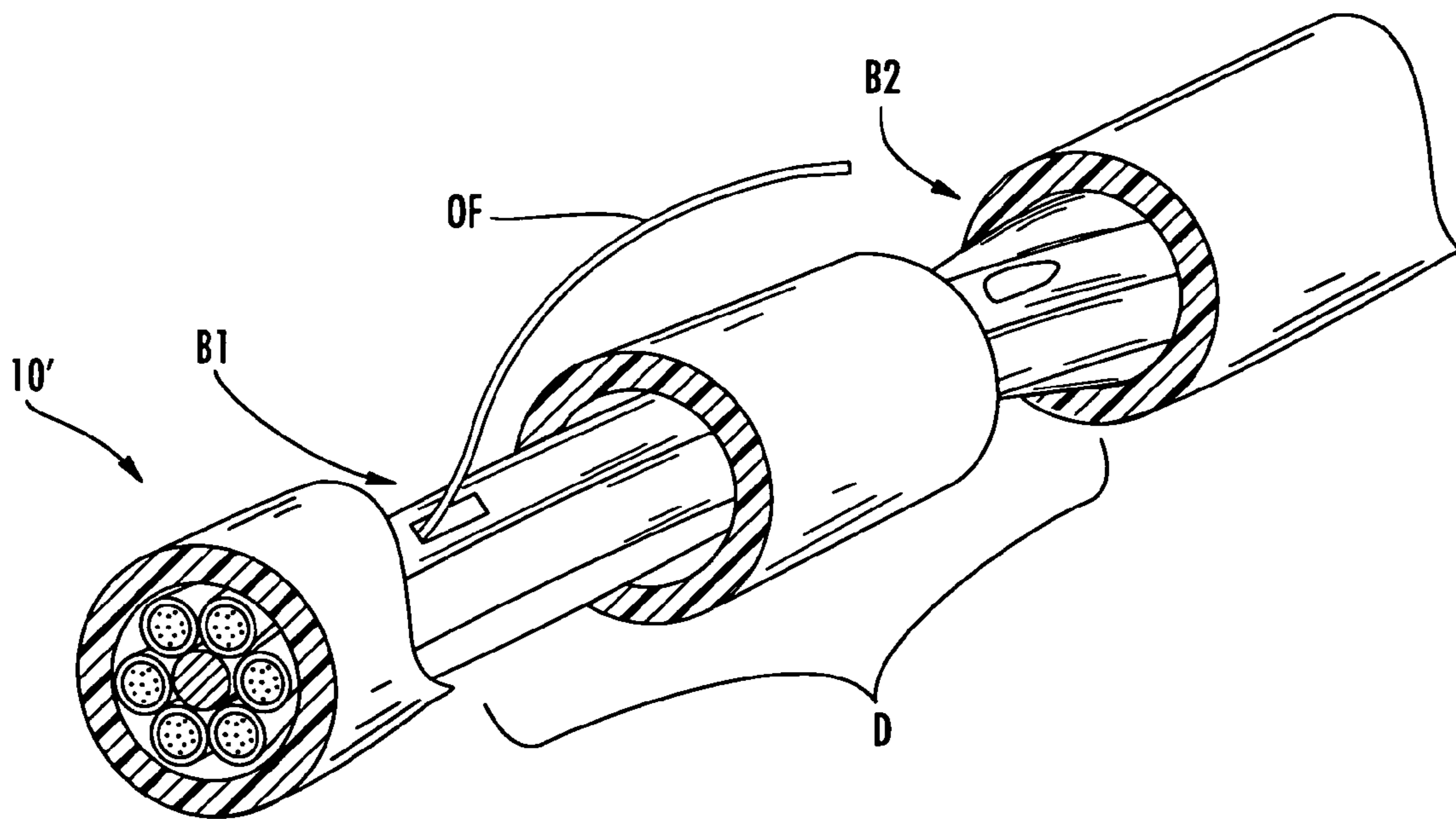
FIG. 2 (PRIOR ART)
