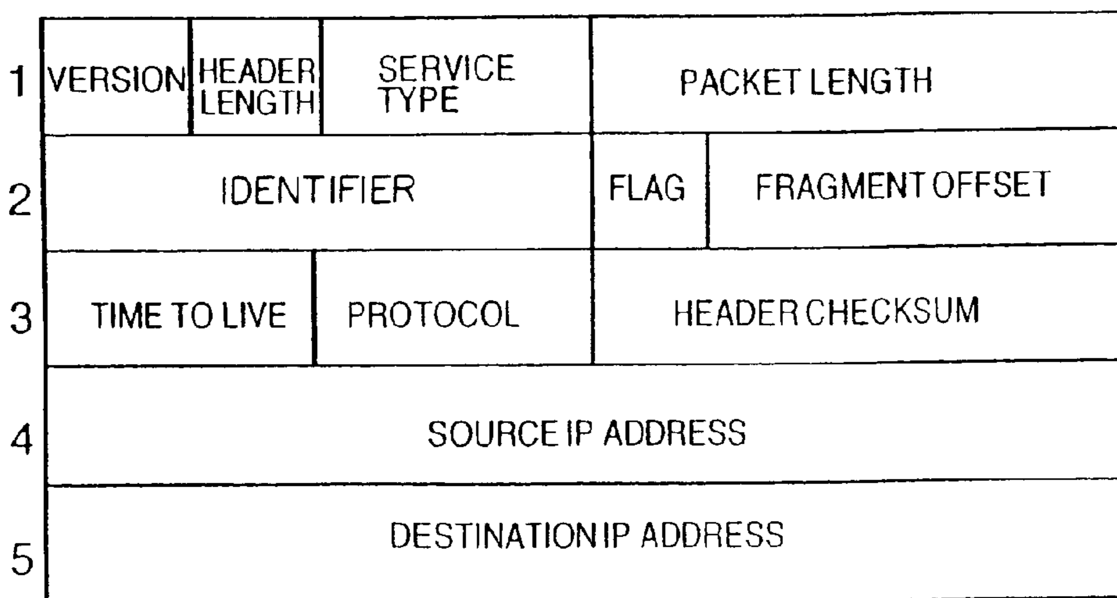
IPv4 HEADER FORMAT
