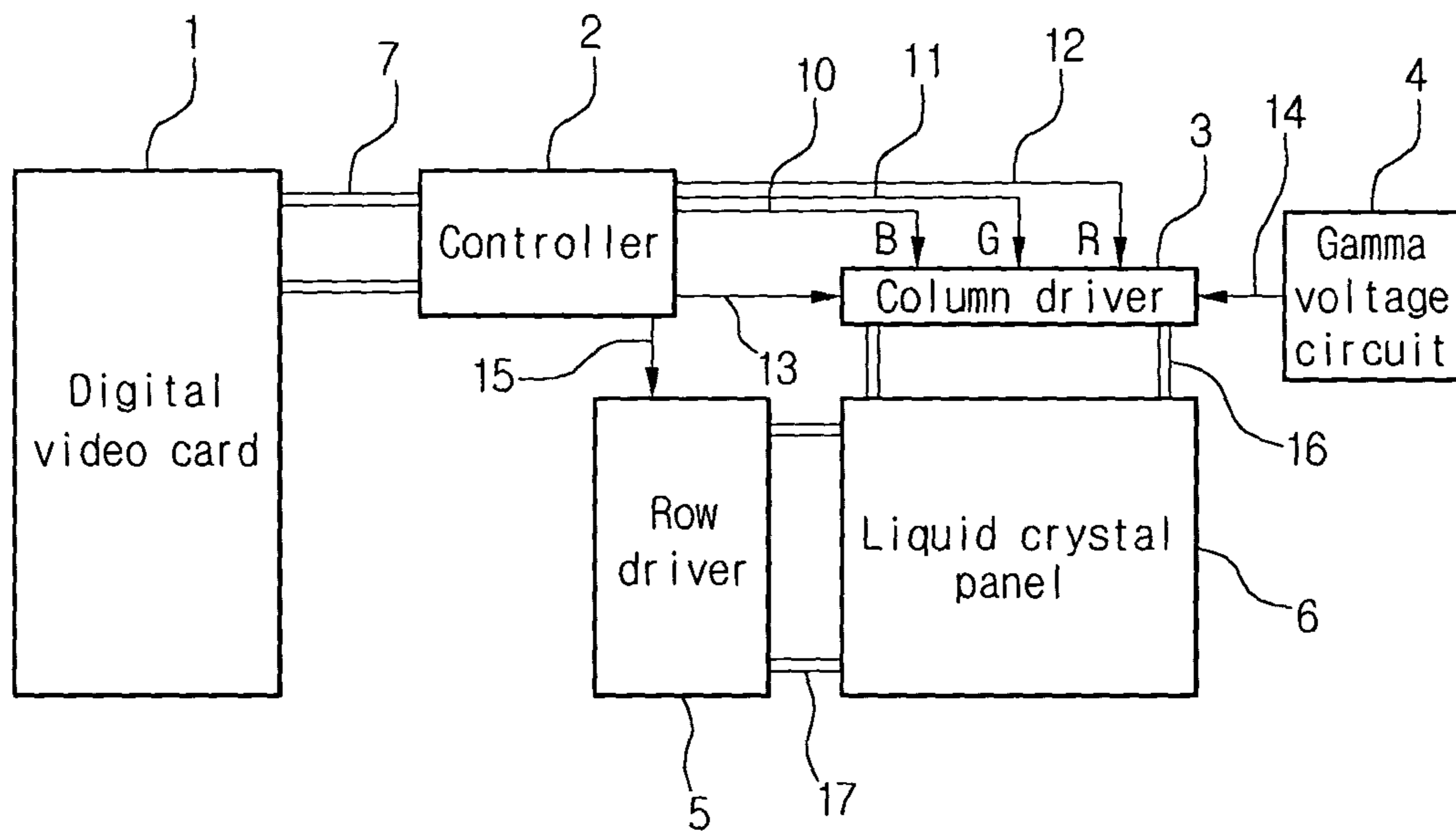
Fig. 1 Related Art
