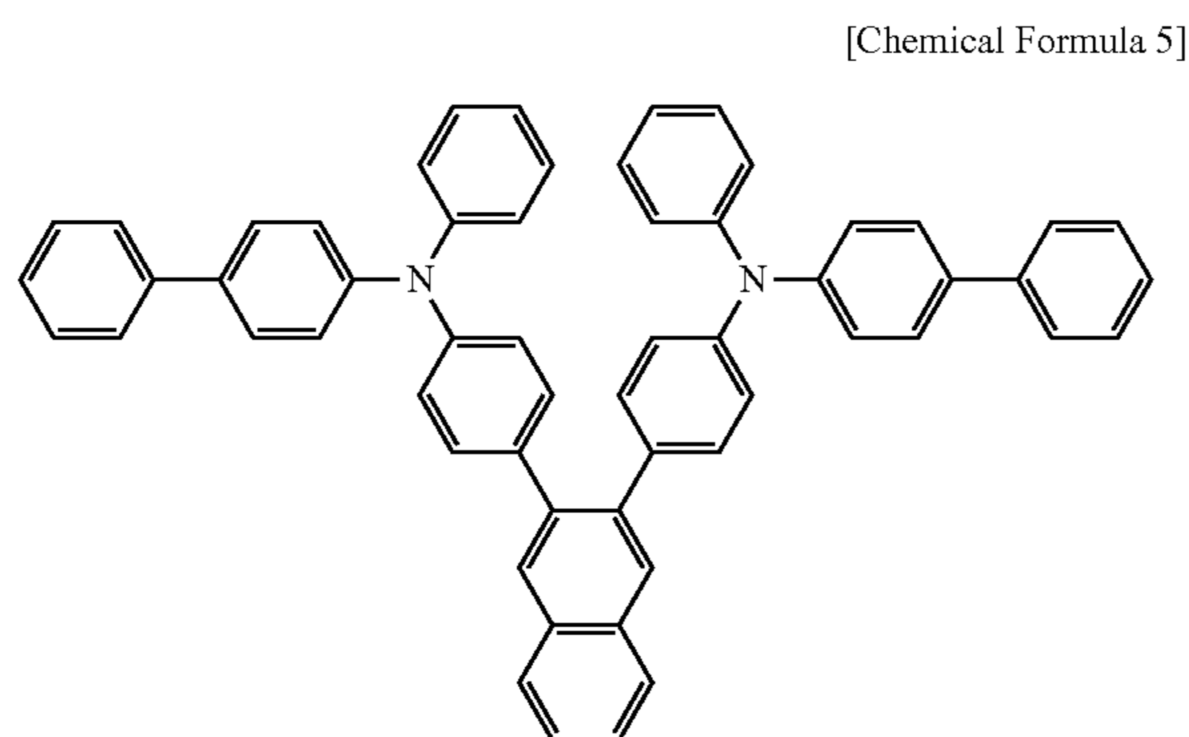
BPAPQ
