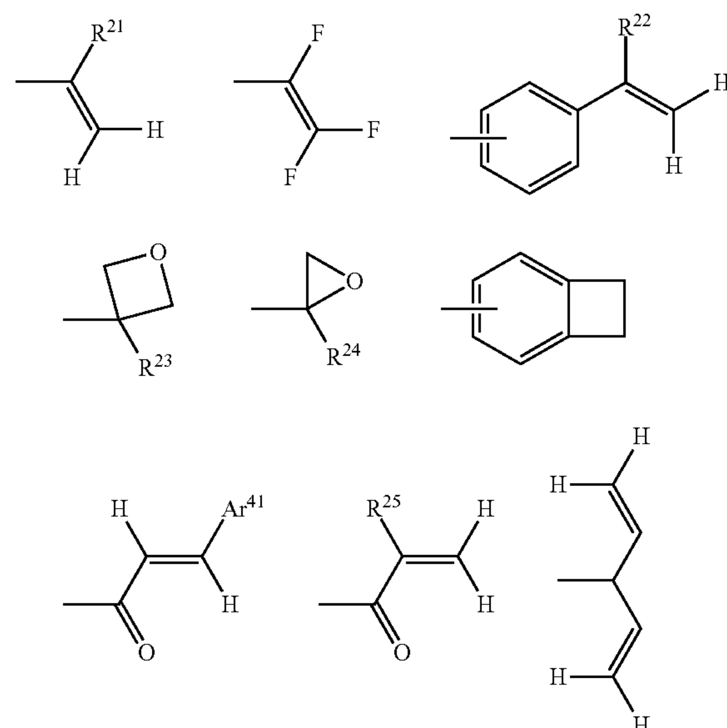
[Chemical Formula 6]
