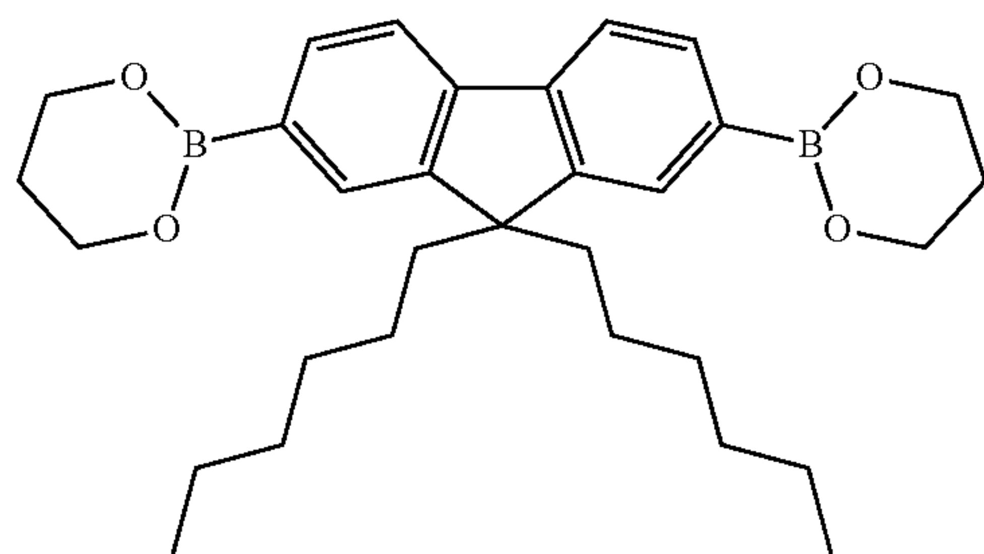
Compound 4
