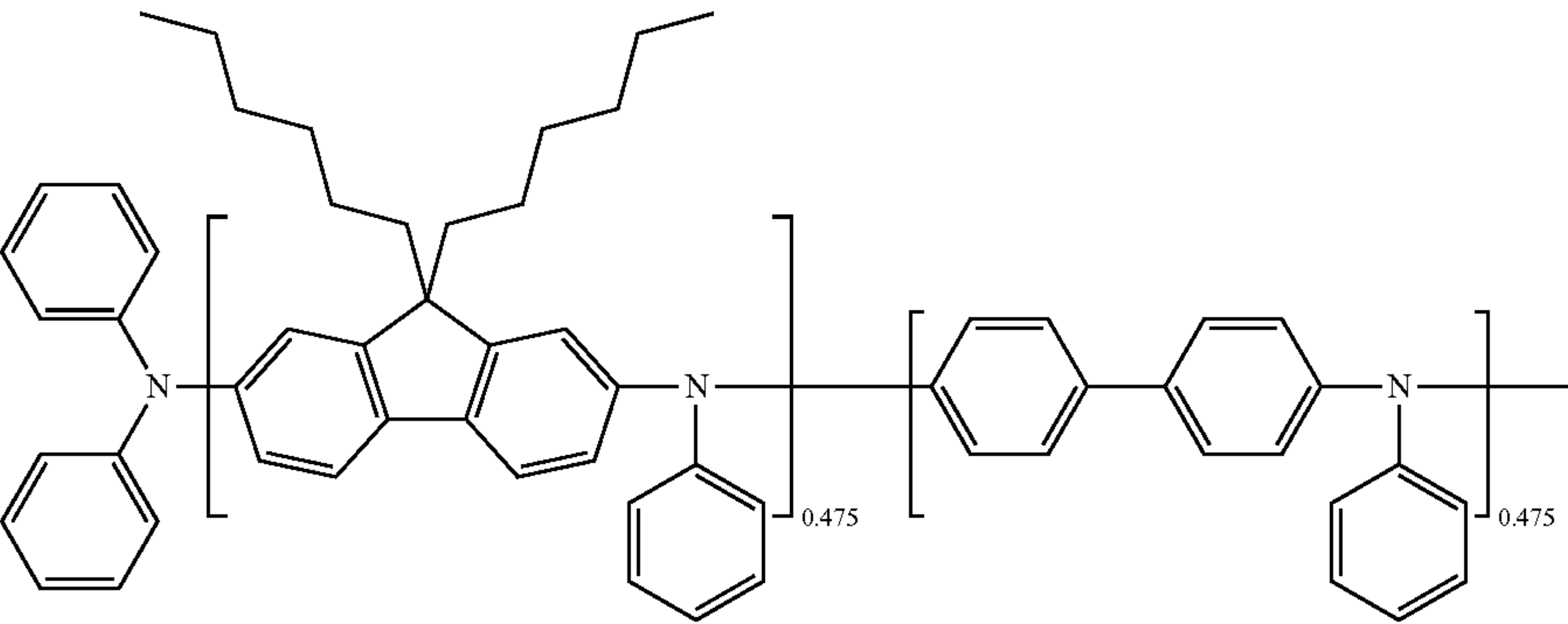
[Chemical Formula 105]
