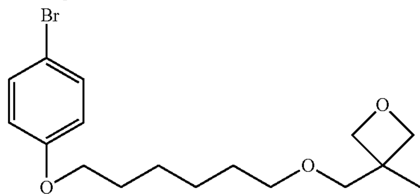
Product 1
