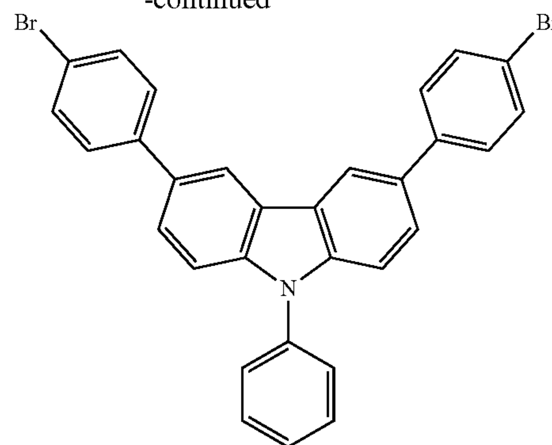
Product 30
