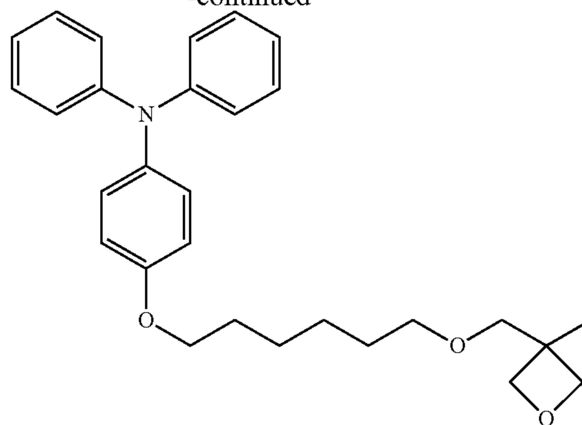
Product 2
