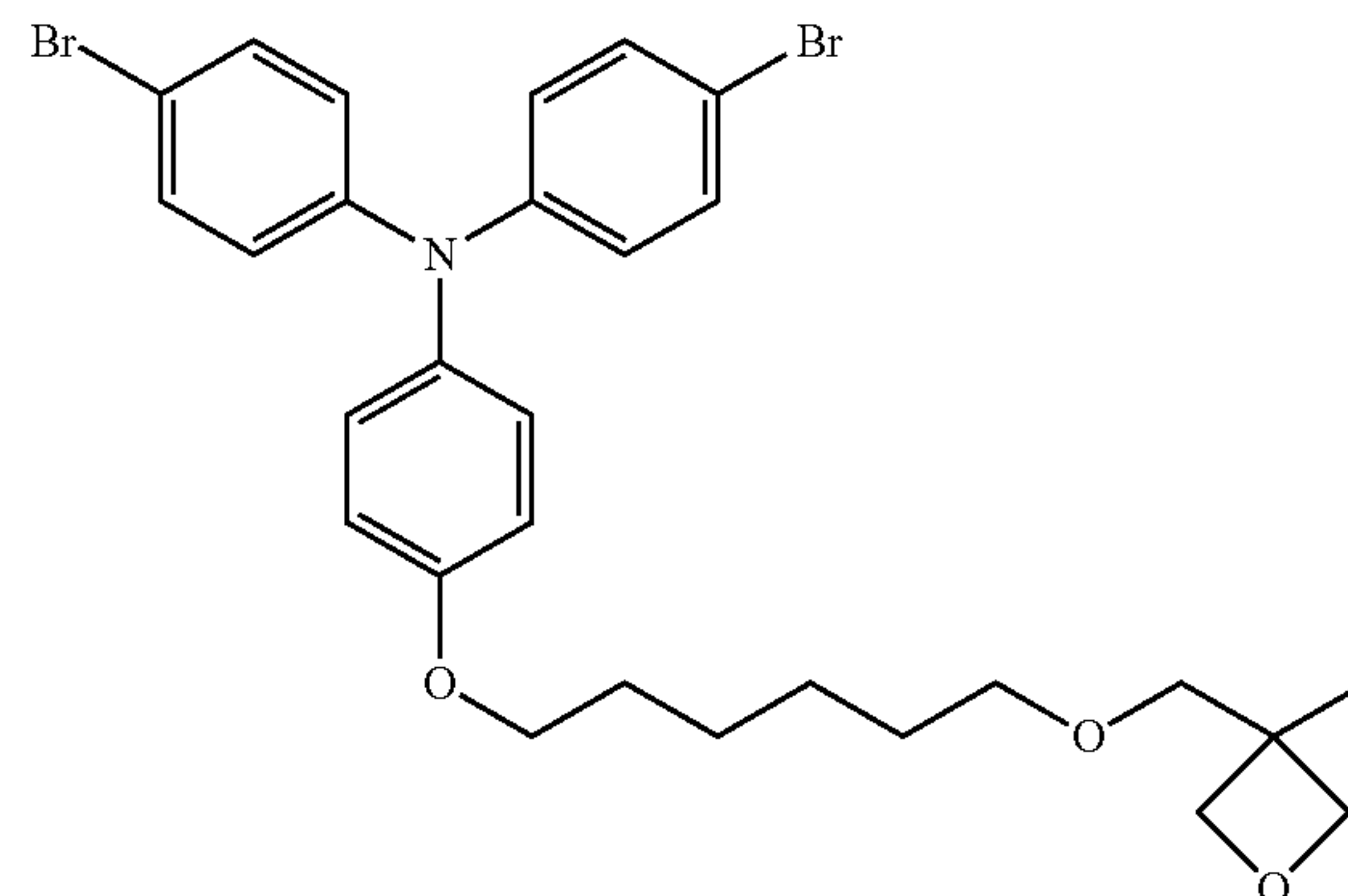
Product 3
