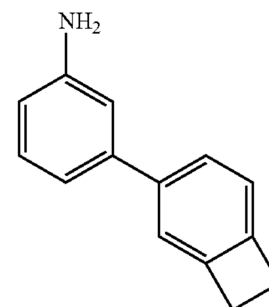
Product 6
