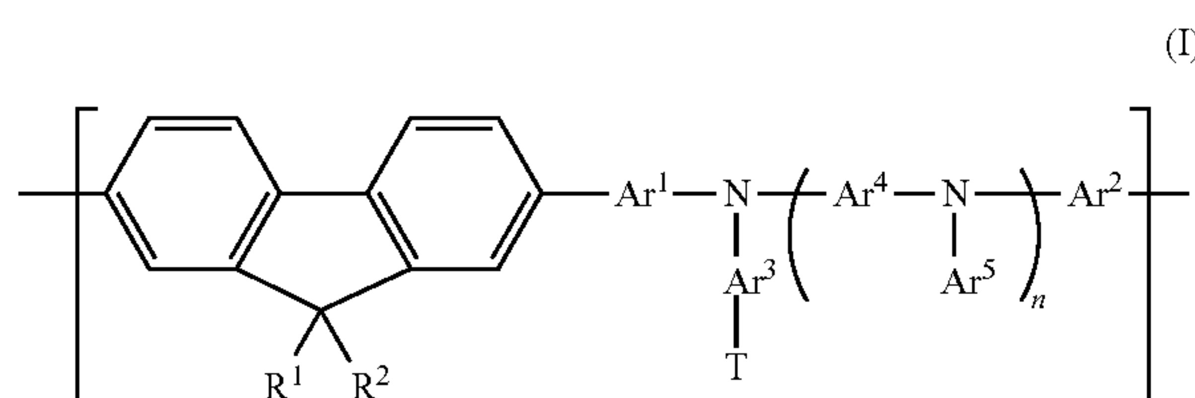
[Chemical Formula 4]
