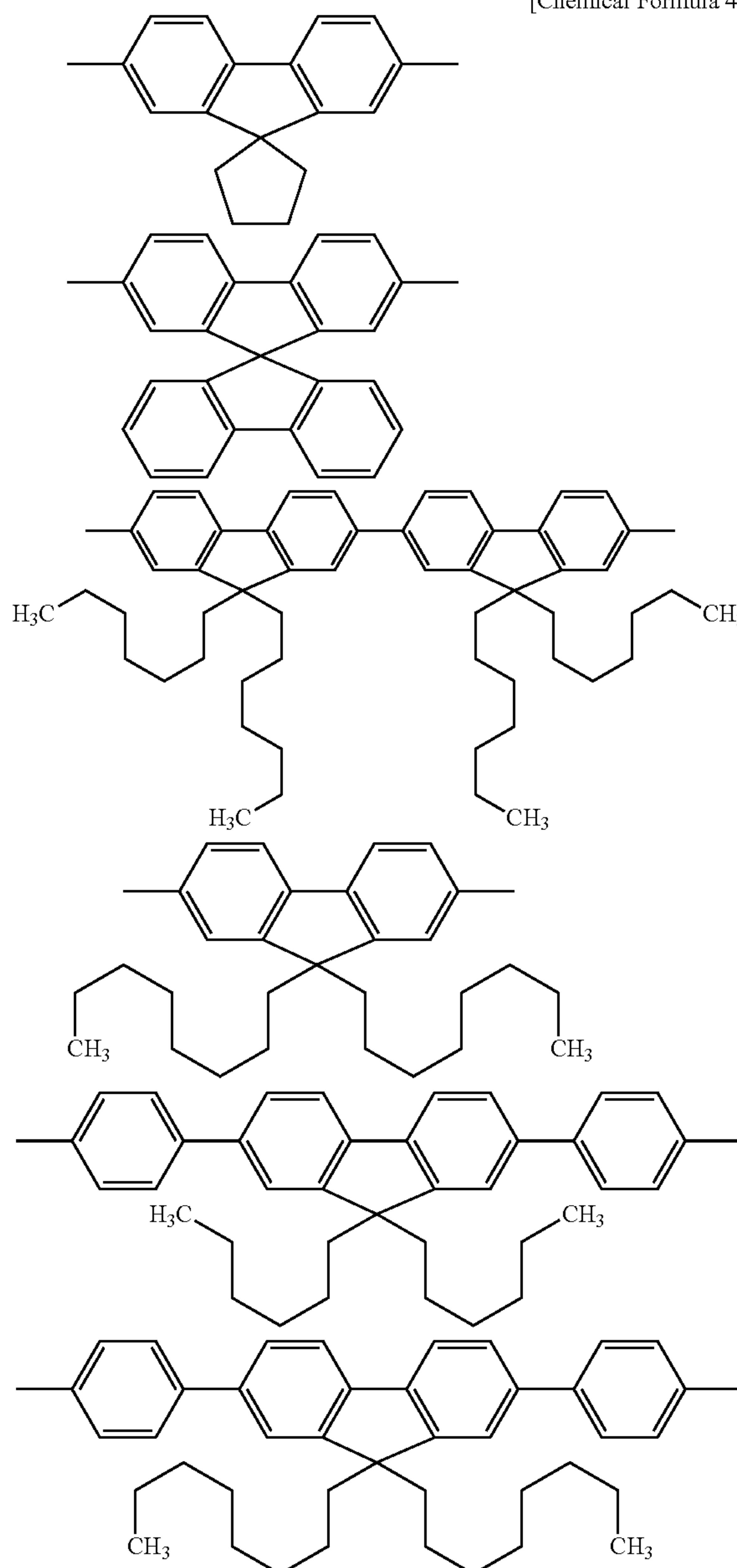
[Chemical Formula 41]
