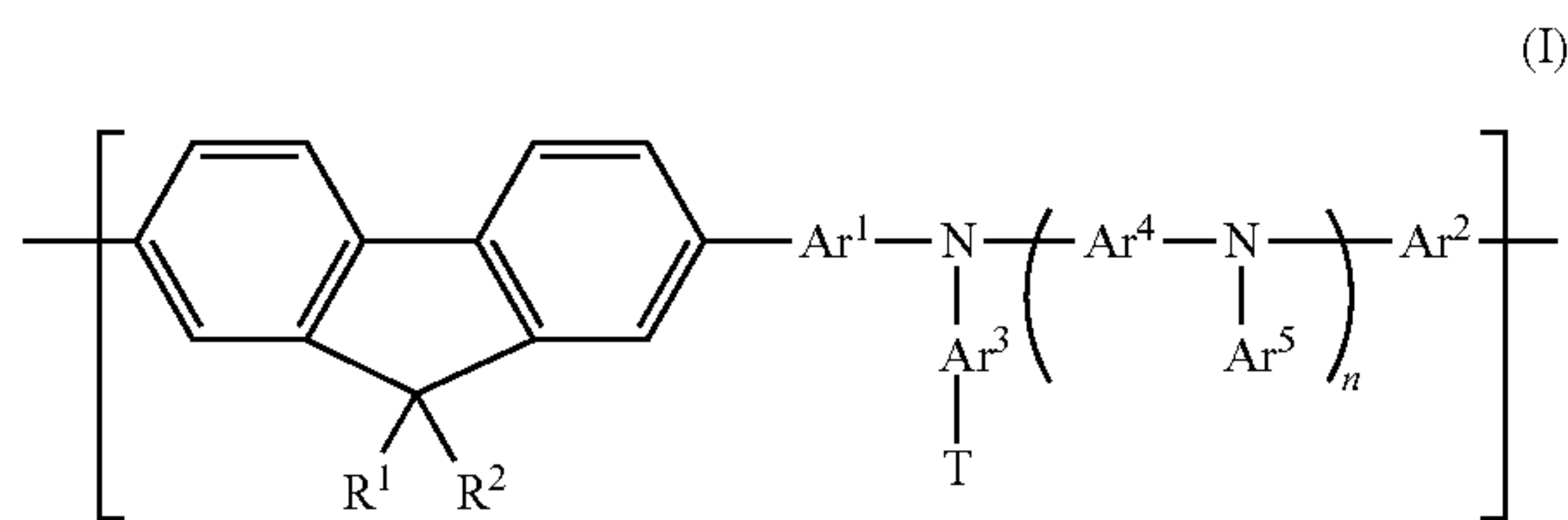
[Chemical Formula 12]
