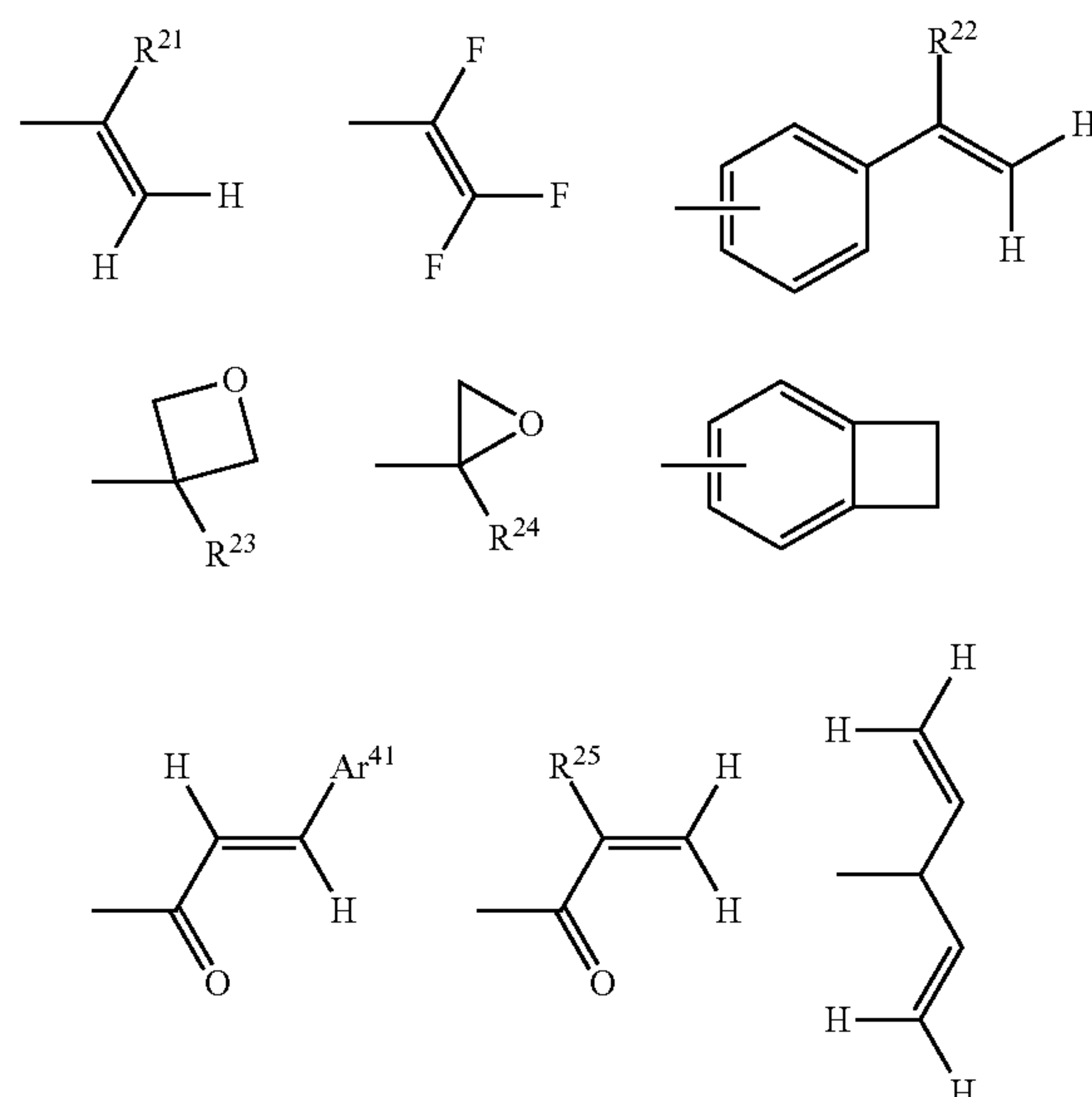
[Chemical Formula 6]
