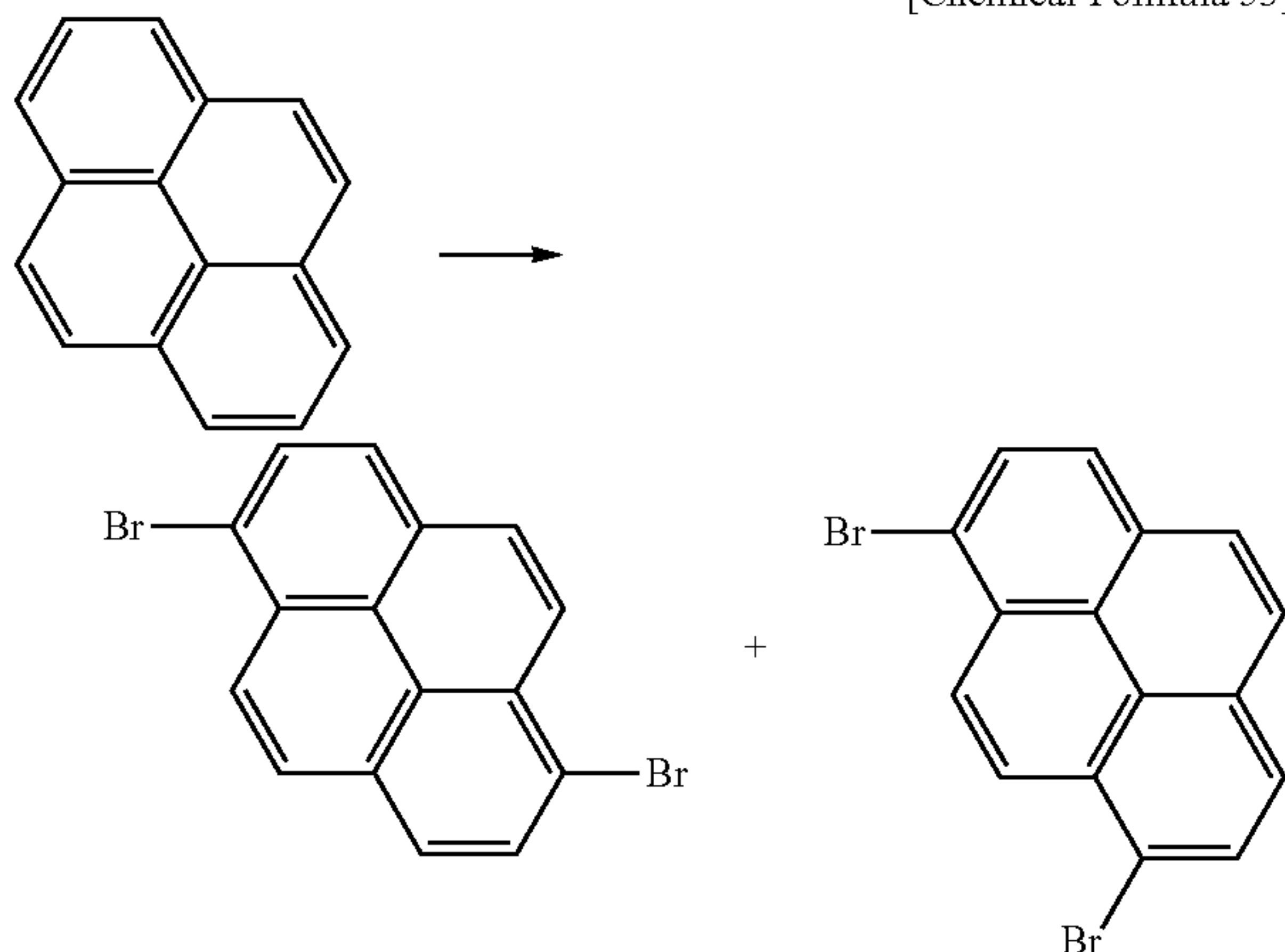
Product 4
