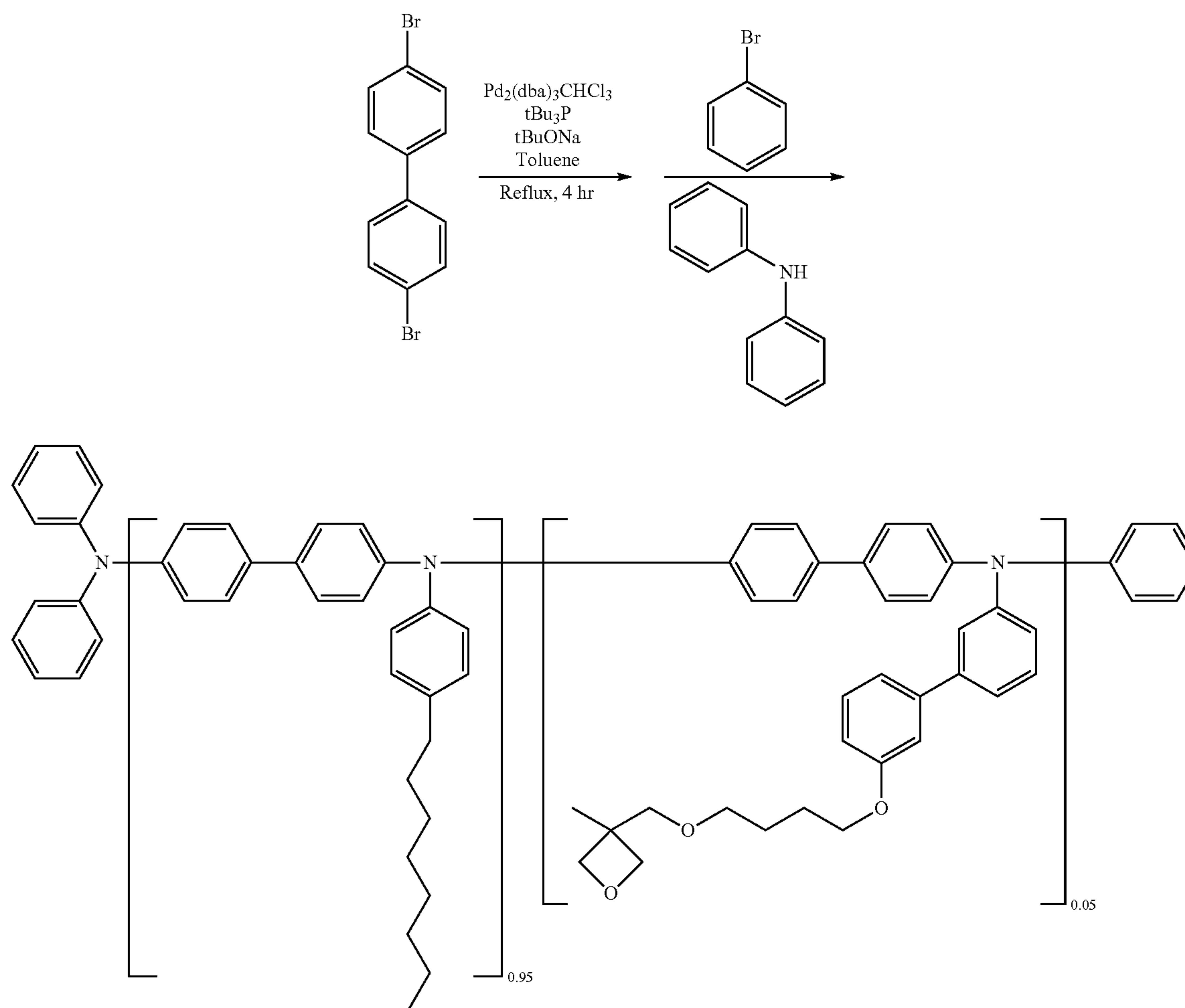
Comparative Polymer 2
