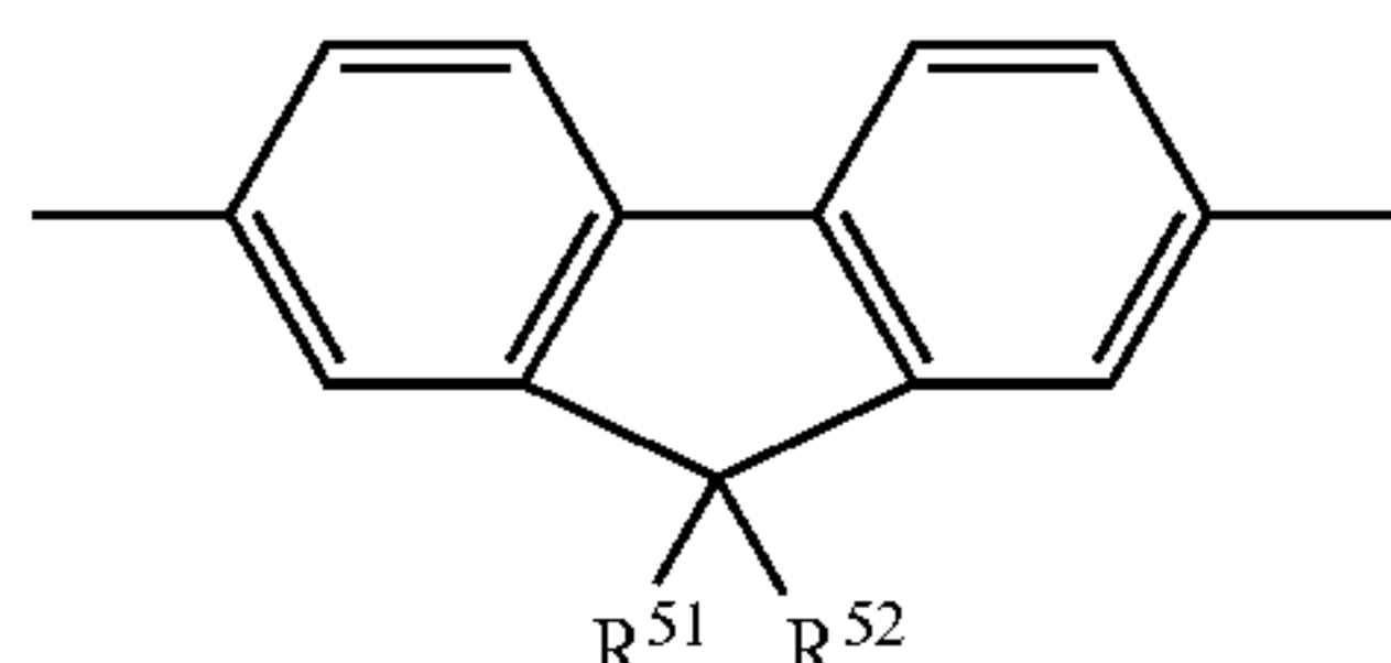
[Chemical Formula 40]
