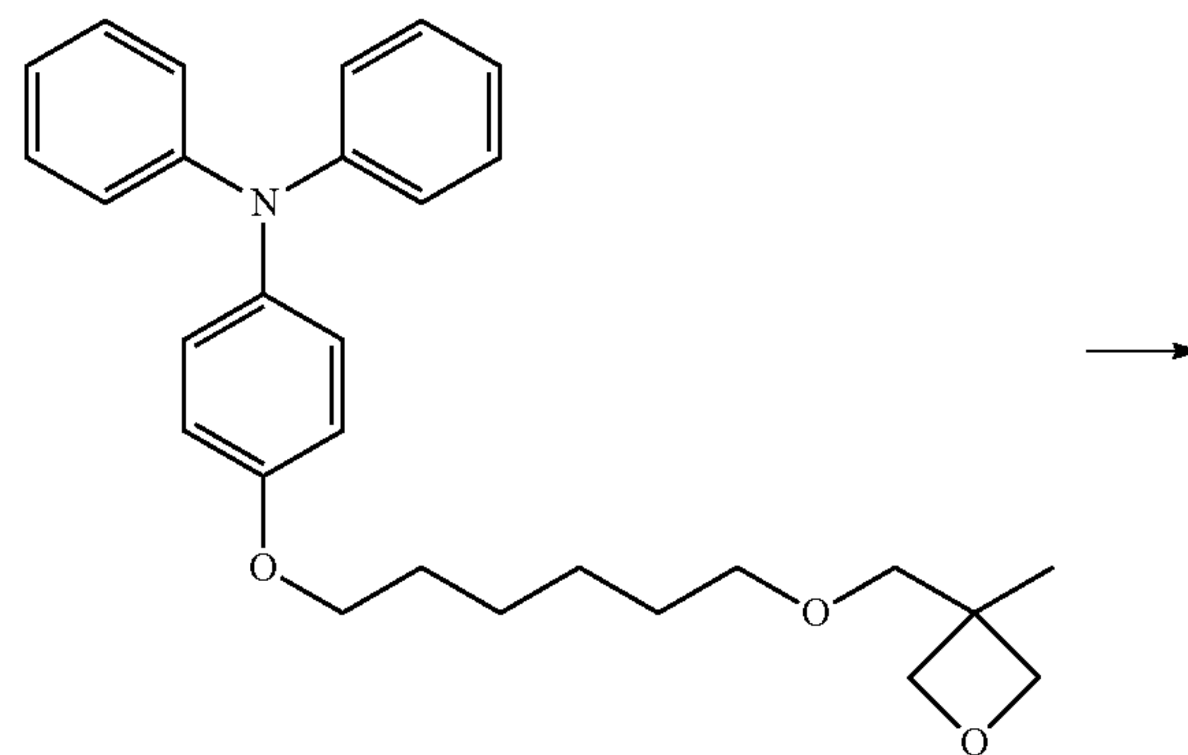
Product 2
