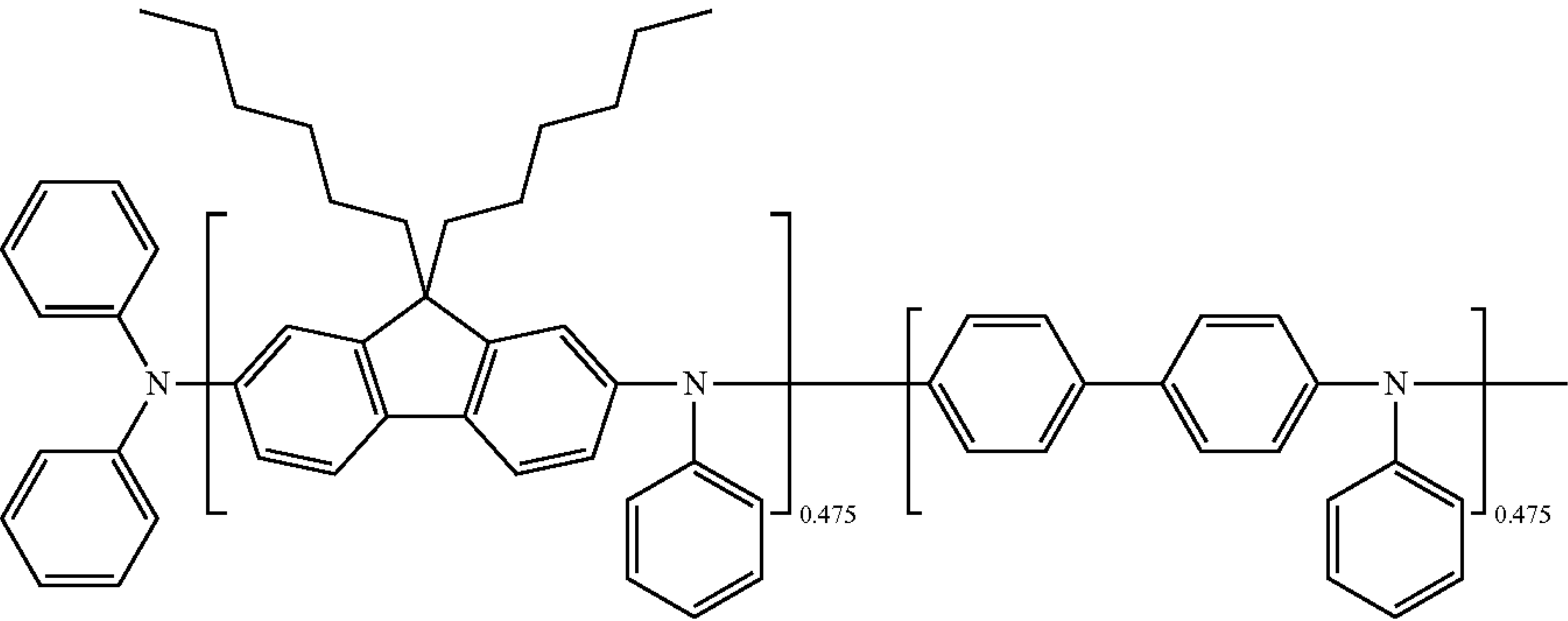
[Chemical Formula 105]
