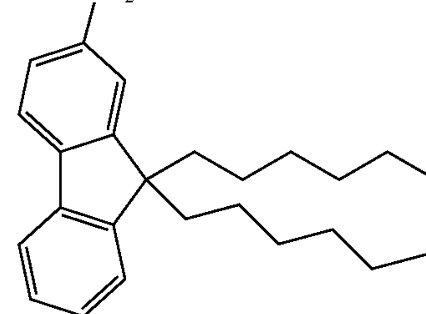
Product 8
