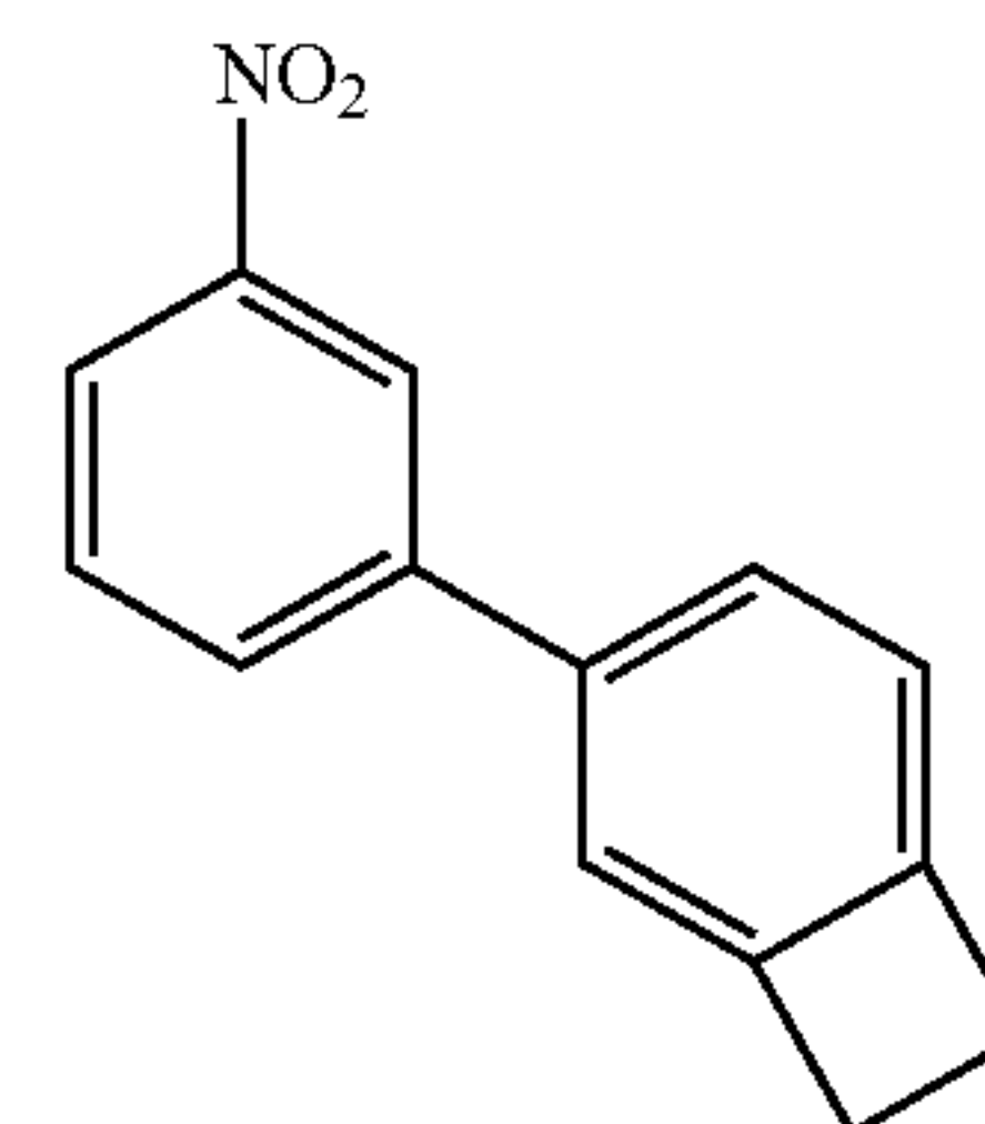
Product 5
