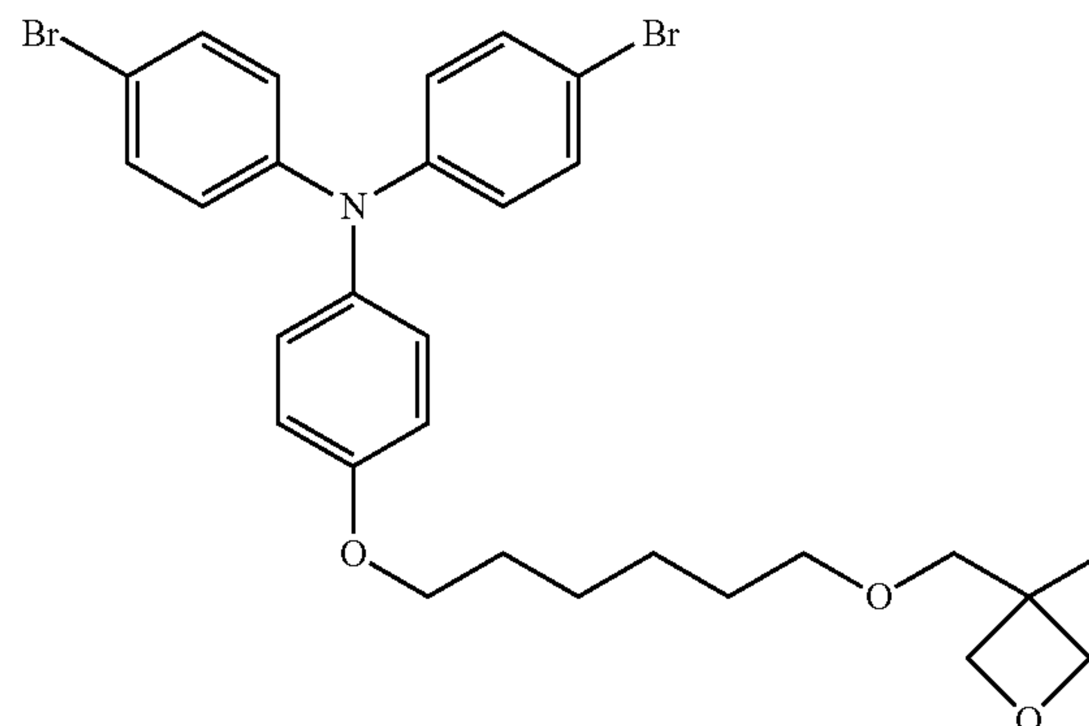
Product 3
