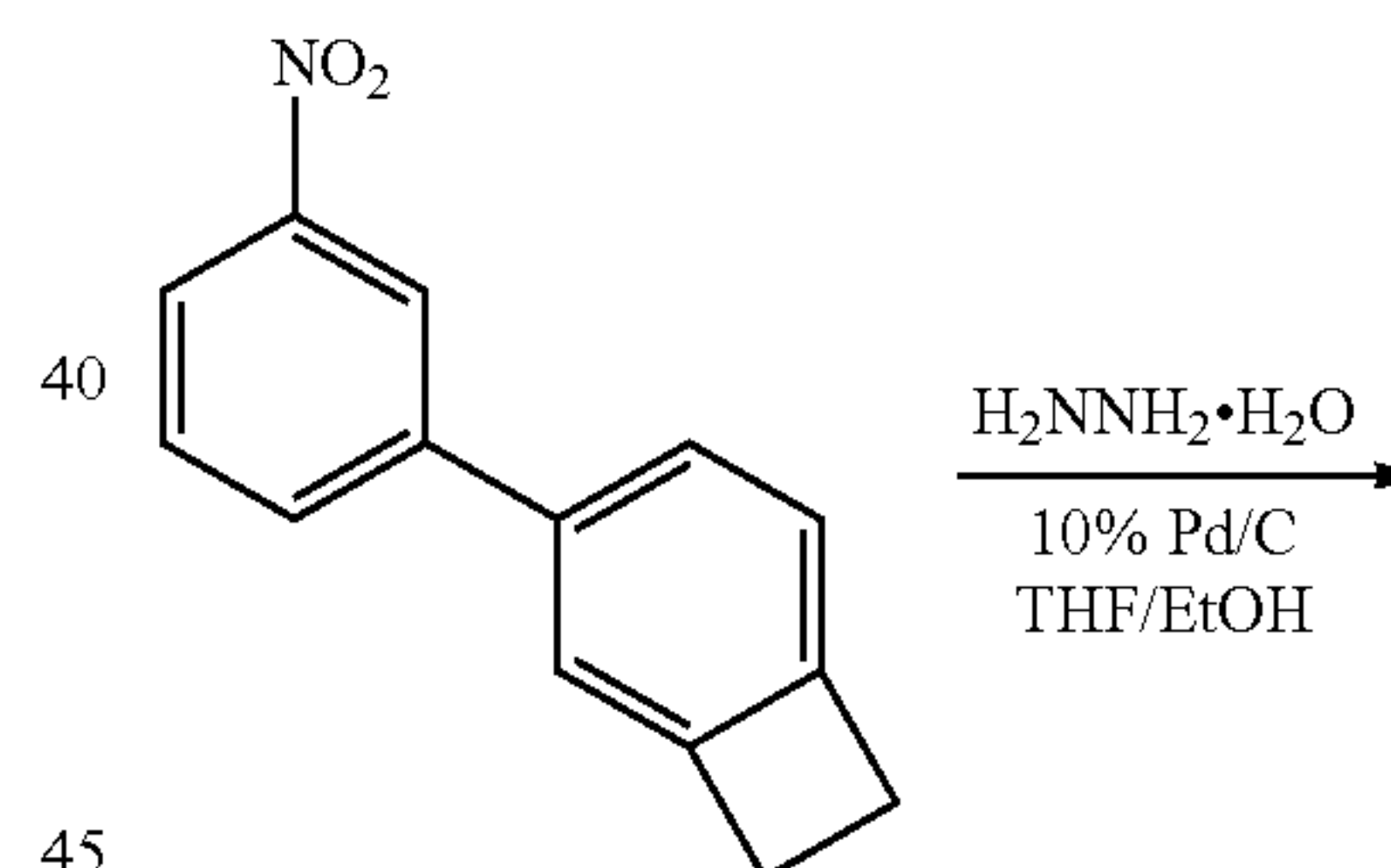
Product 5
