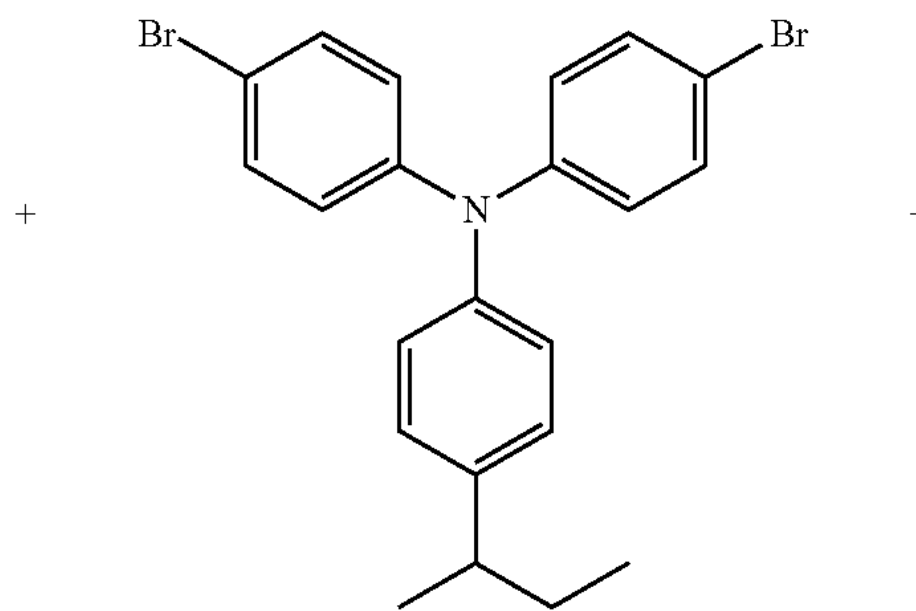
Compound 5
