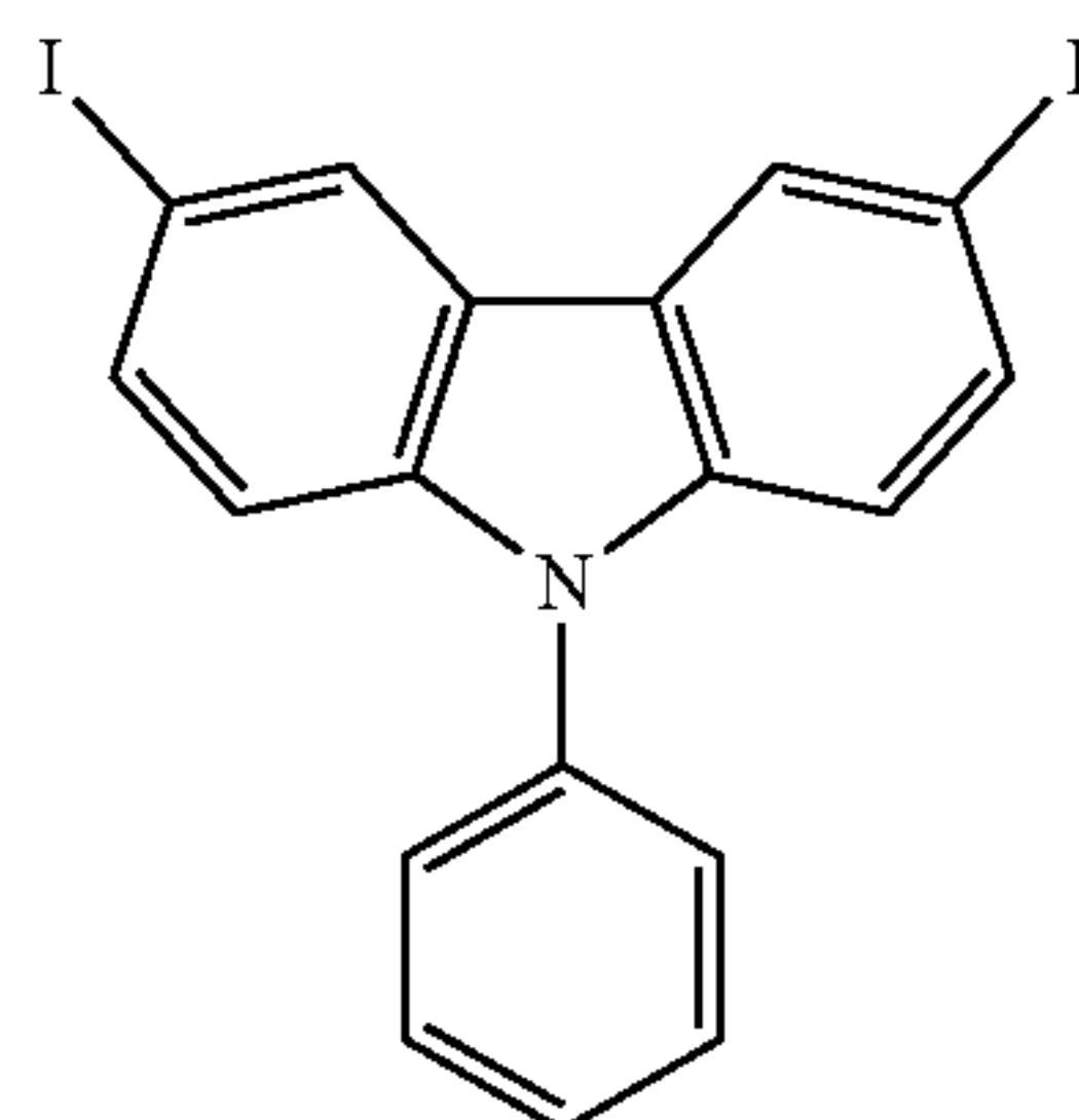
Product 29
