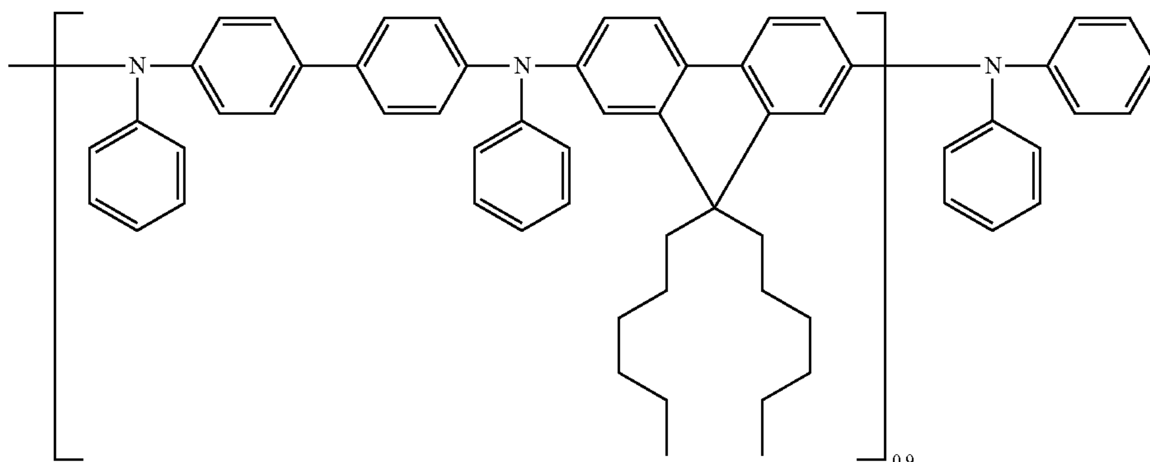
Comparative Polymer 3
