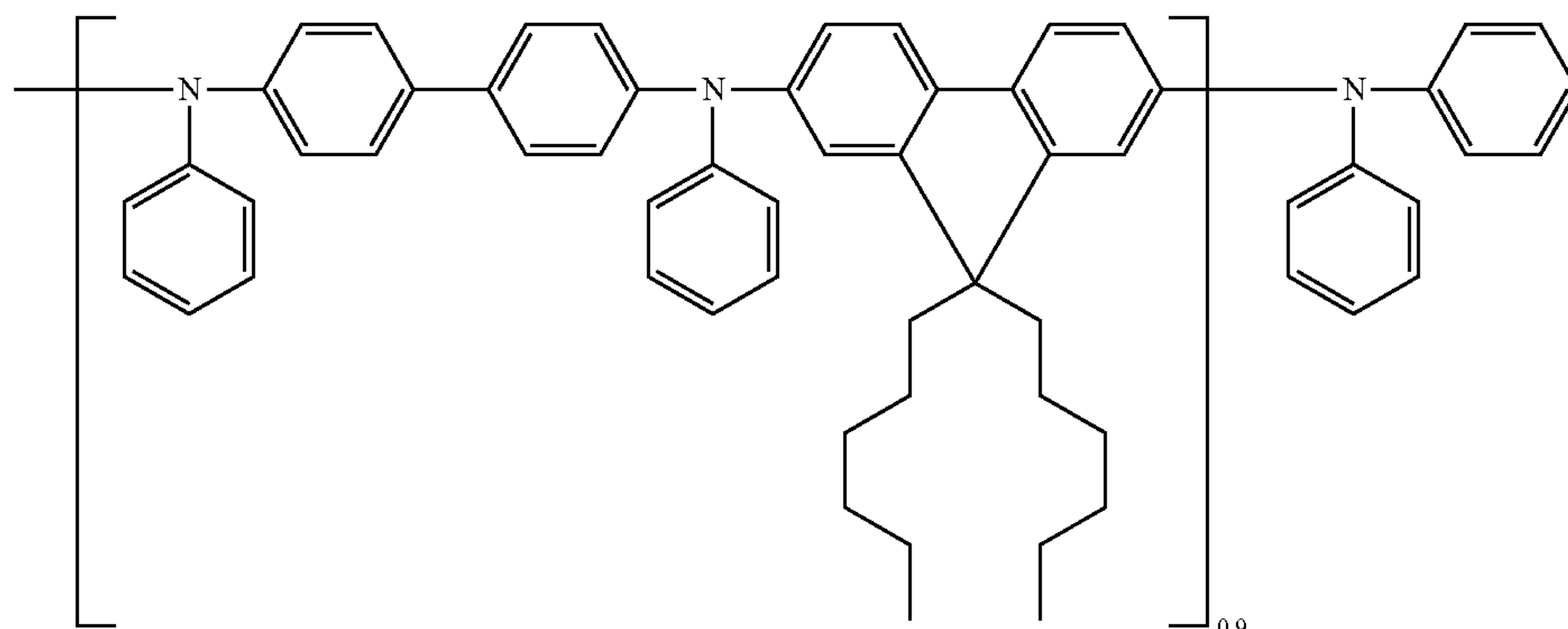
Comparative Polymer 3
