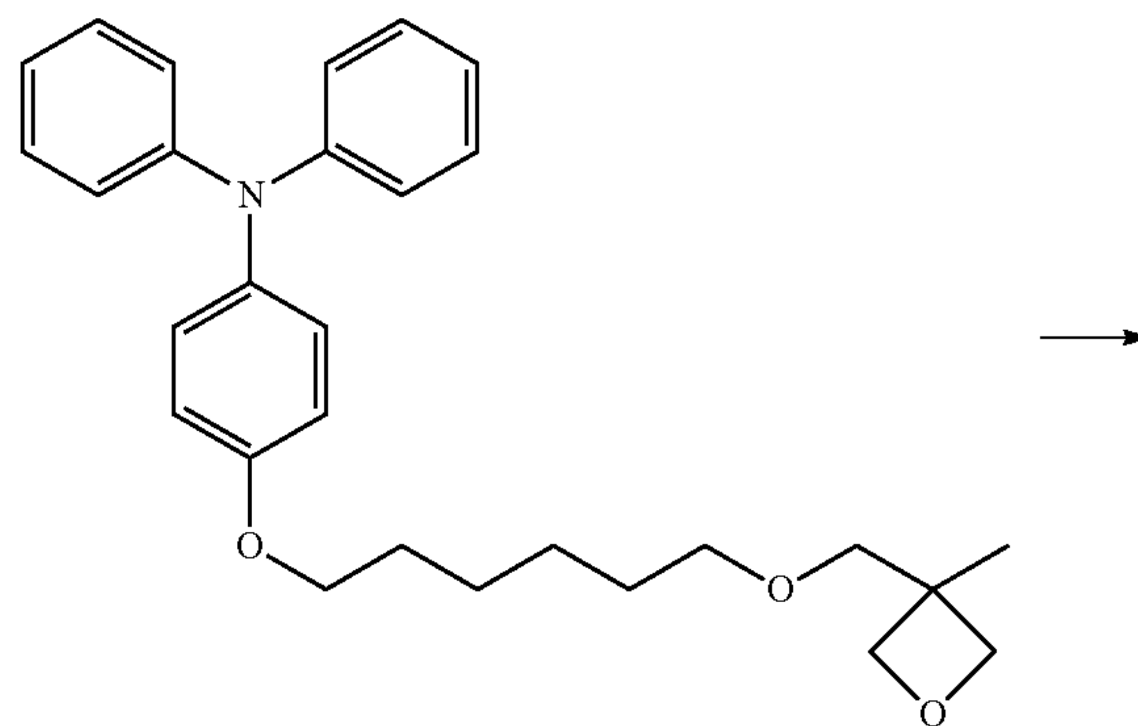
Product 2
