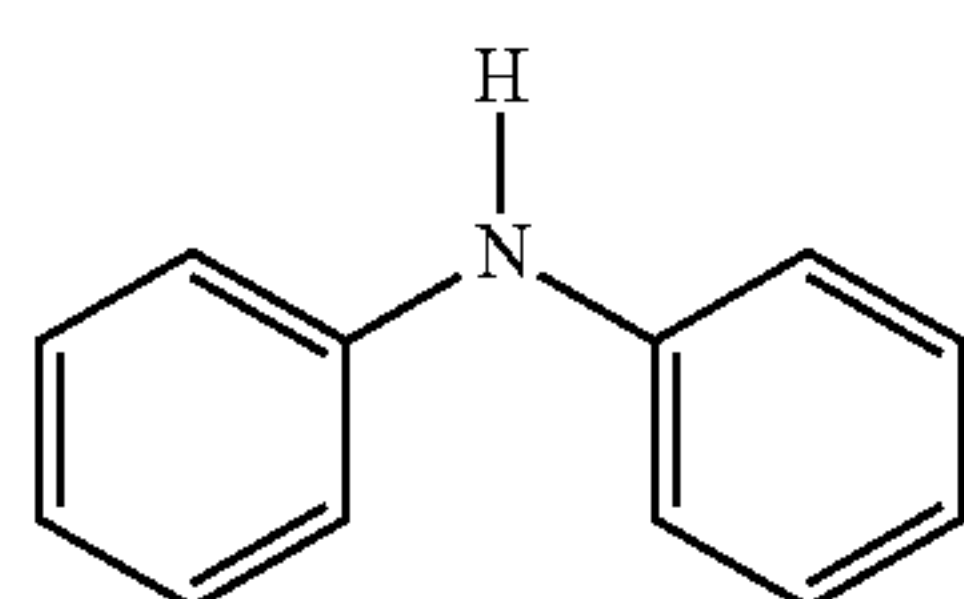
Compound 3
