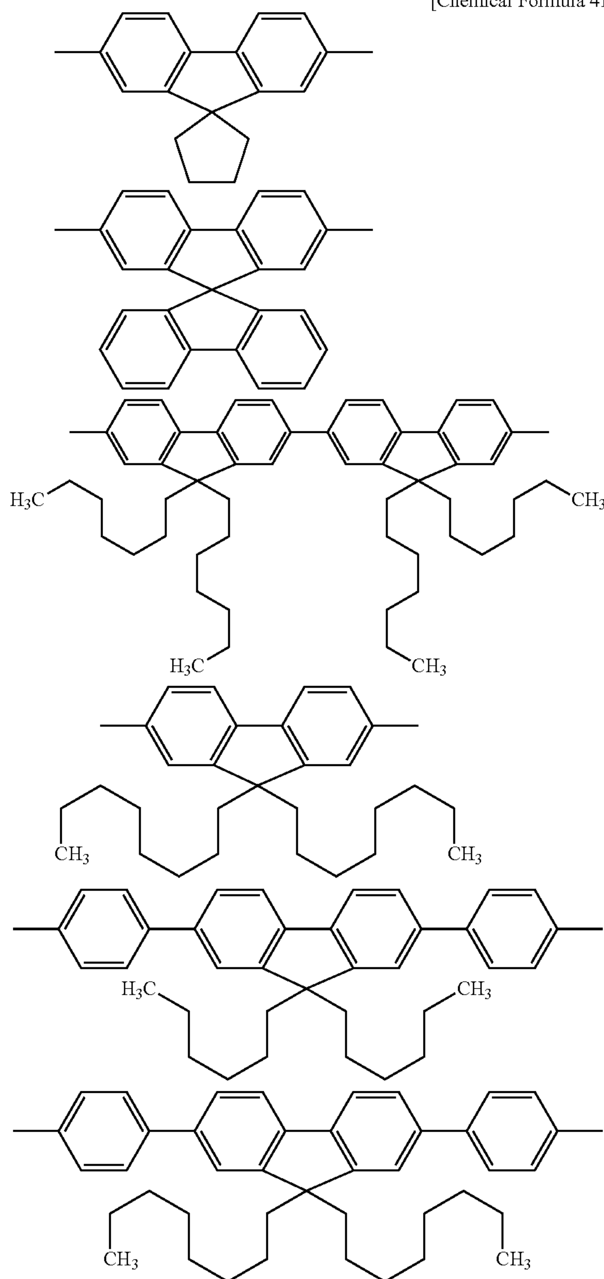
[Chemical Formula 41]
