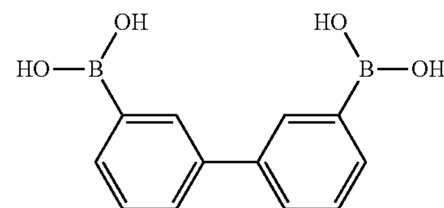
Product 31
