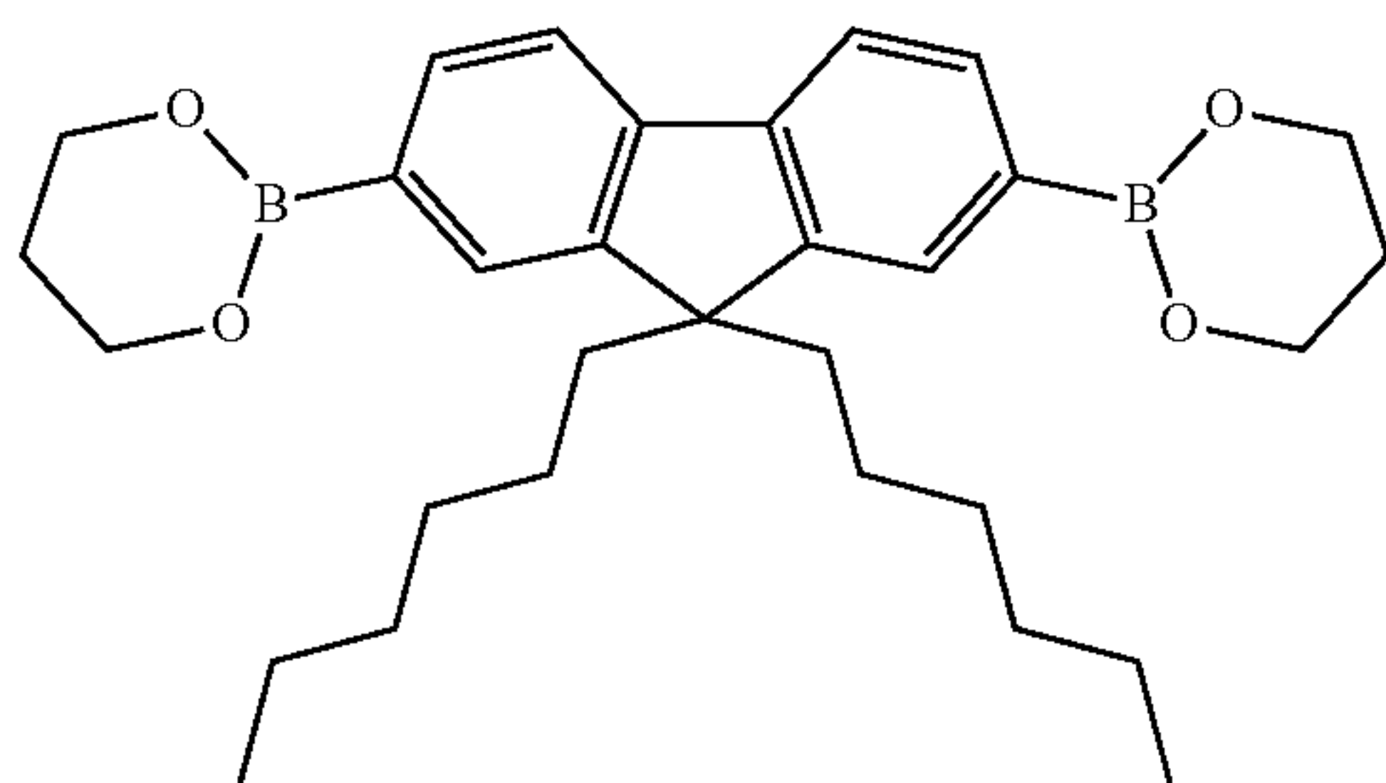
Compound 4
