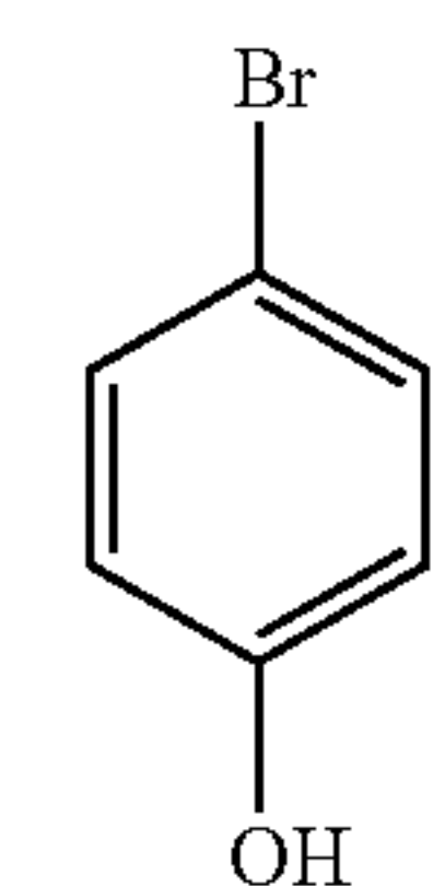
Compound 1
