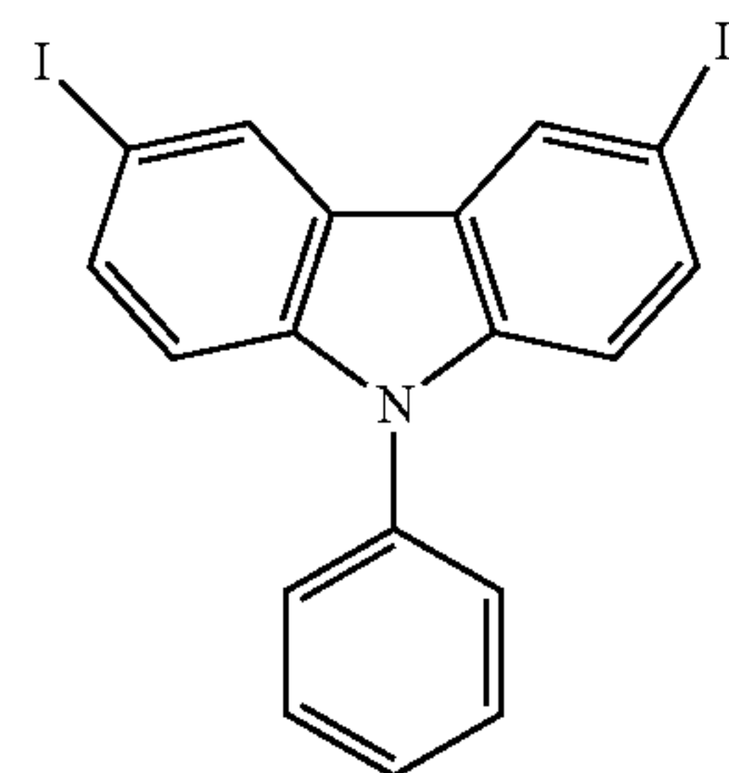
Product 29
