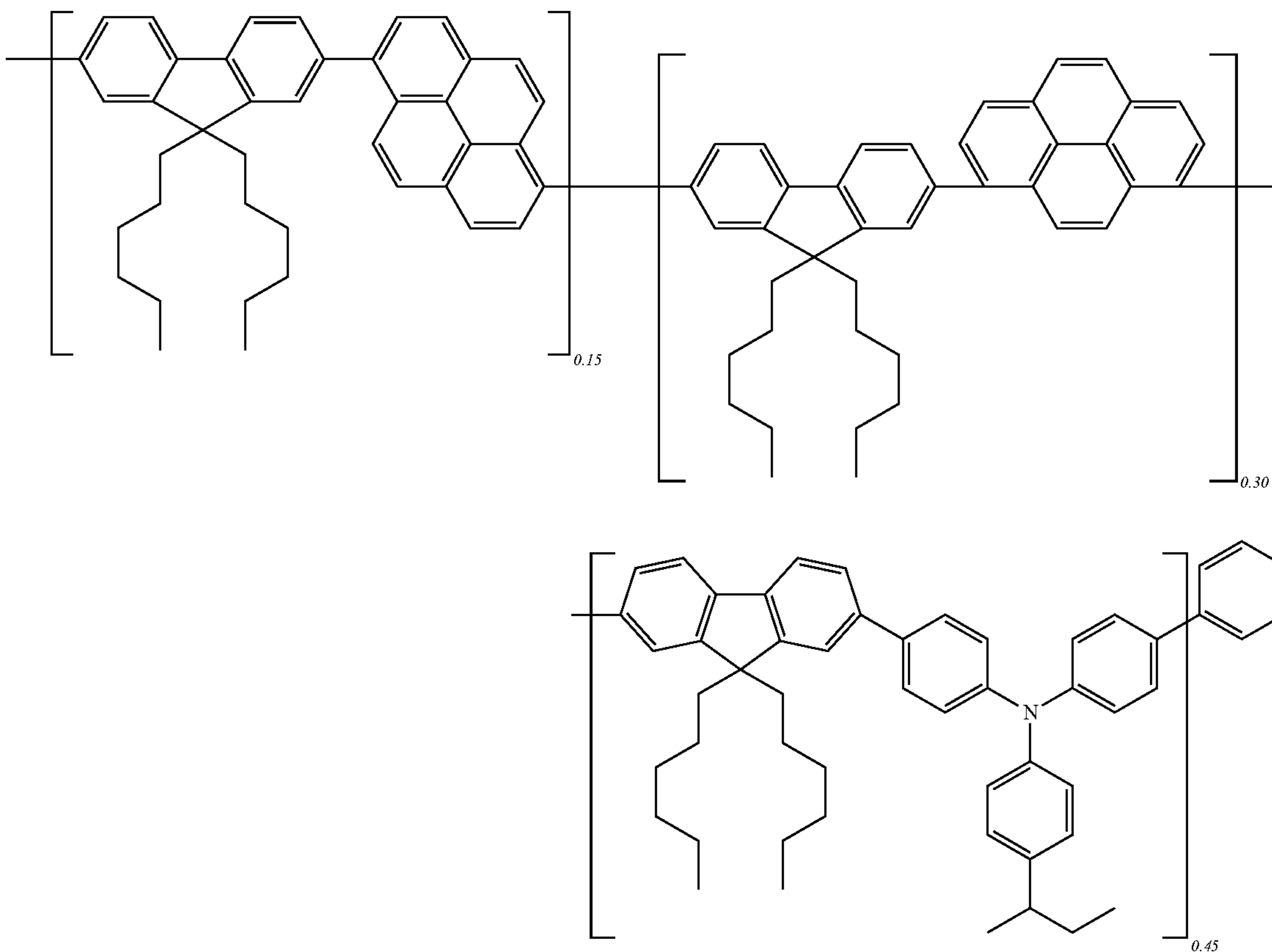
Comparative Polymer 1
