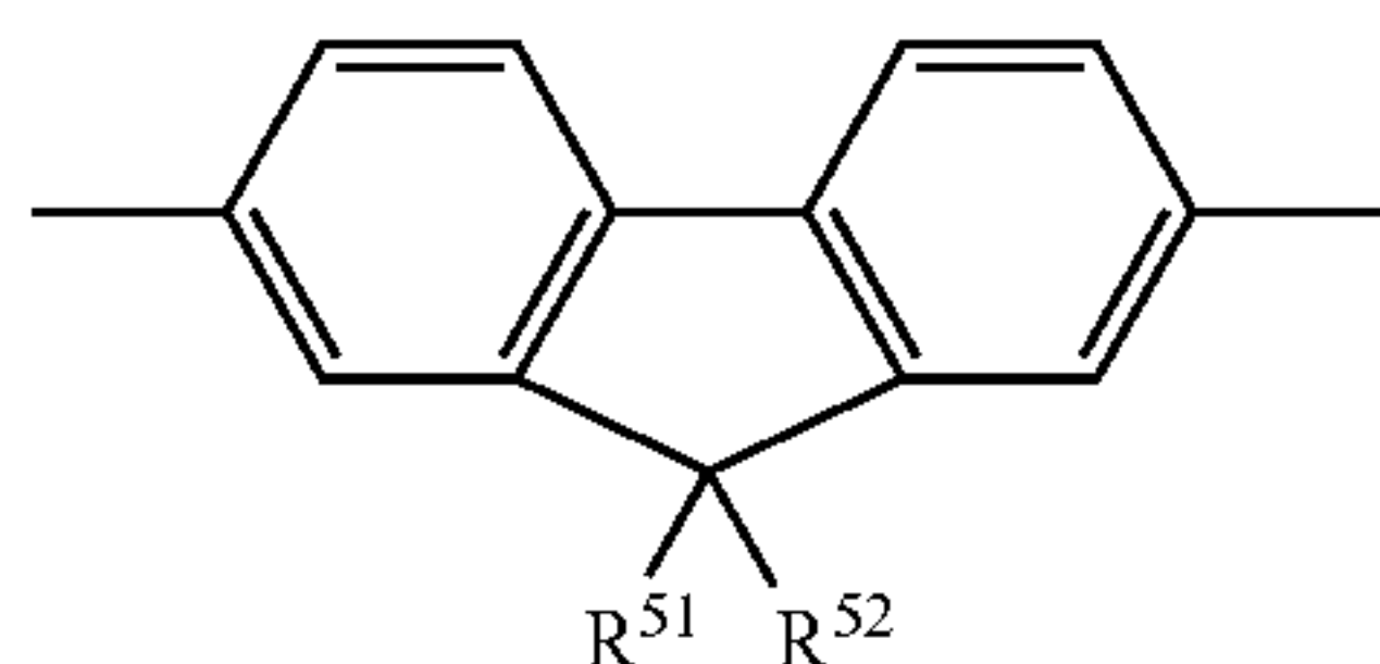
[Chemical Formula 40]
