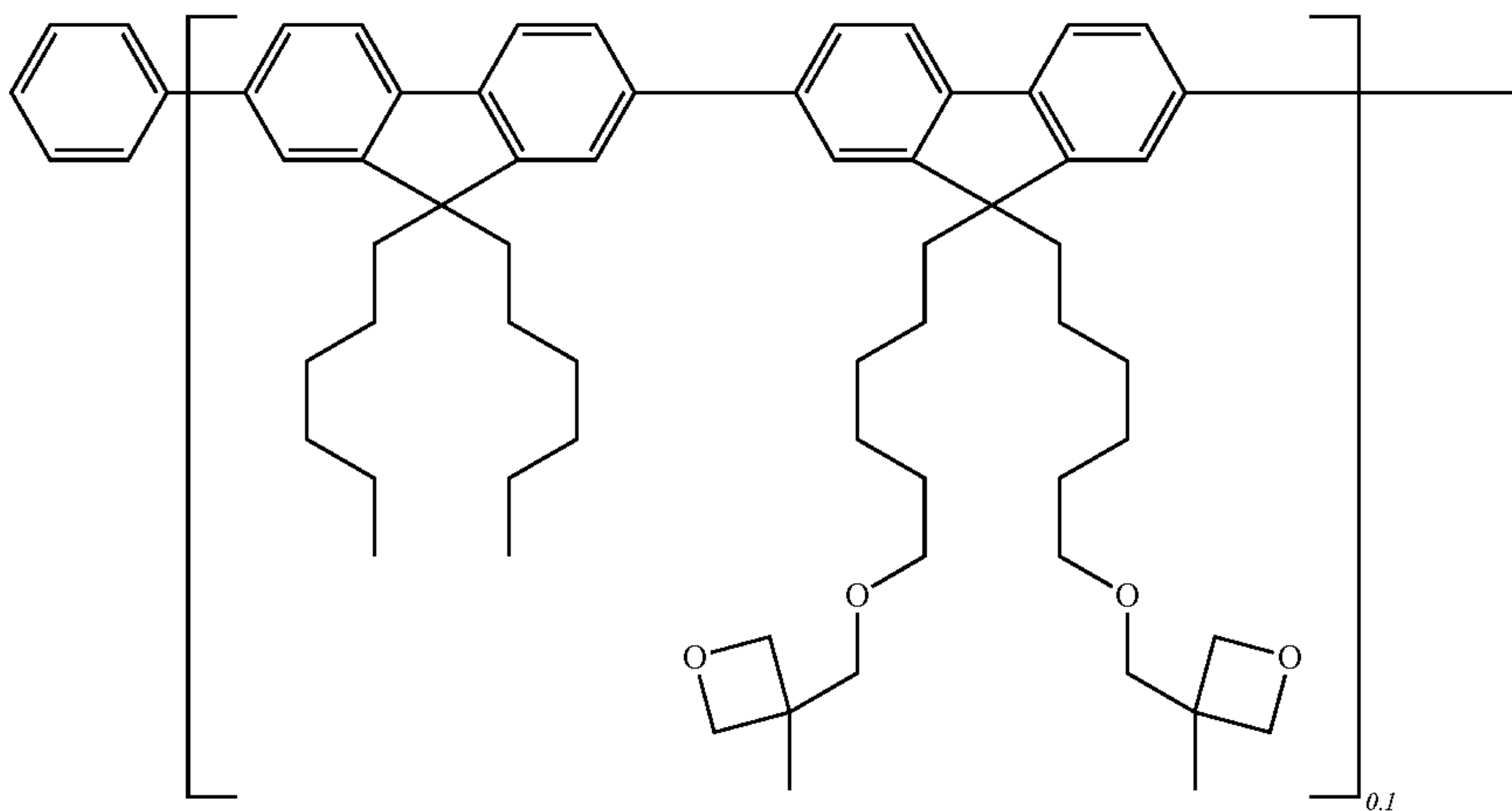
Comparative Polymer 1
