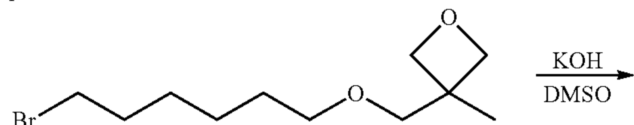
Compound 1
