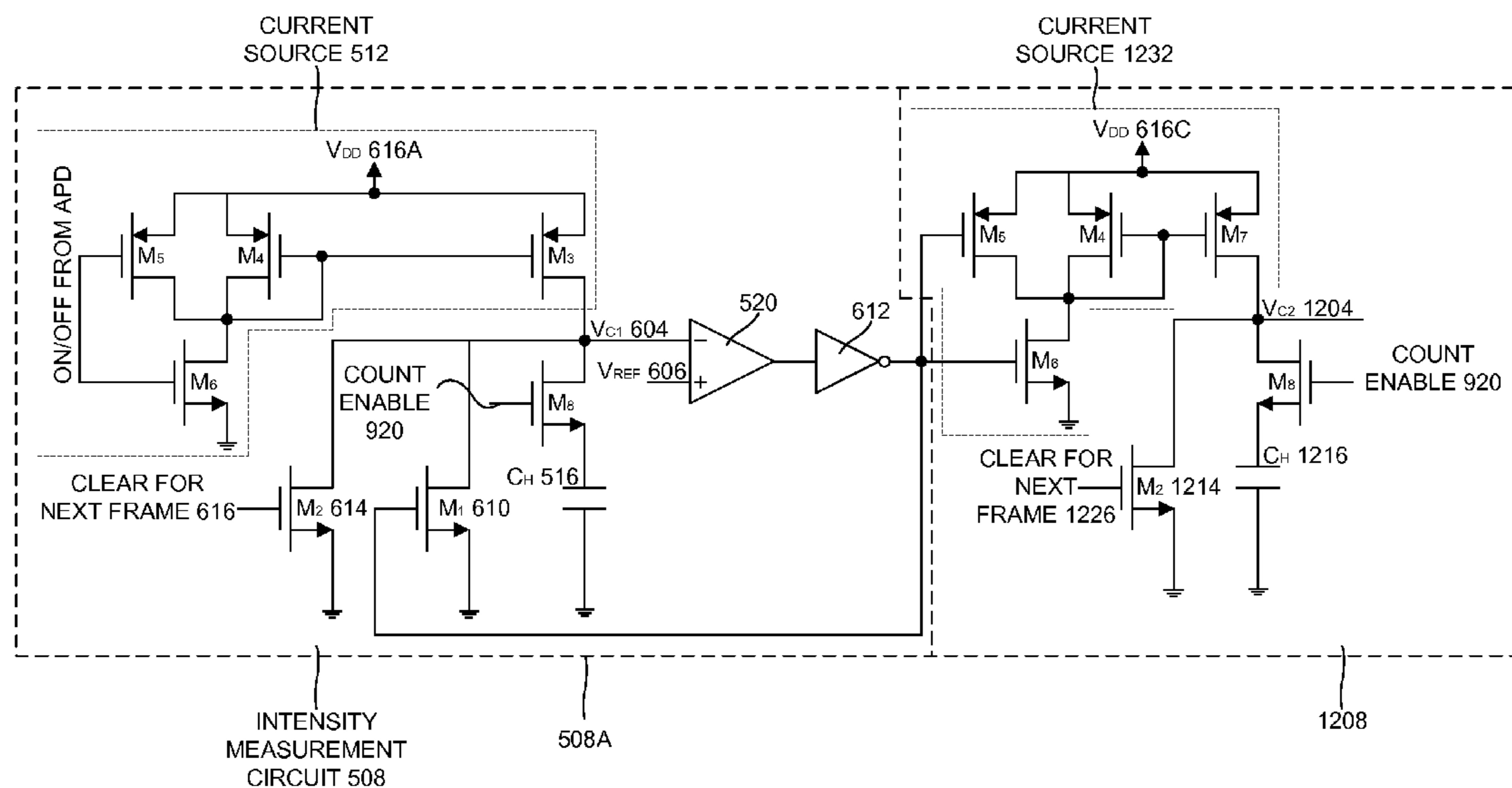
EXAMPLE EMBODIMENT CASCADED MODE WITH TWO COUNTERS 1200
