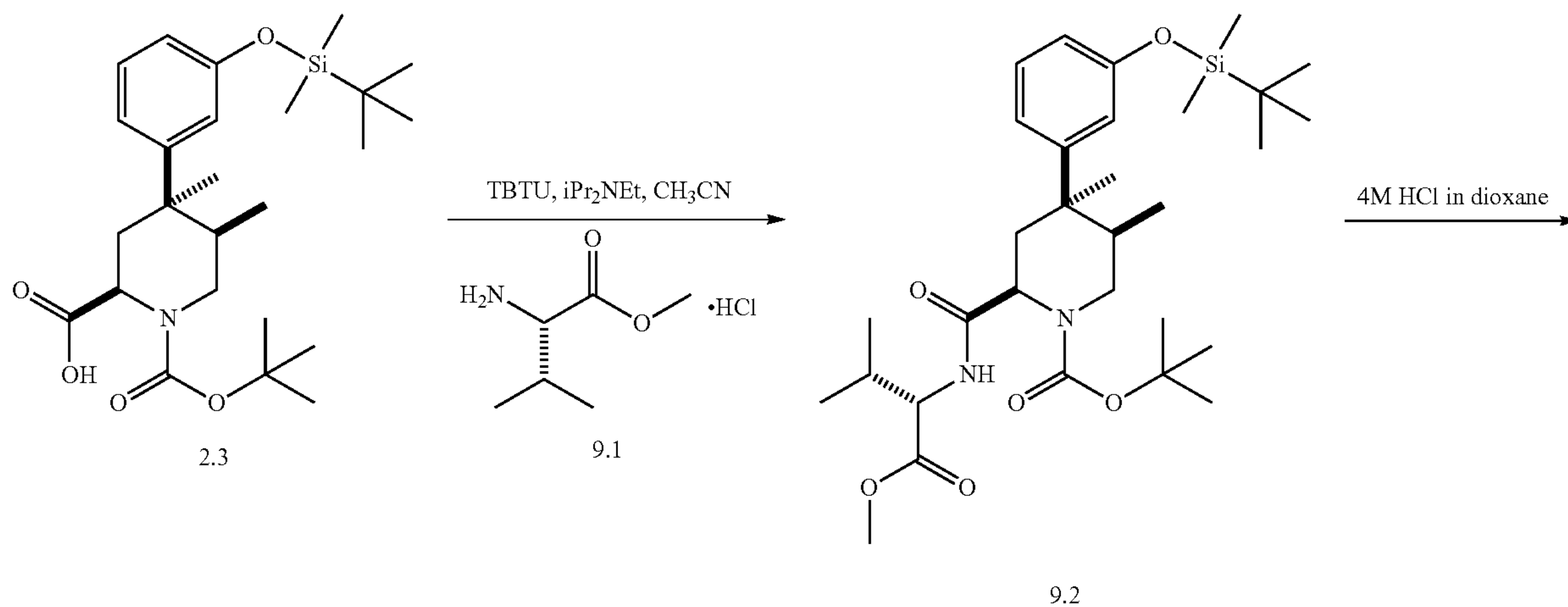
Scheme 9
