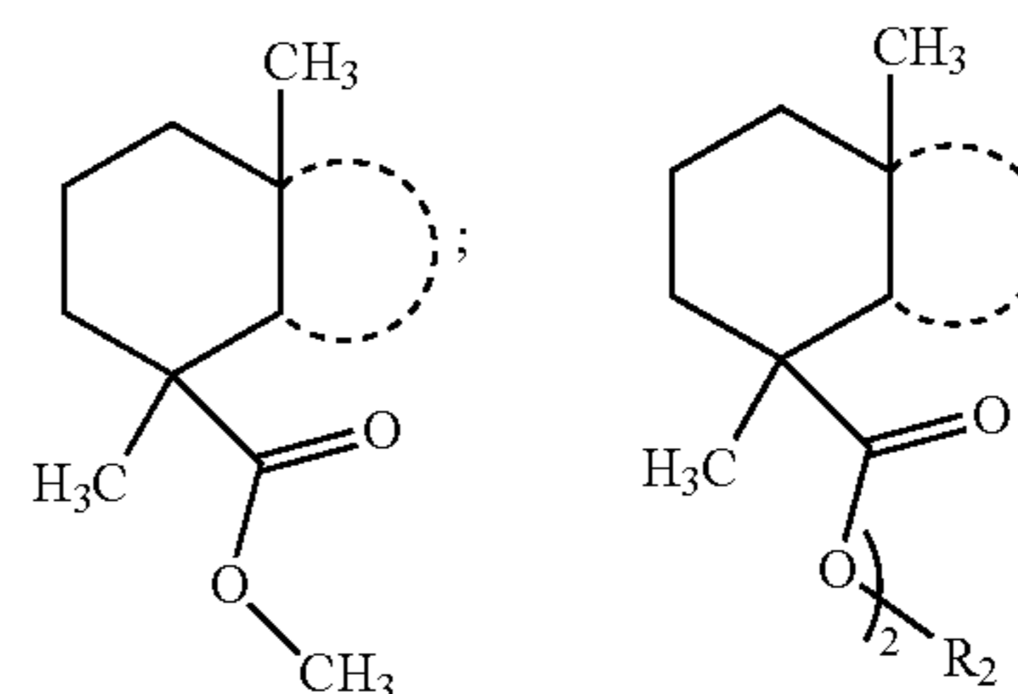
ester derived from diol
