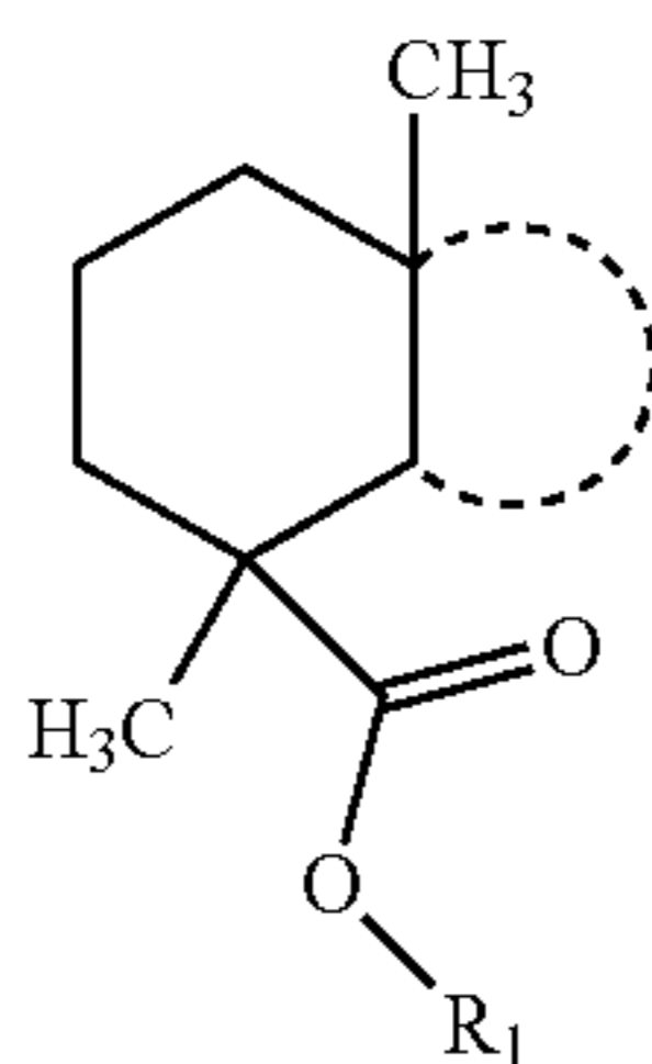
ester derived from monoalcohol
