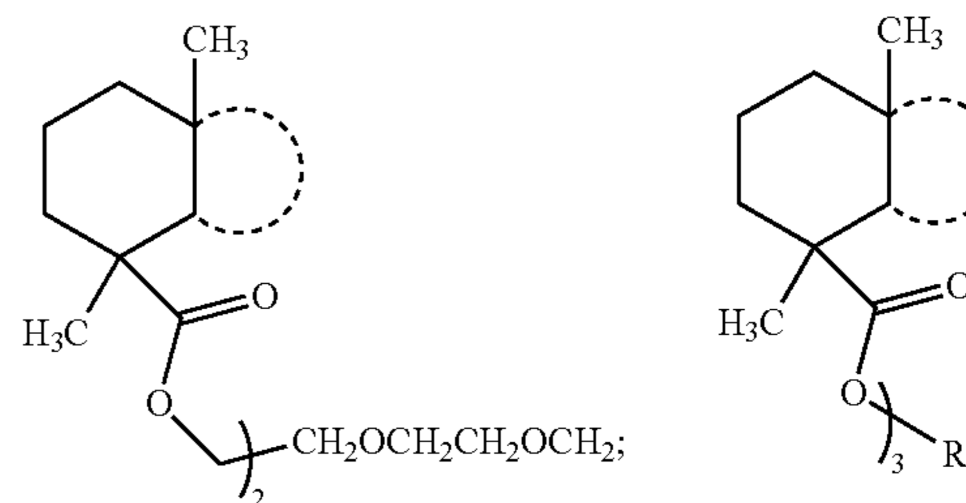
ester derived from triol
