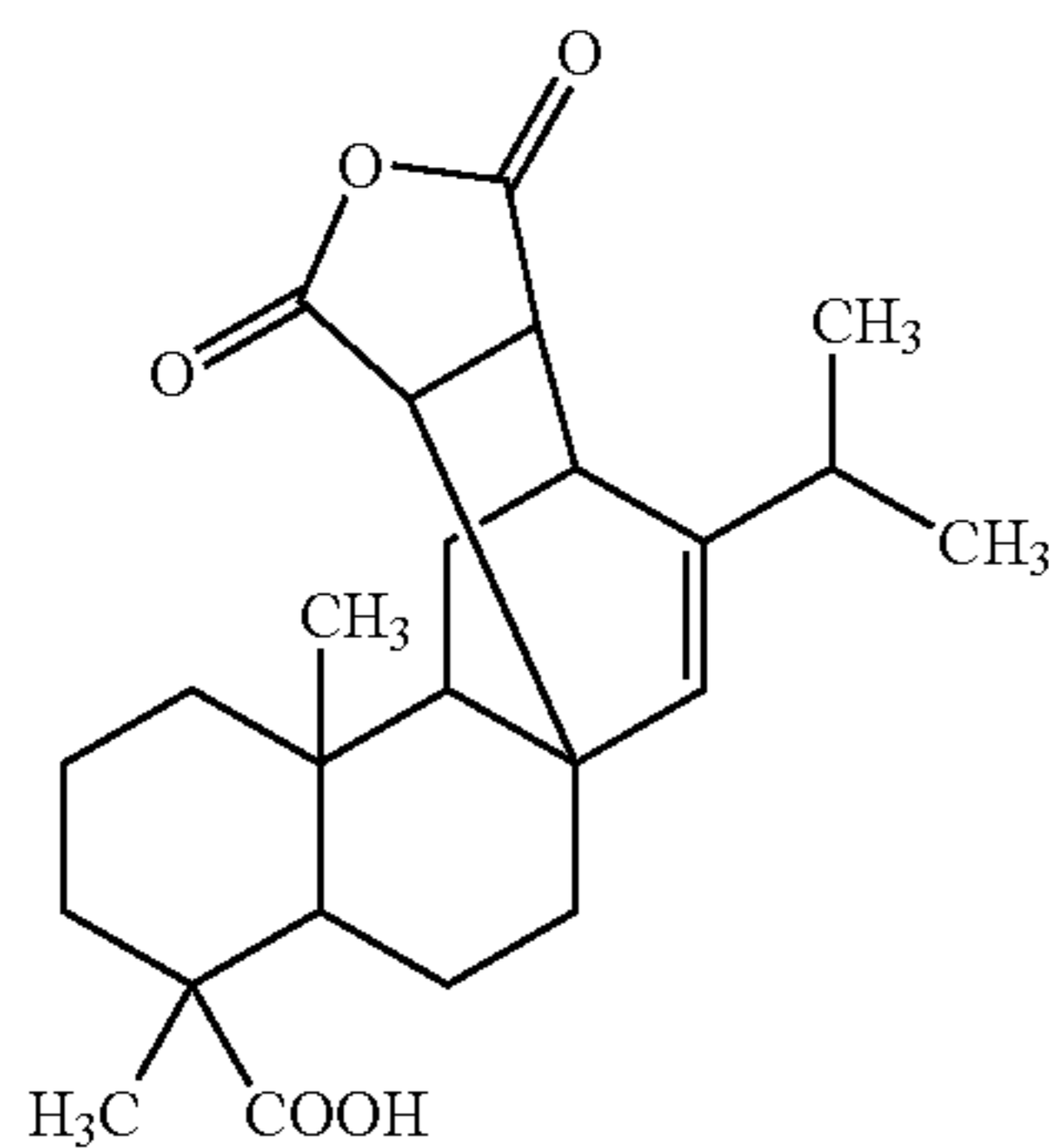
Maleic Anhydride-Modified Abietic Acid
