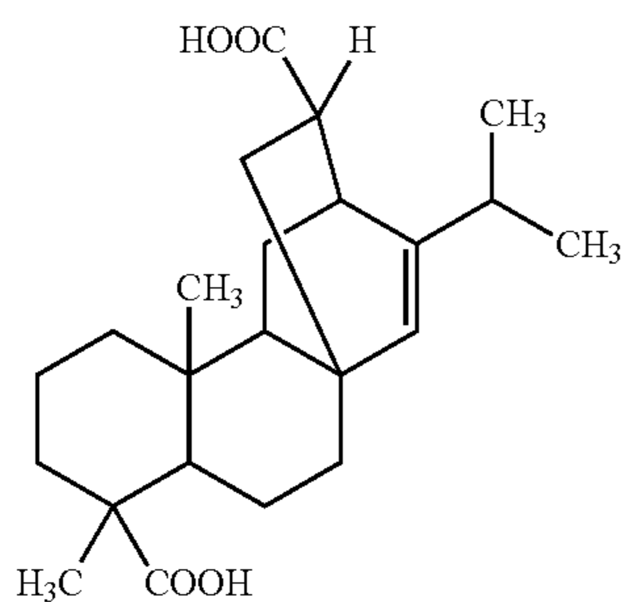
Acrylic Acid-Modified Abietic Acid
