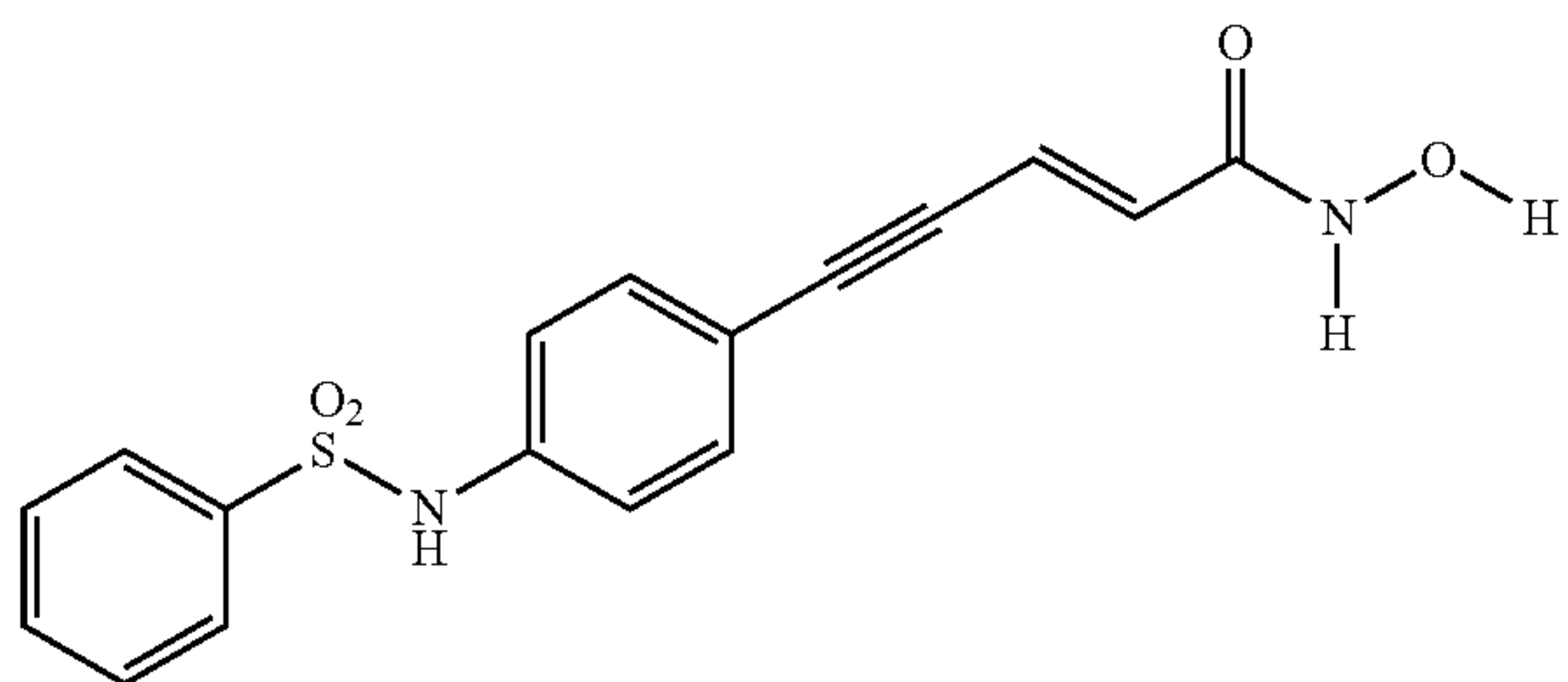
8, Oxamflatin
