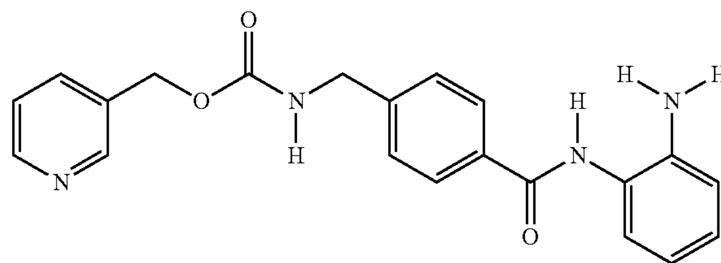
13, MS-275
