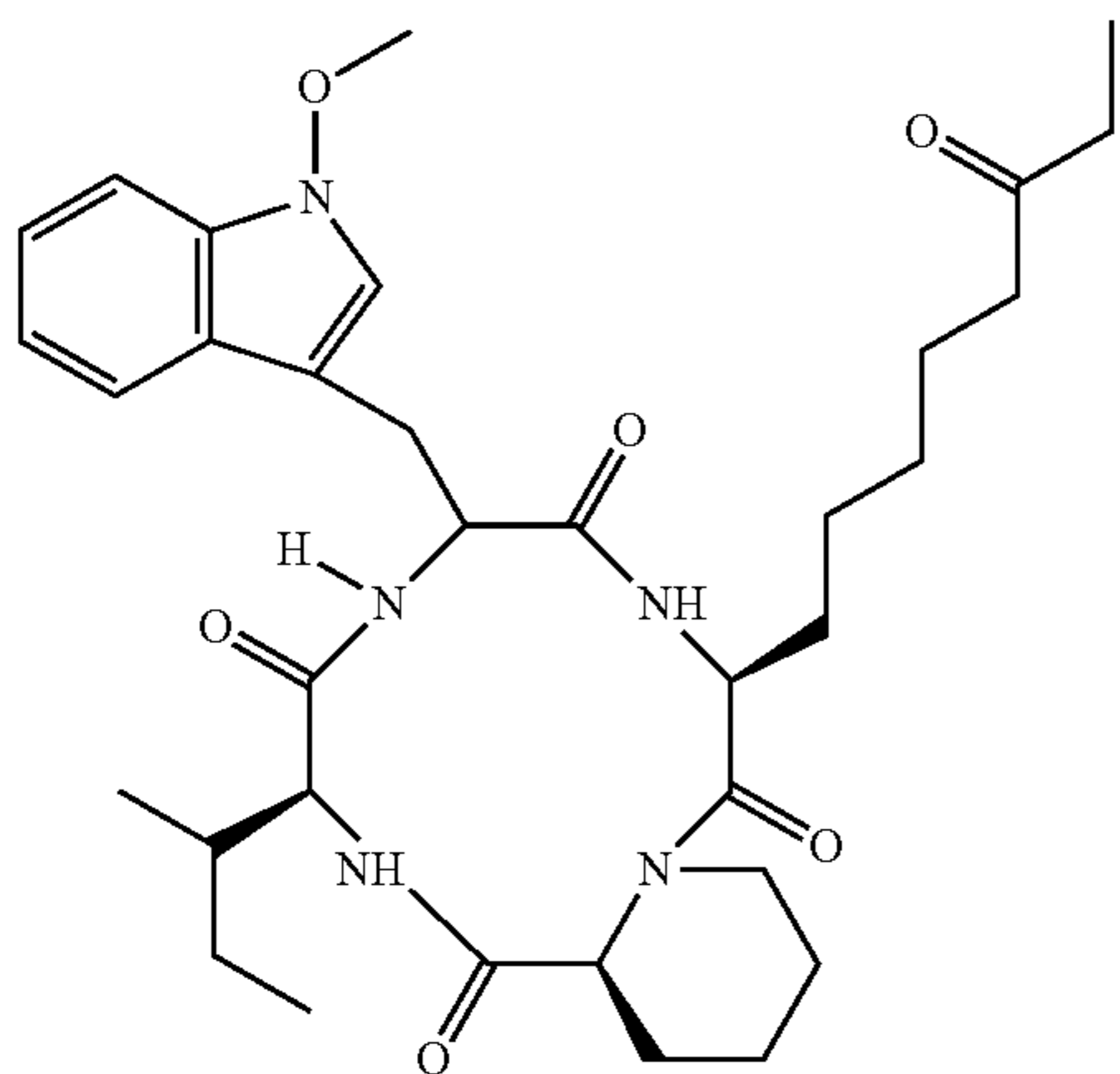
10, Apicidin
