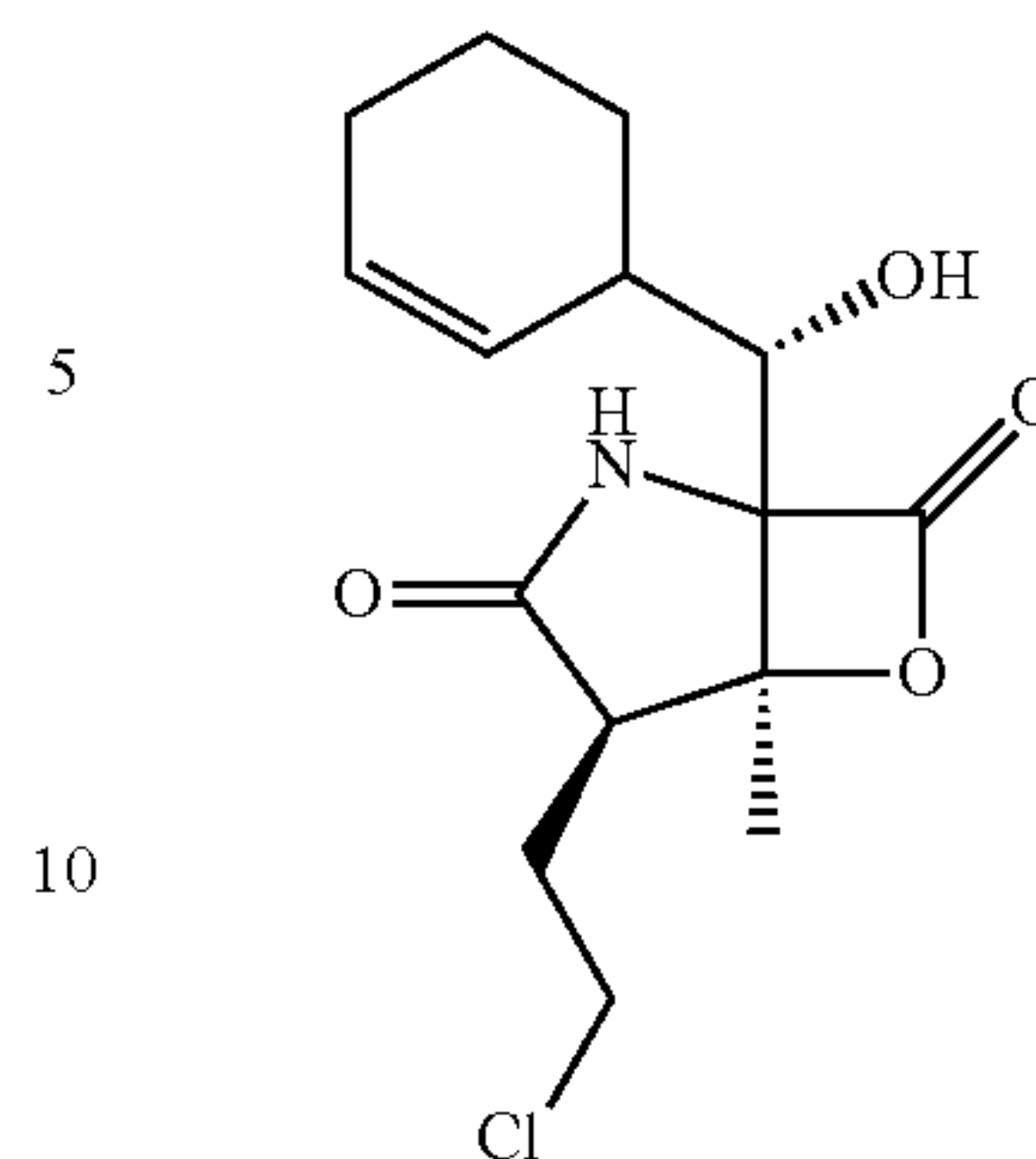
(4R,5S)-4-(2-chloroethyl)-1-((1S)-cyclohex-2-enyl(hydroxy)methyl)-5-methyl-6-oxa-2-azabicyclo[3.2.0]heptane-3,7-dione
