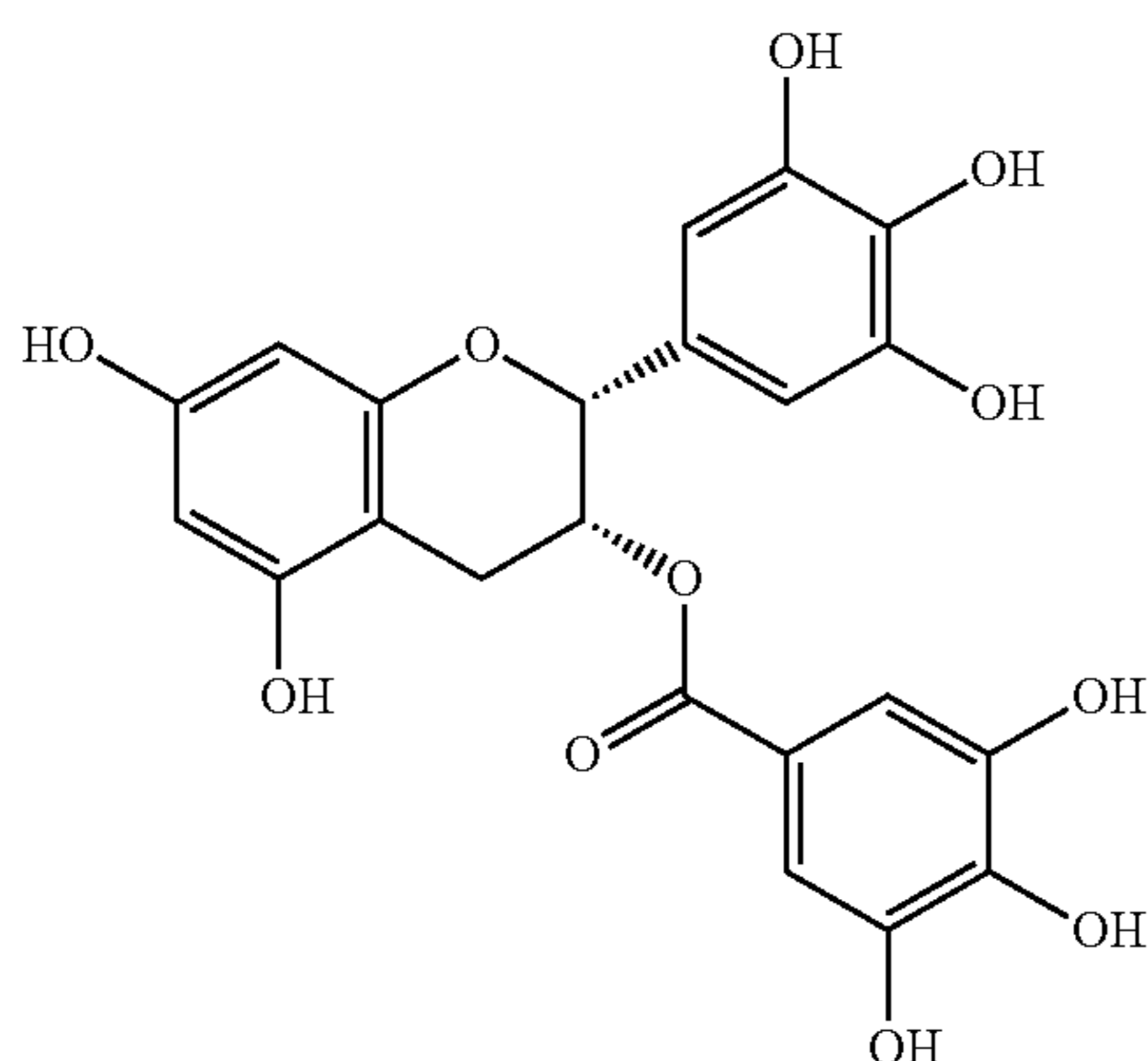
[(2R,3R)-5,7-dihydroxy-2-(3,4,5-trihydroxyphenyl)chroman-3-yl]3,4,5-trihydroxybenzoate
