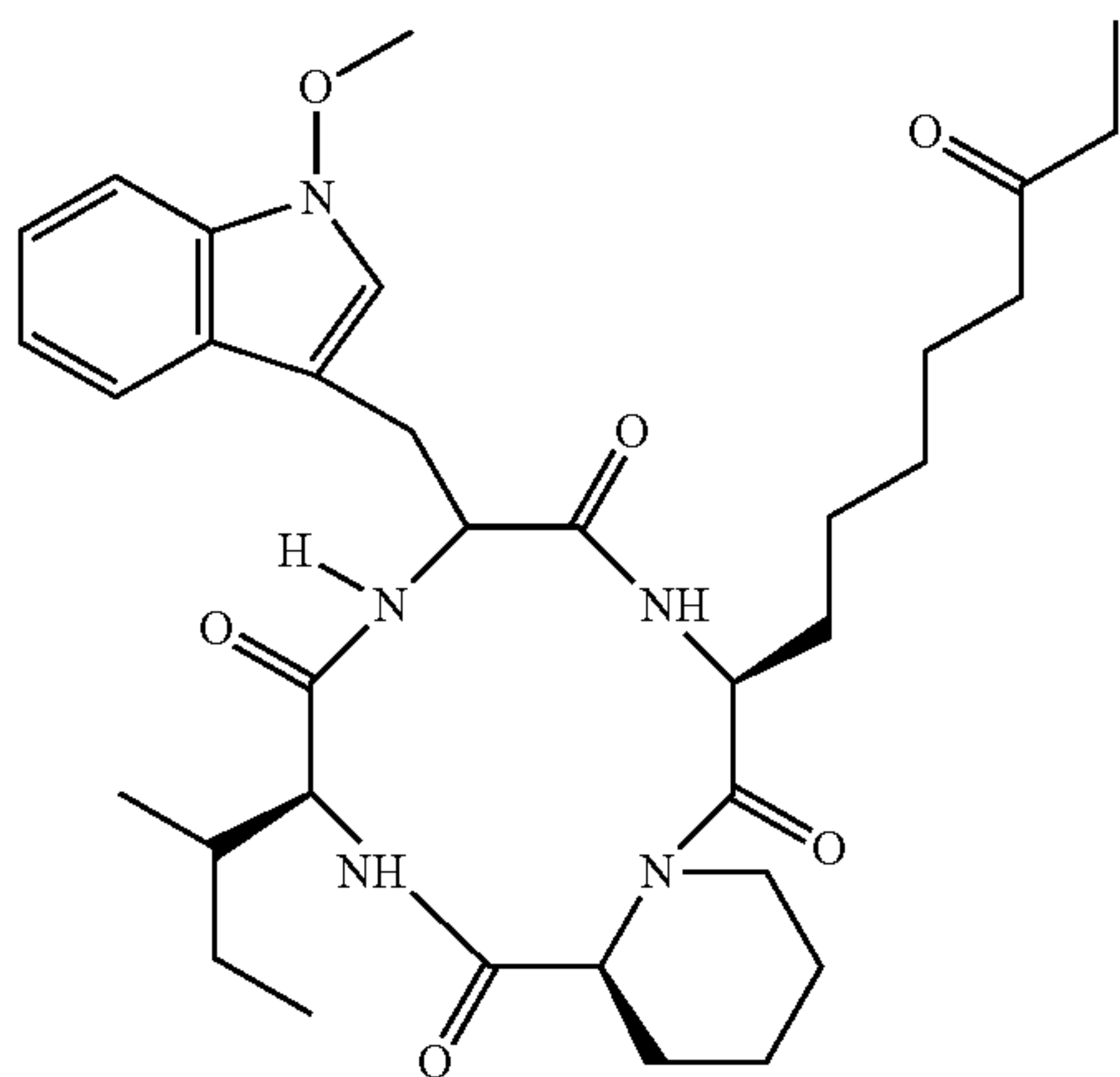
10, Apicidin
