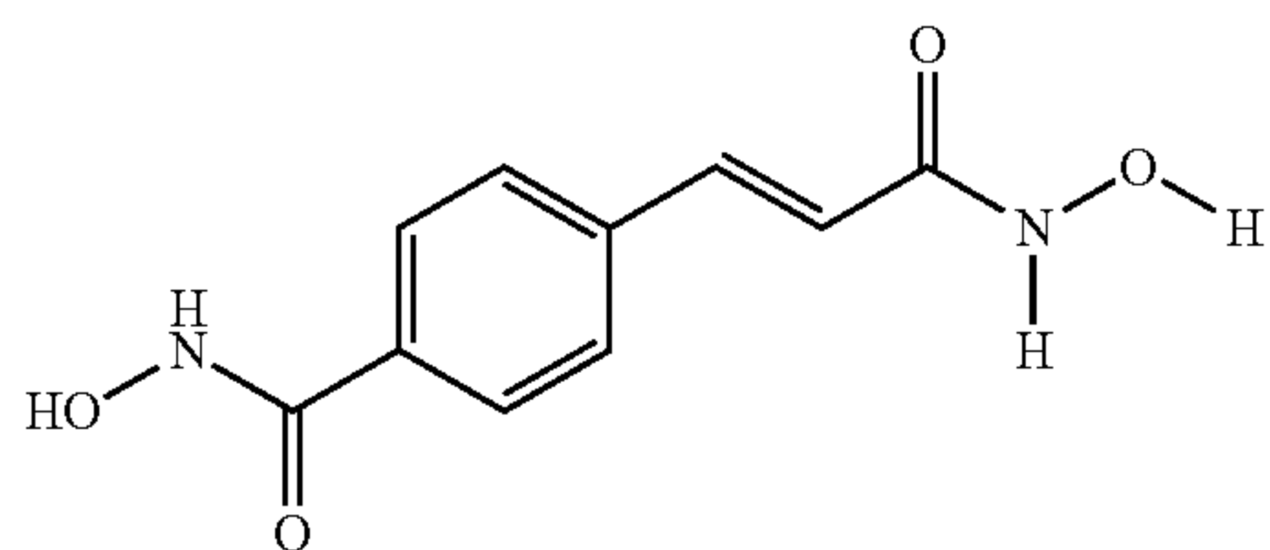
7, CBHA
