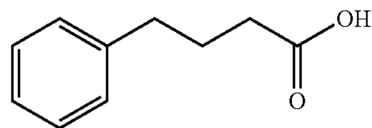
12, Phenylbutyric acid
