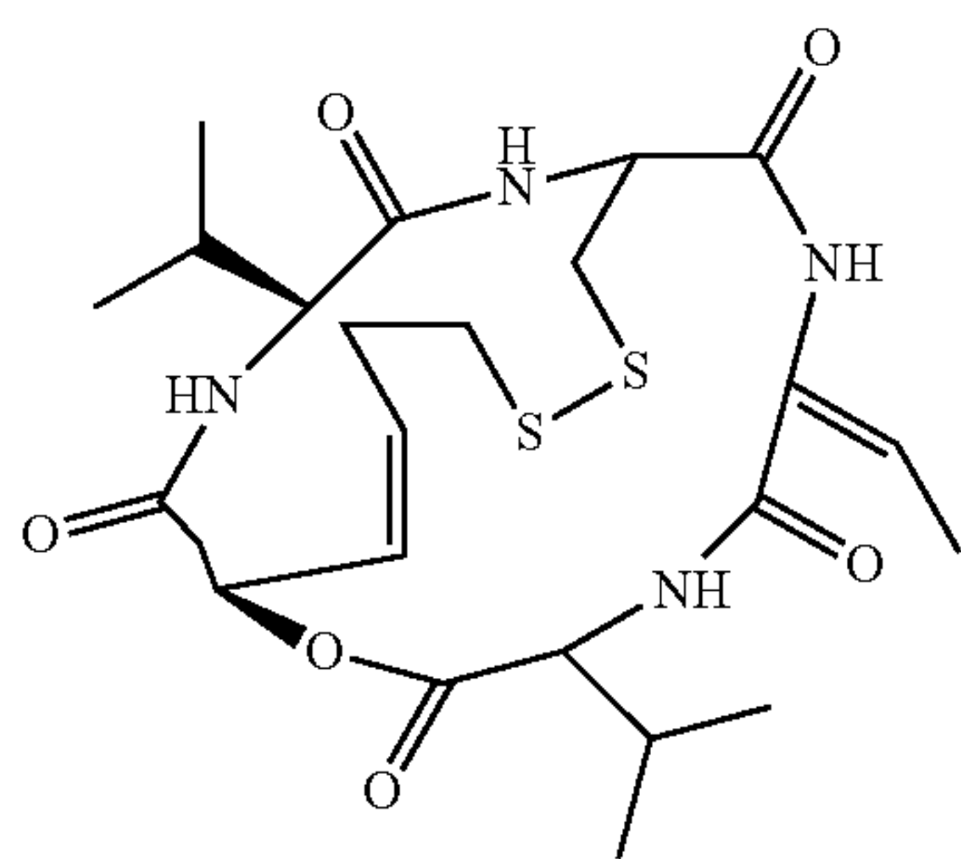
9, FK228
