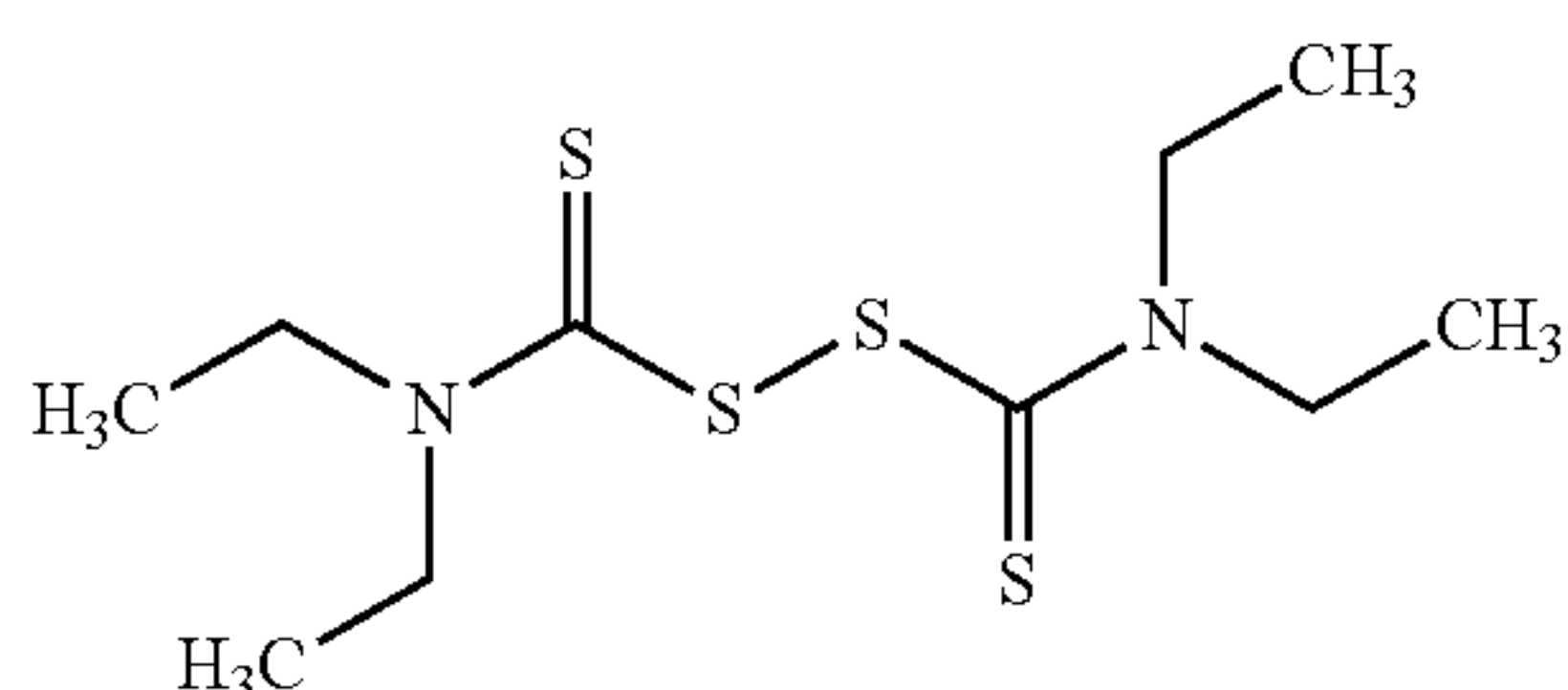
1,1',1'',1'''-[disulfanediy]bis(carbonothioylnitri]l] tetraethane
