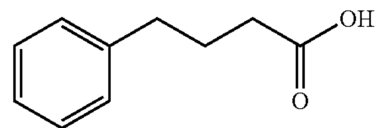
12, Phenylbutyric acid
