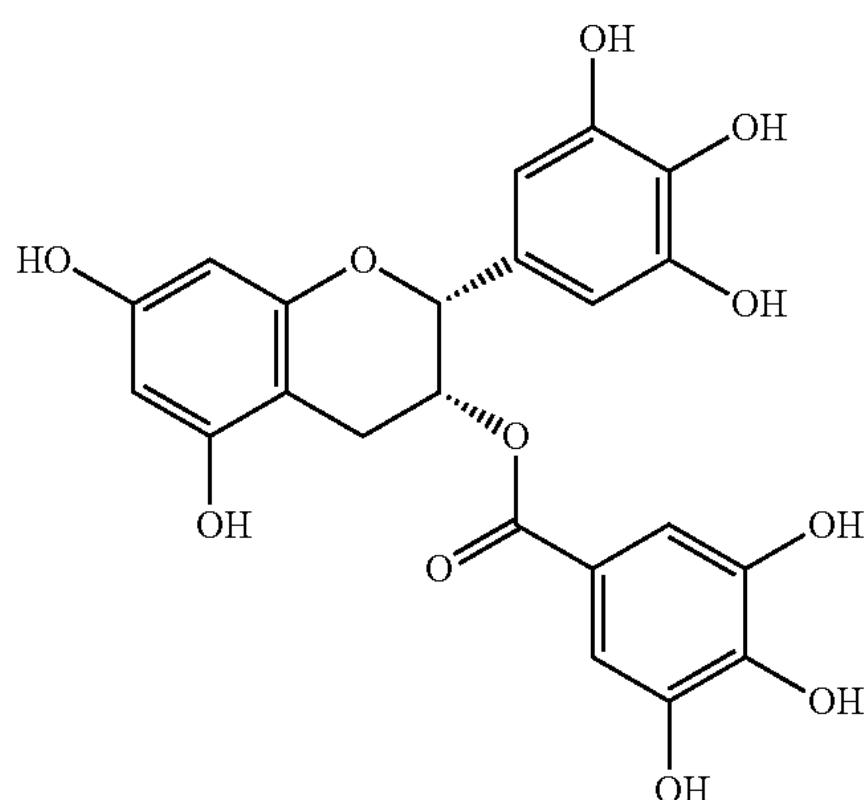
[(2R,3R)-5,7-dihydroxy-2-(3,4,5-trihydroxyphenyl)chroman-3-yl]3,4,5-trihydroxybenzoate
