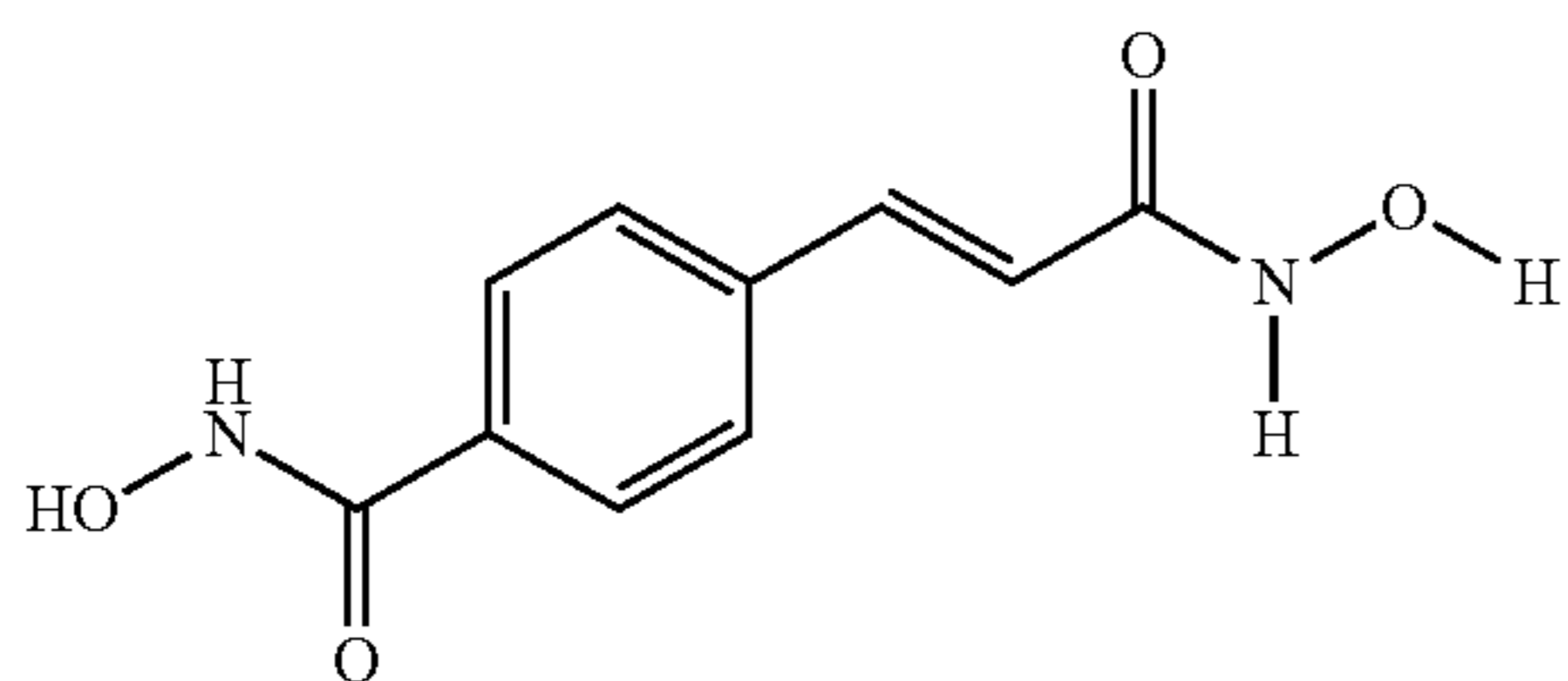
7, CBHA
