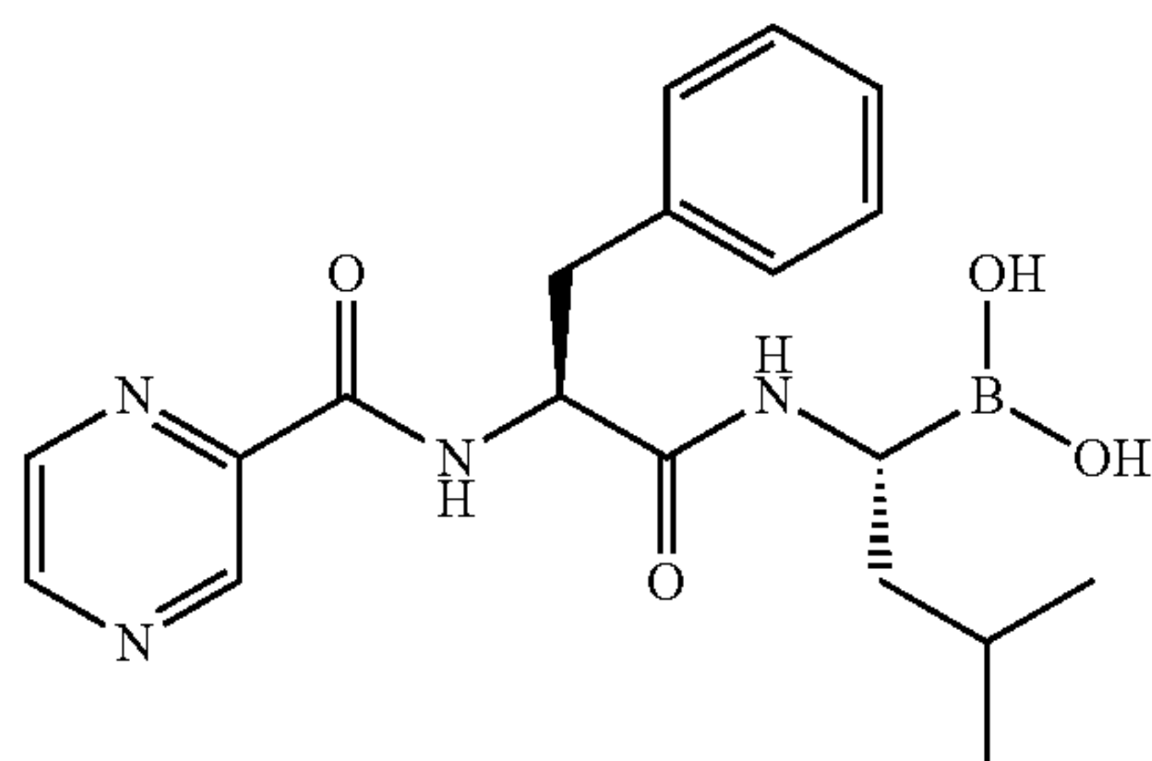
[(1R)-3-methyl-1-({(2S)-3-phenyl-2-[(pyrazin-2-ylcarbonyl)amino]propanoyl}amino)butyl]boronic acid
